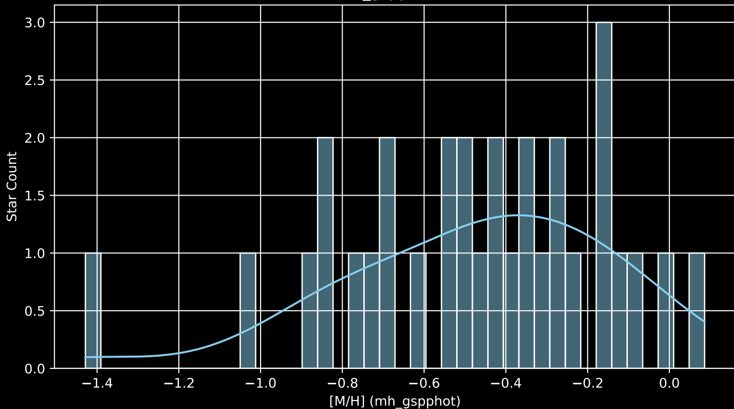
Gaia Cluster: [FSR_0667 [M/H] (mh_gspphot) (n= 31)
