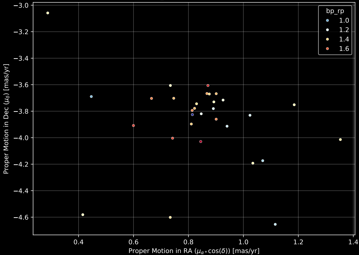
Gaia Cluster: [FSR_0667] Proper Motion Diagram (n= 31)
