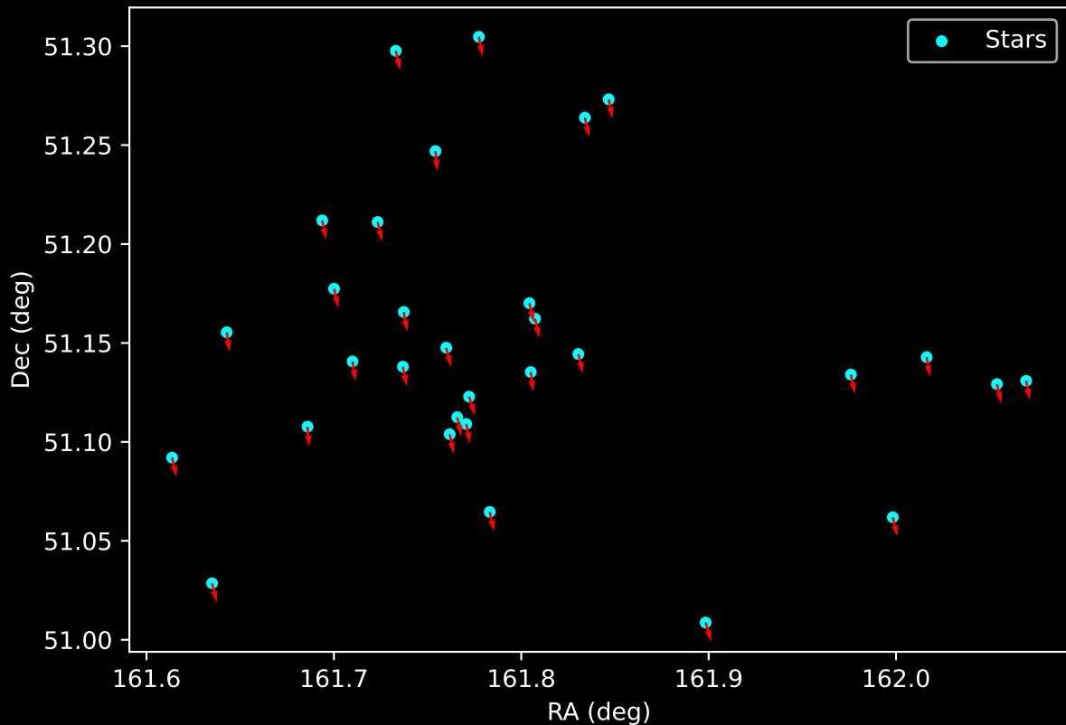
Gaia Cluster: [FSR_0667] Proper Motion Vectors for Gaia Star Field (n= 31)
