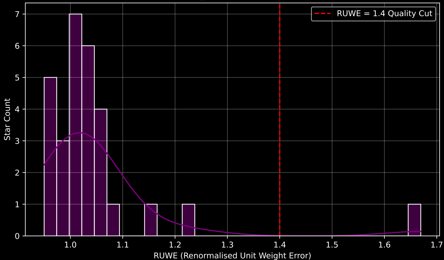
Gaia Cluster: [FSR_0667] RUWE Distribution (n= 29)
