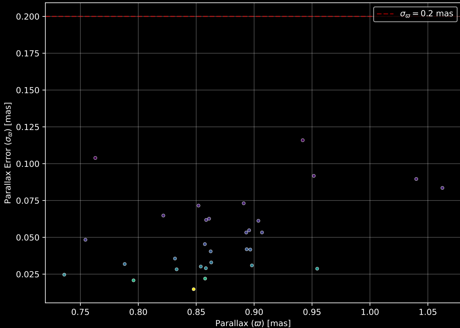
Gaia Cluster: [FSR_0667] Parallax Quality (n= 31)
