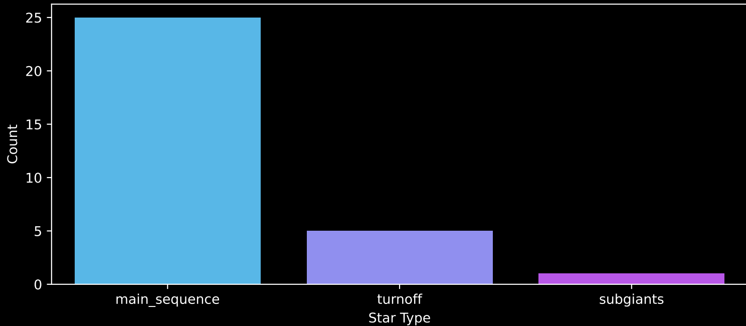
Gaia Cluster: [FSR_0667] Count plot of Star Type
