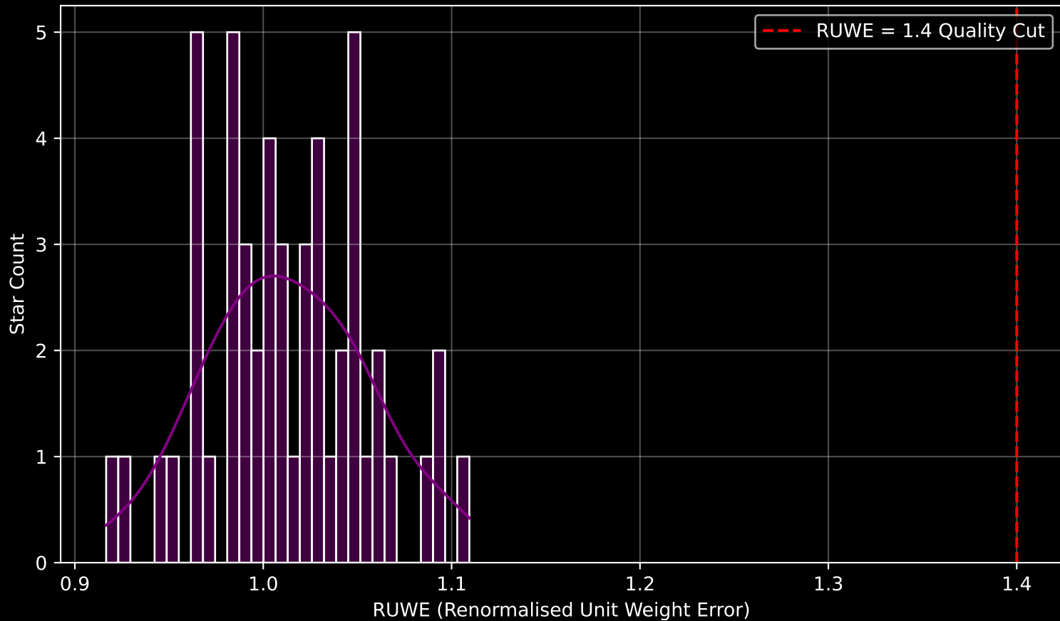
Gaia Cluster: [FSR_0683] RUWE Distribution (n= 51)
