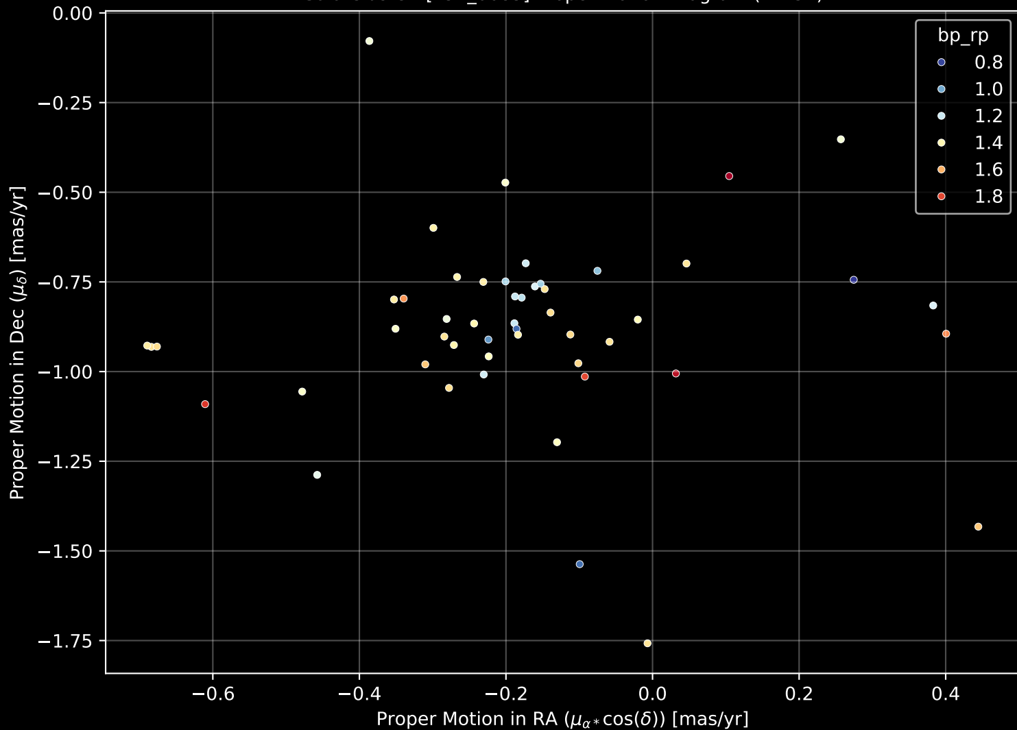
Gaia Cluster: [FSR_0683] Proper Motion Diagram (n= 51)
