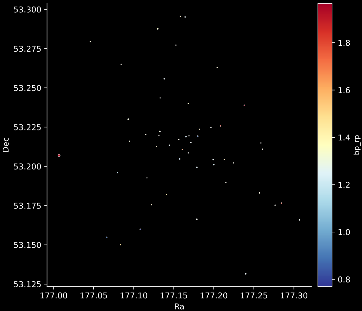
Gaia Cluster: [FSR_0683] Stars: 51
