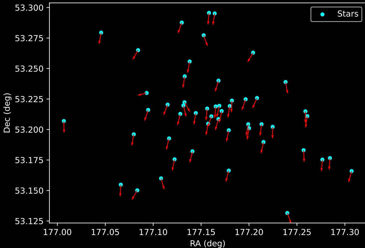
Gaia Cluster: [FSR_0683] Proper Motion Vectors for Gaia Star Field (n= 51)
