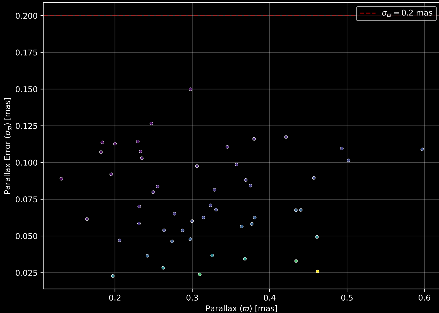
Gaia Cluster: [FSR_0683] Parallax Quality (n= 51)
