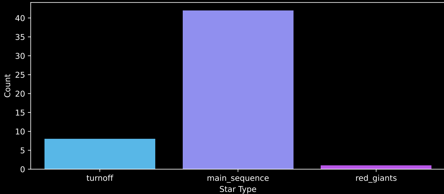
Gaia Cluster: [FSR_0683] Count plot of Star Type
