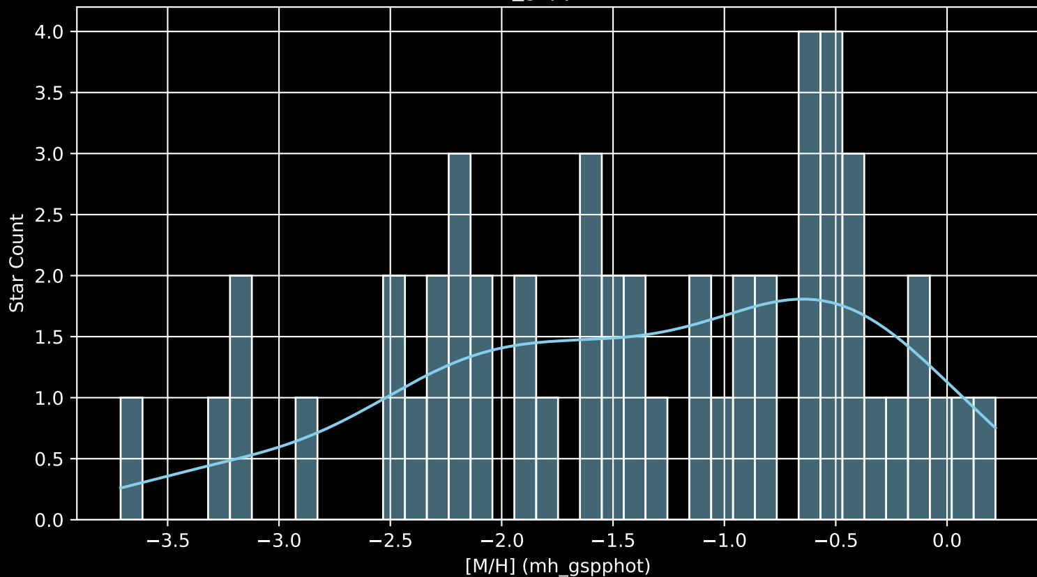
Gaia Cluster: [FSR_0683 [M/H] (mh_gspphot) (n= 51)
