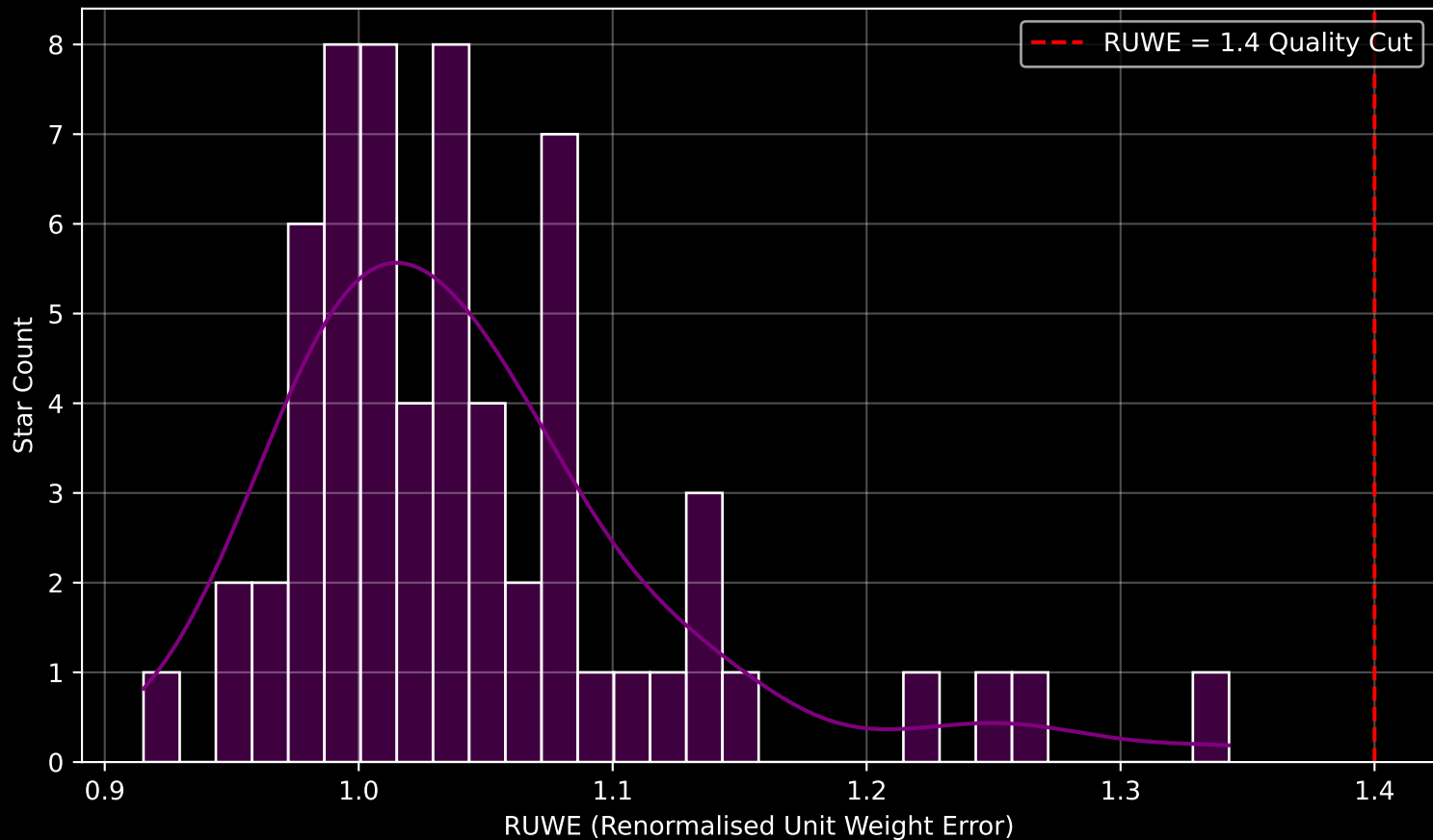
Gaia Cluster: [FSR_0686] RUWE Distribution (n= 63)
