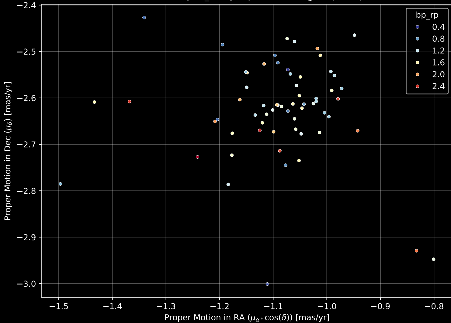
Gaia Cluster: [FSR_0686] Proper Motion Diagram (n= 63)
