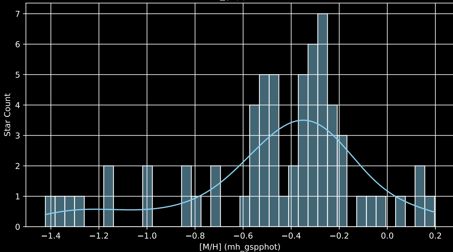
Gaia Cluster: [FSR_0686 [M/H] (mh_gspphot) (n= 63)
