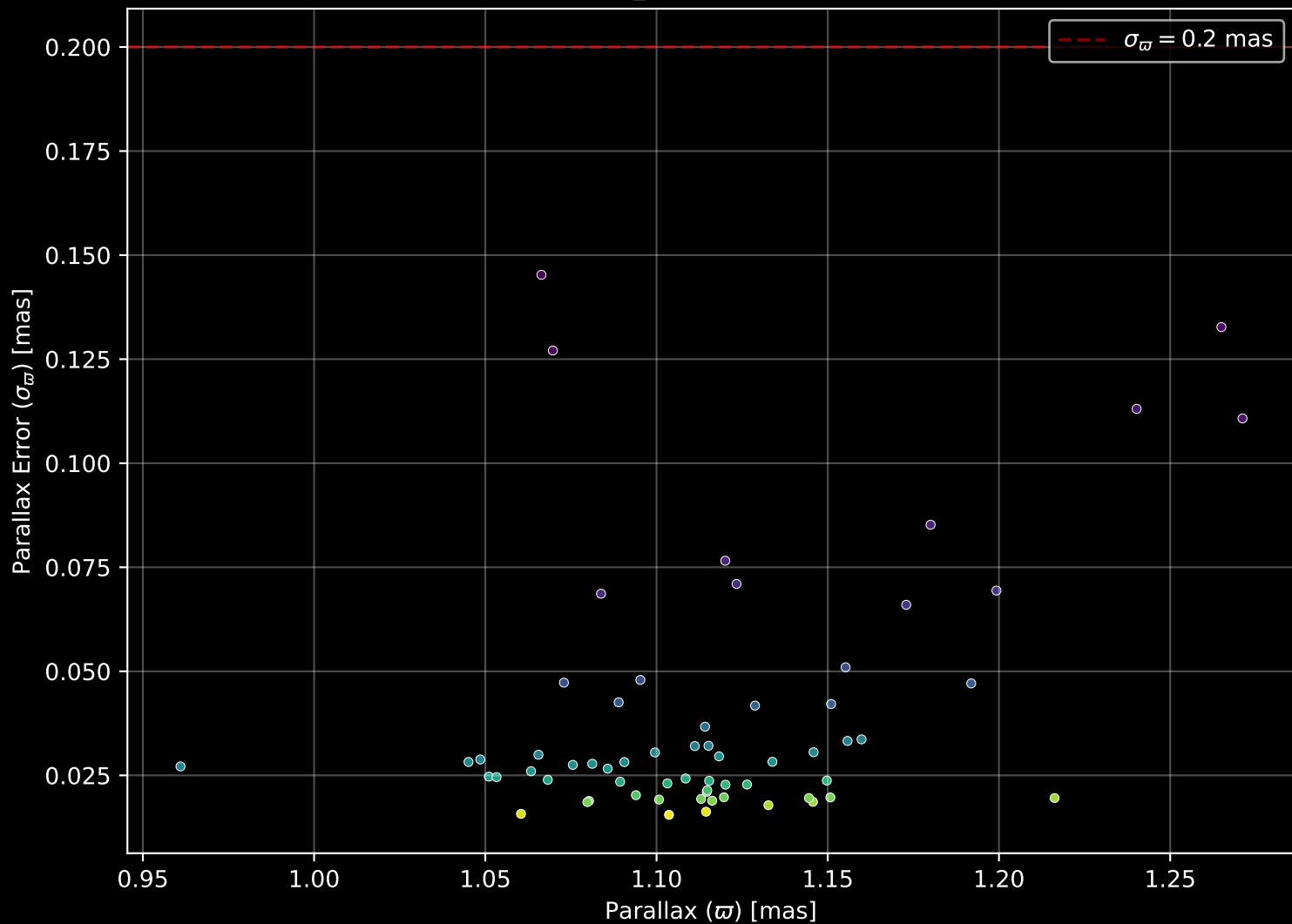
Gaia Cluster: [FSR_0686] Parallax Quality (n= 63)
