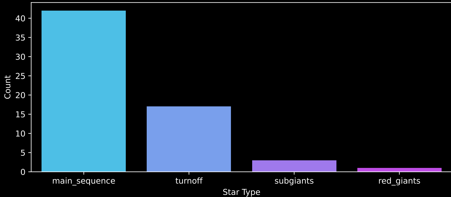
Gaia Cluster: [FSR_0686] Count plot of Star Type
