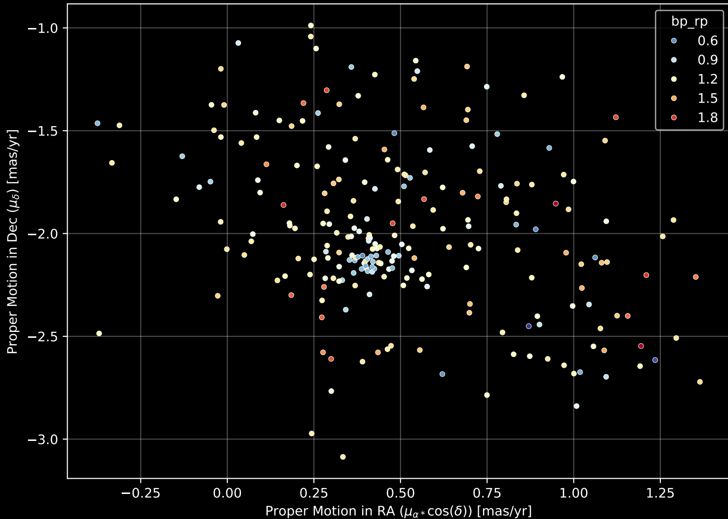
Gaia Cluster: [FSR_0735] Proper Motion Diagram (n= 237)
