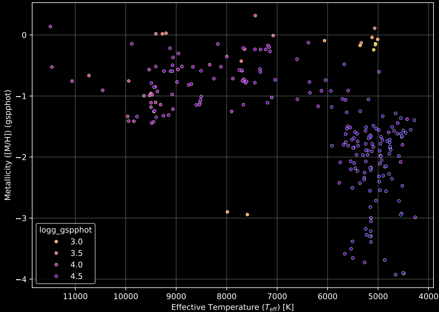
Gaia Cluster: [FSR_0735] Stellar Population Parameters (n= 237)
