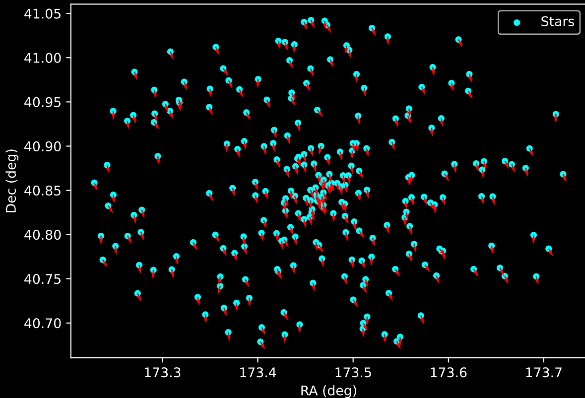
Gaia Cluster: [FSR_0735] Proper Motion Vectors for Gaia Star Field (n= 237)
