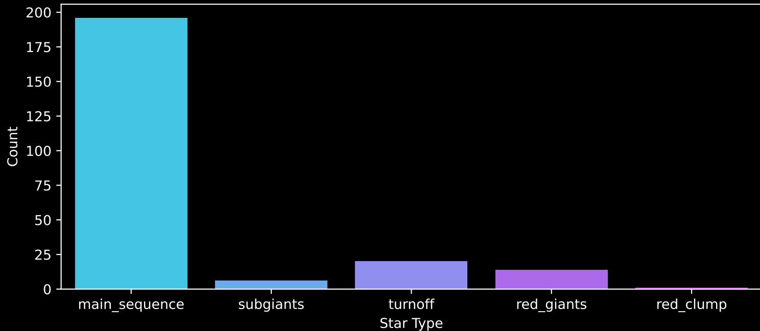
Gaia Cluster: [FSR_0735] Count plot of Star Type
