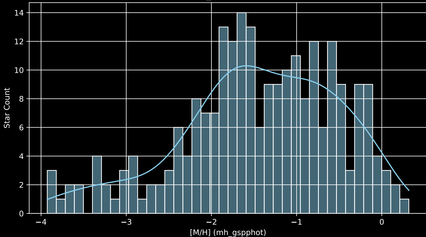
Gaia Cluster: [FSR_0735 [M/H] (mh_gspphot) (n= 237)
