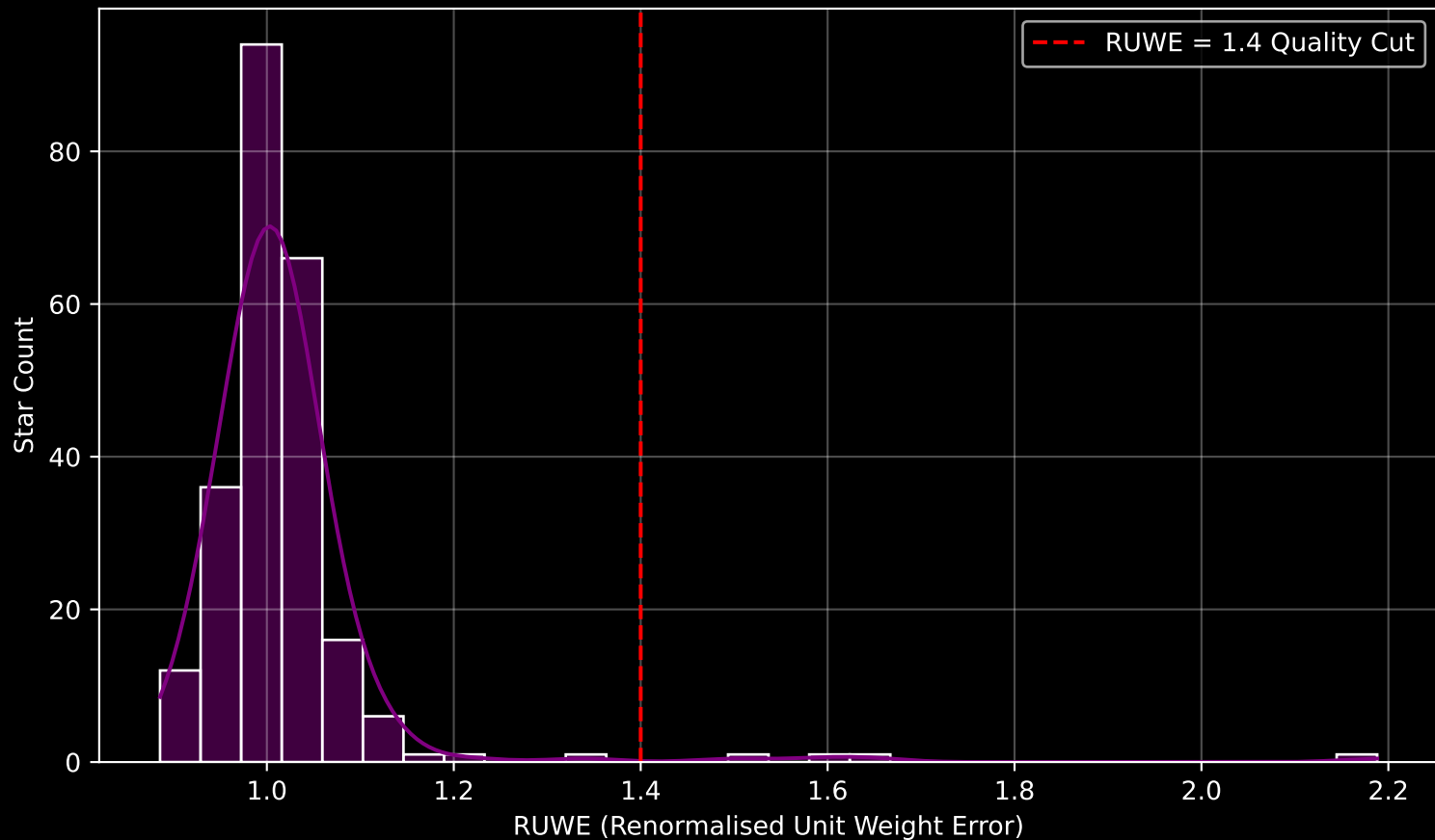
Gaia Cluster: [FSR_0735] RUWE Distribution (n= 237)
