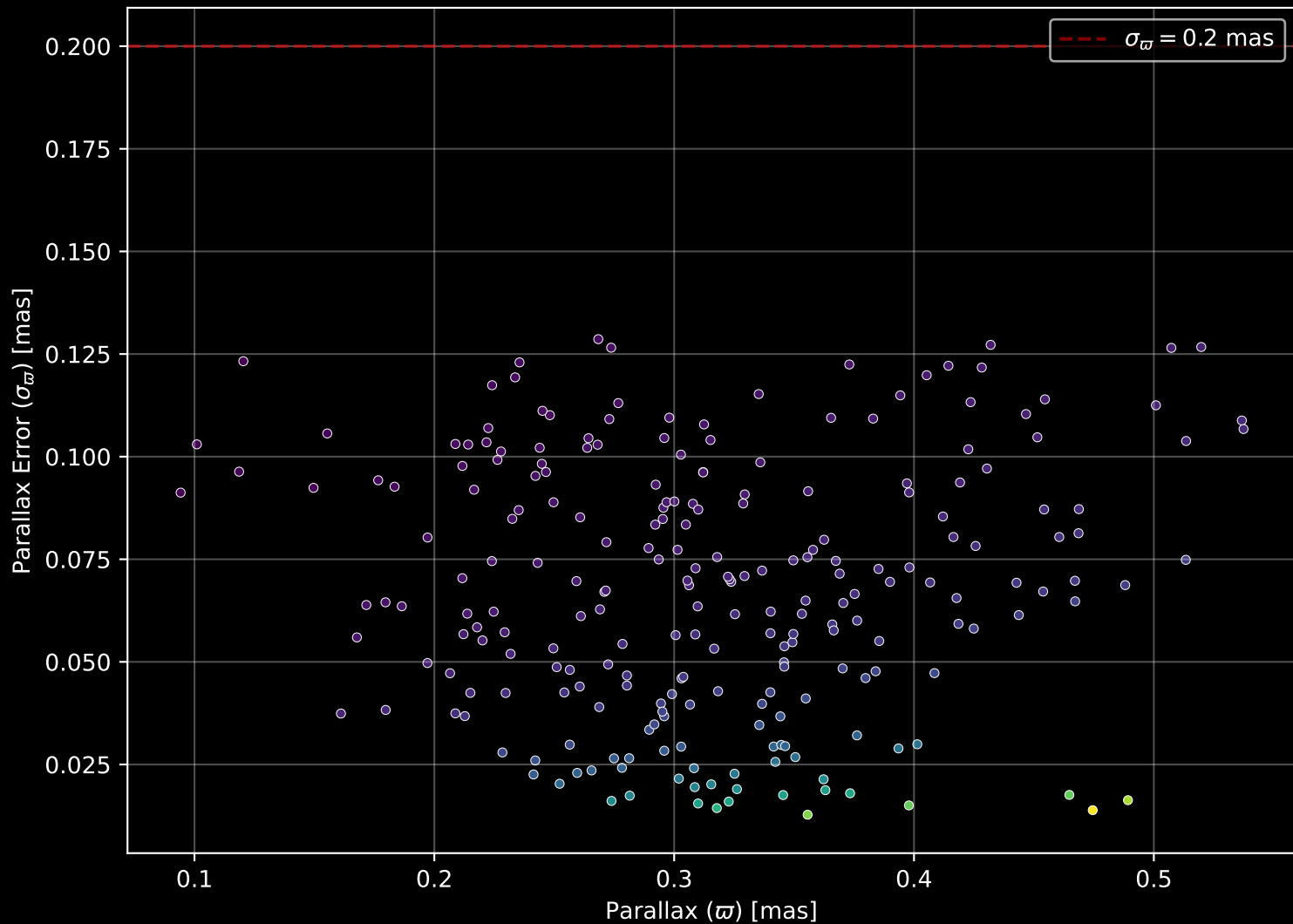
Gaia Cluster: [FSR_0735] Parallax Quality (n= 237)
