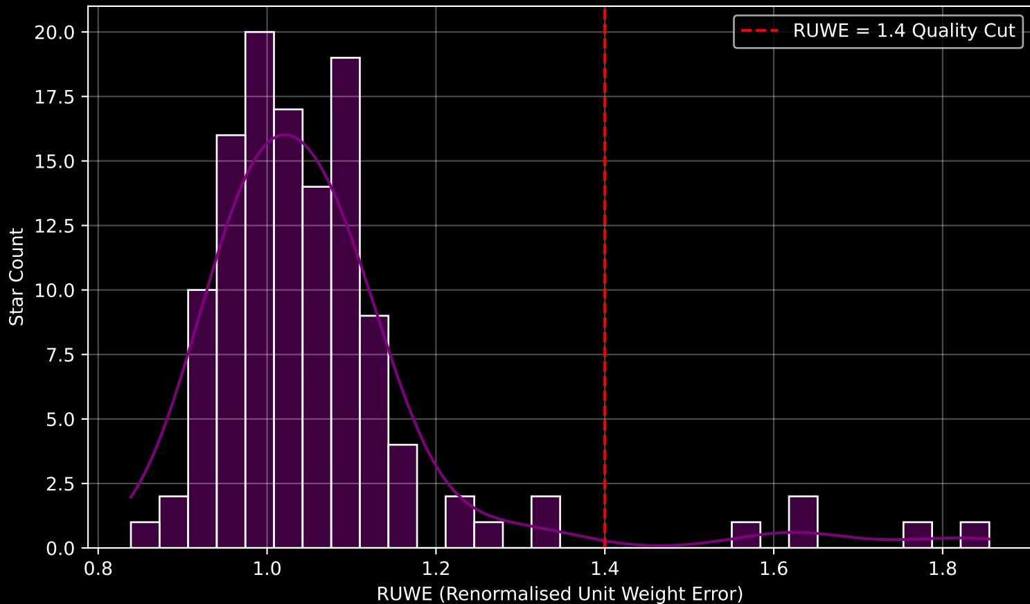
Gaia Cluster: [FSR_0866] RUWE Distribution (n= 122)
