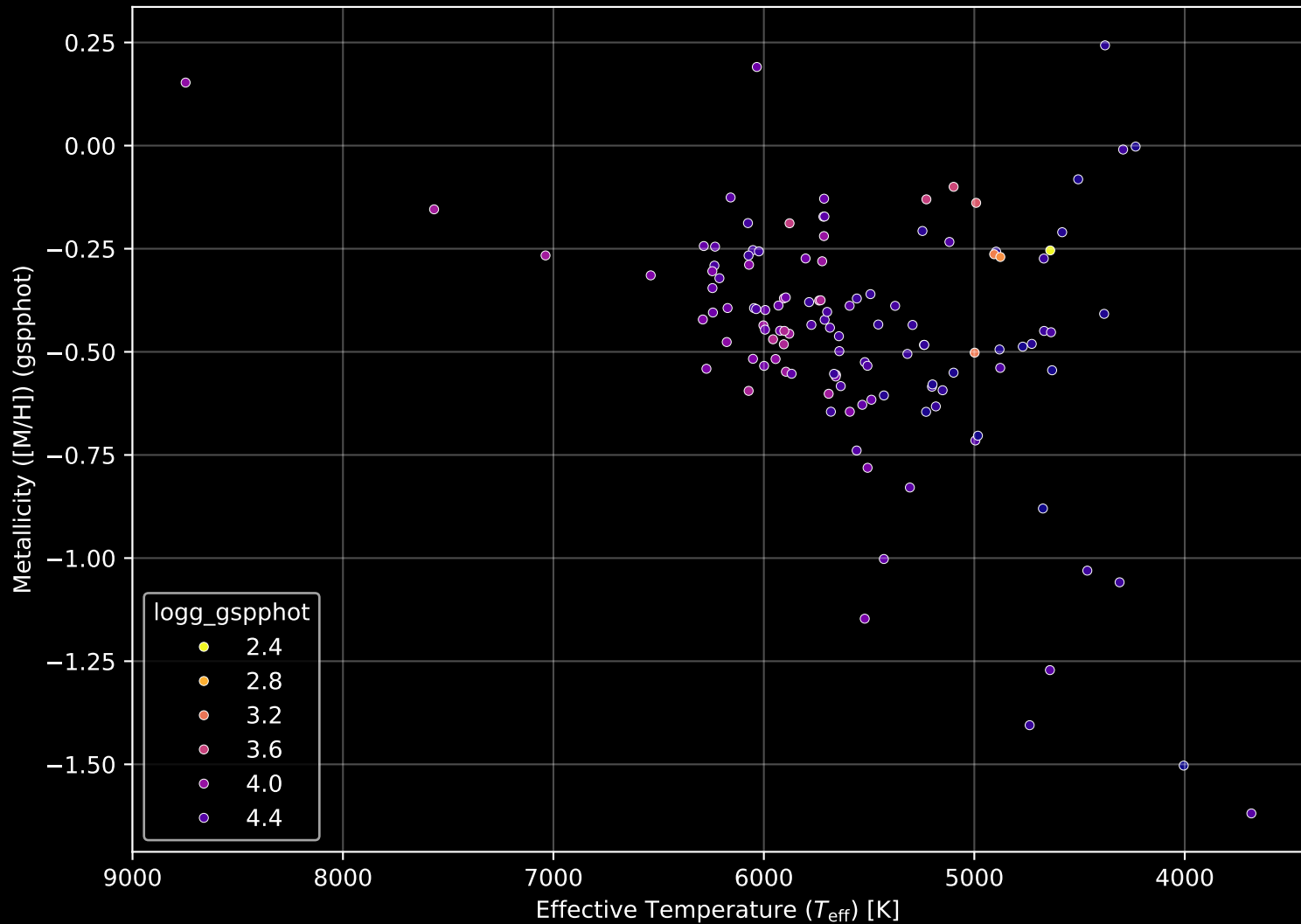
Gaia Cluster: [FSR_0866] Stellar Population Parameters (n= 122)
