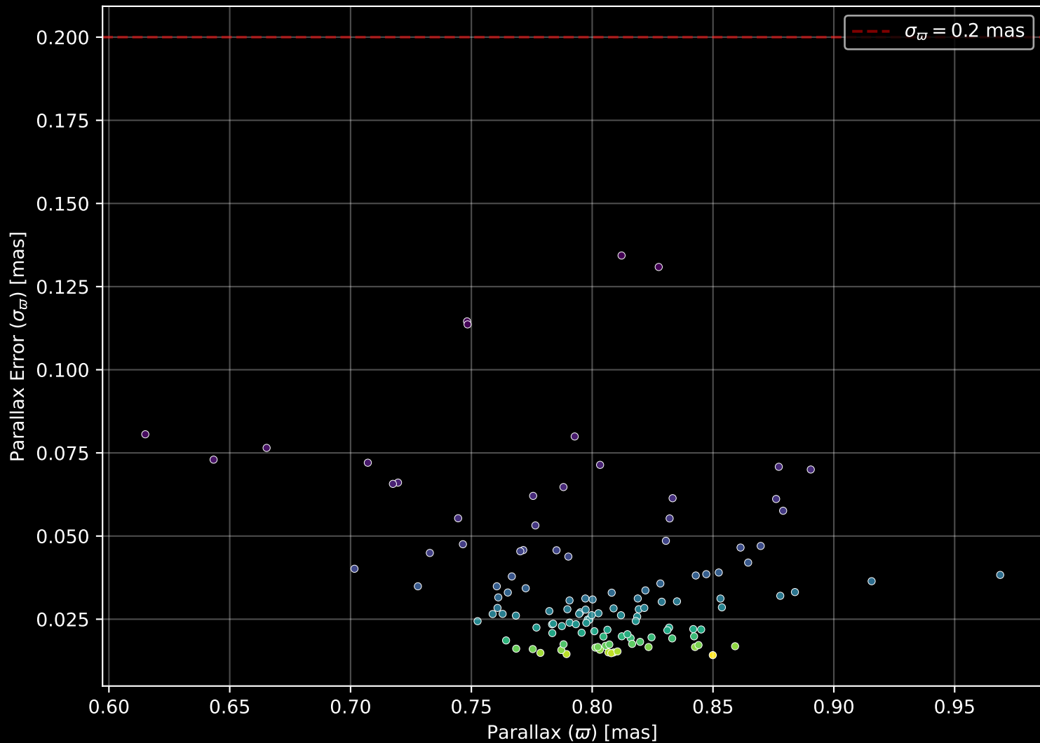
Gaia Cluster: [FSR_0866] Parallax Quality (n= 122)
