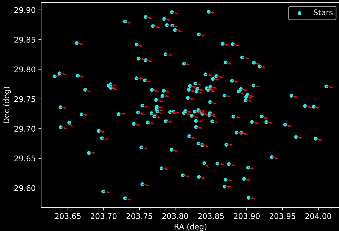
Gaia Cluster: [FSR_0866] Proper Motion Vectors for Gaia Star Field (n= 122)
