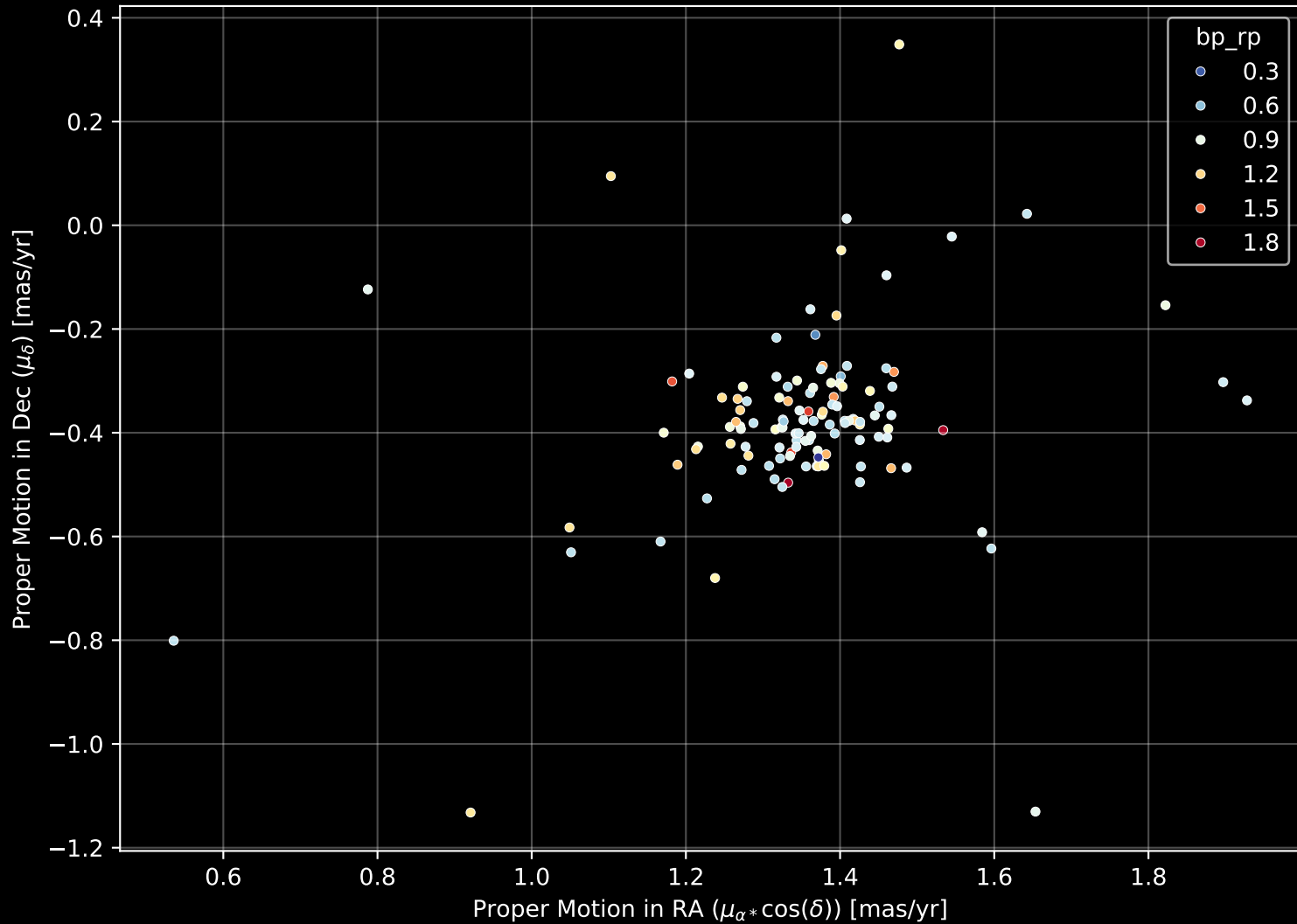
Gaia Cluster: [FSR_0866] Proper Motion Diagram (n= 122)
