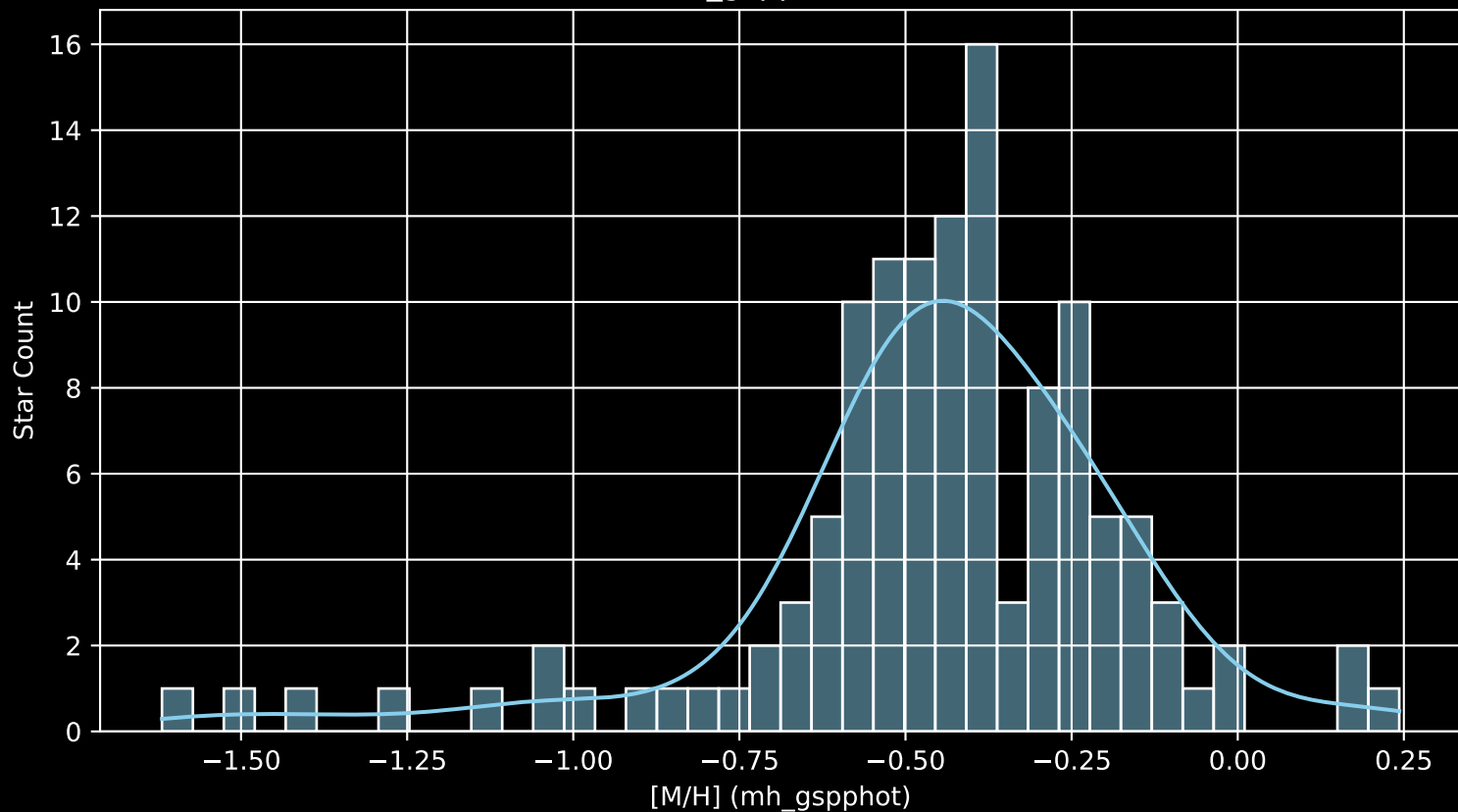
Gaia Cluster: [FSR_0866 [M/H] (mh_gspphot) (n= 122)
