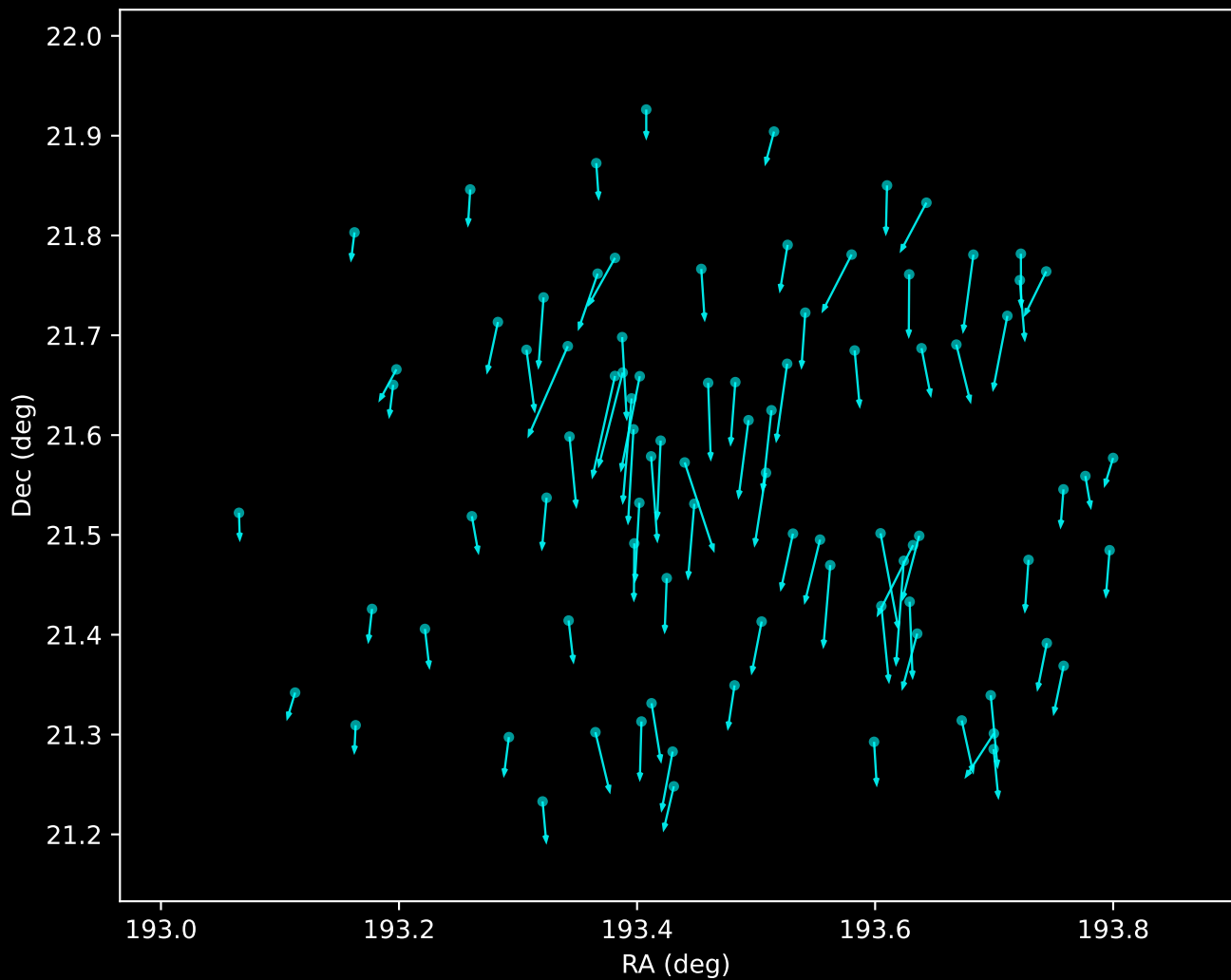
Gaia DR3 Noise Stream Proper Motion Vectors (n=87)
