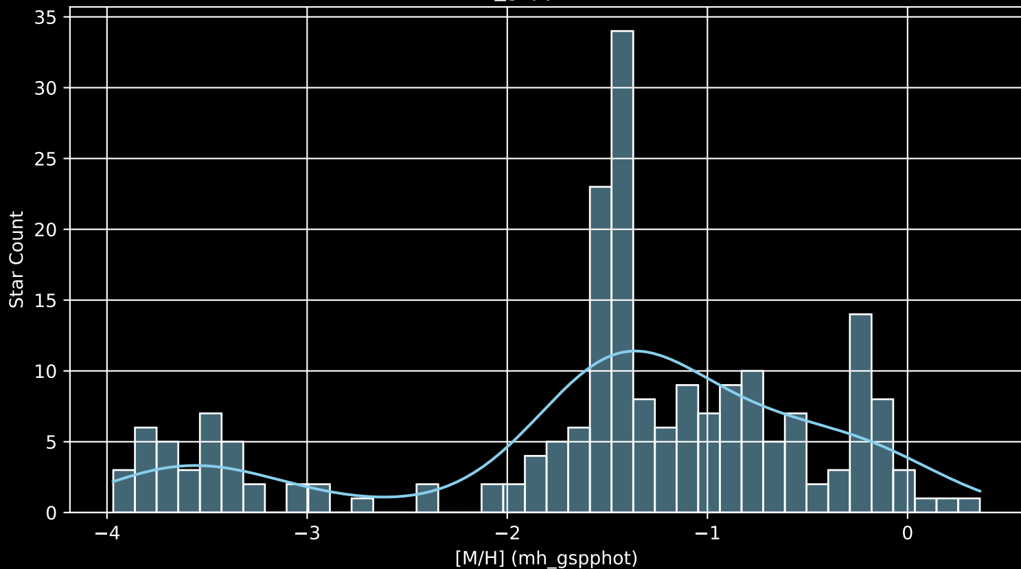
Gaia Cluster: [FSR_0893 [M/H] (mh_gspphot) (n= 208)
