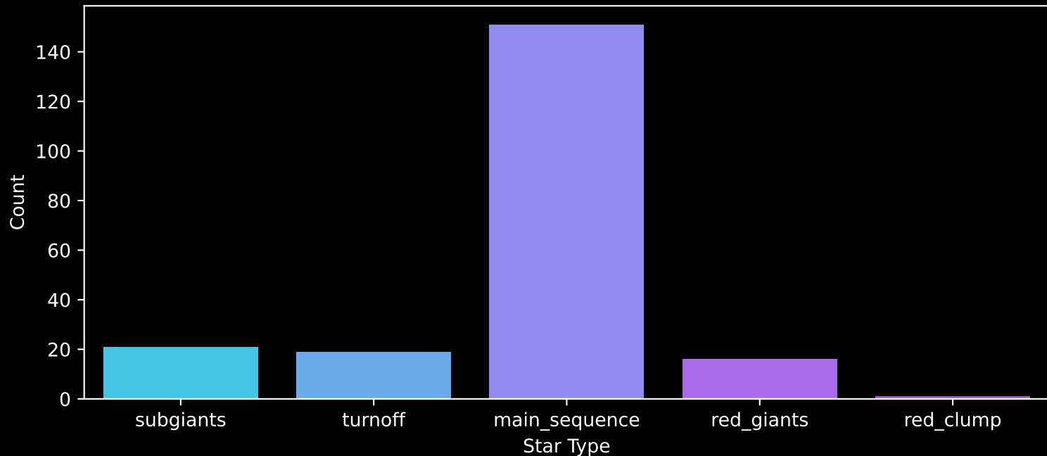
Gaia Cluster: [FSR_0893] Count plot of Star Type
