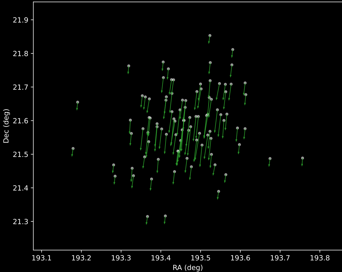
Gaia DR3 Cluster 4 Proper Motion Vectors (n=93)
