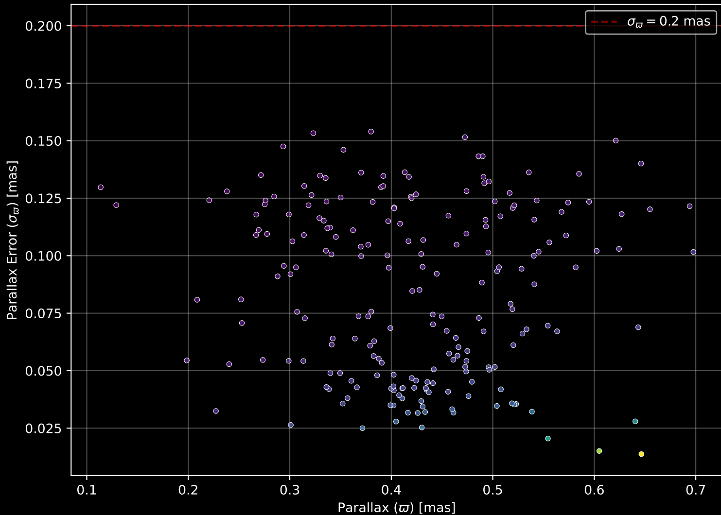
Gaia Cluster: [FSR_0893] Parallax Quality (n= 208)
