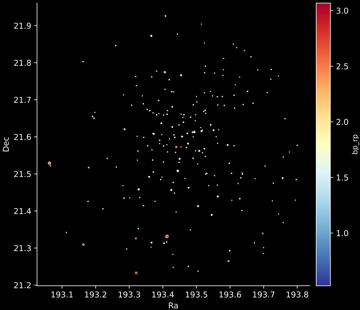
Gaia Cluster: [FSR_0893] Stars: 208
