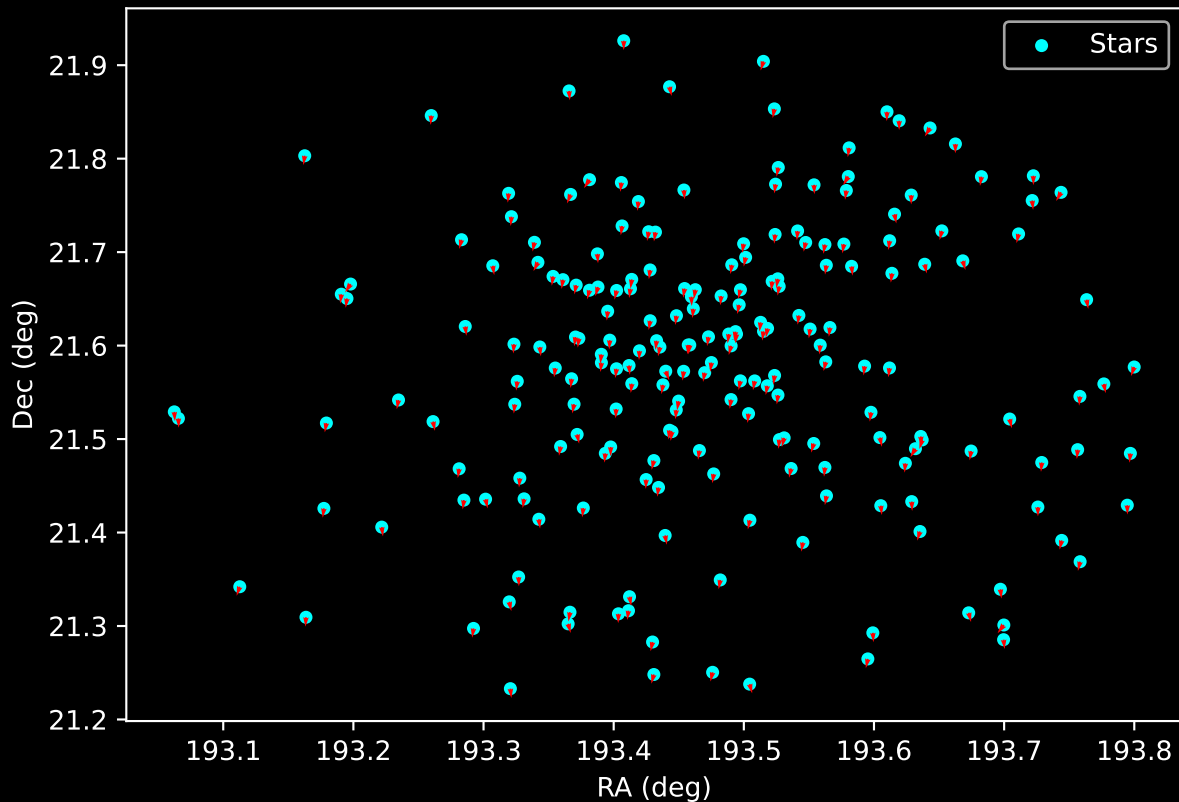
Gaia Cluster: [FSR_0893] Proper Motion Vectors for Gaia Star Field (n= 208)
