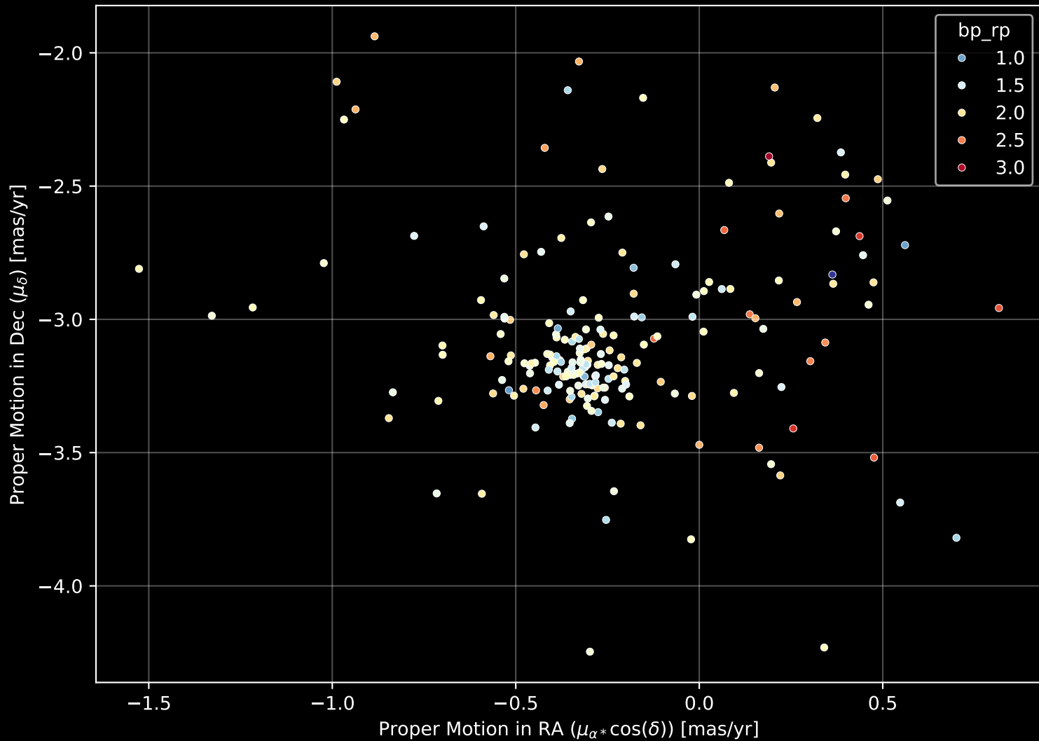
Gaia Cluster: [FSR_0893] Proper Motion Diagram (n= 208)
