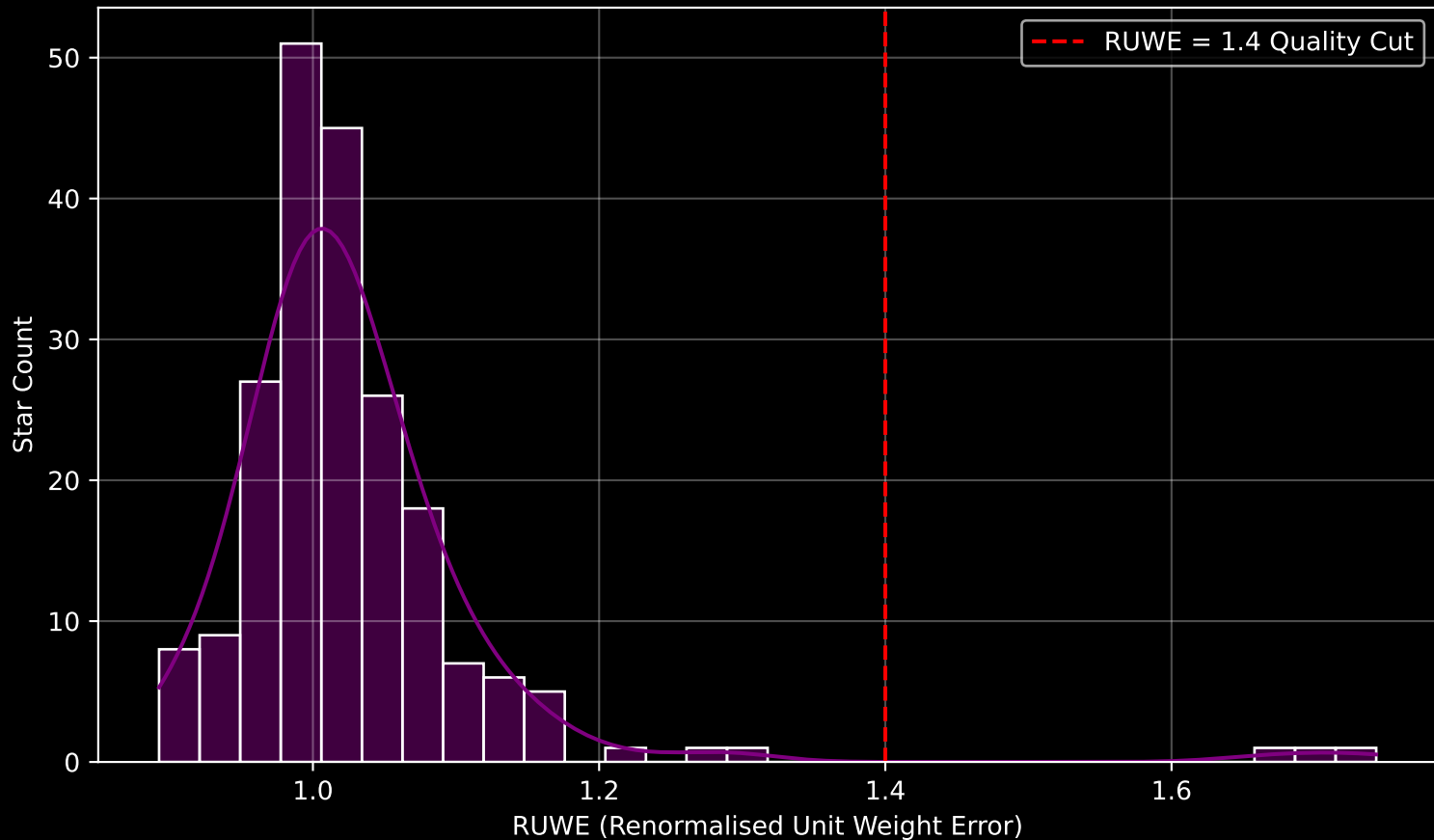
Gaia Cluster: [FSR_0893] RUWE Distribution (n= 208)
