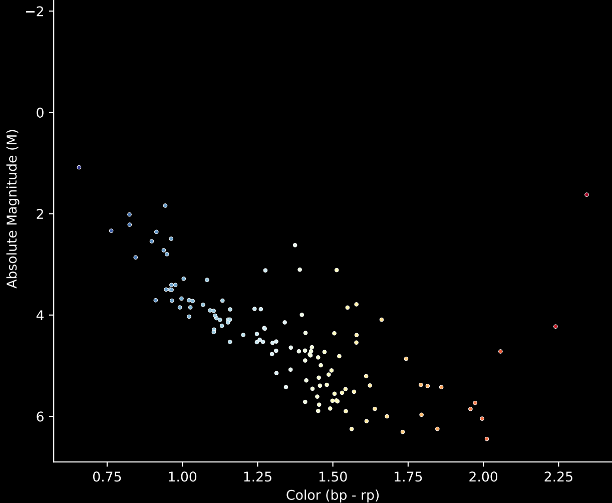
Gaia Cluster: [FSR_0904] Stars (n= 123) Hertzsprung-Russel Diagram
