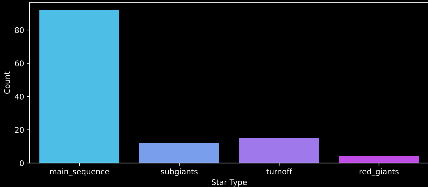
Gaia Cluster: [FSR_0904] Count plot of Star Type
