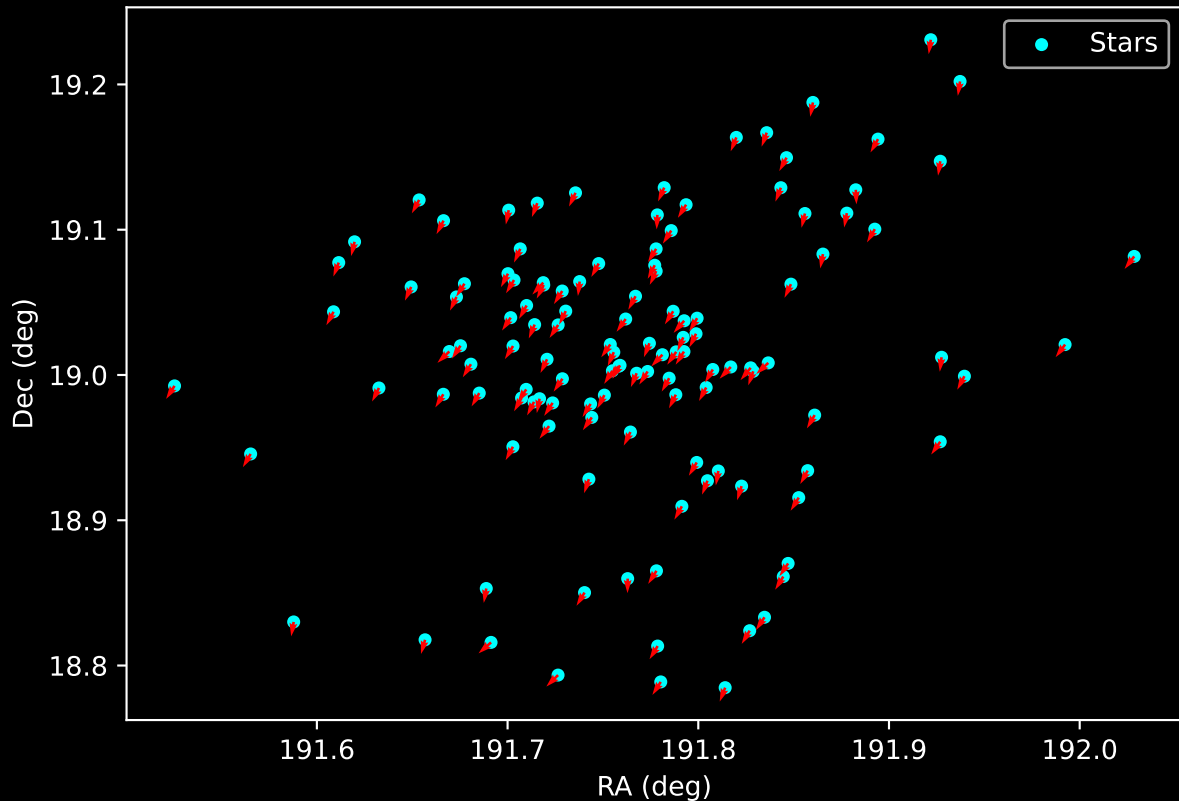
Gaia Cluster: [FSR_0904] Proper Motion Vectors for Gaia Star Field (n= 123)
