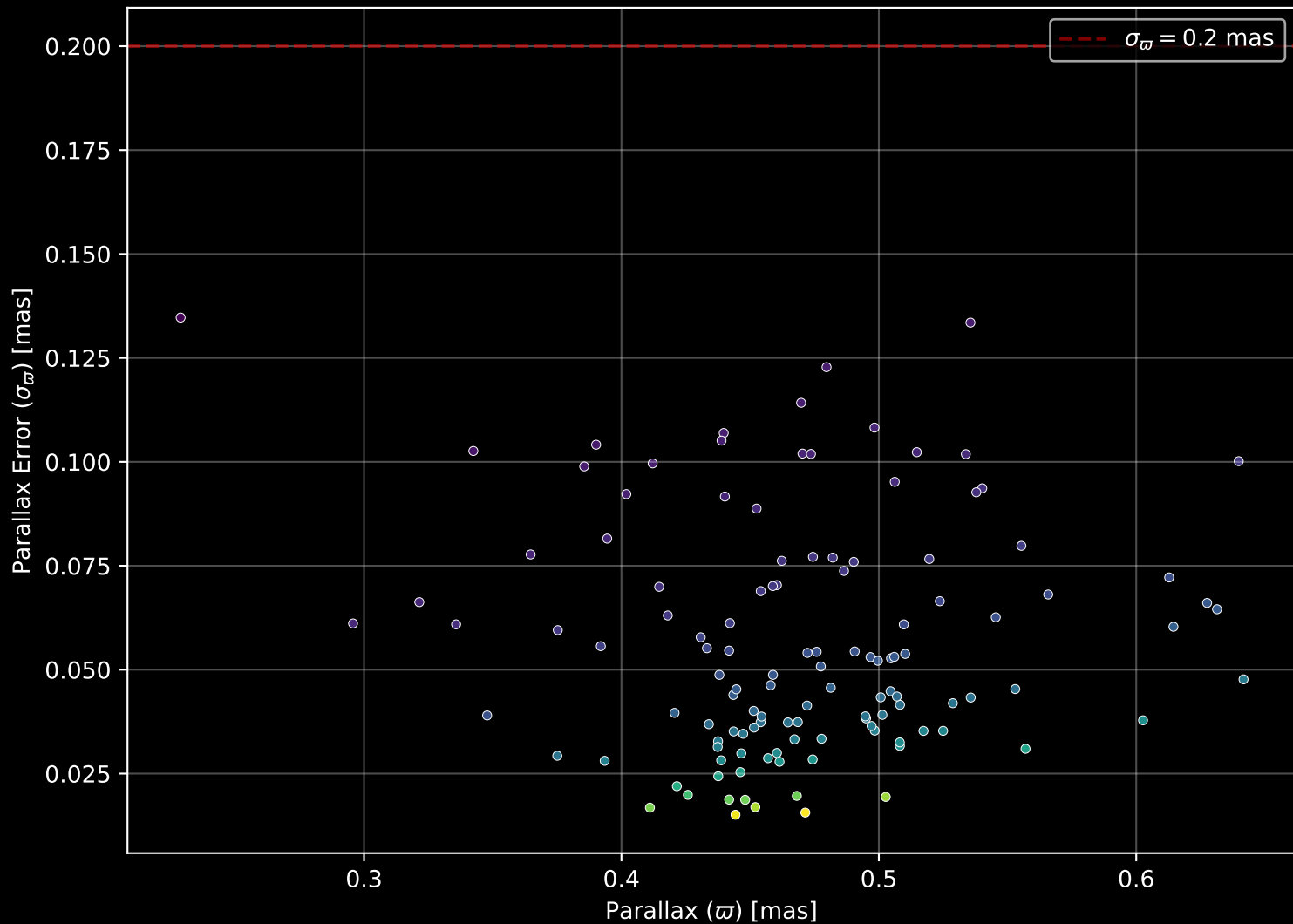
Gaia Cluster: [FSR_0904] Parallax Quality (n= 123)
