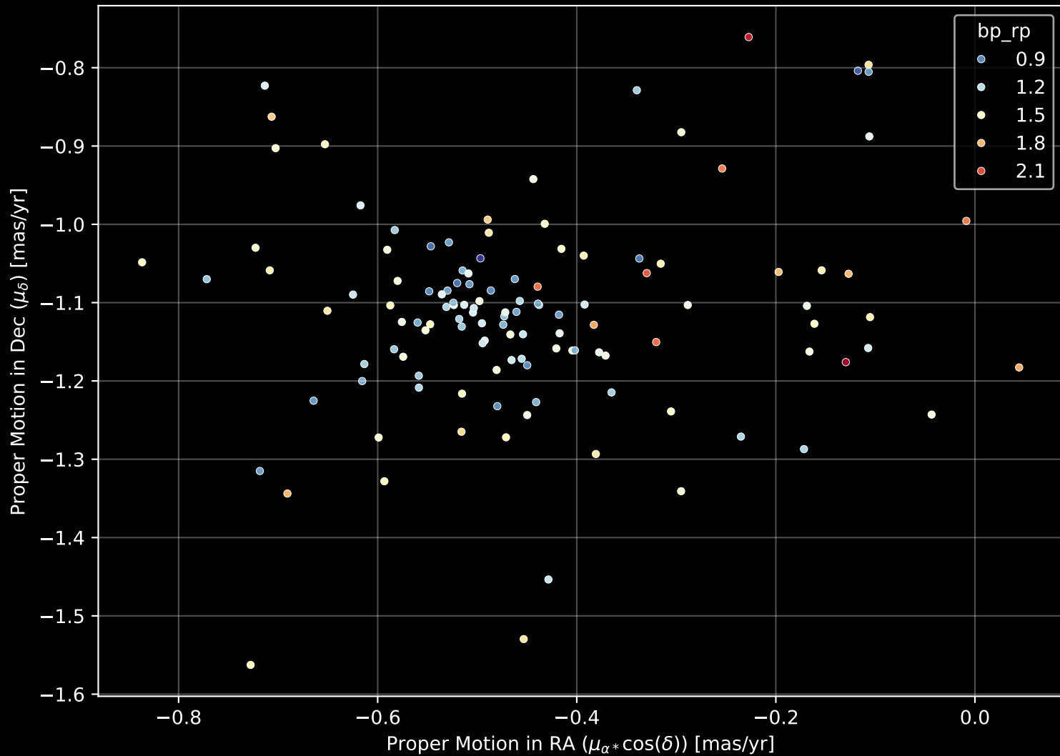
Gaia Cluster: [FSR_0904] Proper Motion Diagram (n= 123)
