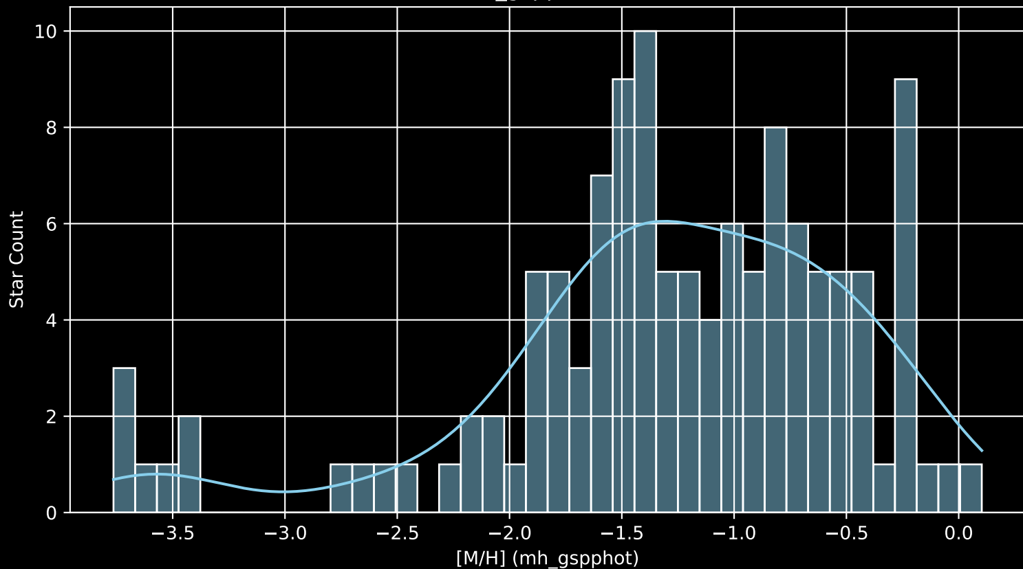
Gaia Cluster: [FSR_0904 [M/H] (mh_gspphot) (n= 123)
