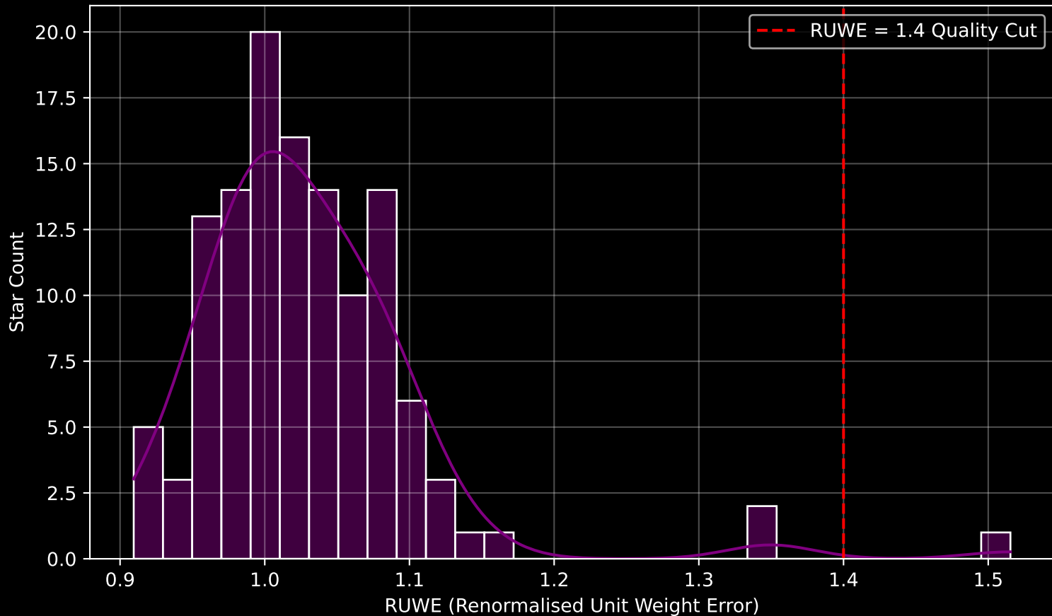
Gaia Cluster: [FSR_0904] RUWE Distribution (n= 123)
