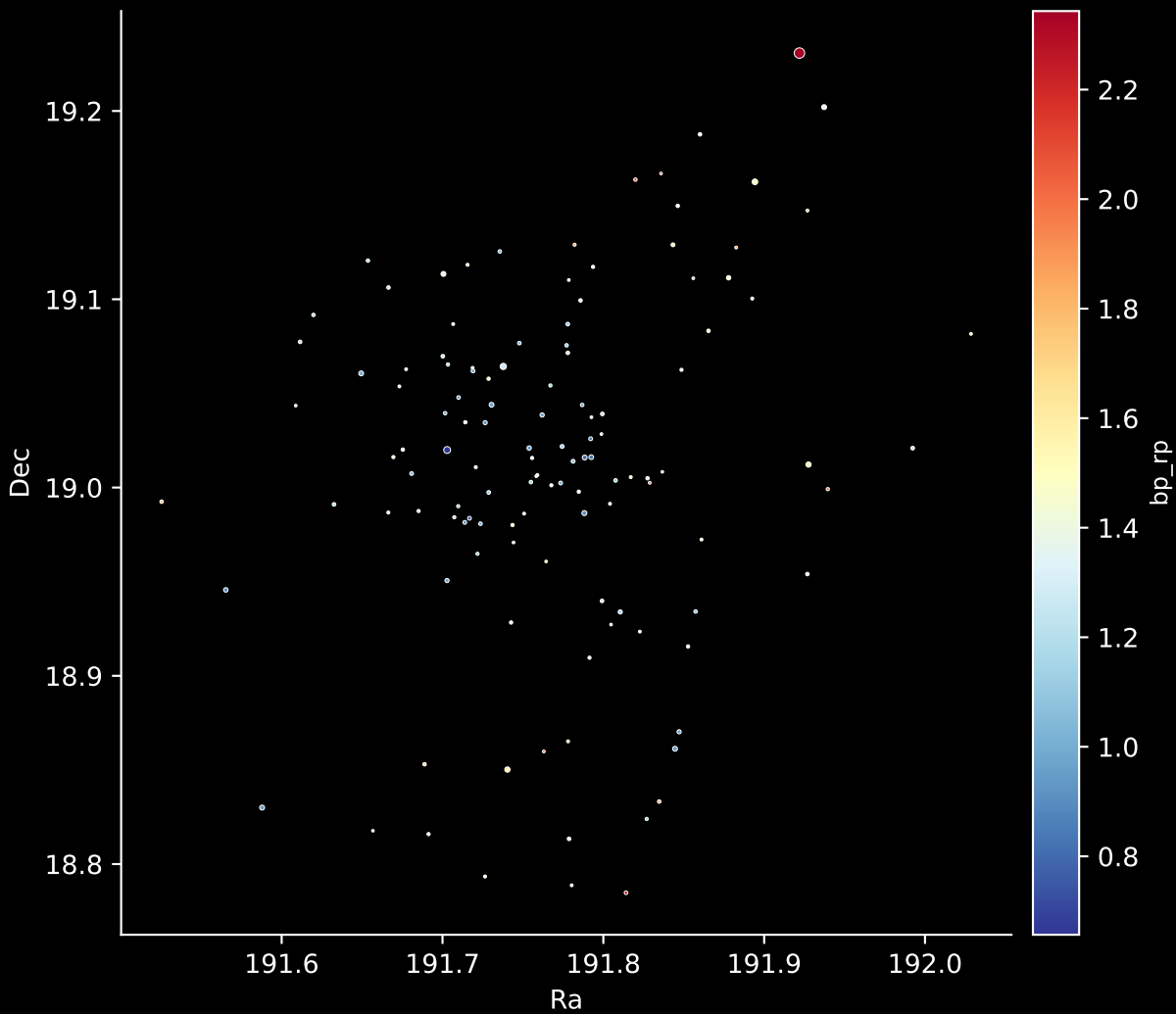
Gaia Cluster: [FSR_0904] Stars: 123
