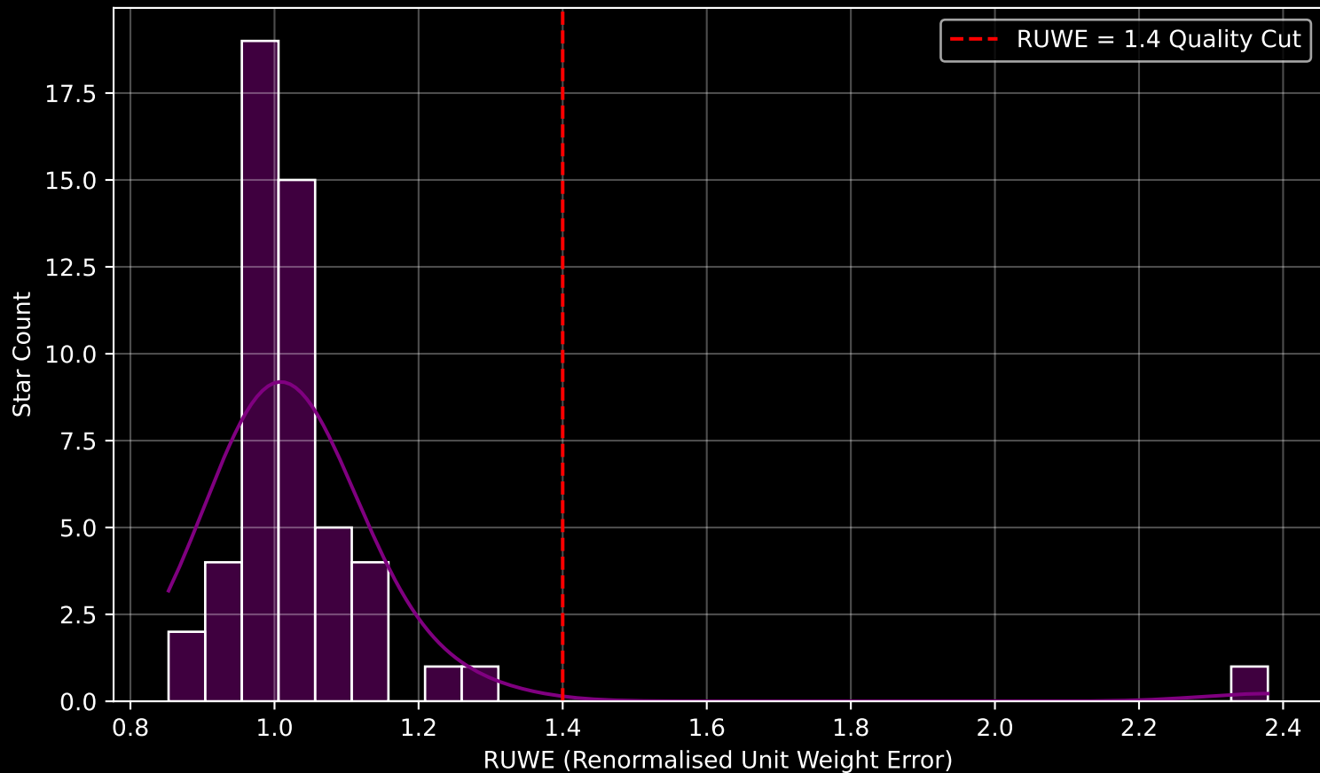
Gaia Cluster: [FSR_0923] RUWE Distribution (n= 52)
