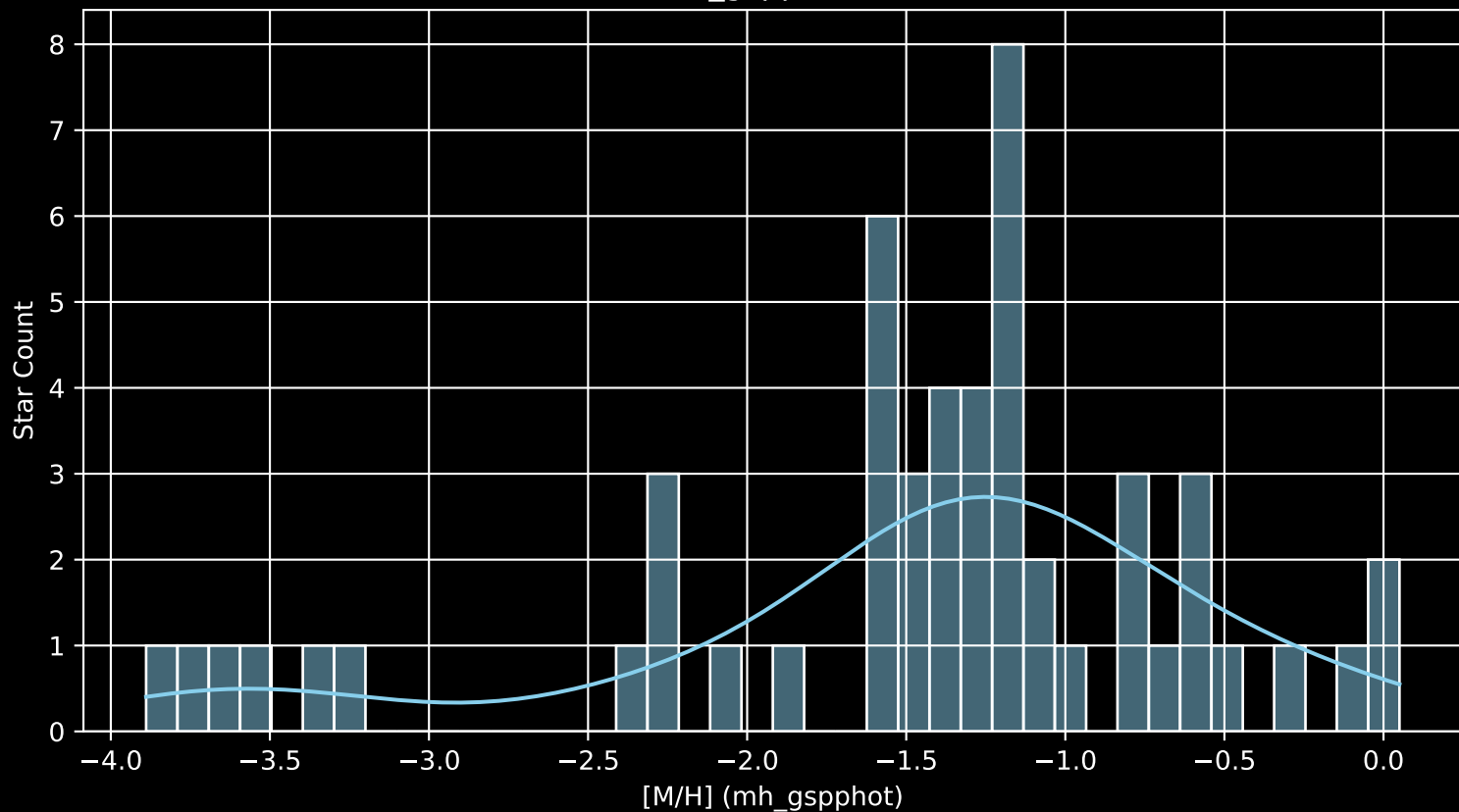
Gaia Cluster: [FSR_0923 [M/H] (mh_gspphot) (n= 52)
