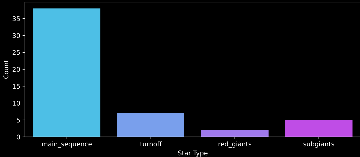
Gaia Cluster: [FSR_0923] Count plot of Star Type
