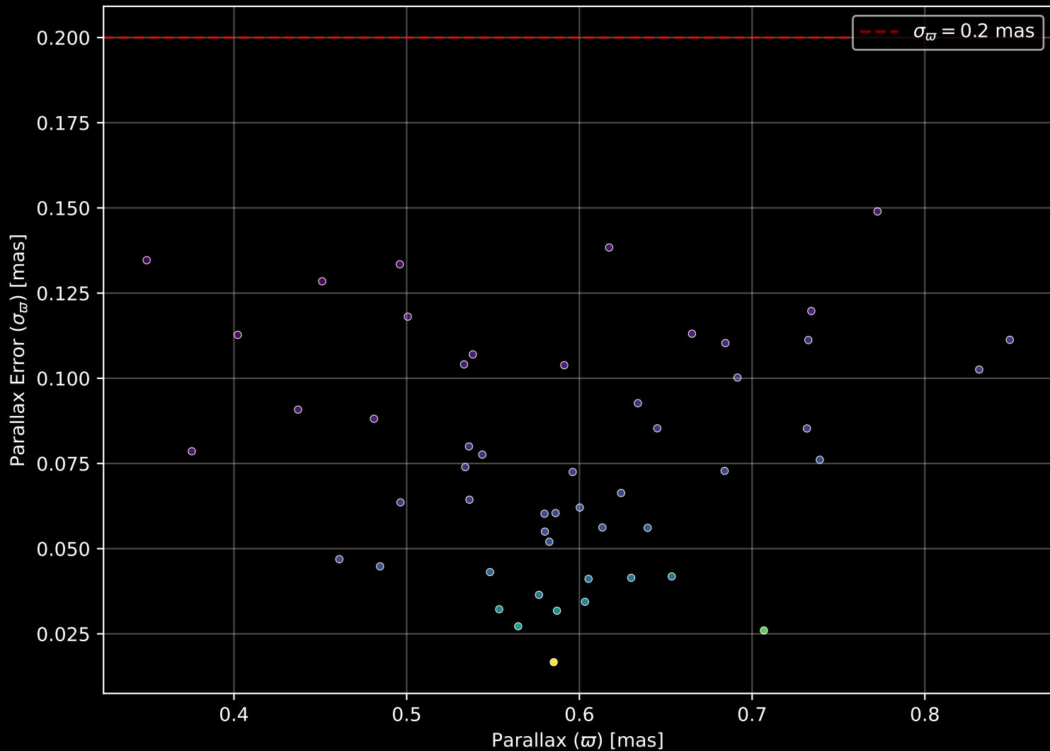
Gaia Cluster: [FSR_0923] Parallax Quality (n= 52)
