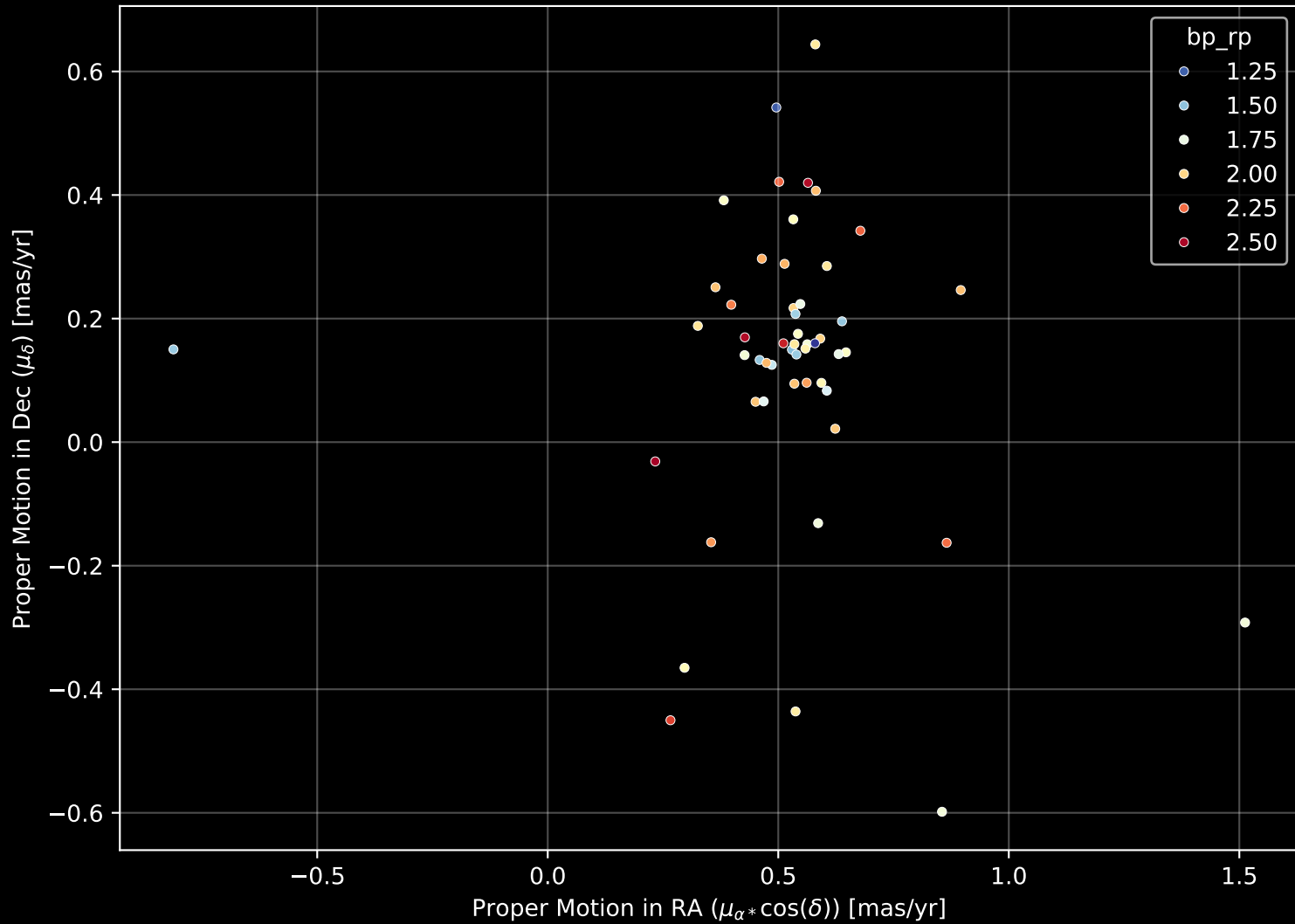
Gaia Cluster: [FSR_0923] Proper Motion Diagram (n= 52)
