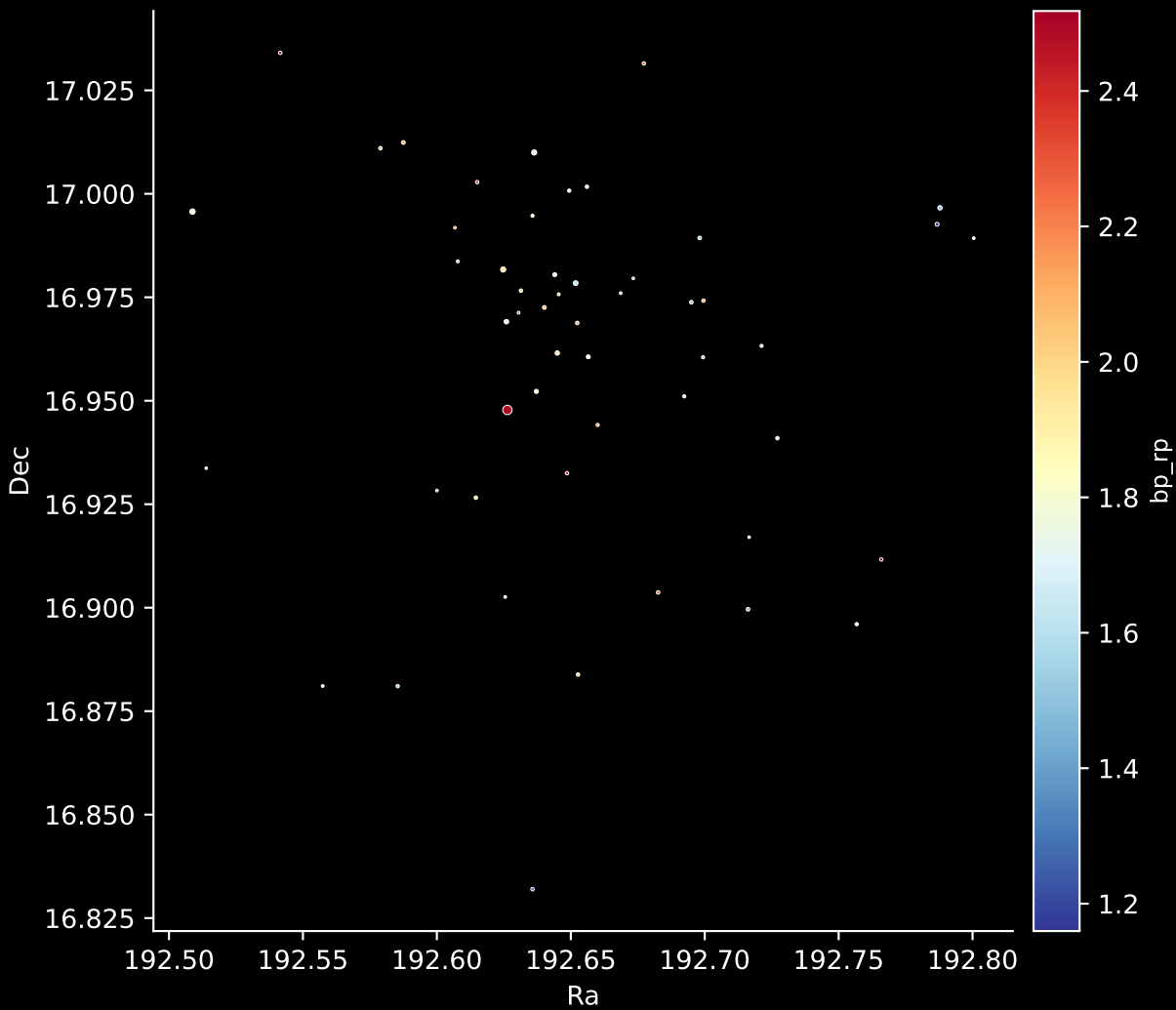
Gaia Cluster: [FSR_0923] Stars: 52
