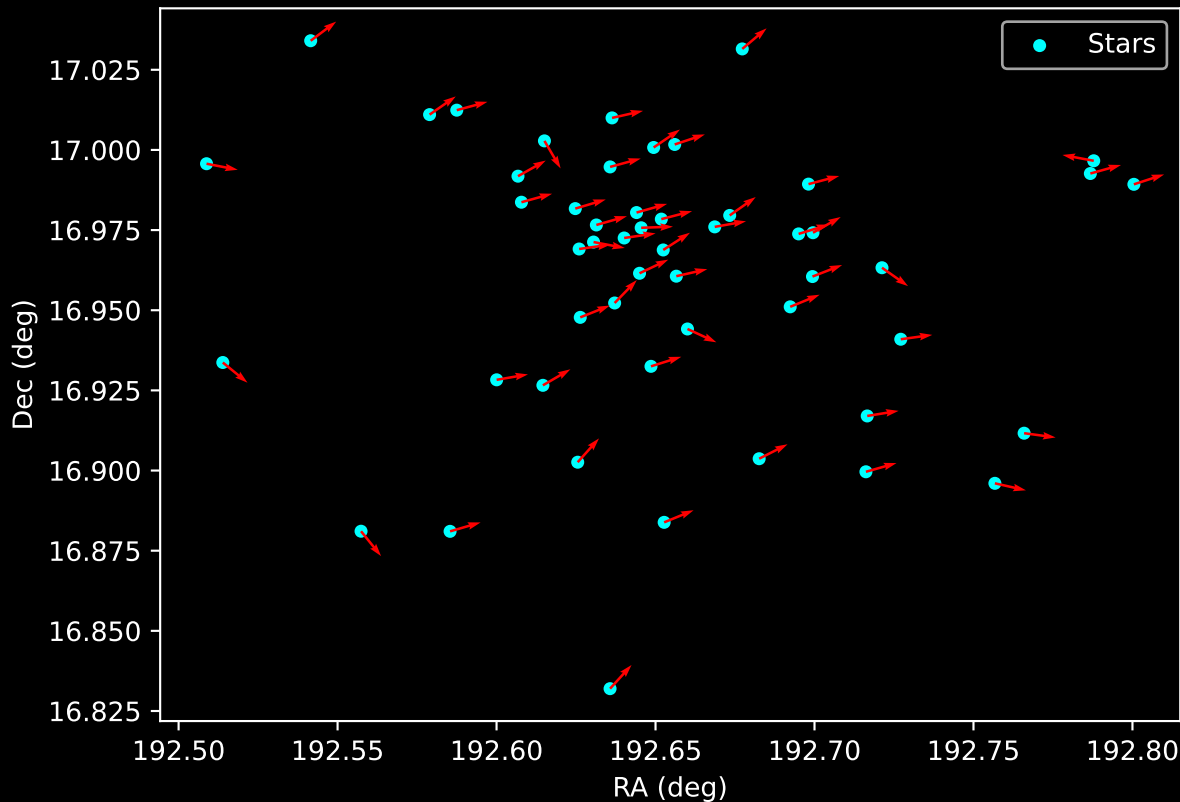
Gaia Cluster: [FSR_0923] Proper Motion Vectors for Gaia Star Field (n= 52)
