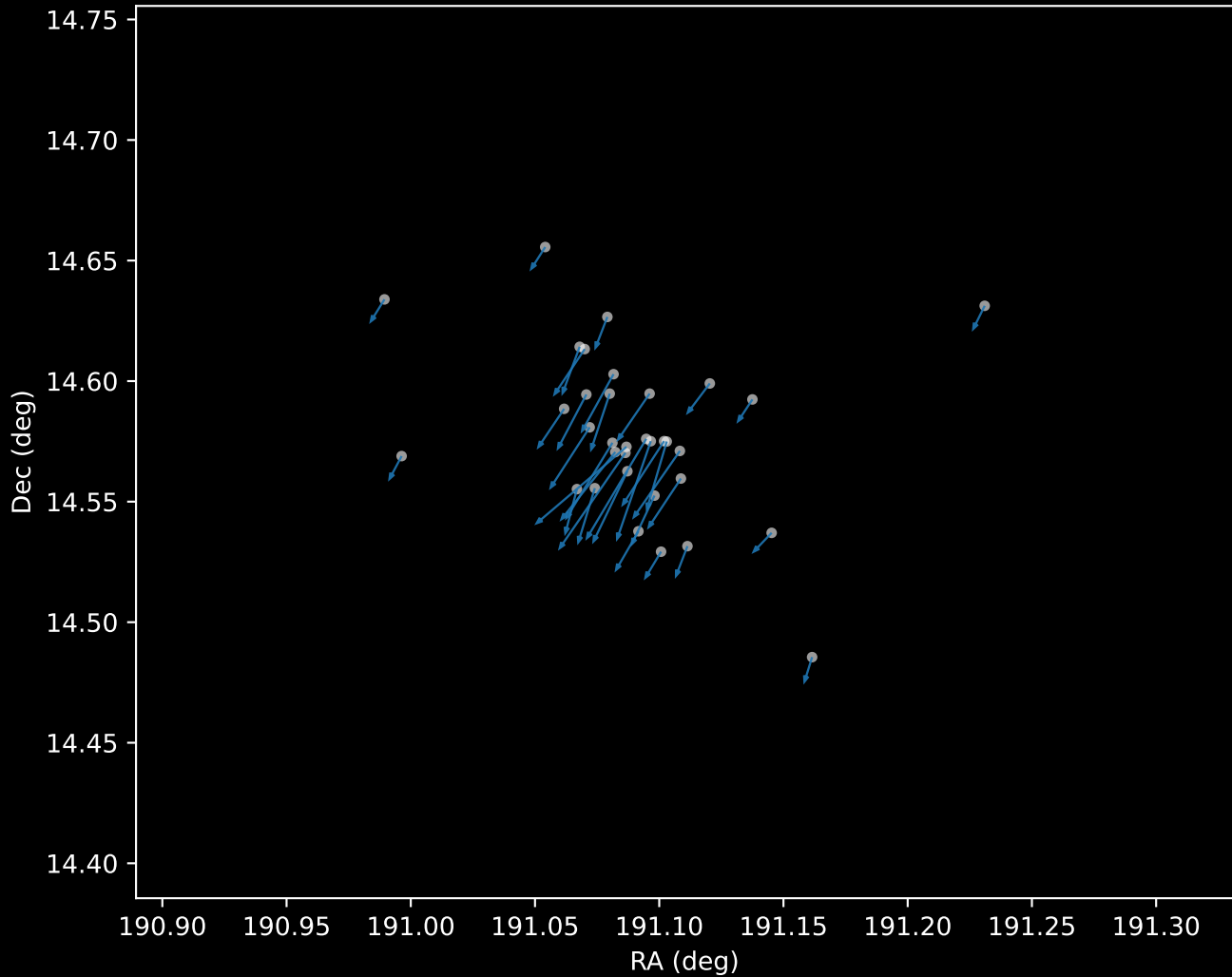
Gaia DR3 Cluster 0 Proper Motion Vectors (n=34)
