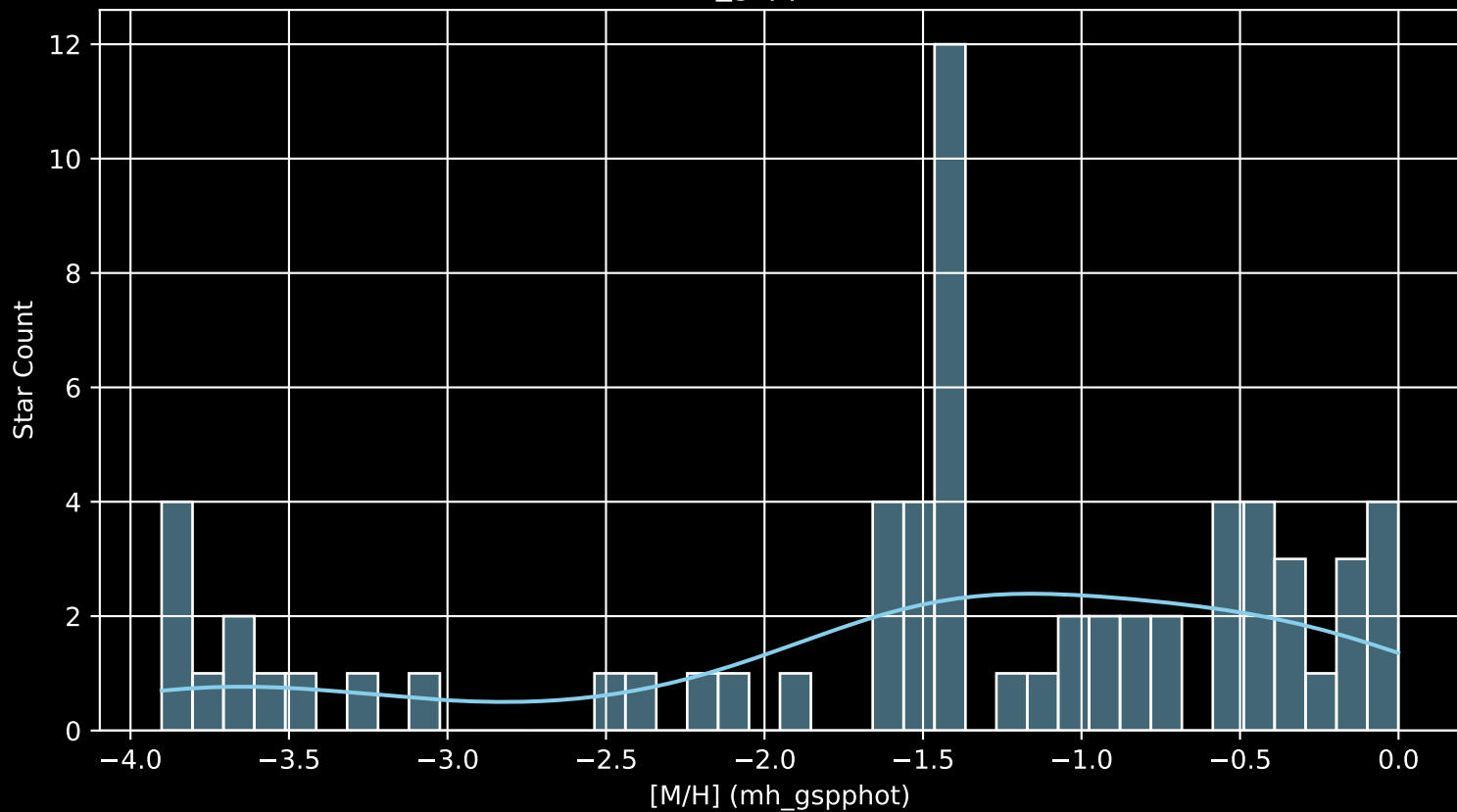
Gaia Cluster: [FSR_0932 [M/H] (mh_gspphot) (n= 65)
