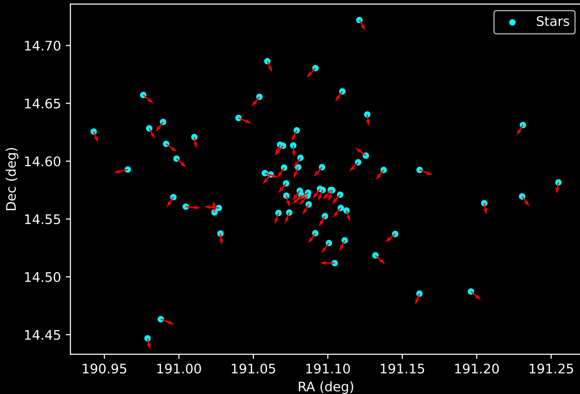
Gaia Cluster: [FSR_0932] Proper Motion Vectors for Gaia Star Field (n= 65)
