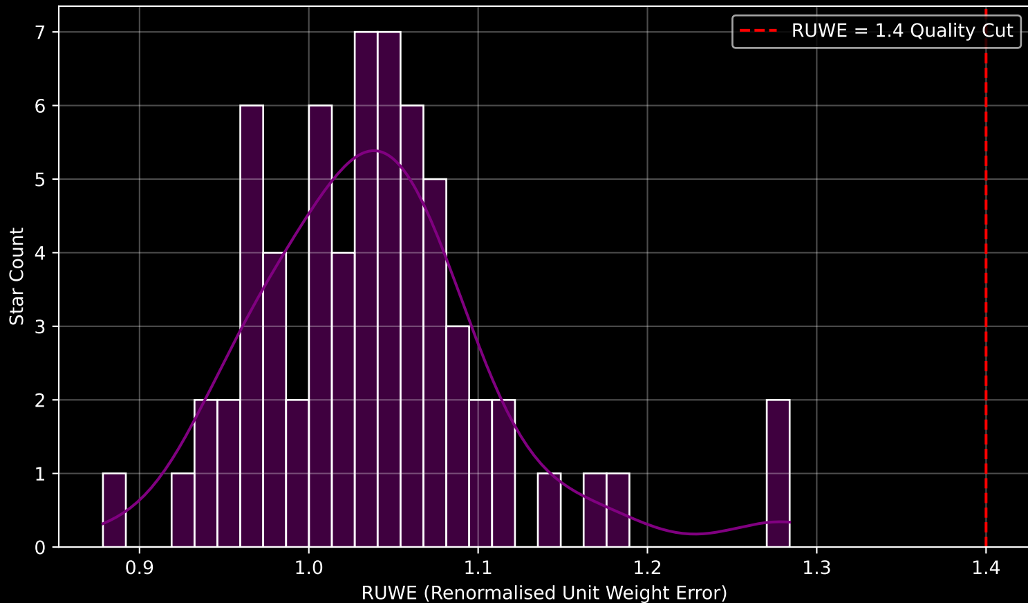
Gaia Cluster: [FSR_0932] RUWE Distribution (n= 65)
