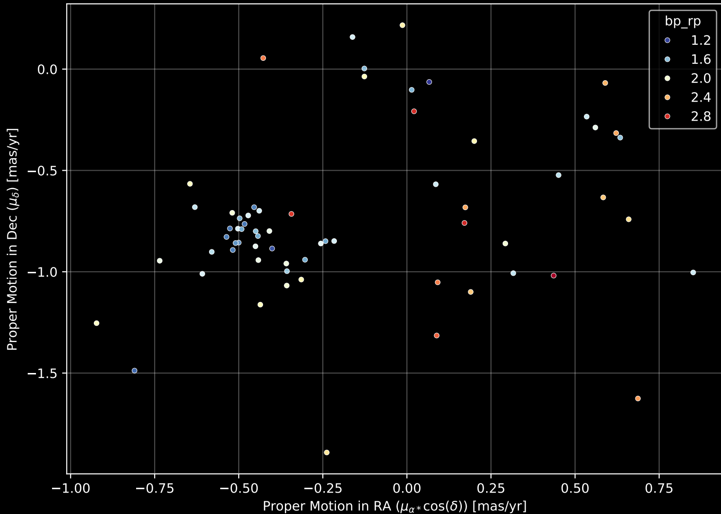
Gaia Cluster: [FSR_0932] Proper Motion Diagram (n= 65)
