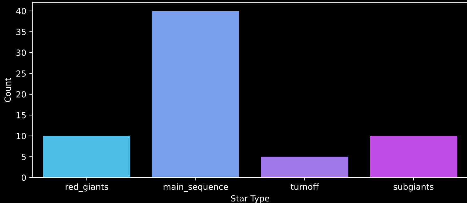
Gaia Cluster: [FSR_0932] Count plot of Star Type
