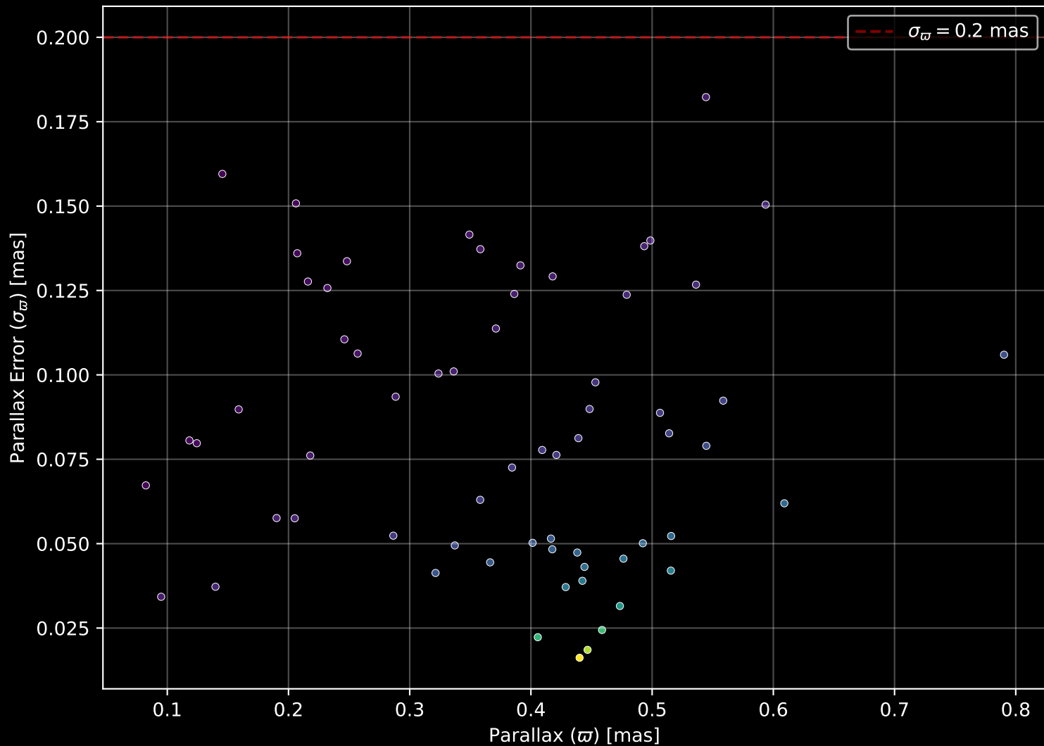
Gaia Cluster: [FSR_0932] Parallax Quality (n= 65)
