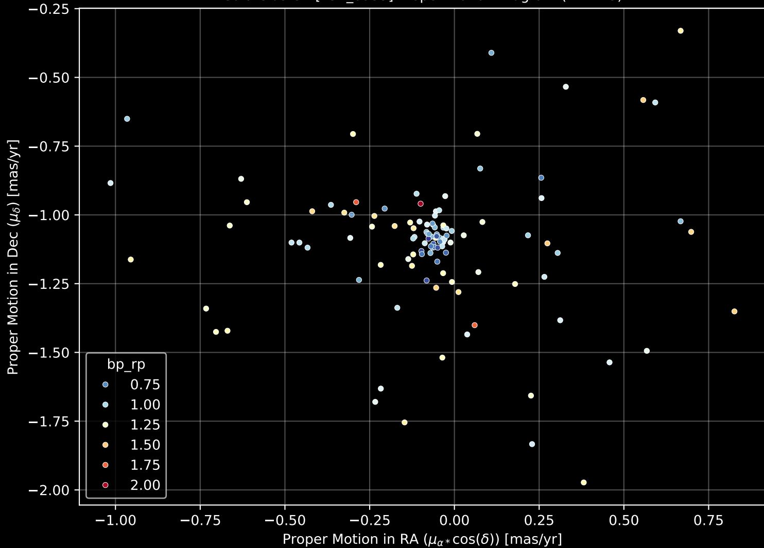
Gaia Cluster: [FSR_0935] Proper Motion Diagram (n= 113)
