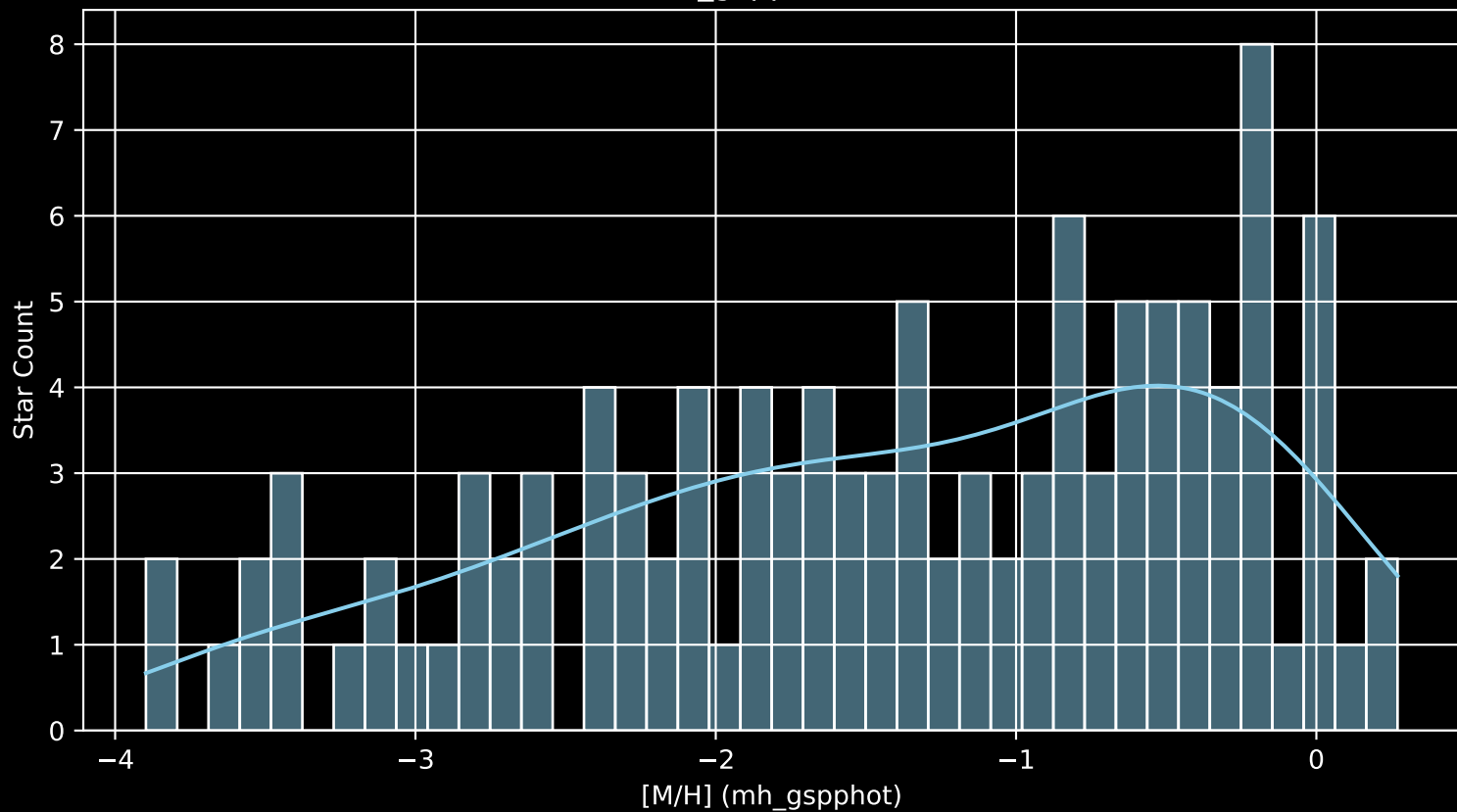
Gaia Cluster: [FSR_0935 [M/H] (mh_gspphot) (n= 113)
