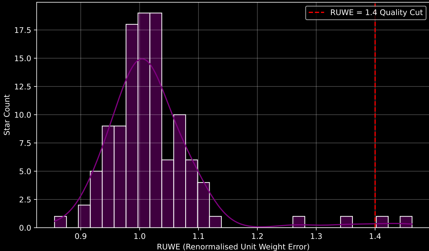
Gaia Cluster: [FSR_0935] RUWE Distribution (n= 113)
