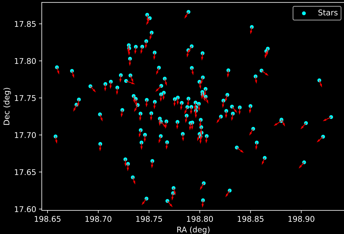
Gaia Cluster: [FSR_0935] Proper Motion Vectors for Gaia Star Field (n= 113)
