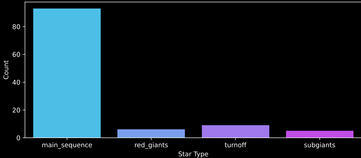
Gaia Cluster: [FSR_0935] Count plot of Star Type
