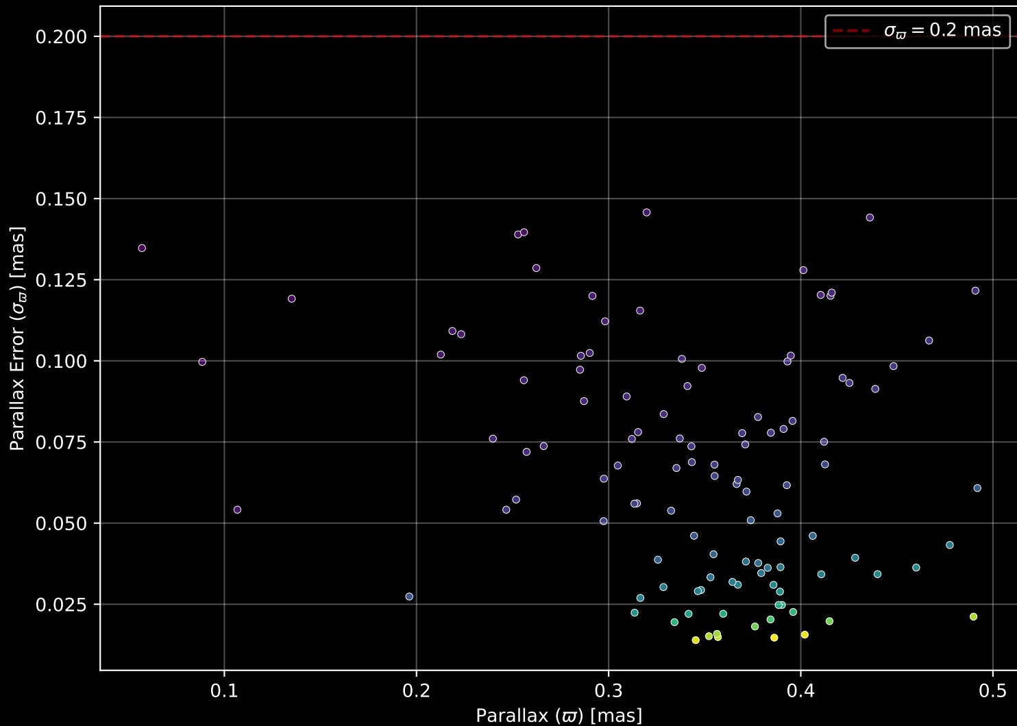
Gaia Cluster: [FSR_0935] Parallax Quality (n= 113)
