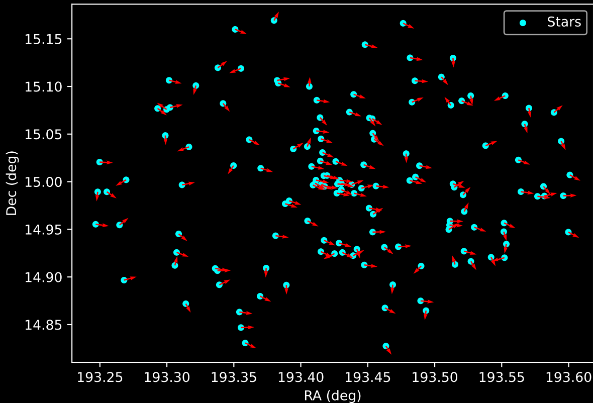
Gaia Cluster: [FSR_0937] Proper Motion Vectors for Gaia Star Field (n= 139)
