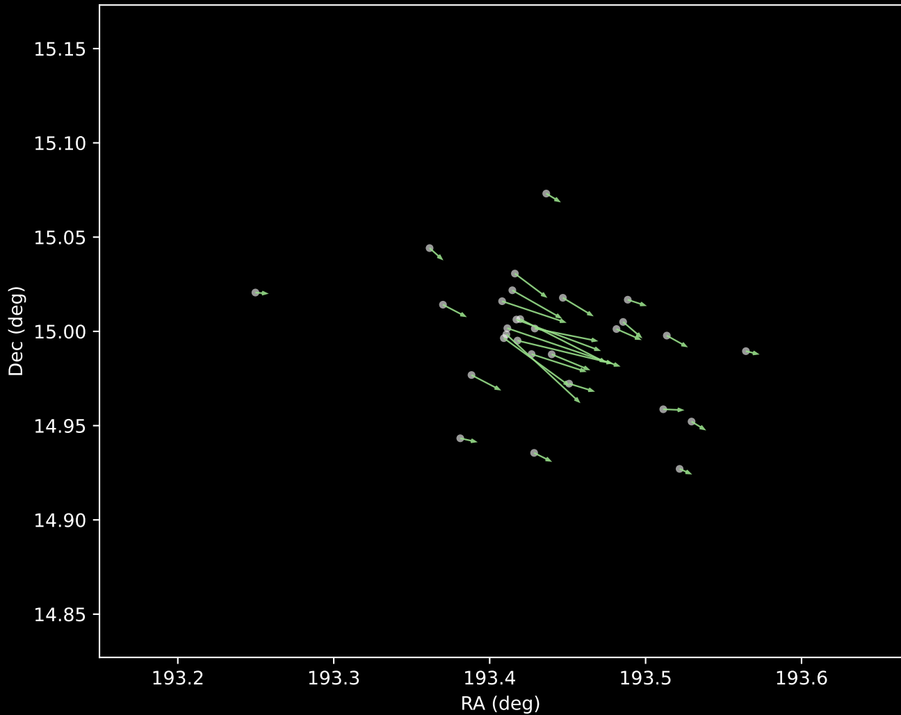
Gaia DR3 Cluster 5 Proper Motion Vectors (n=29)
