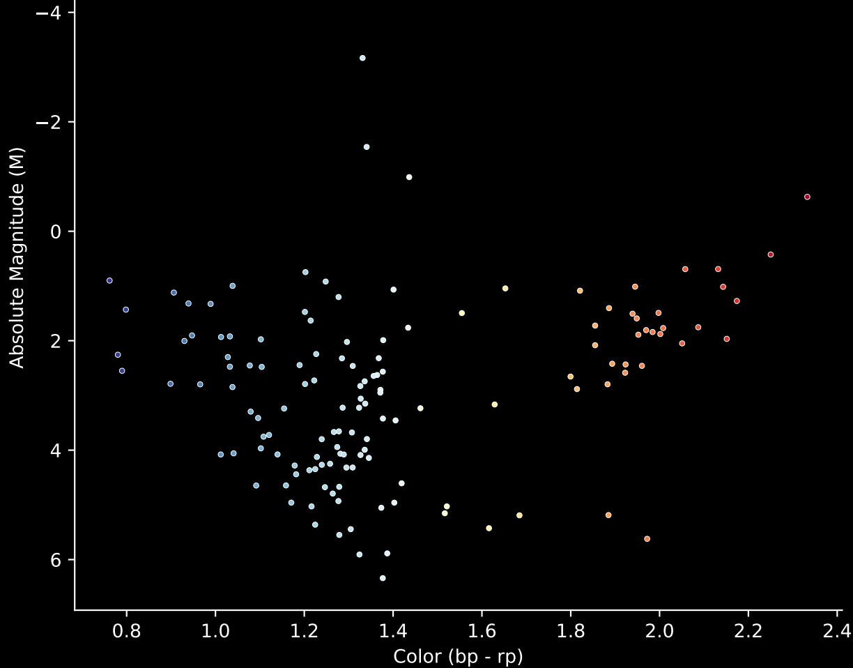
Gaia Cluster: [FSR_0937] Stars (n= 139) Hertzsprung-Russel Diagram
