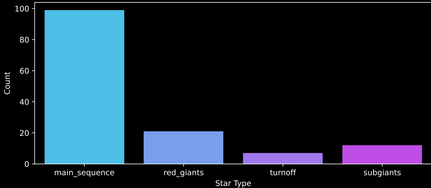
Gaia Cluster: [FSR_0937] Count plot of Star Type
