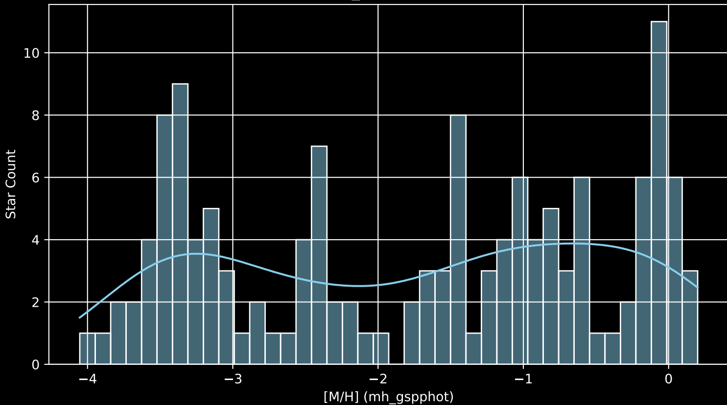
Gaia Cluster: [FSR_0937 [M/H] (mh_gspphot) (n= 139)
