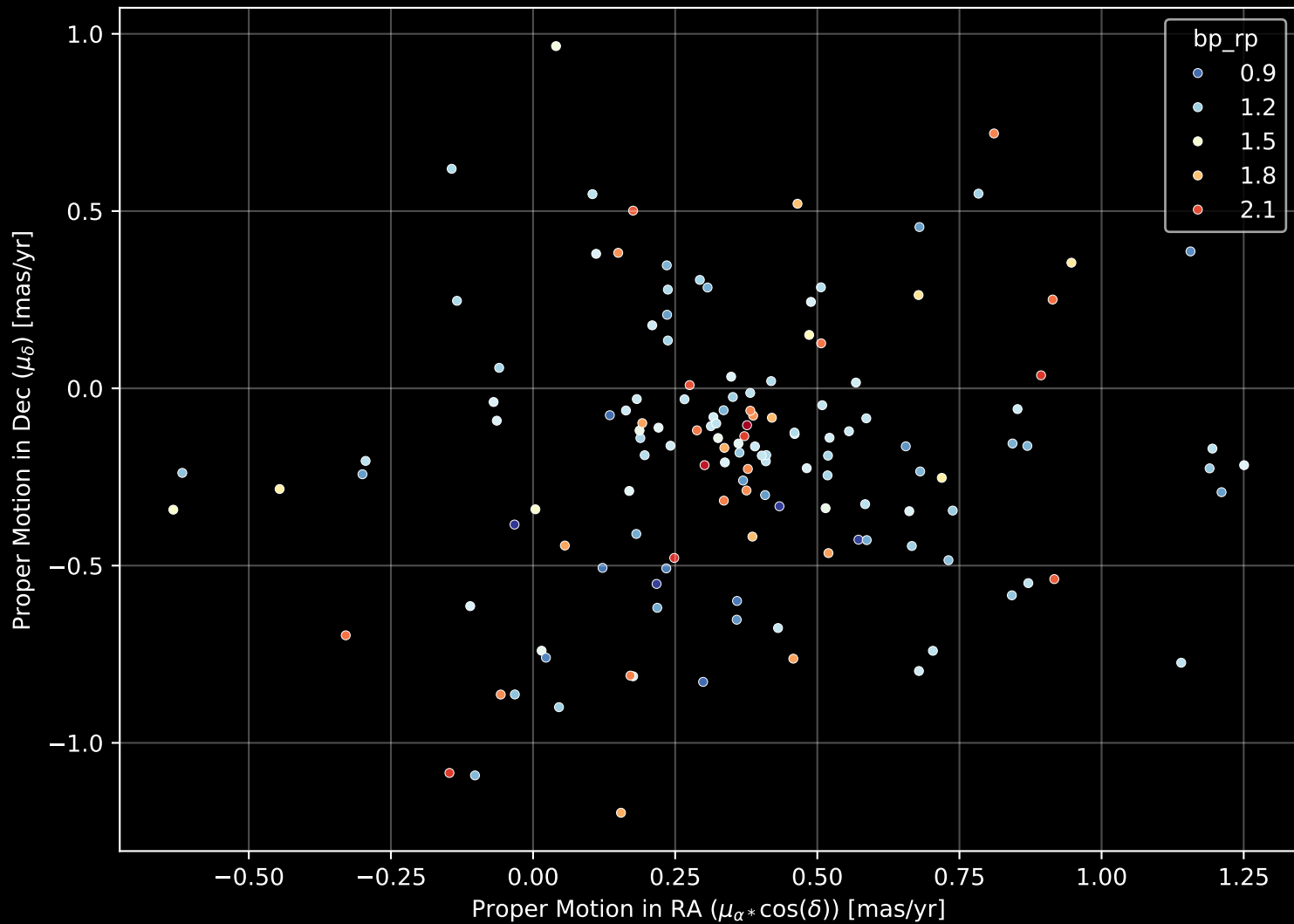
Gaia Cluster: [FSR_0937] Proper Motion Diagram (n= 139)
