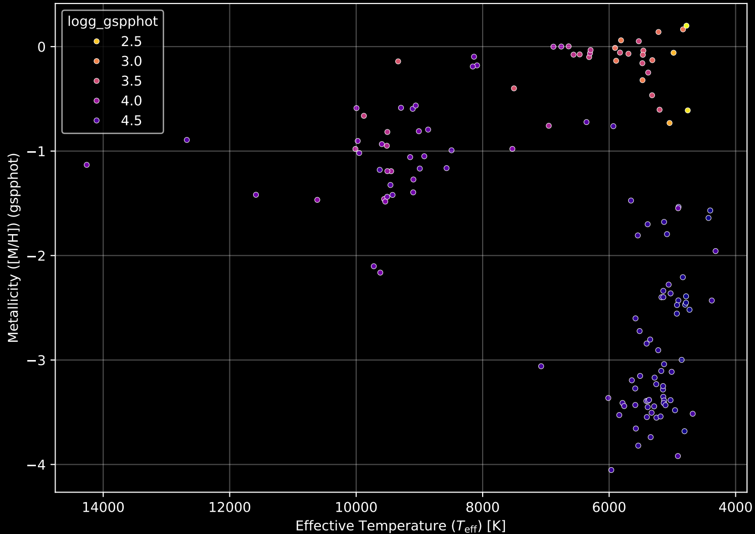
Gaia Cluster: [FSR_0937] Stellar Population Parameters (n= 139)
