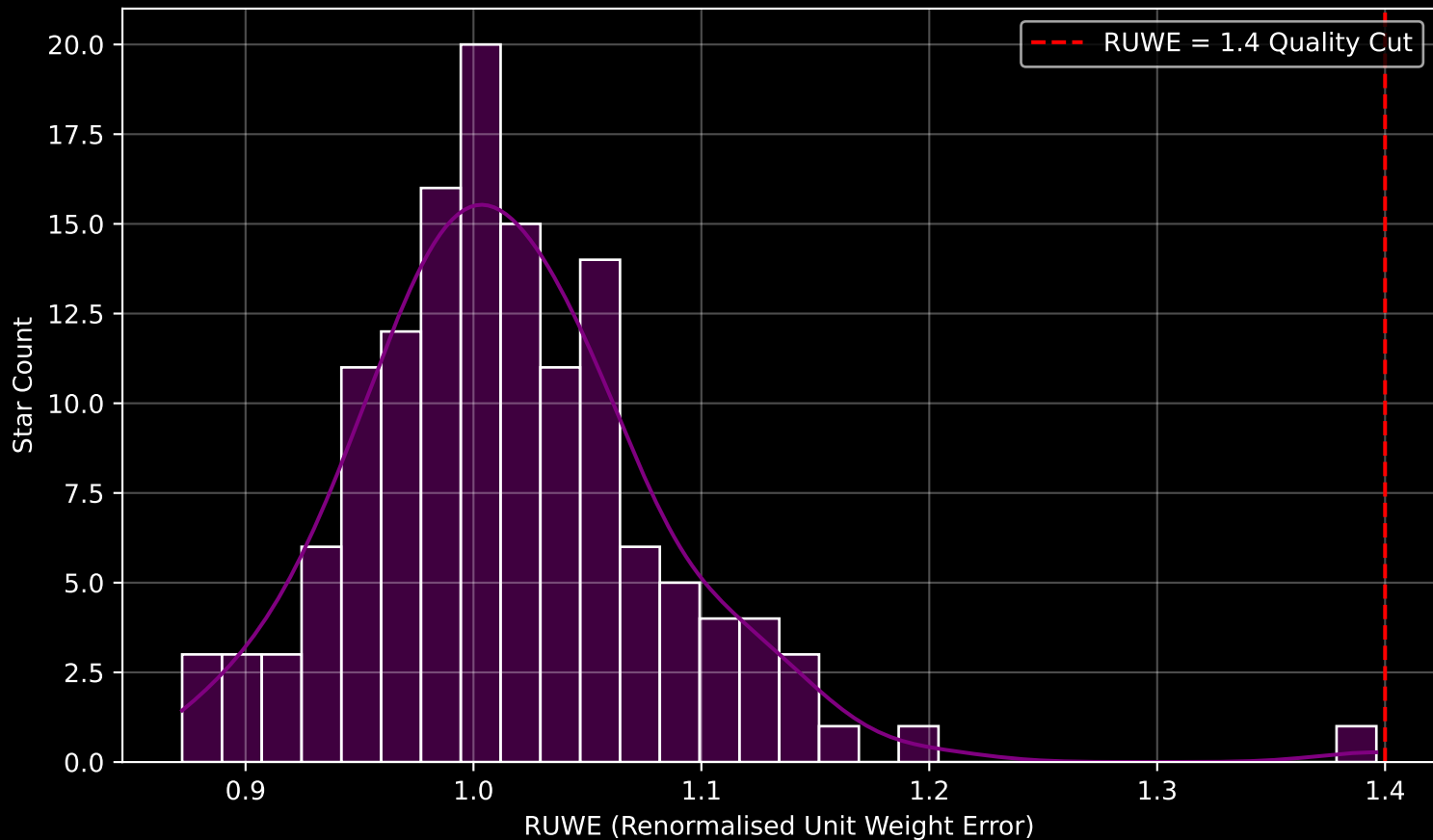
Gaia Cluster: [FSR_0937] RUWE Distribution (n= 139)
