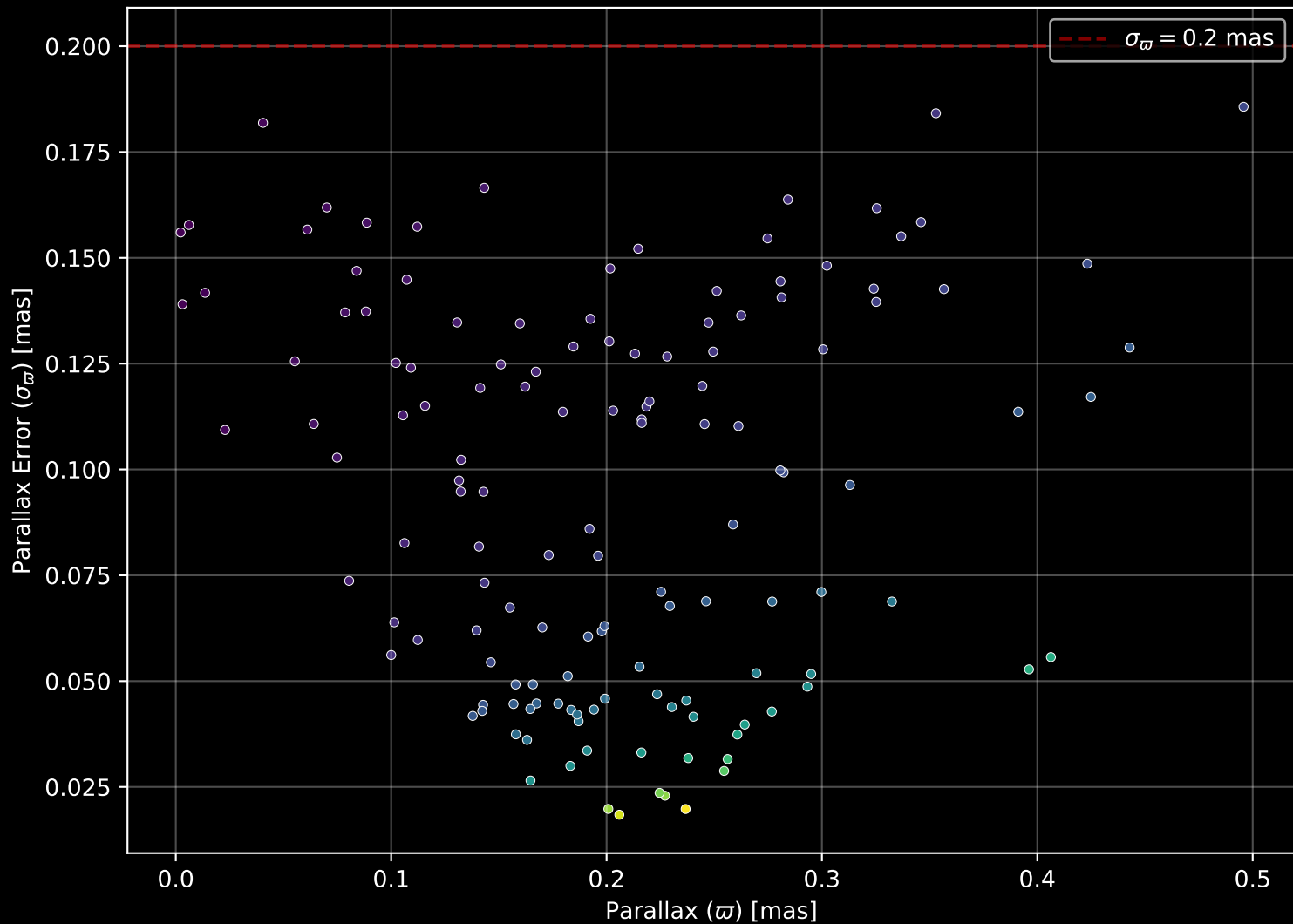
Gaia Cluster: [FSR_0937] Parallax Quality (n= 139)
