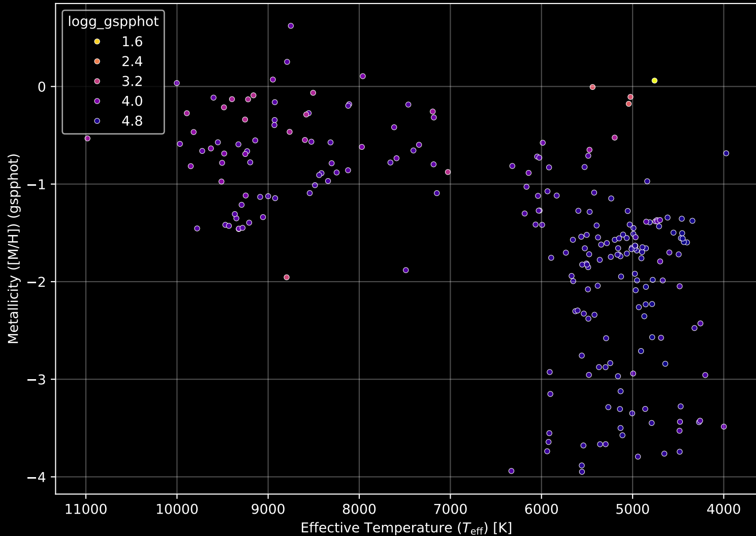
Gaia Cluster: [FSR_0953] Stellar Population Parameters (n= 229)
