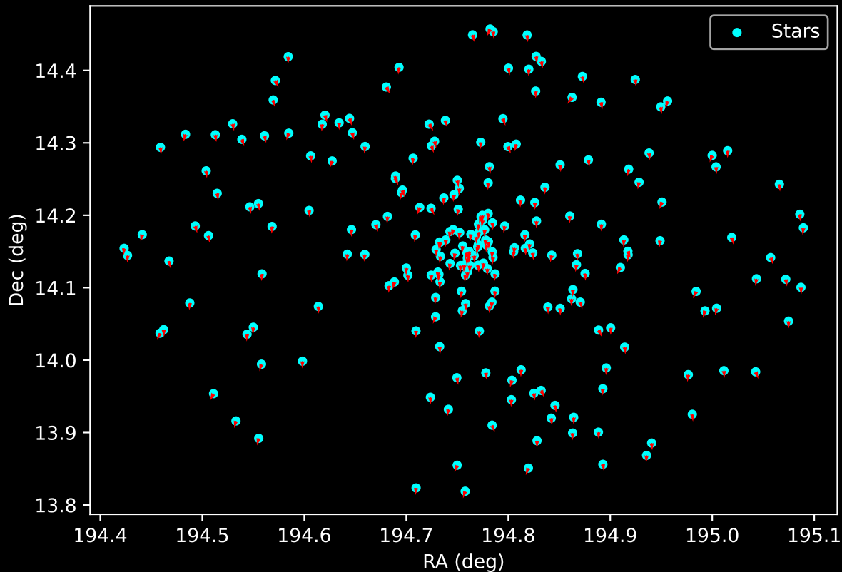
Gaia Cluster: [FSR_0953] Proper Motion Vectors for Gaia Star Field (n= 229)
