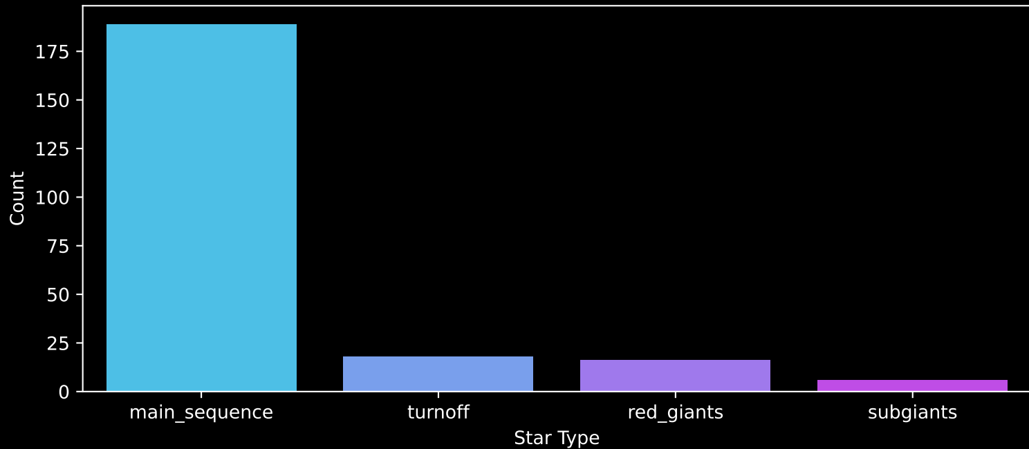
Gaia Cluster: [FSR_0953] Count plot of Star Type
