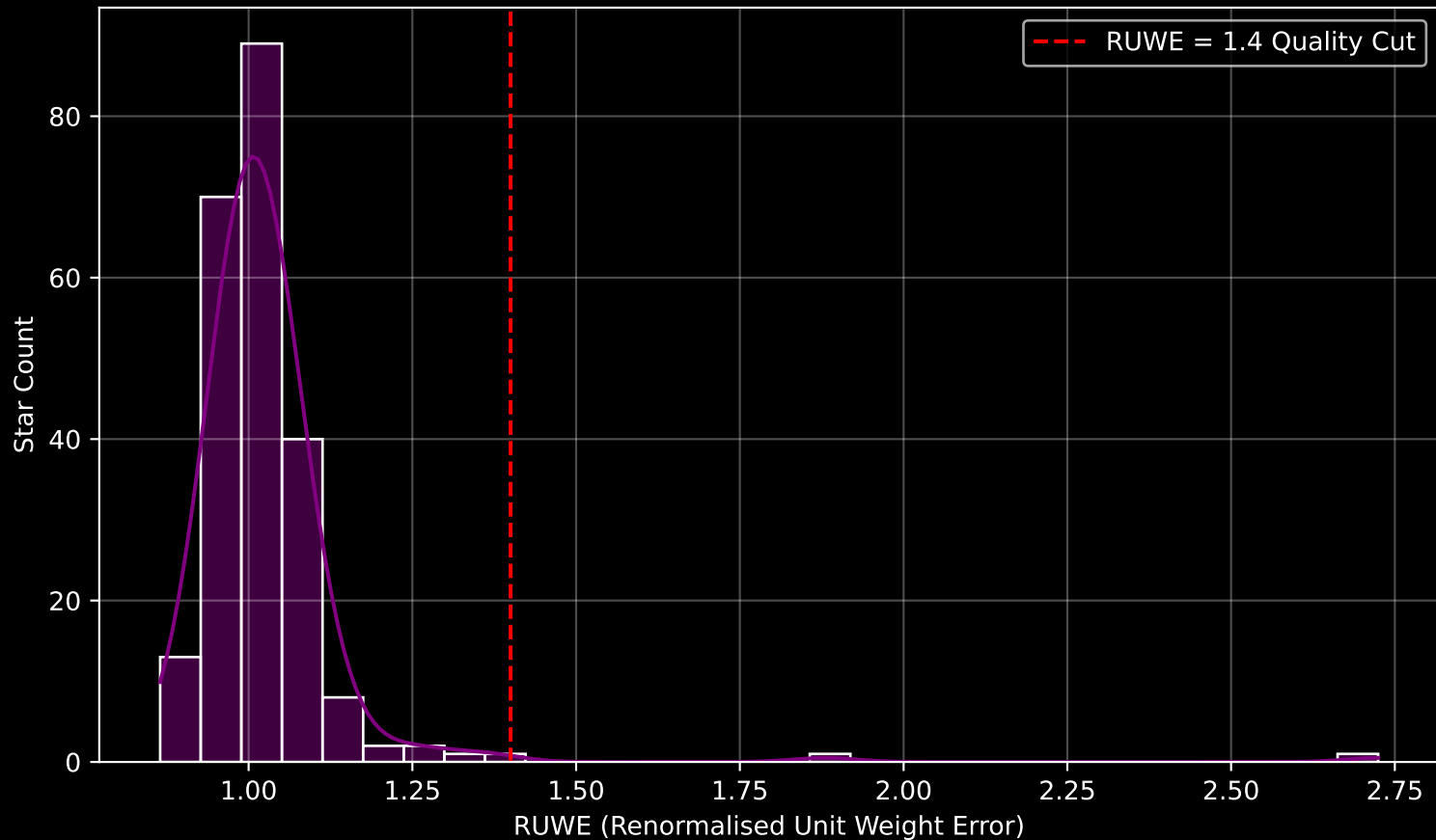
Gaia Cluster: [FSR_0953] RUWE Distribution (n= 228)
