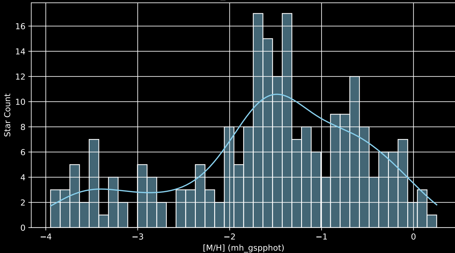
Gaia Cluster: [FSR_0953 [M/H] (mh_gspphot) (n= 228)
