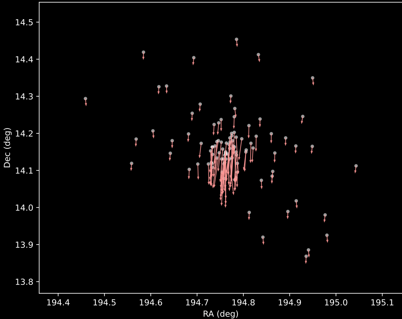
Gaia DR3 Cluster 7 Proper Motion Vectors (n=99)
