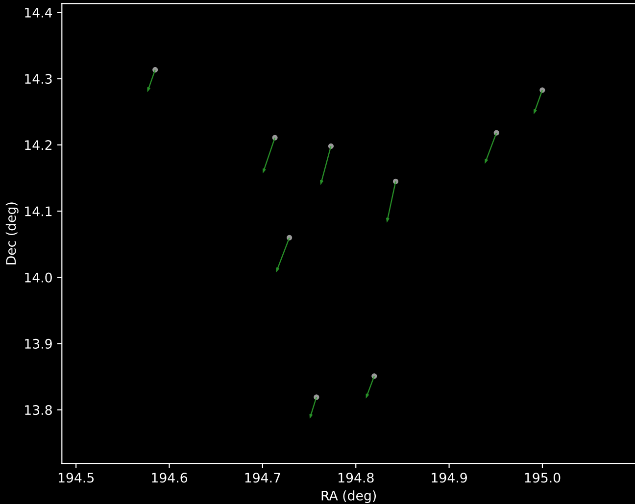
Gaia DR3 Cluster 4 Proper Motion Vectors (n=9)
