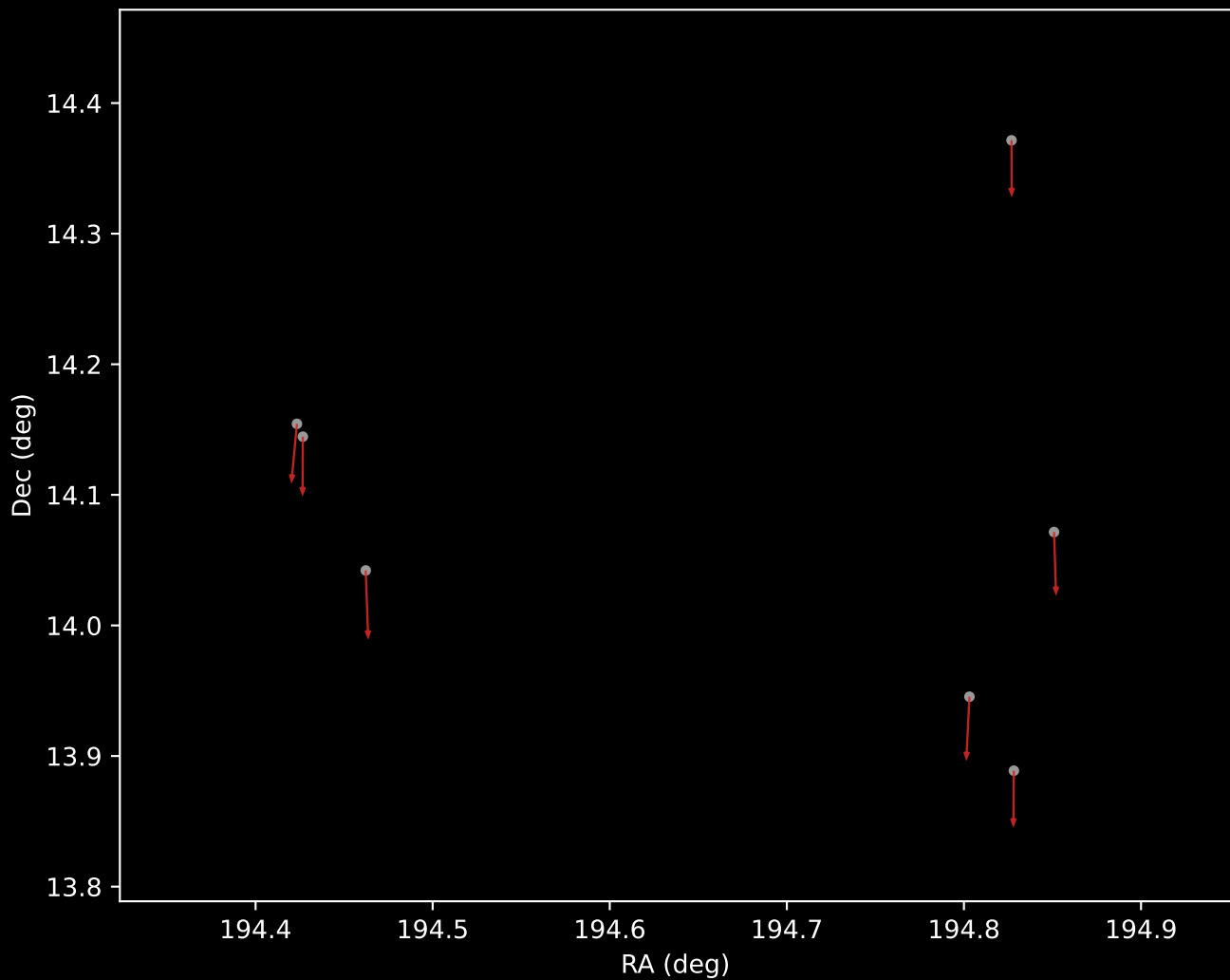
Gaia DR3 Cluster 6 Proper Motion Vectors (n=7)
