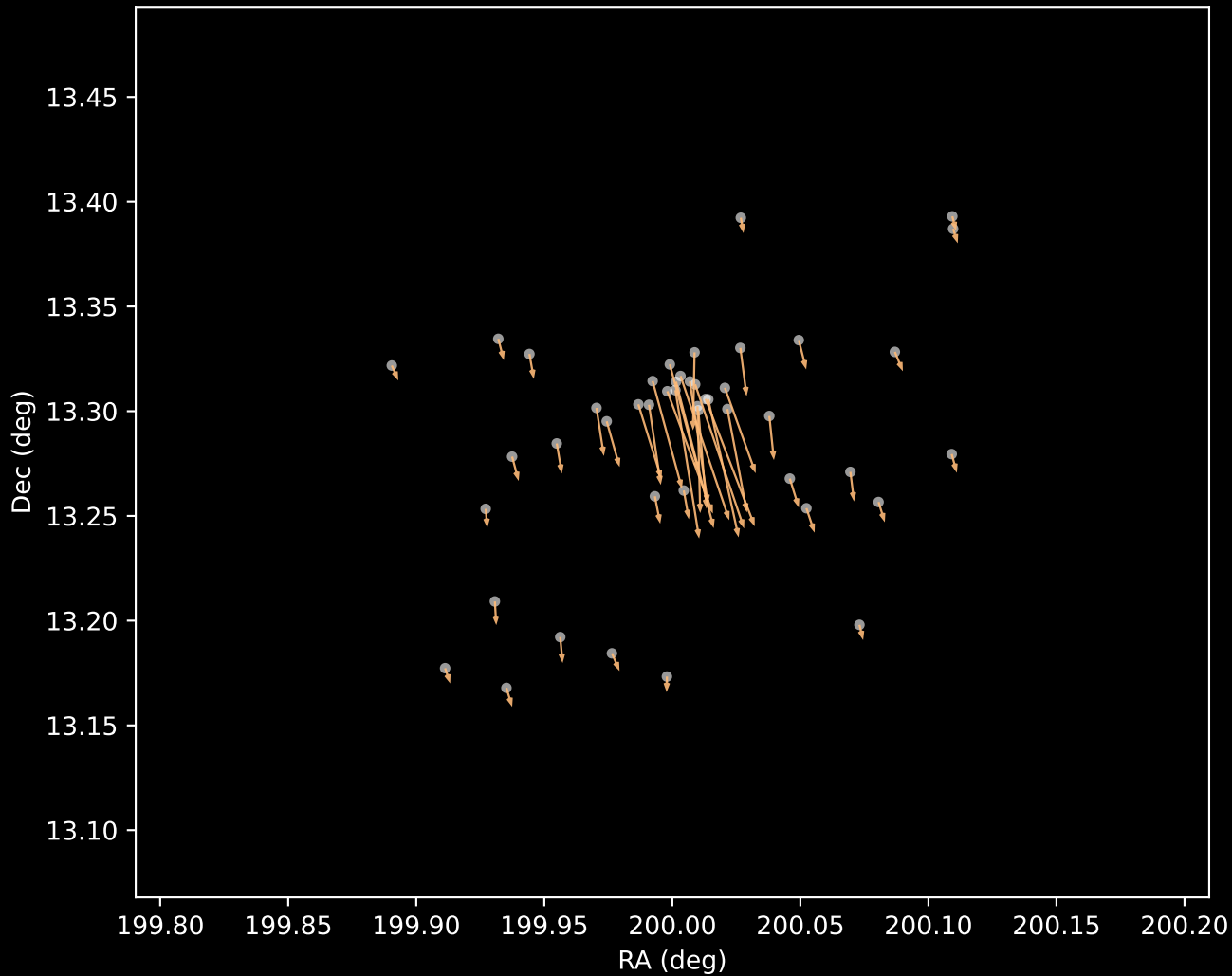
Gaia DR3 Cluster 3 Proper Motion Vectors (n=46)
