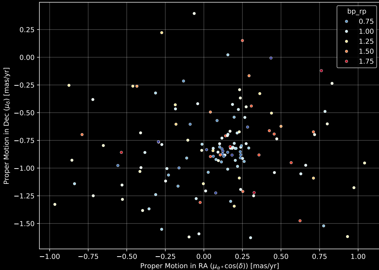
Gaia Cluster: [FSR_0975] Proper Motion Diagram (n= 142)
