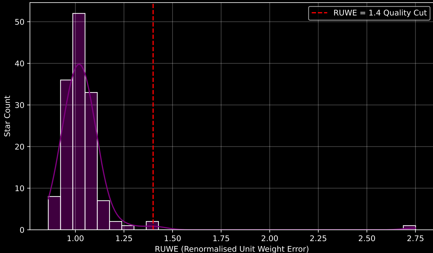
Gaia Cluster: [FSR_0975] RUWE Distribution (n= 142)
