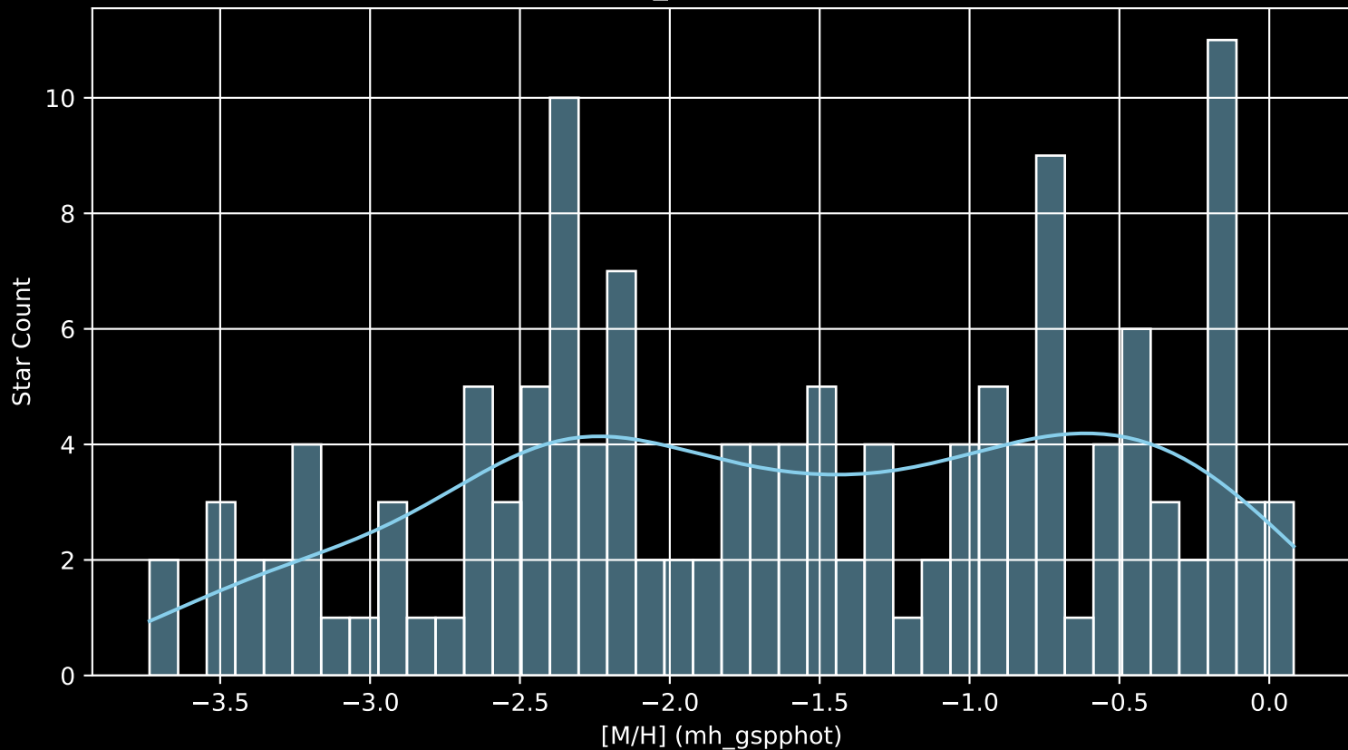
Gaia Cluster: [FSR_0975 [M/H] (mh_gspphot) (n= 141)
