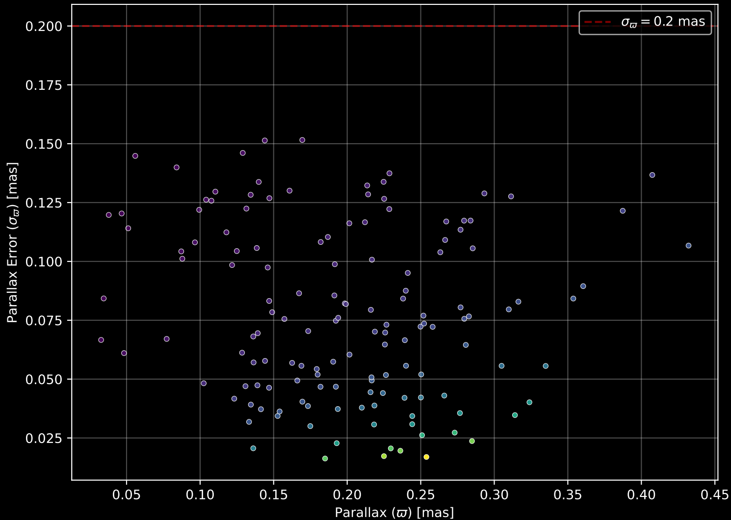
Gaia Cluster: [FSR_0975] Parallax Quality (n= 142)
