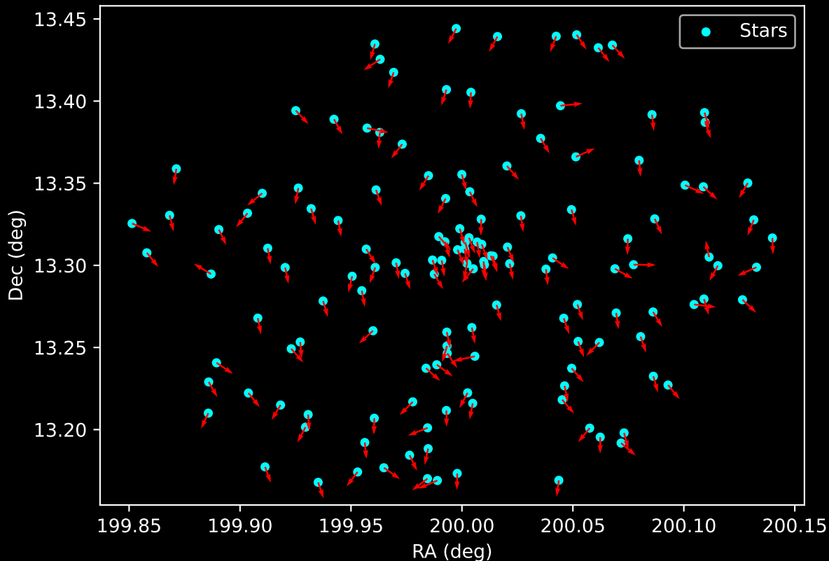
Gaia Cluster: [FSR_0975] Proper Motion Vectors for Gaia Star Field (n= 142)
