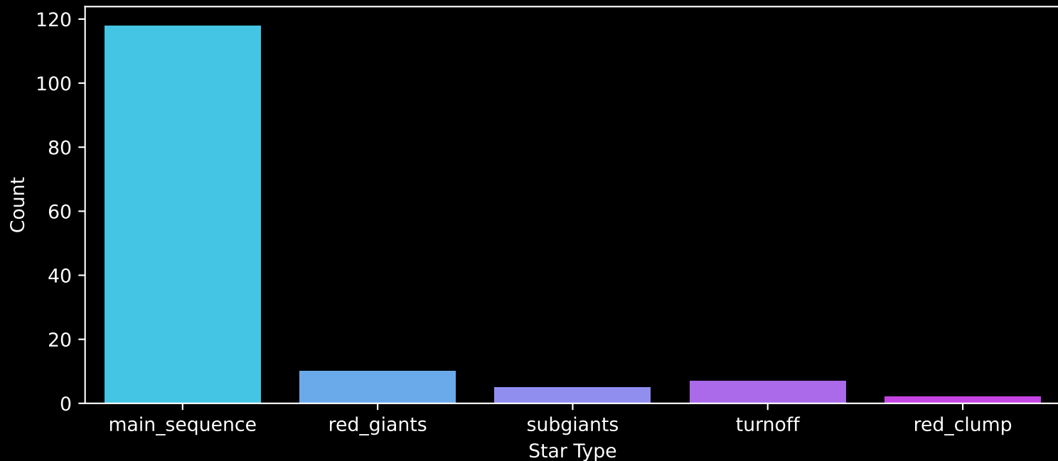
Gaia Cluster: [FSR_0975] Count plot of Star Type
