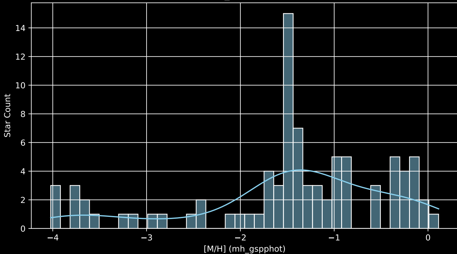
Gaia Cluster: [FSR_0979 [M/H] (mh_gspphot) (n= 87)
