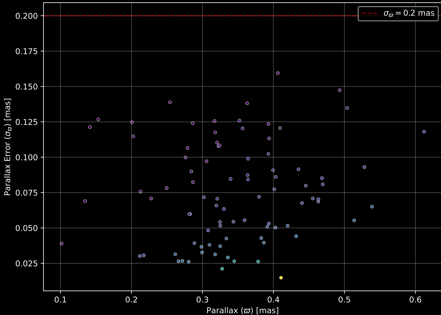
Gaia Cluster: [FSR_0979] Parallax Quality (n= 87)
