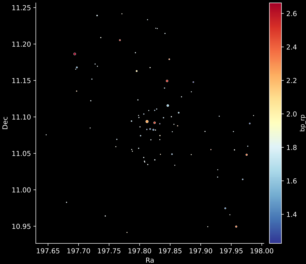
Gaia Cluster: [FSR_0979] Stars: 87
