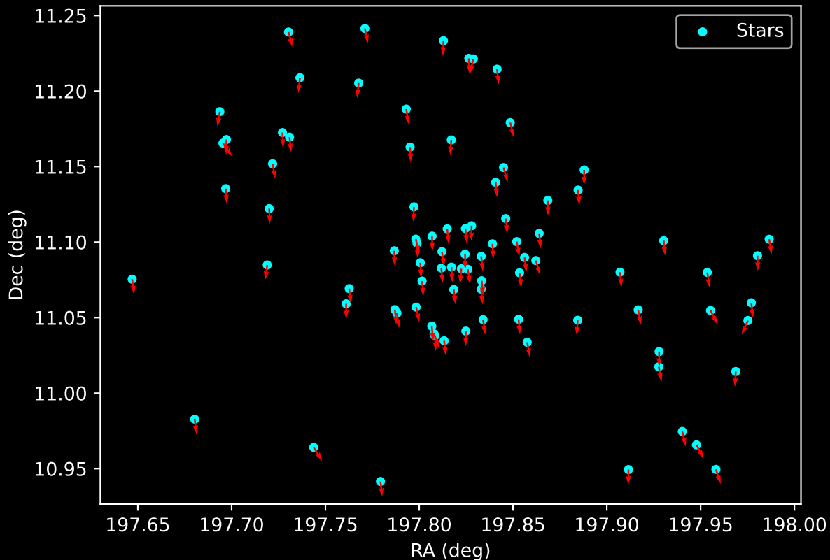
Gaia Cluster: [FSR_0979] Proper Motion Vectors for Gaia Star Field (n= 87)
