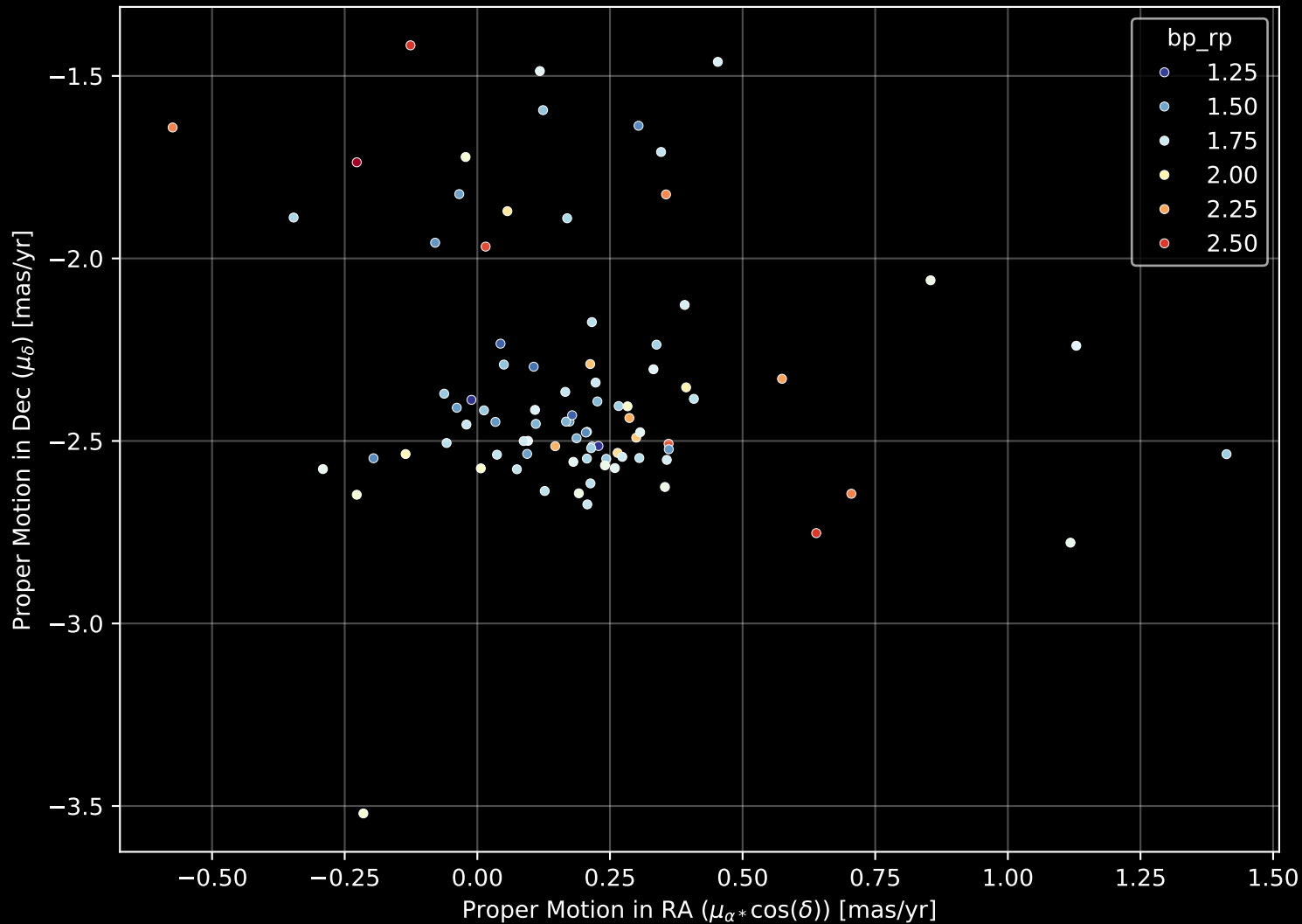
Gaia Cluster: [FSR_0979] Proper Motion Diagram (n= 87)
