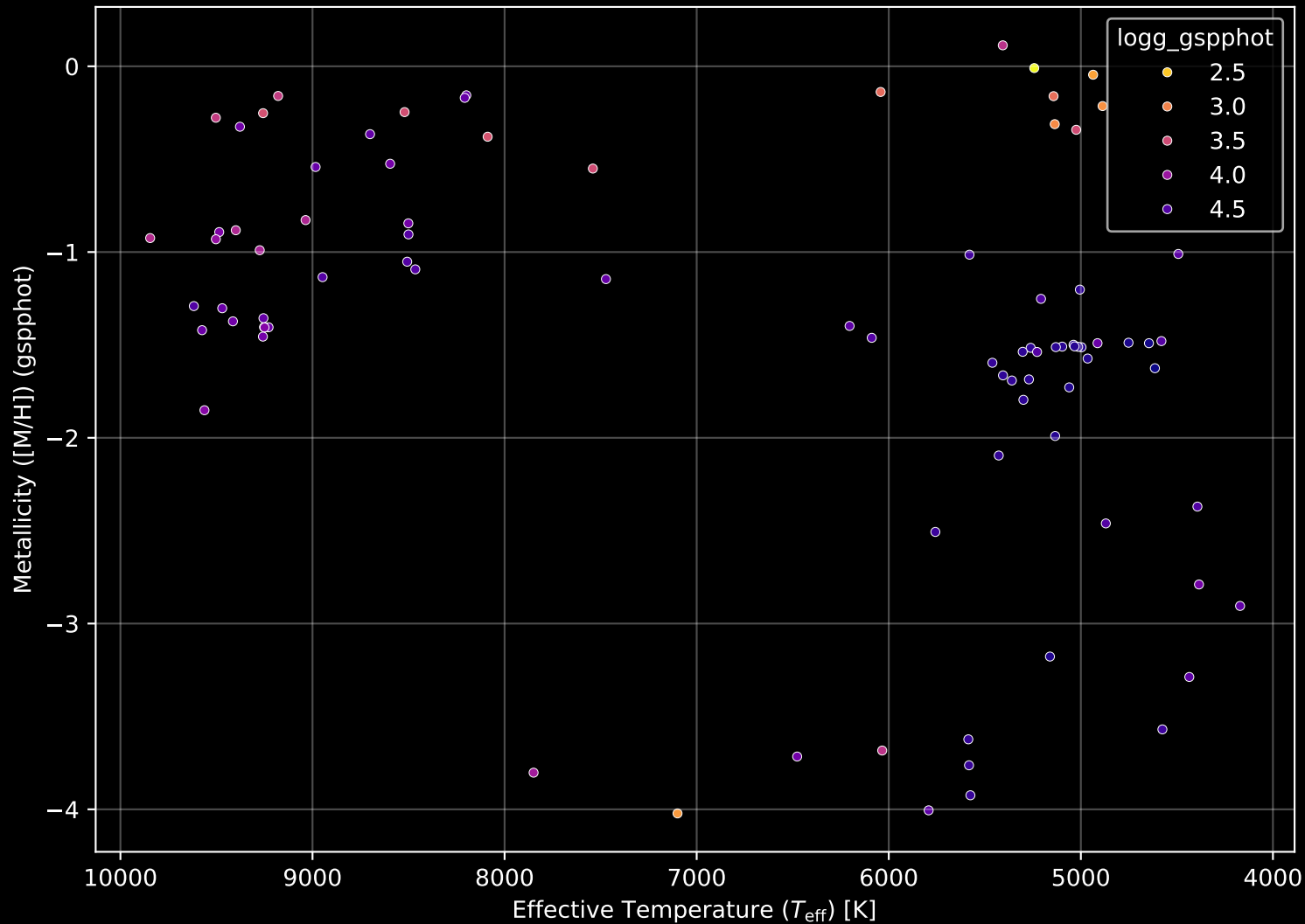
Gaia Cluster: [FSR_0979] Stellar Population Parameters (n= 87)
