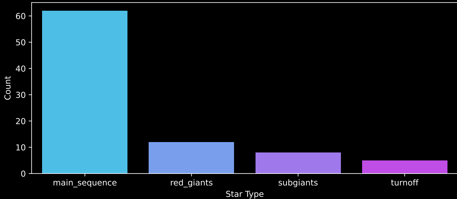
Gaia Cluster: [FSR_0979] Count plot of Star Type
