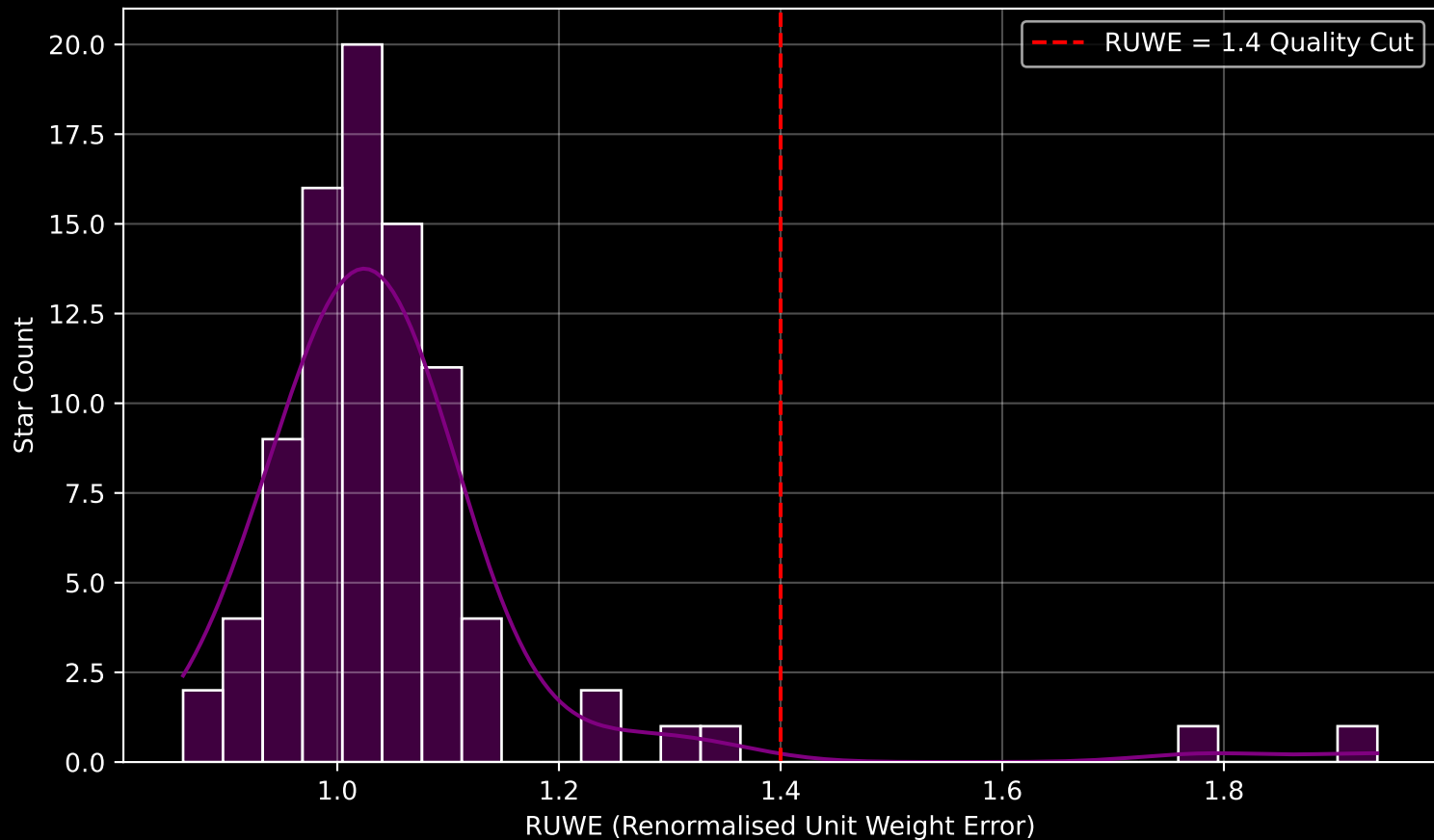
Gaia Cluster: [FSR_0979] RUWE Distribution (n= 87)
