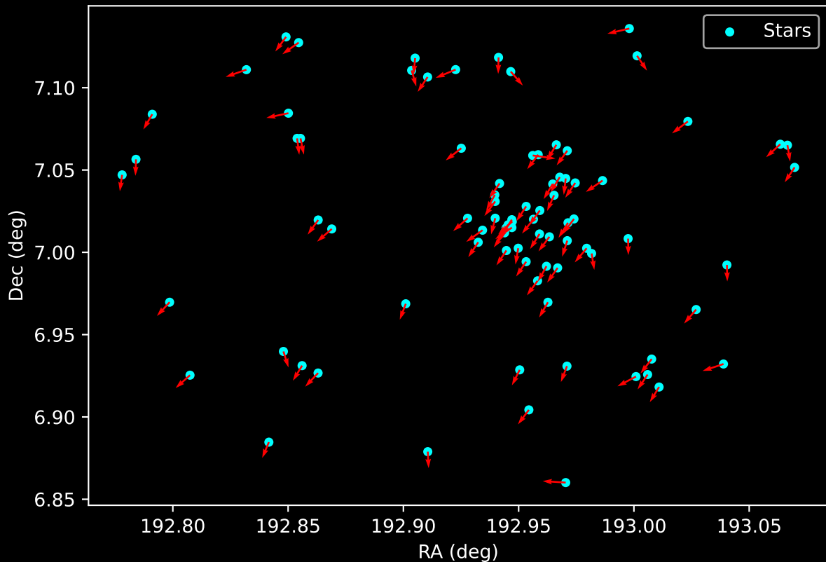
Gaia Cluster: [FSR_0985] Proper Motion Vectors for Gaia Star Field (n= 84)
