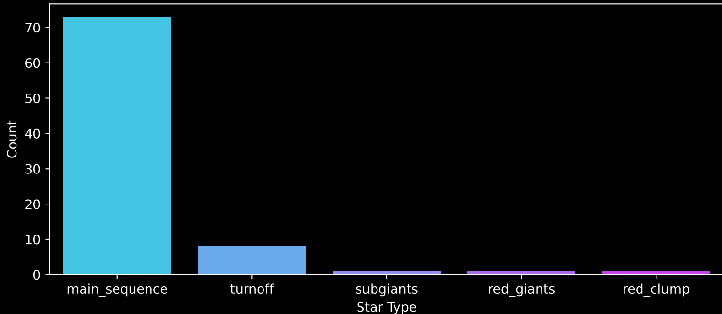
Gaia Cluster: [FSR_0985] Count plot of Star Type
