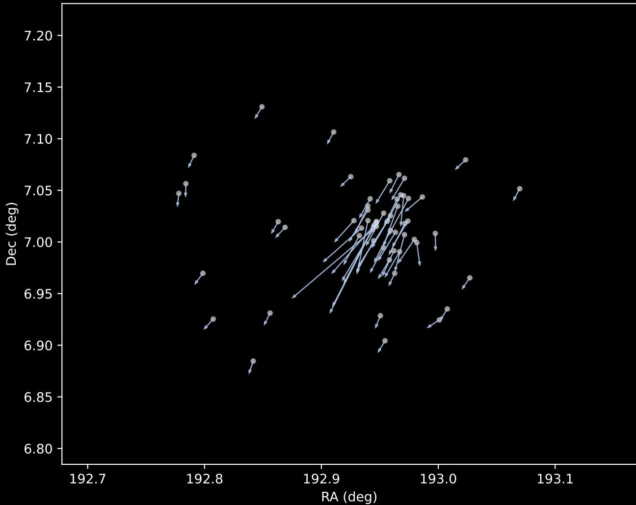
Gaia DR3 Cluster 1 Proper Motion Vectors (n=58)
