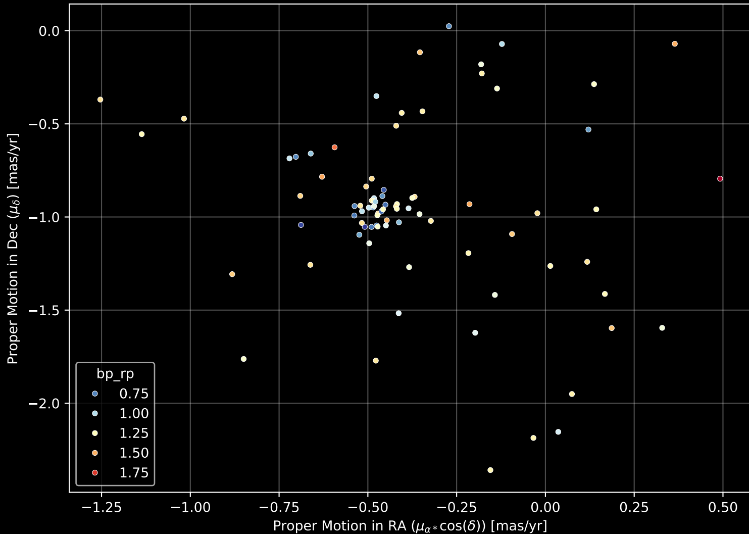
Gaia Cluster: [FSR_0985] Proper Motion Diagram (n= 84)
