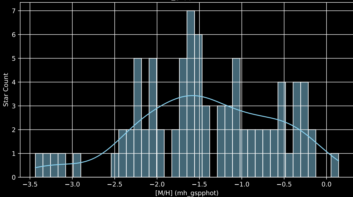
Gaia Cluster: [FSR_0985 [M/H] (mh_gspphot) (n= 84)
