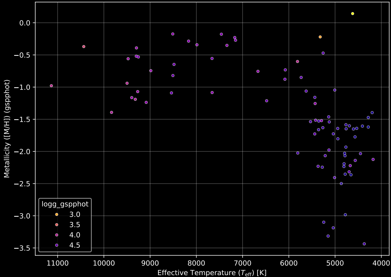
Gaia Cluster: [FSR_0985] Stellar Population Parameters (n= 84)
