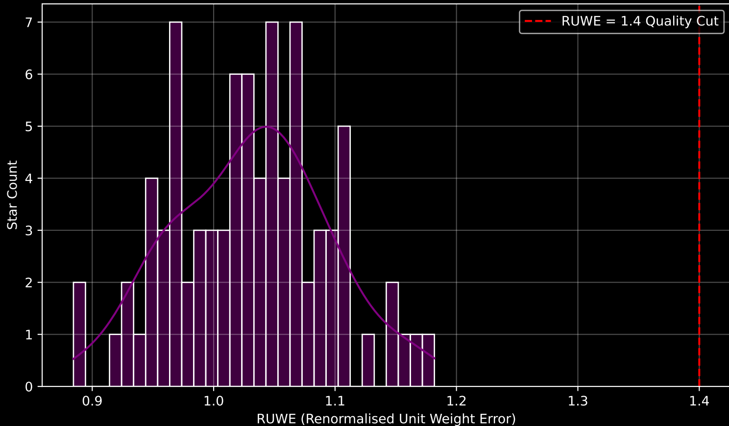
Gaia Cluster: [FSR_0985] RUWE Distribution (n= 84)
