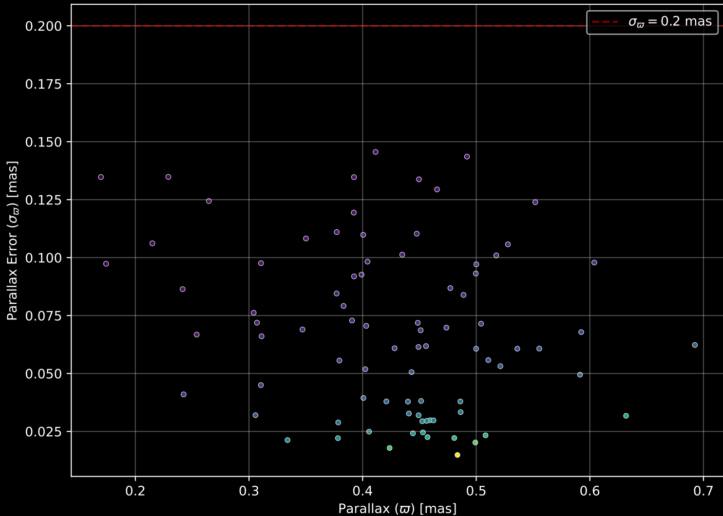
Gaia Cluster: [FSR_0985] Parallax Quality (n= 84)
