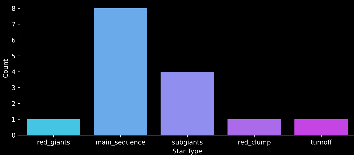
Gaia Cluster: [FSR_1032] Count plot of Star Type
