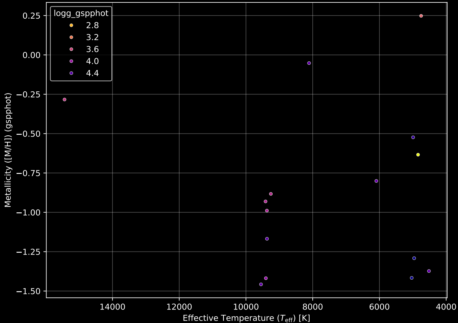
Gaia Cluster: [FSR_1032] Stellar Population Parameters (n= 15)
