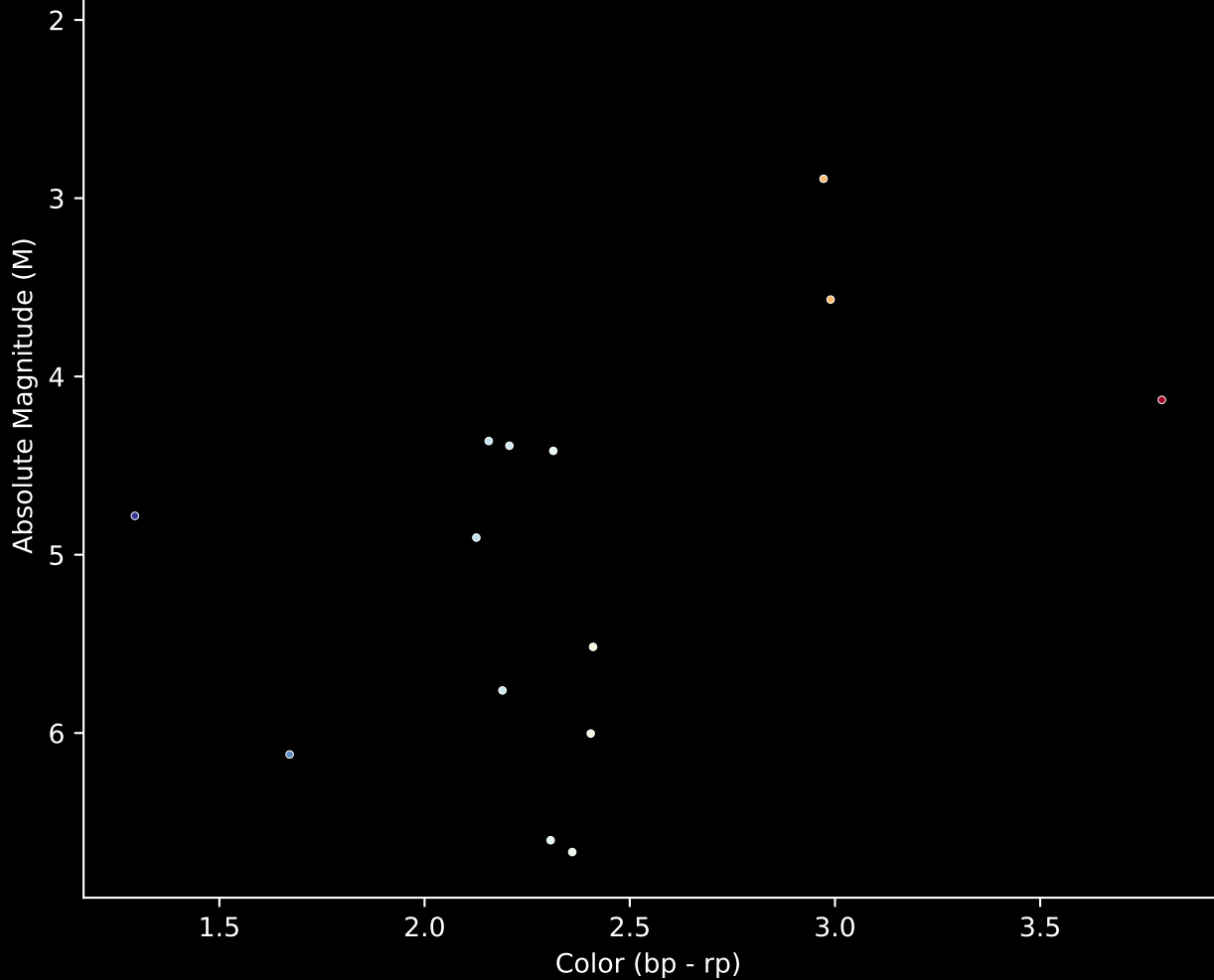
Gaia Cluster: [FSR_1032] Stars (n= 15) Hertzsprung-Russel Diagram
