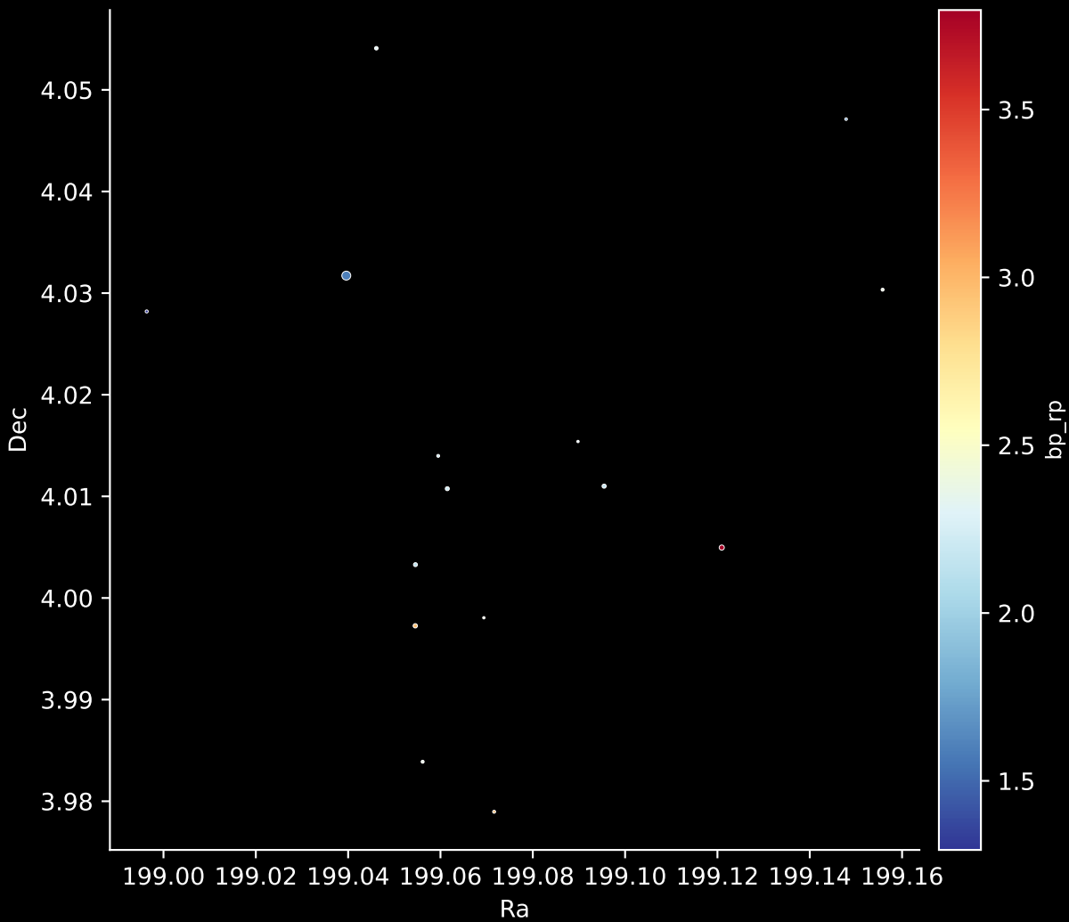
Gaia Cluster: [FSR_1032] Stars: 15
