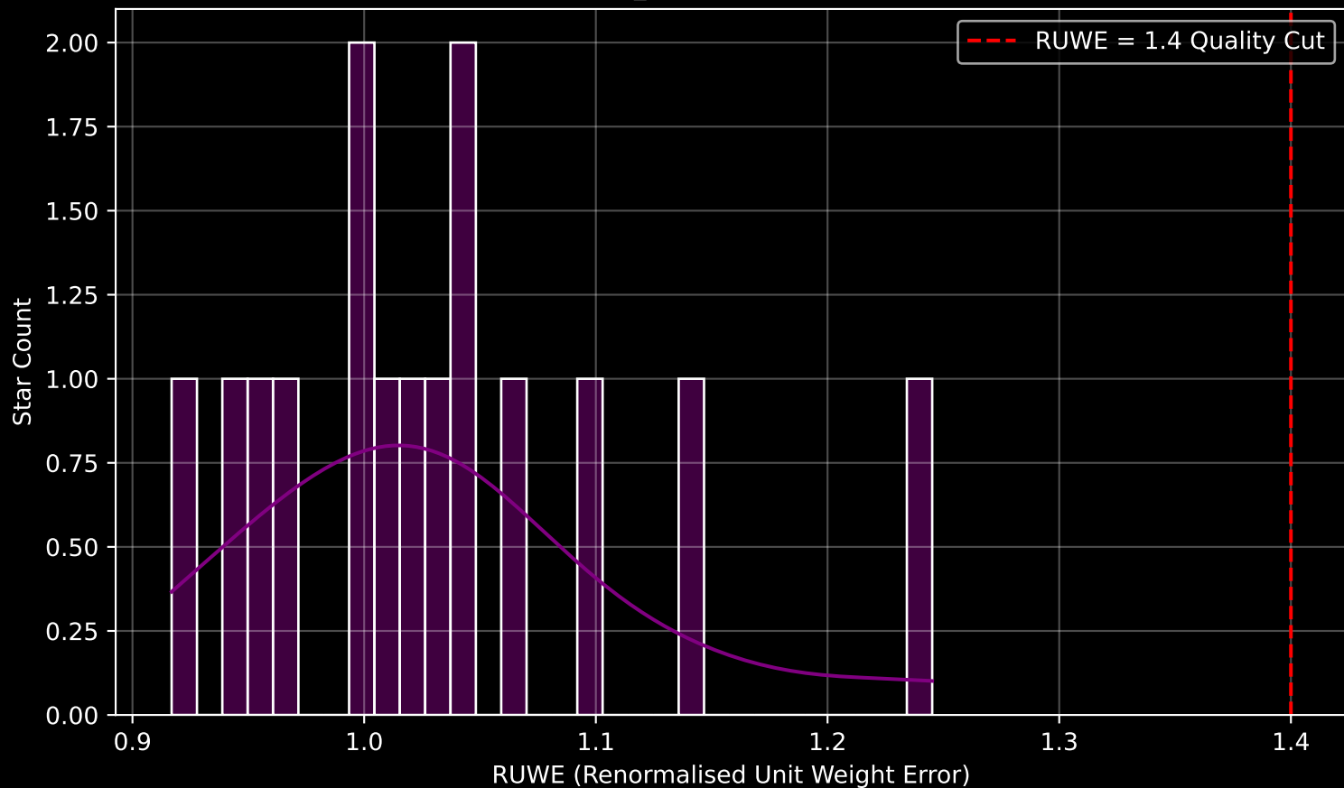
Gaia Cluster: [FSR_1032] RUWE Distribution (n= 15)
