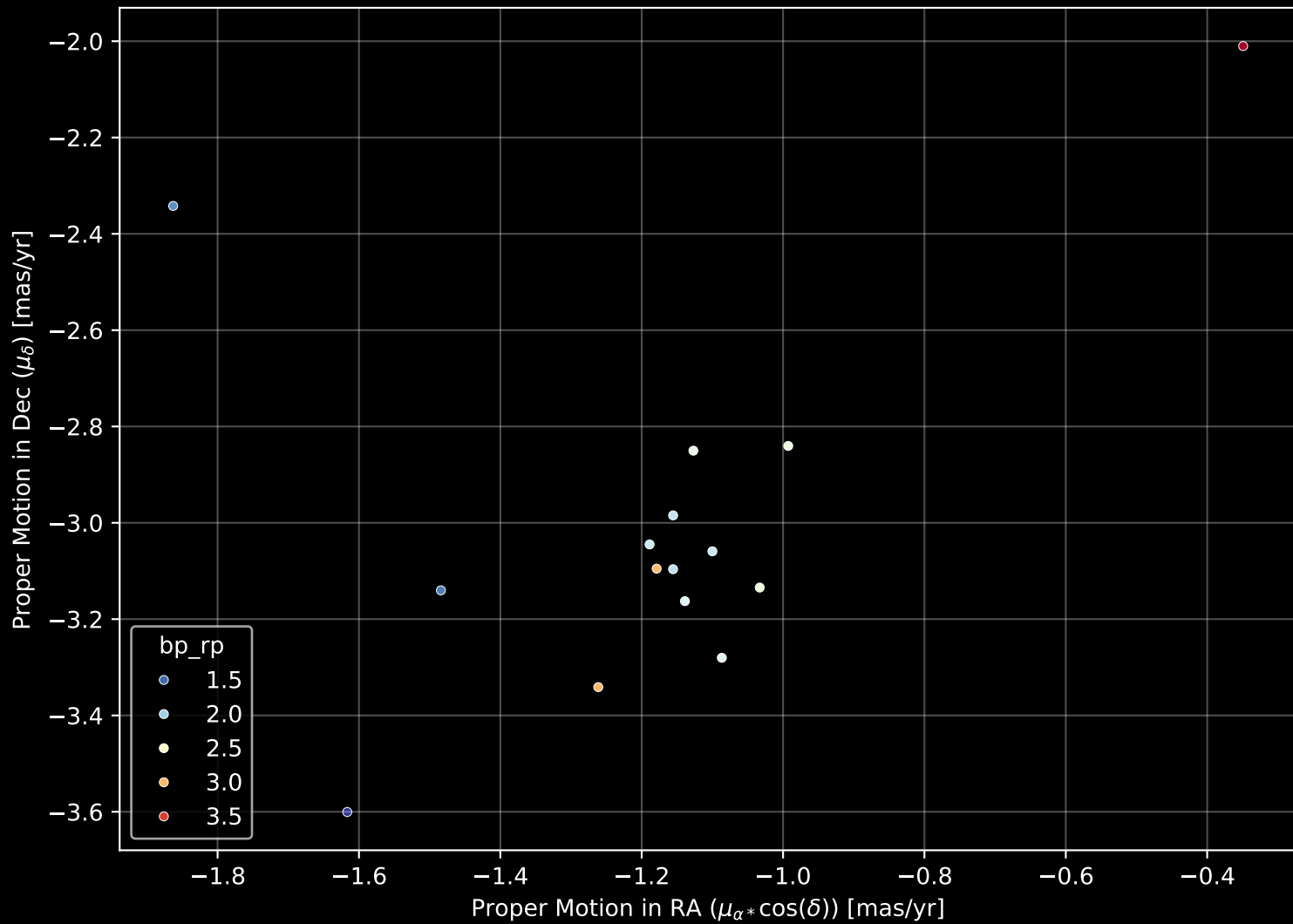
Gaia Cluster: [FSR_1032] Proper Motion Diagram (n= 15)
