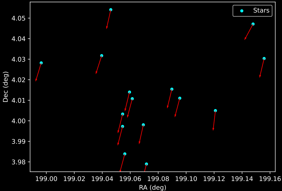
Gaia Cluster: [FSR_1032] Proper Motion Vectors for Gaia Star Field (n= 15)
