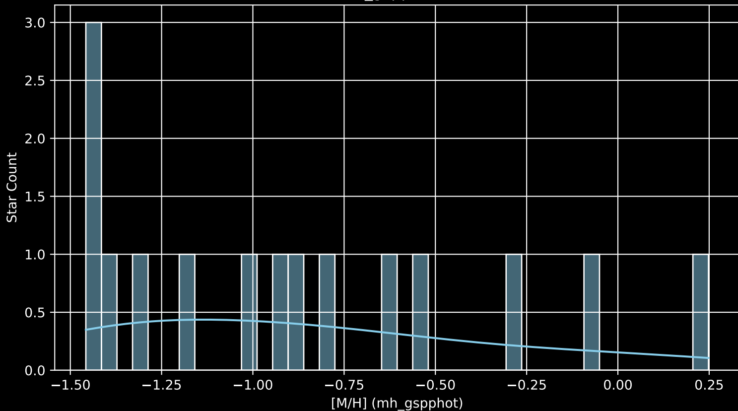
Gaia Cluster: [FSR_1032 [M/H] (mh_gspphot) (n= 15)
