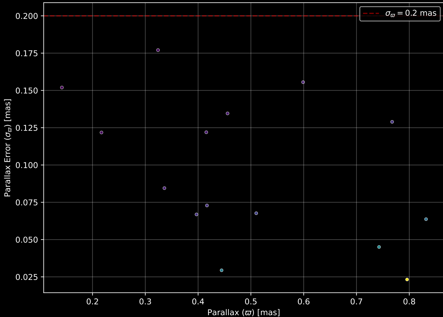
Gaia Cluster: [FSR_1032] Parallax Quality (n= 15)
