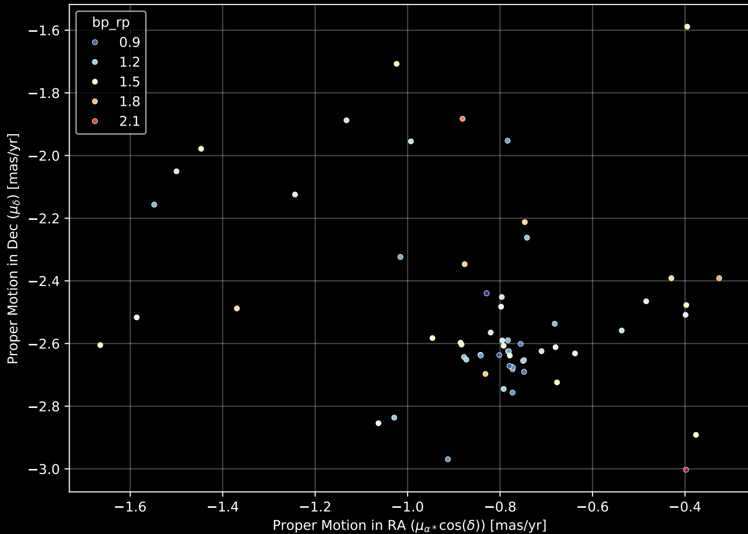
Gaia Cluster: [FSR_1051] Proper Motion Diagram (n= 62)
