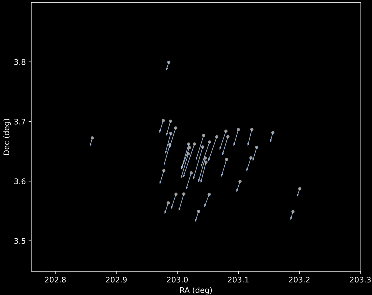
Gaia DR3 Cluster 1 Proper Motion Vectors (n=35)
