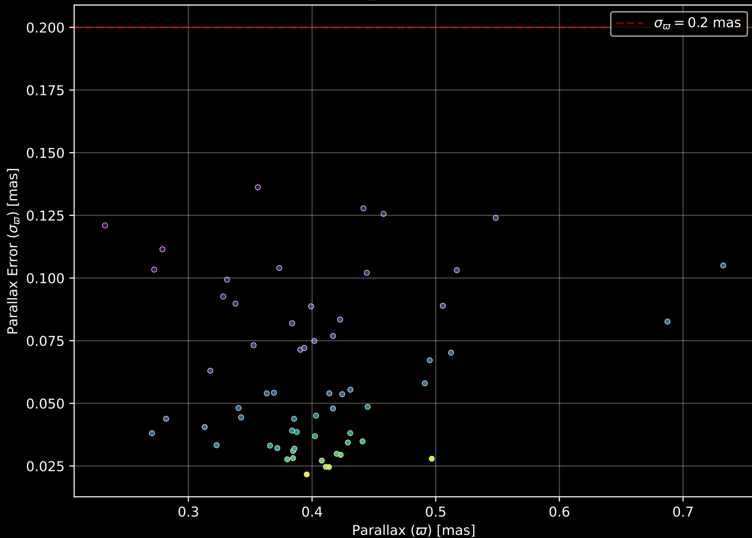
Gaia Cluster: [FSR_1051] Parallax Quality (n= 62)
