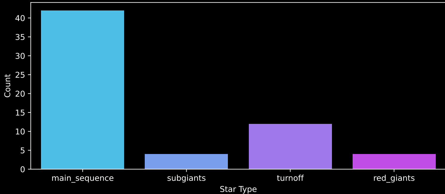
Gaia Cluster: [FSR_1051] Count plot of Star Type
