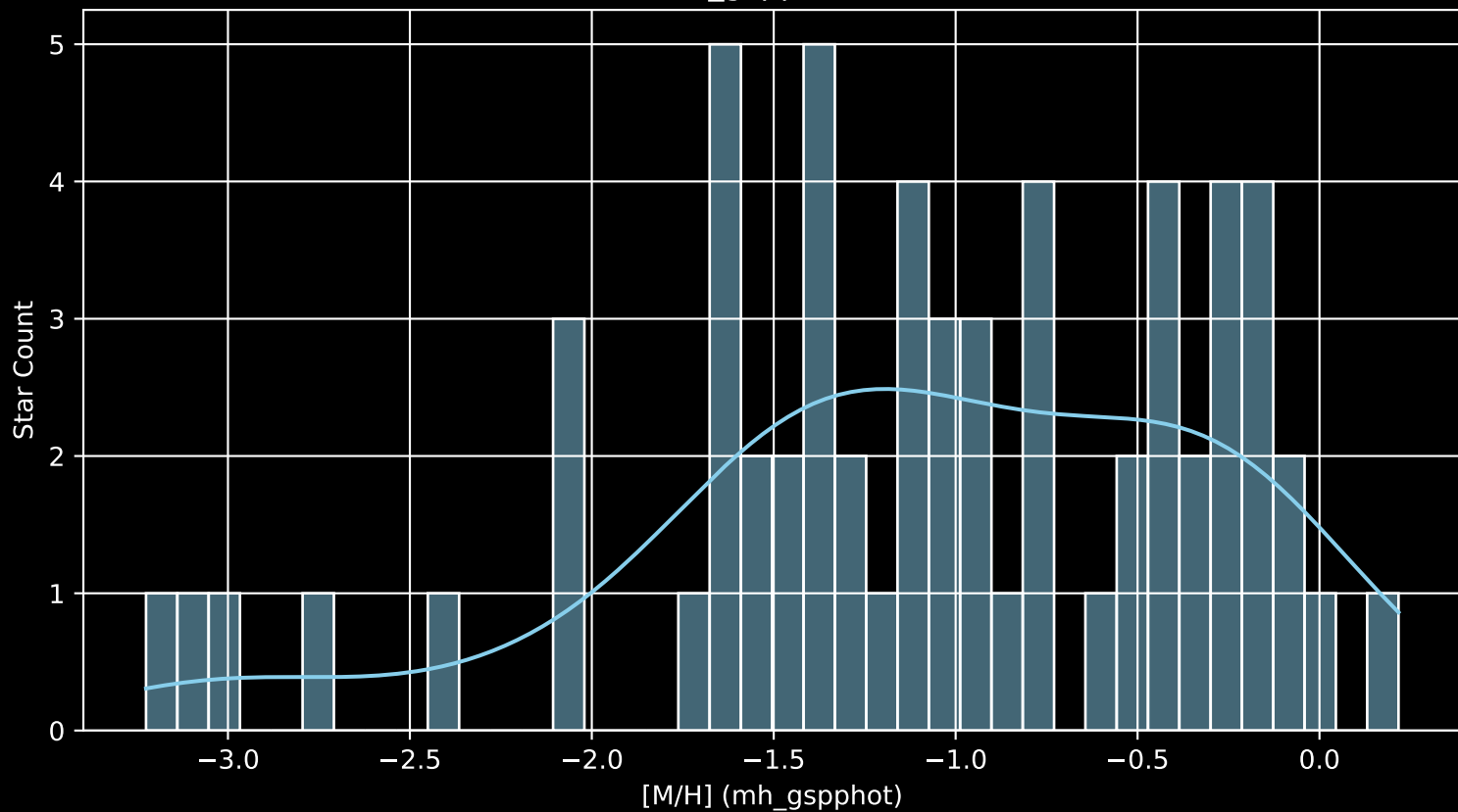
Gaia Cluster: [FSR_1051 [M/H] (mh_gspphot) (n= 62)
