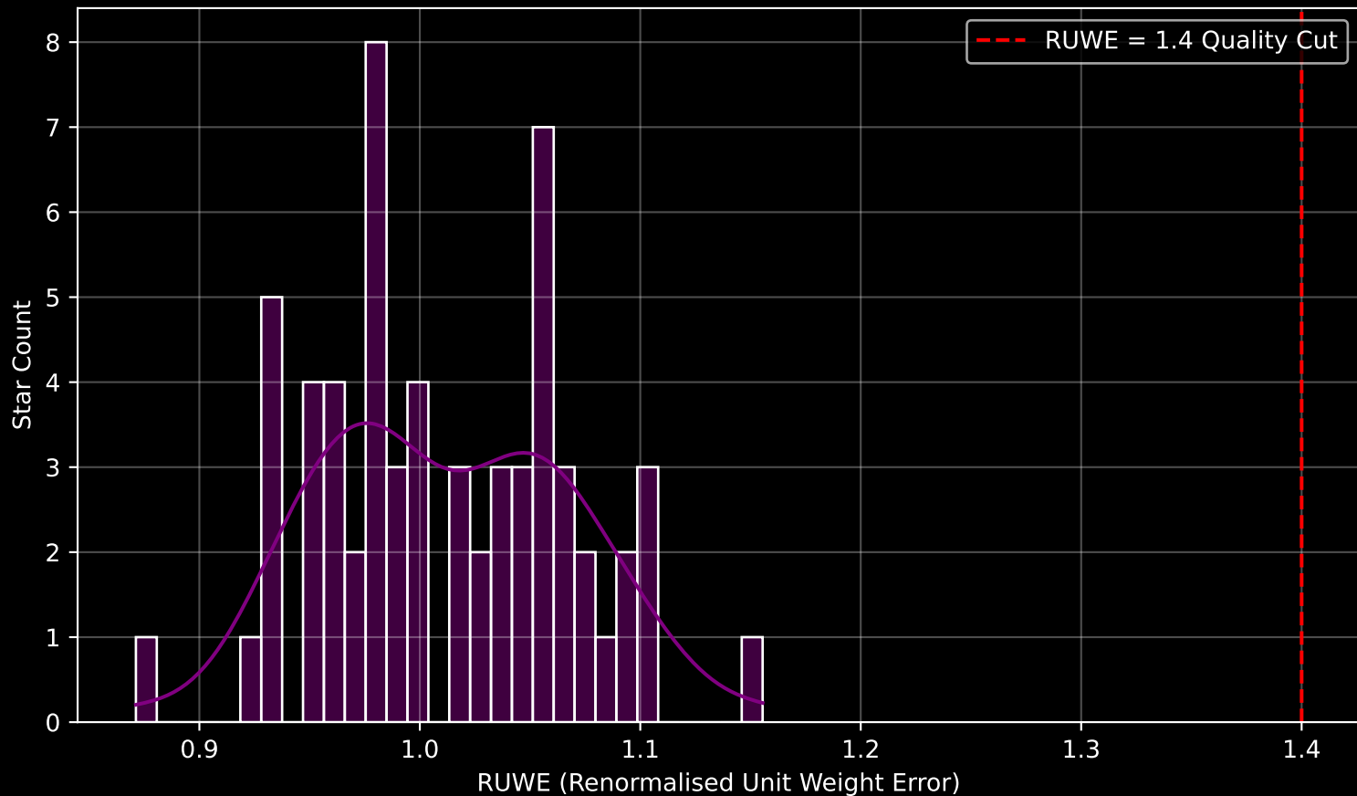
Gaia Cluster: [FSR_1051] RUWE Distribution (n= 62)
