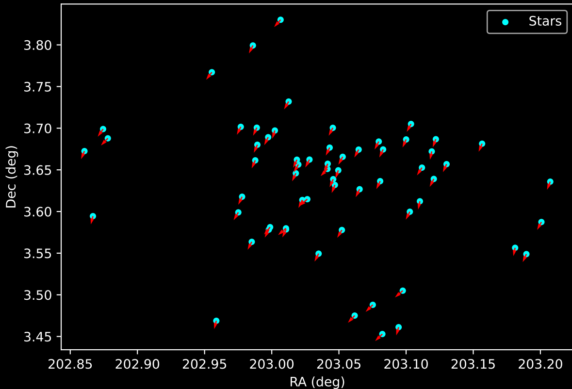
Gaia Cluster: [FSR_1051] Proper Motion Vectors for Gaia Star Field (n= 62)
