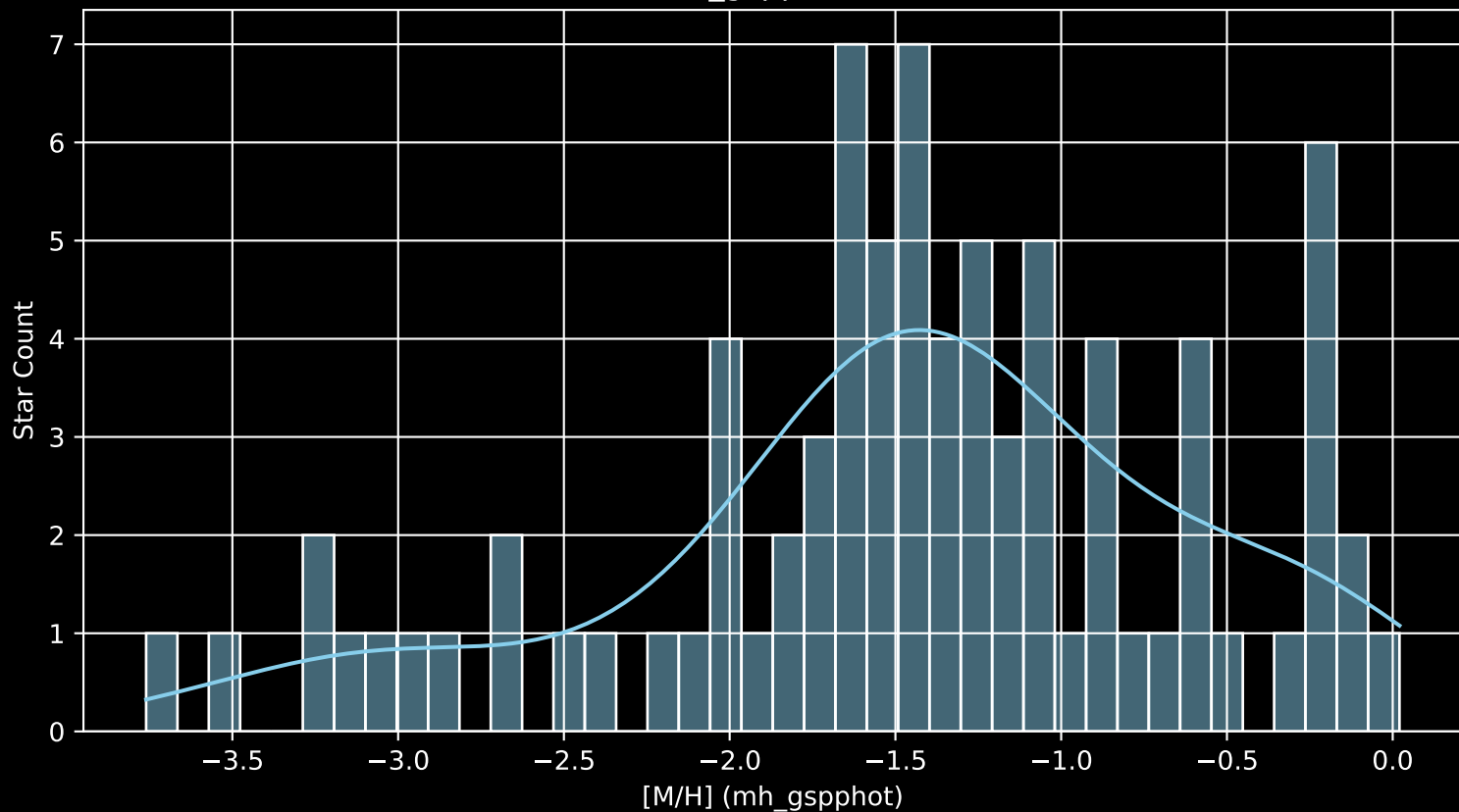
Gaia Cluster: [FSR_1063 [M/H] (mh_gspphot) (n= 82)
