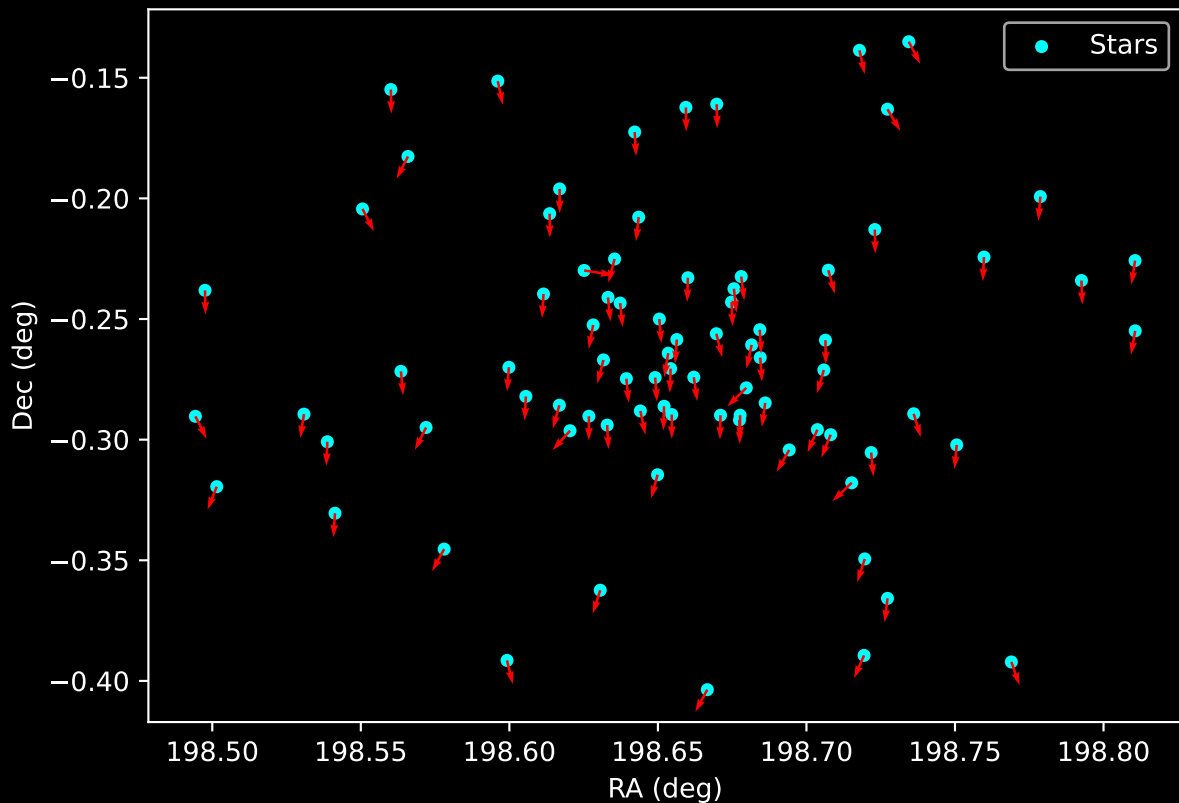
Gaia Cluster: [FSR_1063] Proper Motion Vectors for Gaia Star Field (n= 82)
