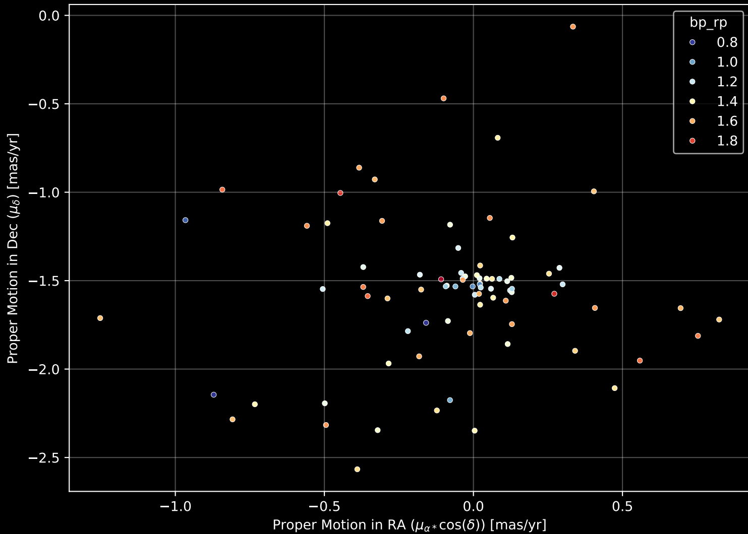
Gaia Cluster: [FSR_1063] Proper Motion Diagram (n= 82)
