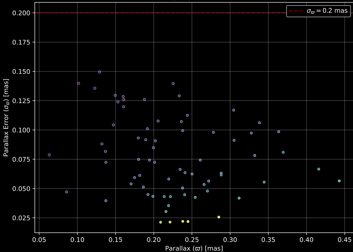
Gaia Cluster: [FSR_1113] Parallax Quality (n= 70)
