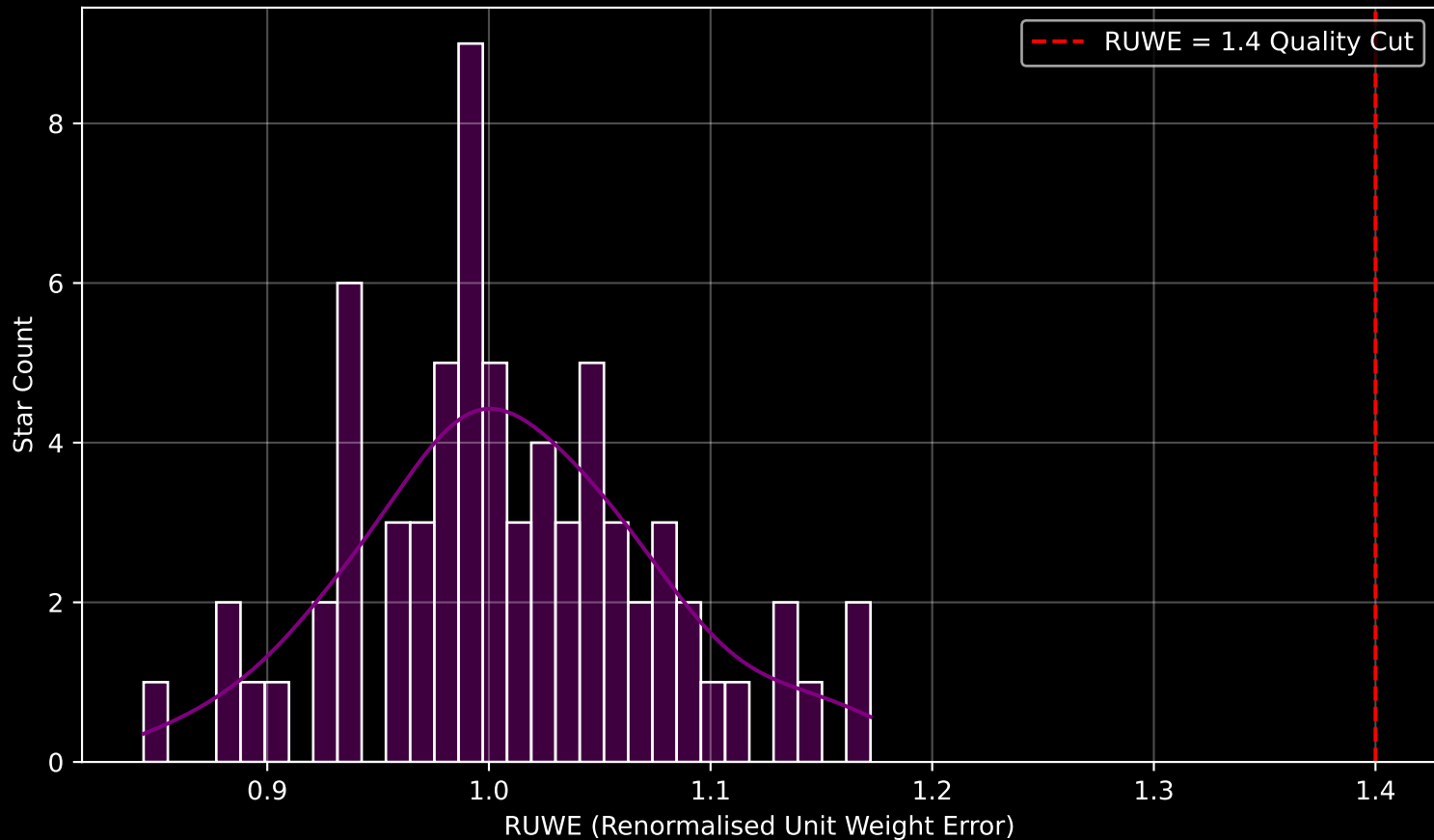
Gaia Cluster: [FSR_1113] RUWE Distribution (n= 70)
