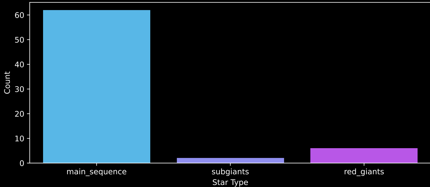
Gaia Cluster: [FSR_1113] Count plot of Star Type
