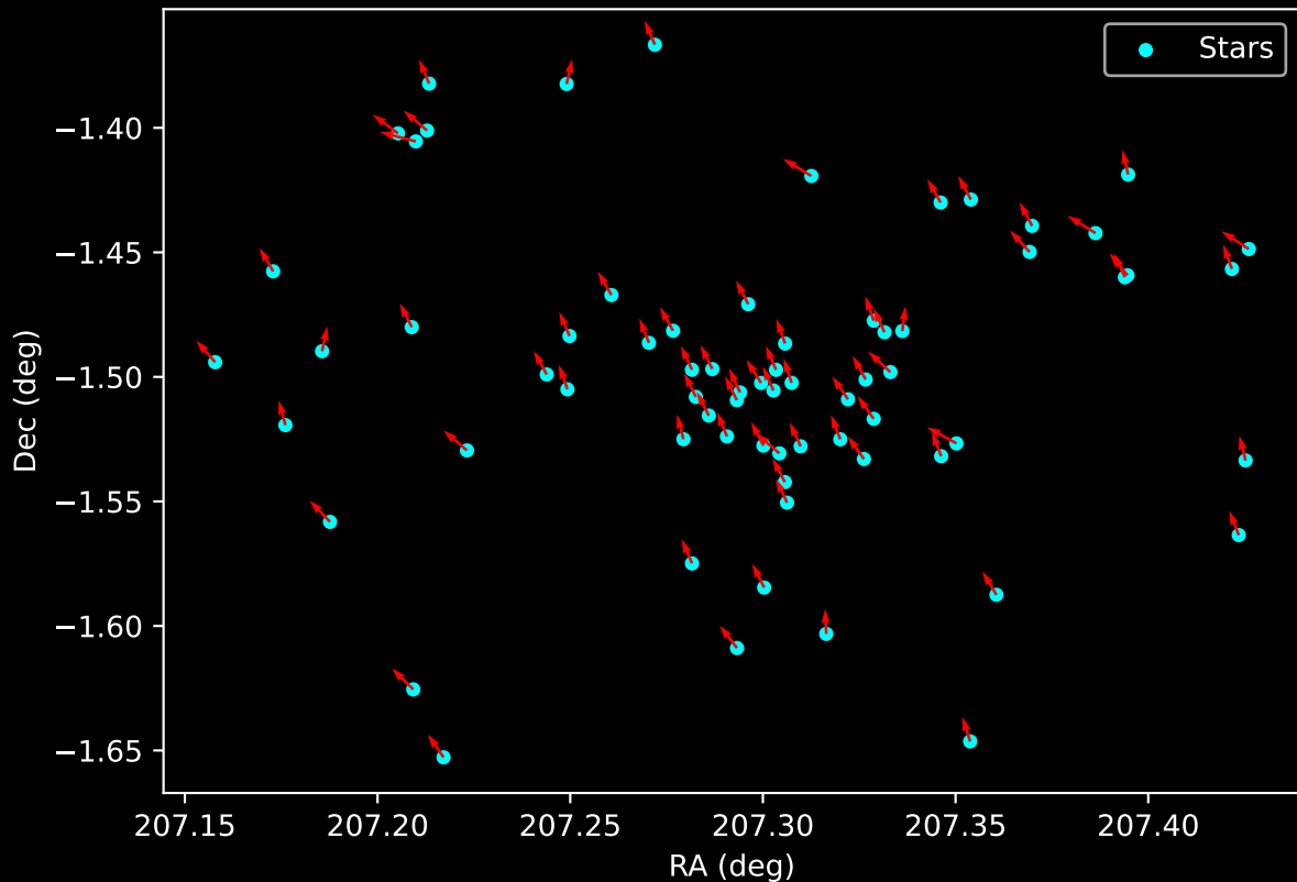
Gaia Cluster: [FSR_1113] Proper Motion Vectors for Gaia Star Field (n= 70)
