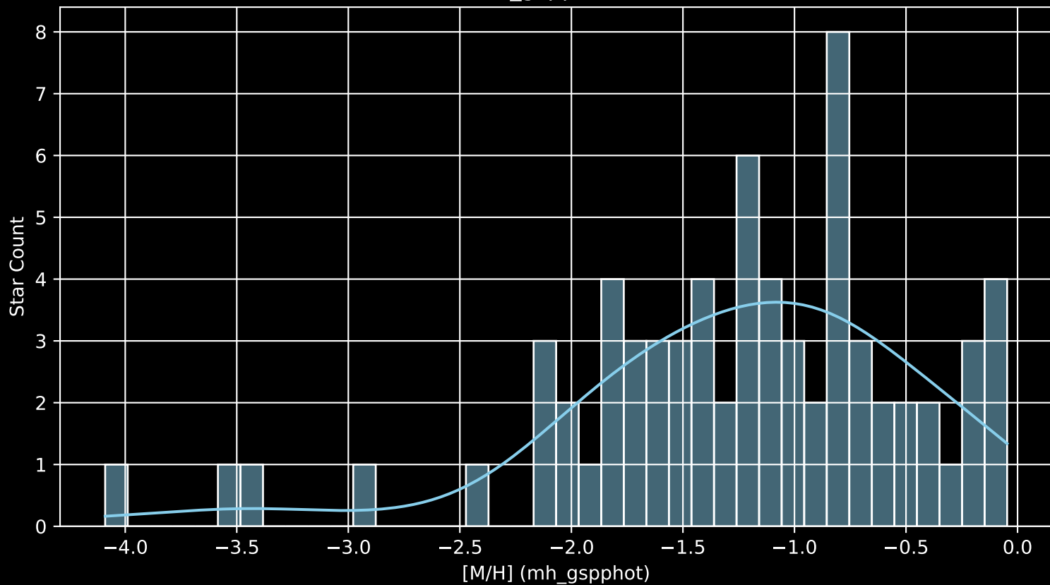
Gaia Cluster: [FSR_1113 [M/H] (mh_gspphot) (n= 70)
