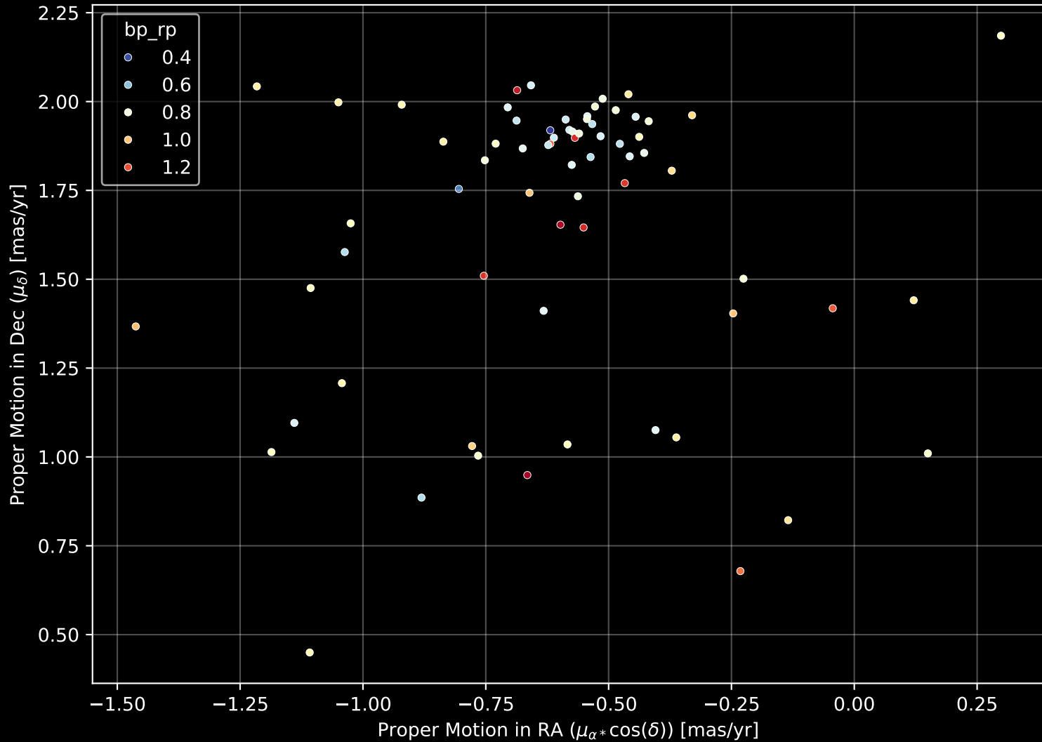
Gaia Cluster: [FSR_1113] Proper Motion Diagram (n= 70)
