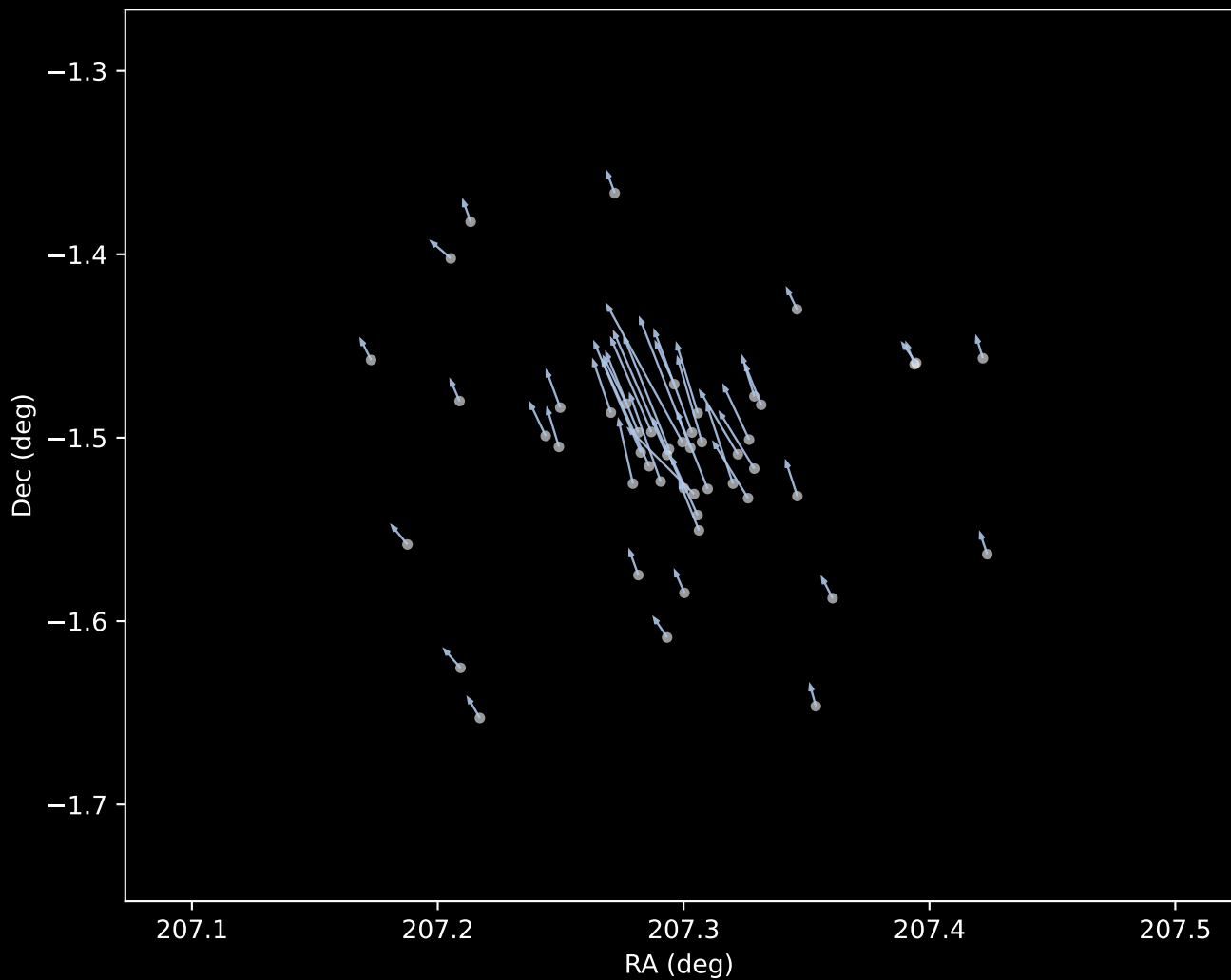
Gaia DR3 Cluster 1 Proper Motion Vectors (n=50)
