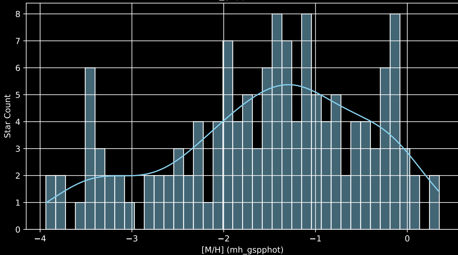
Gaia Cluster: [FSR_1163 [M/H] (mh_gspphot) (n= 139)
