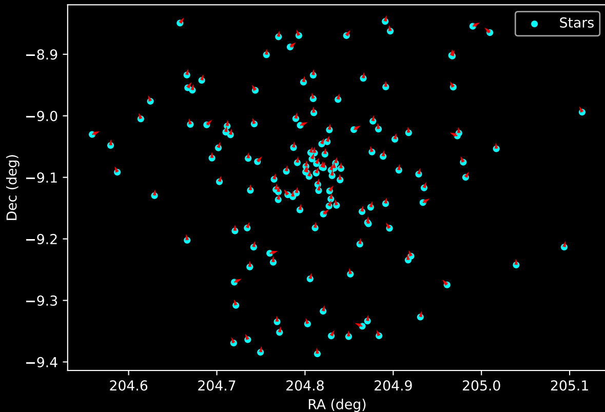
Gaia Cluster: [FSR_1163] Proper Motion Vectors for Gaia Star Field (n= 139)
