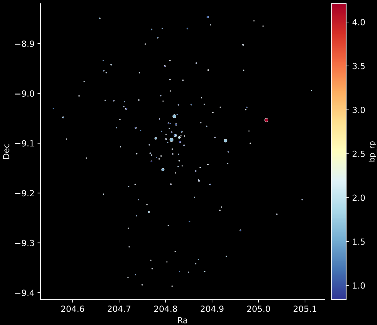
Gaia Cluster: [FSR_1163] Stars: 139
