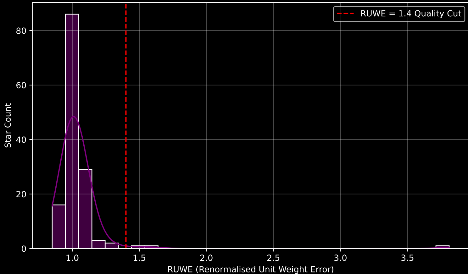
Gaia Cluster: [FSR_1163] RUWE Distribution (n= 139)
