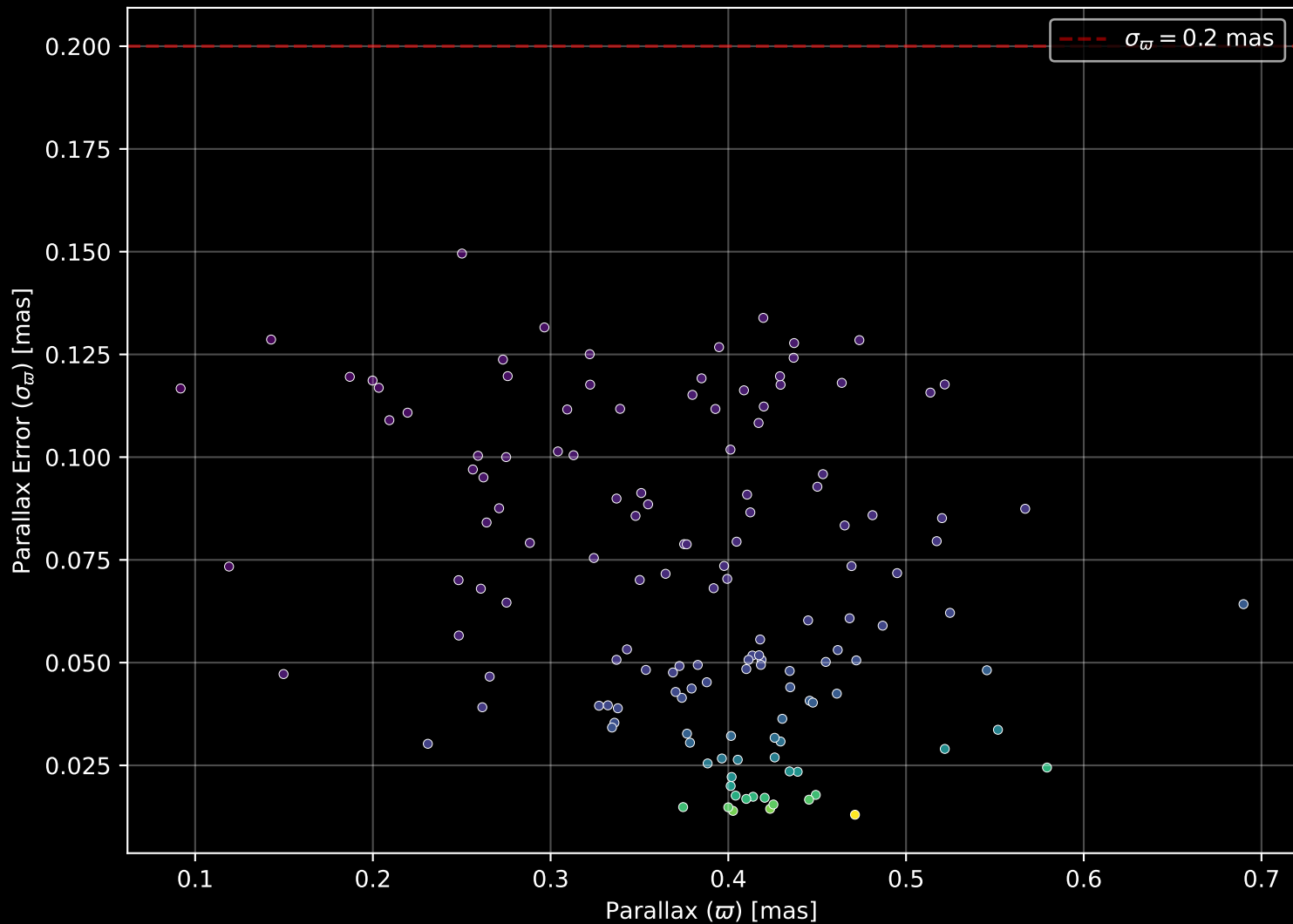
Gaia Cluster: [FSR_1163] Parallax Quality (n= 139)
