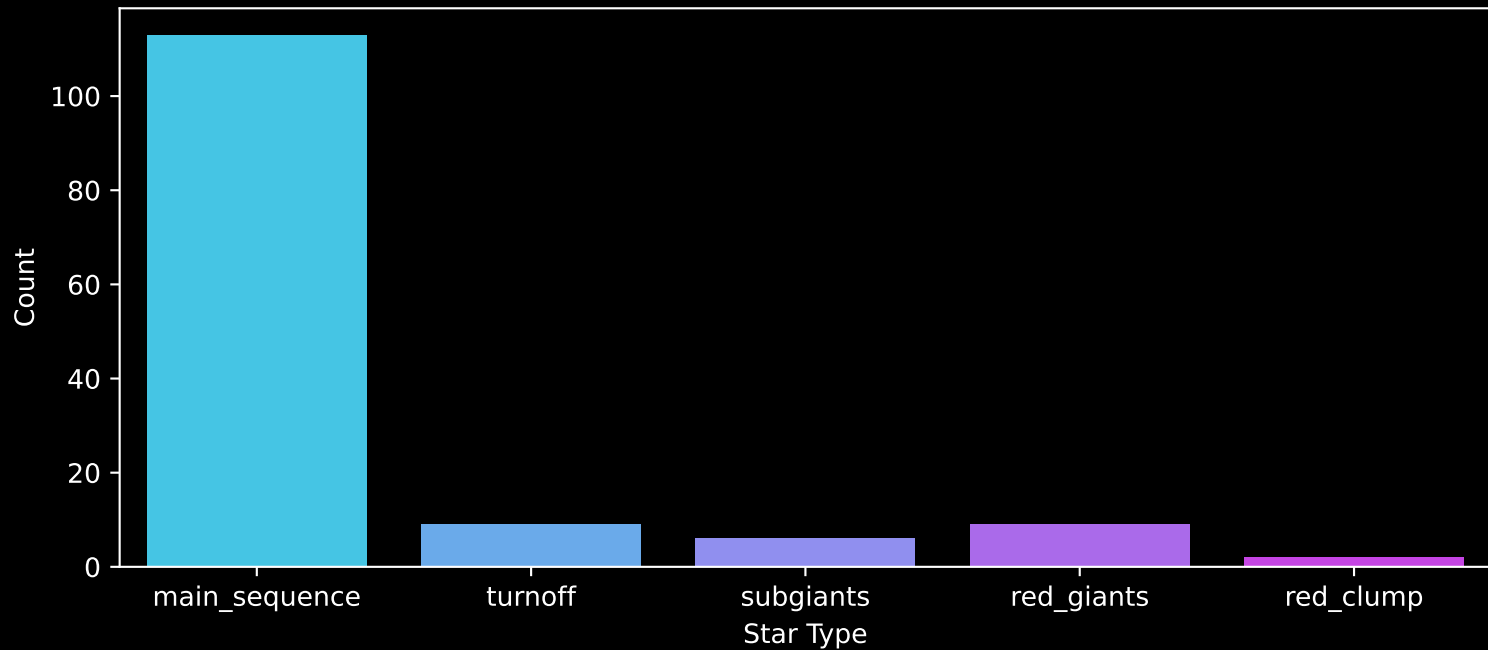
Gaia Cluster: [FSR_1163] Count plot of Star Type
