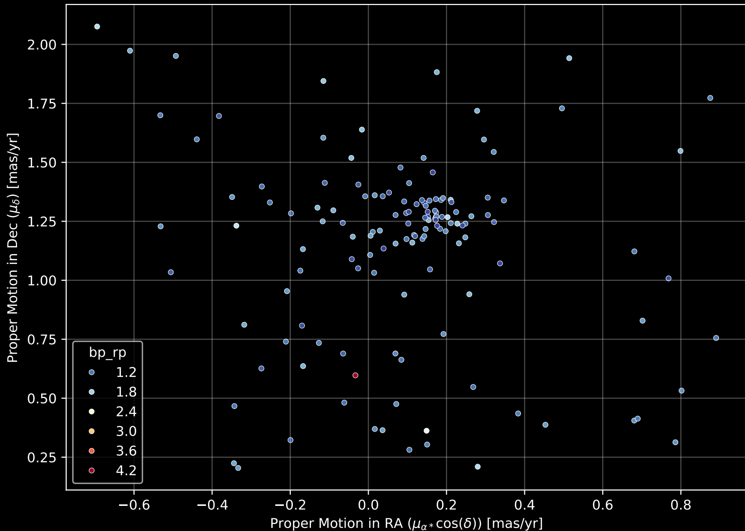
Gaia Cluster: [FSR_1163] Proper Motion Diagram (n= 139)
