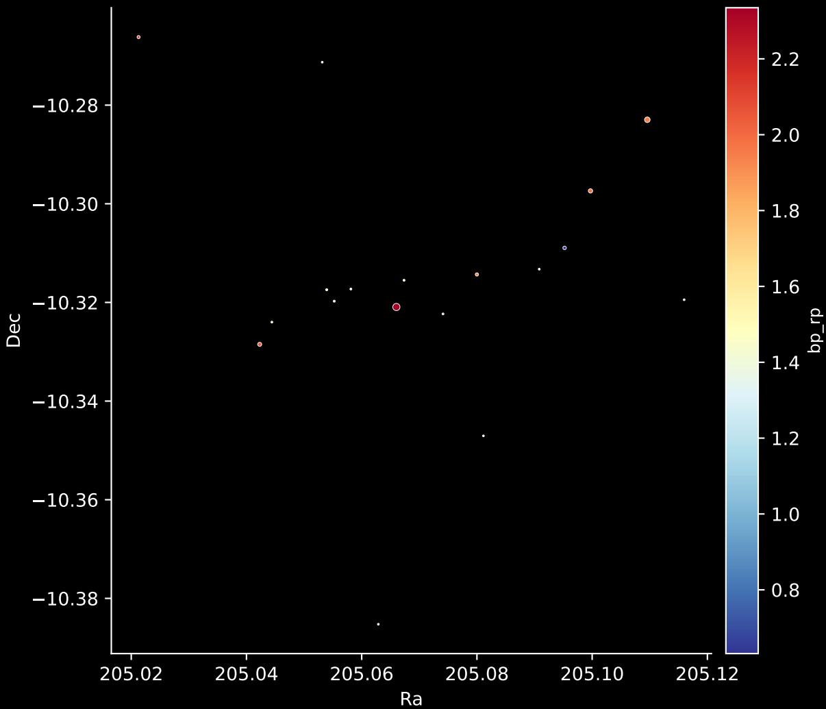
Gaia Cluster: [FSR_1171] Stars: 18
