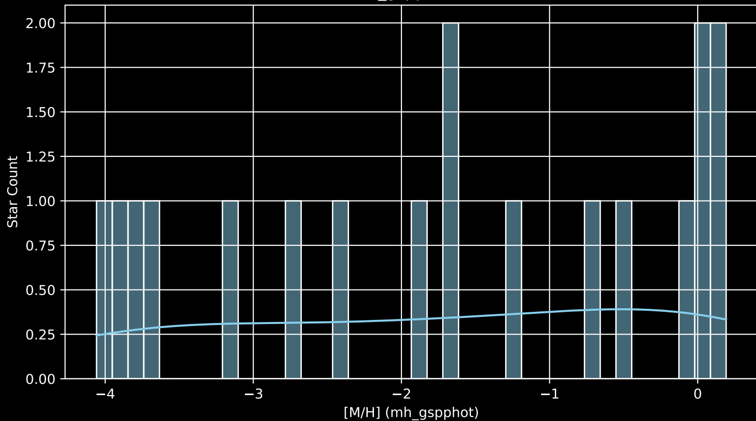
Gaia Cluster: [FSR_1171 [M/H] (mh_gspphot) (n= 18)
