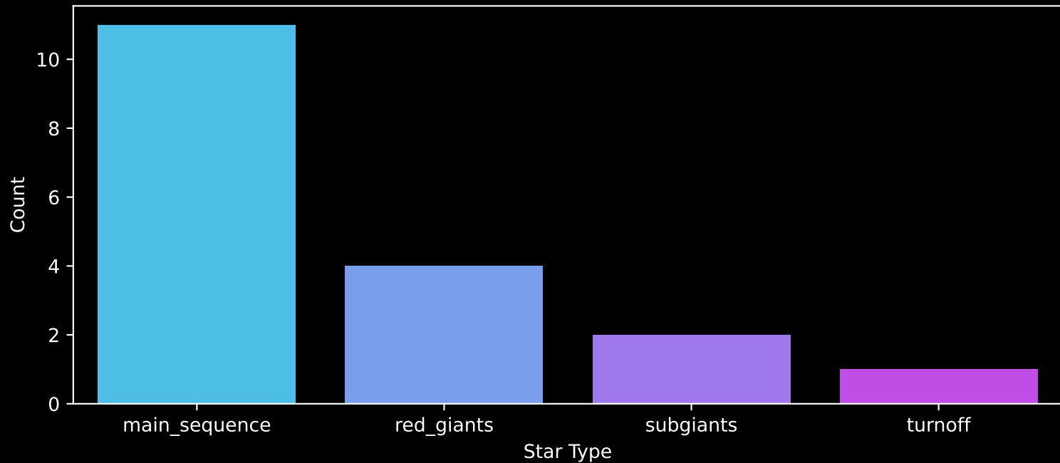
Gaia Cluster: [FSR_1171] Count plot of Star Type
