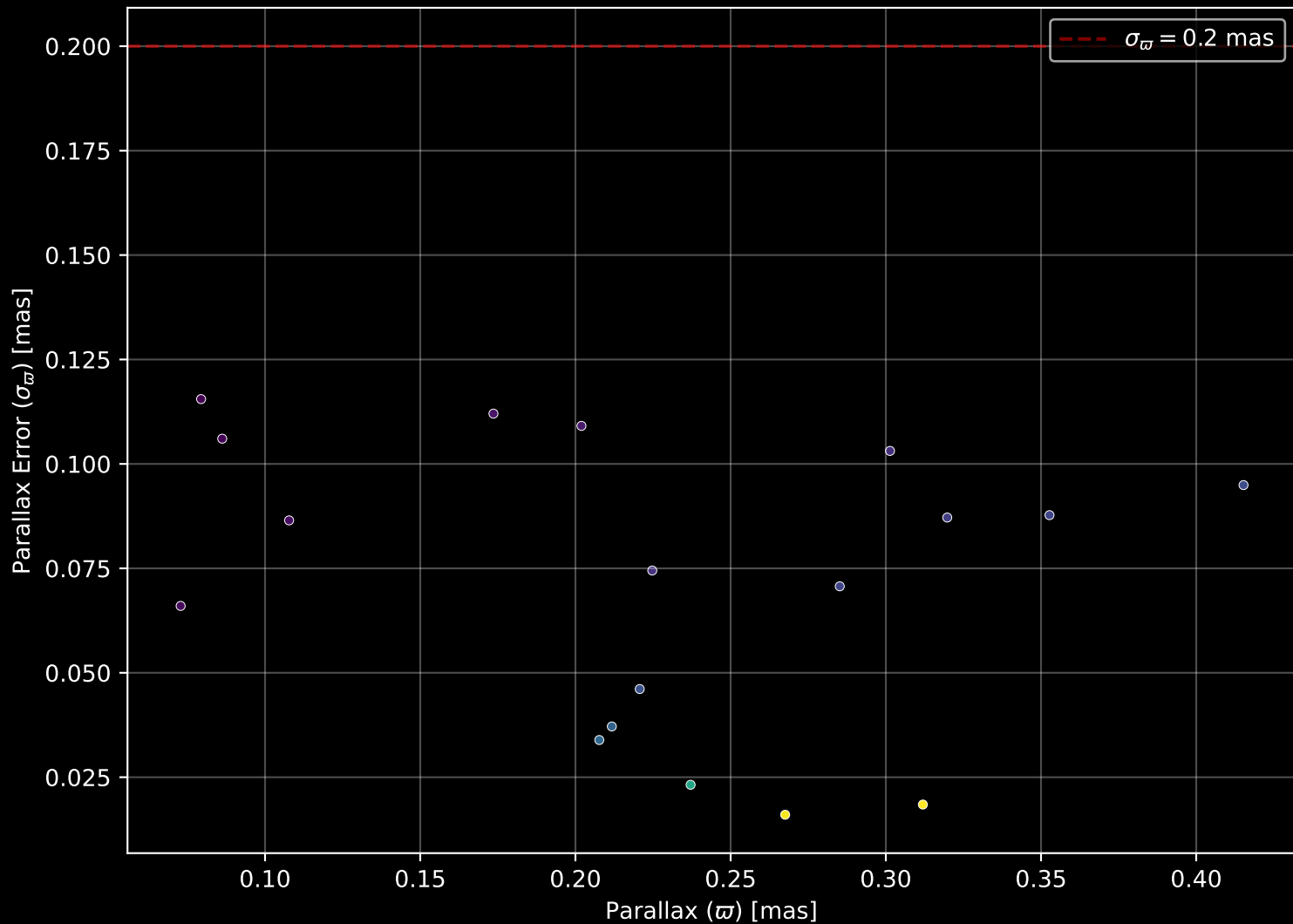
Gaia Cluster: [FSR_1171] Parallax Quality (n= 18)
