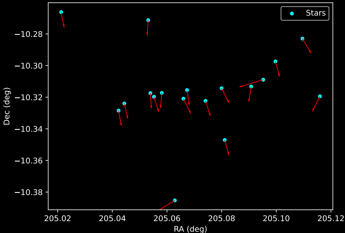
Gaia Cluster: [FSR_1171] Proper Motion Vectors for Gaia Star Field (n= 18)
