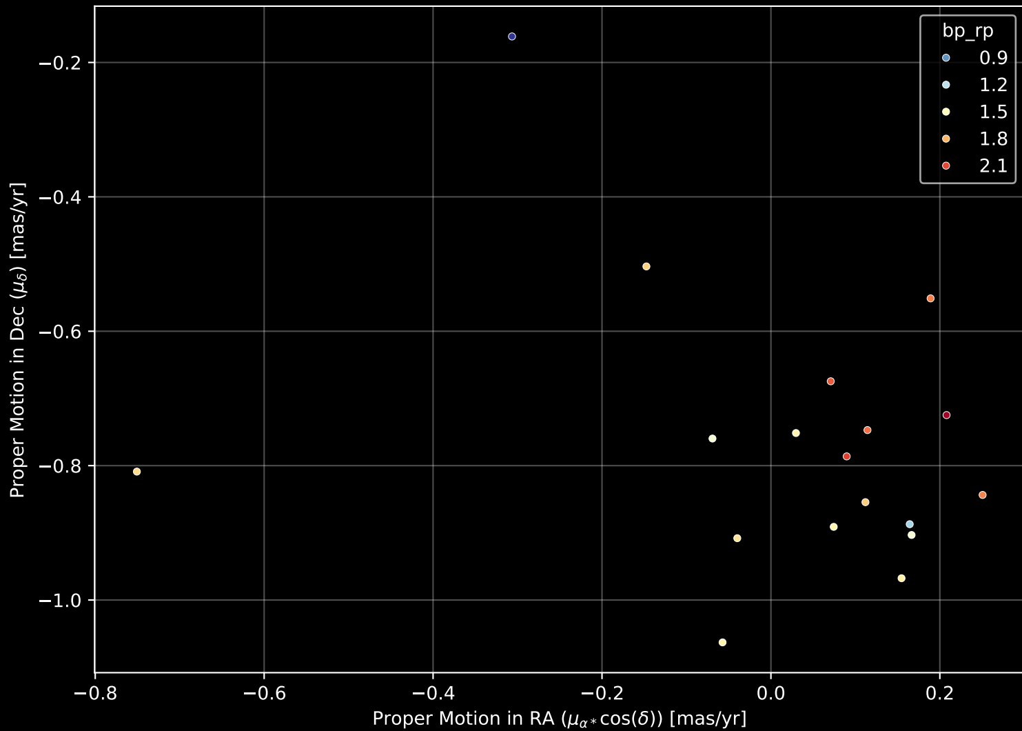
Gaia Cluster: [FSR_1171] Proper Motion Diagram (n= 18)
