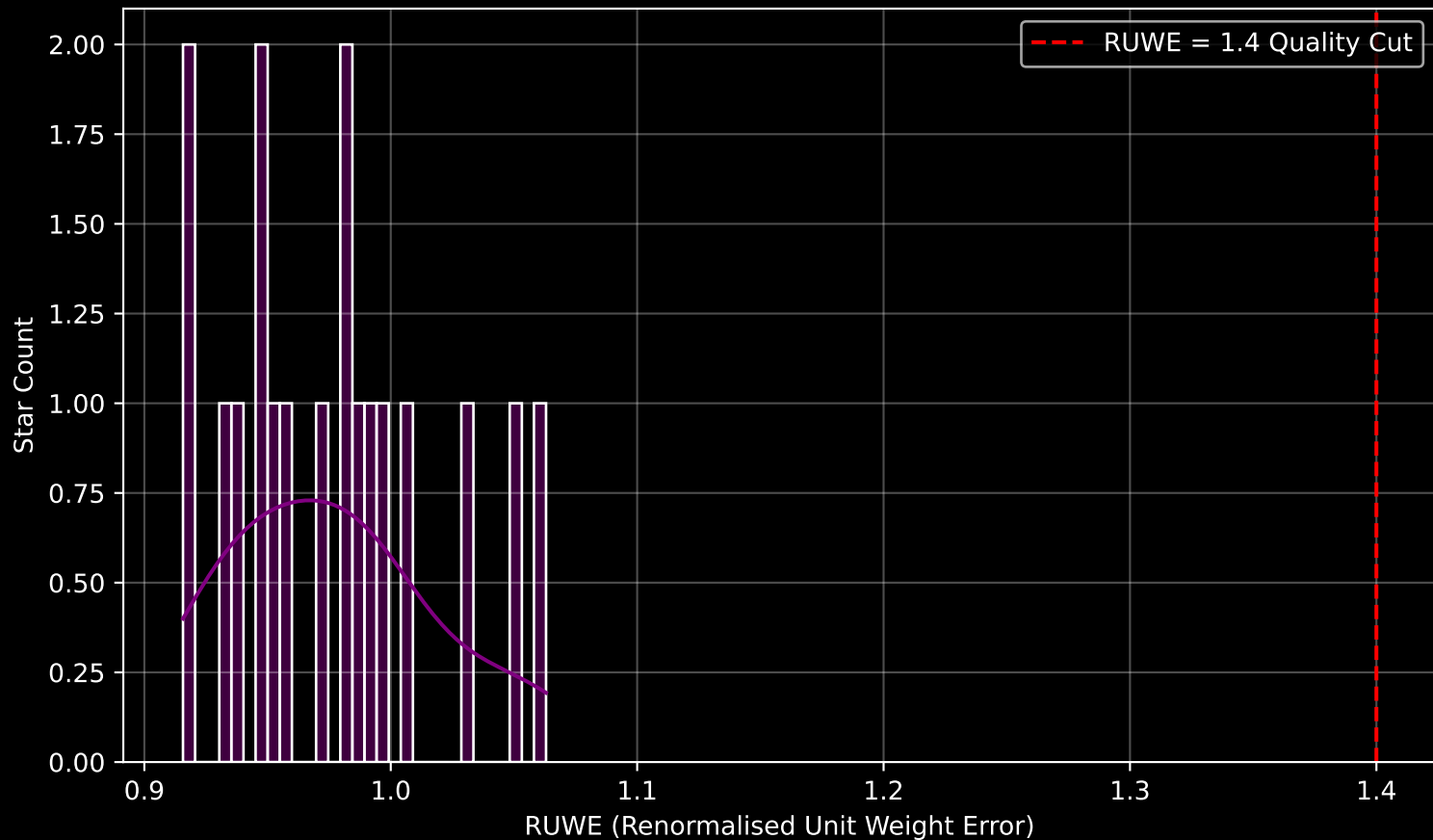
Gaia Cluster: [FSR_1171] RUWE Distribution (n= 18)
