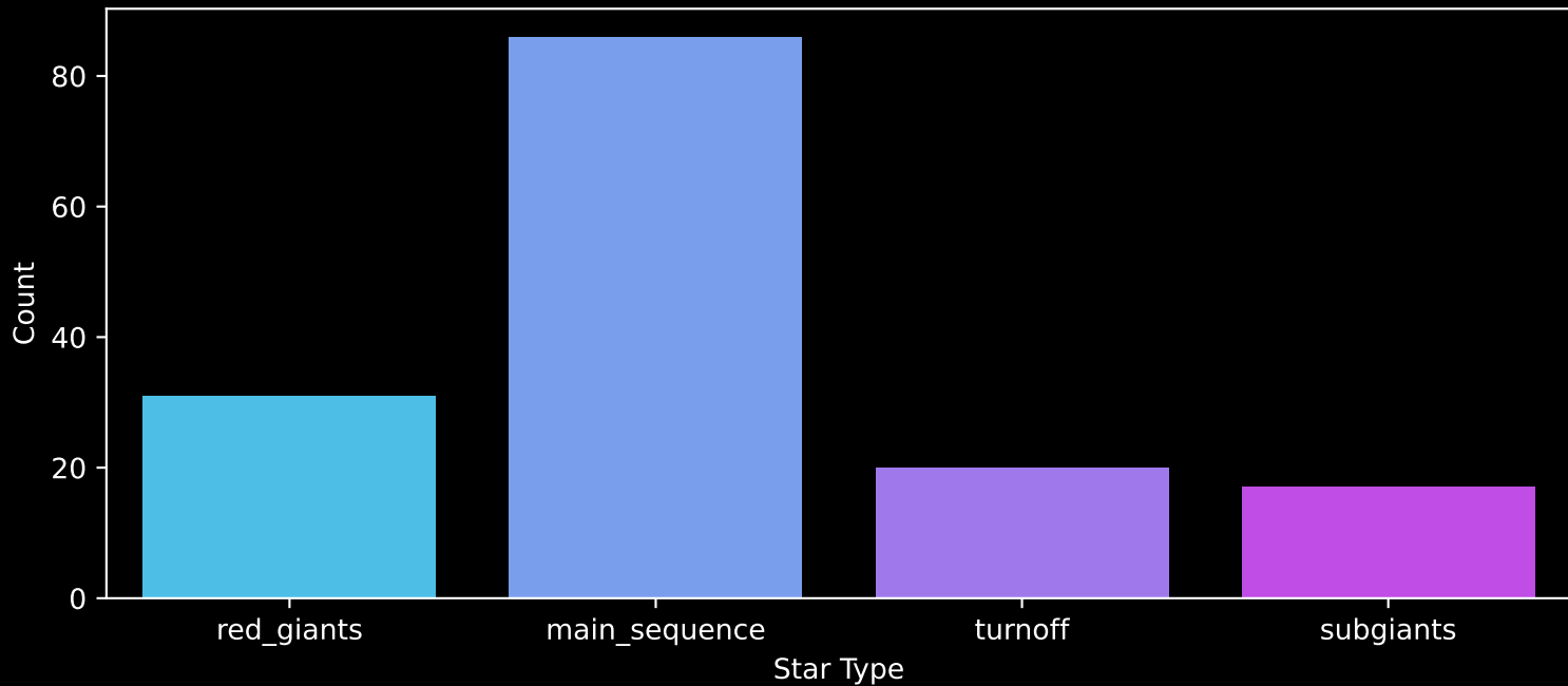
Gaia Cluster: [FSR_1180] Count plot of Star Type
