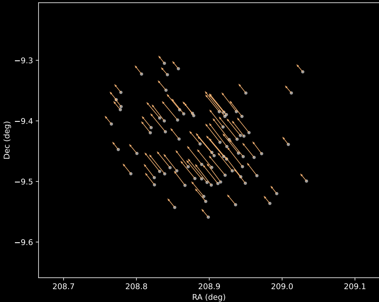
Gaia DR3 Cluster 3 Proper Motion Vectors (n=81)
