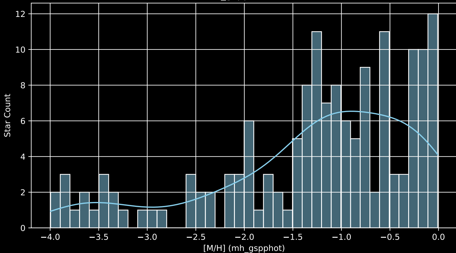
Gaia Cluster: [FSR_1180 [M/H] (mh_gspphot) (n= 154)
