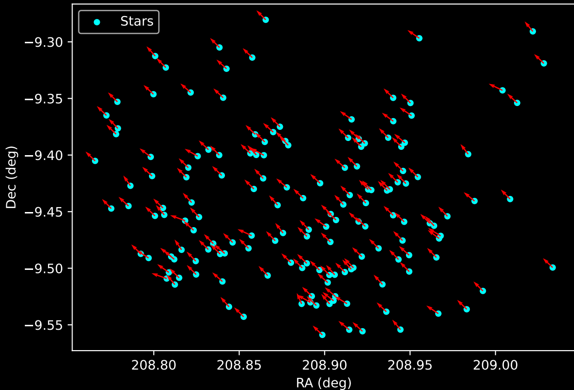
Gaia Cluster: [FSR_1180] Proper Motion Vectors for Gaia Star Field (n= 154)
