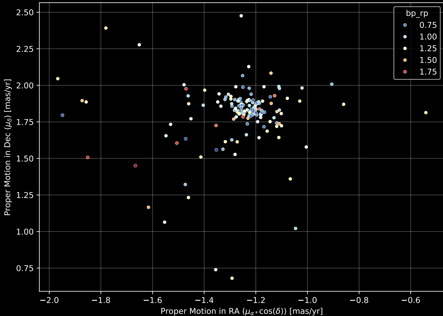
Gaia Cluster: [FSR_1180] Proper Motion Diagram (n= 154)
