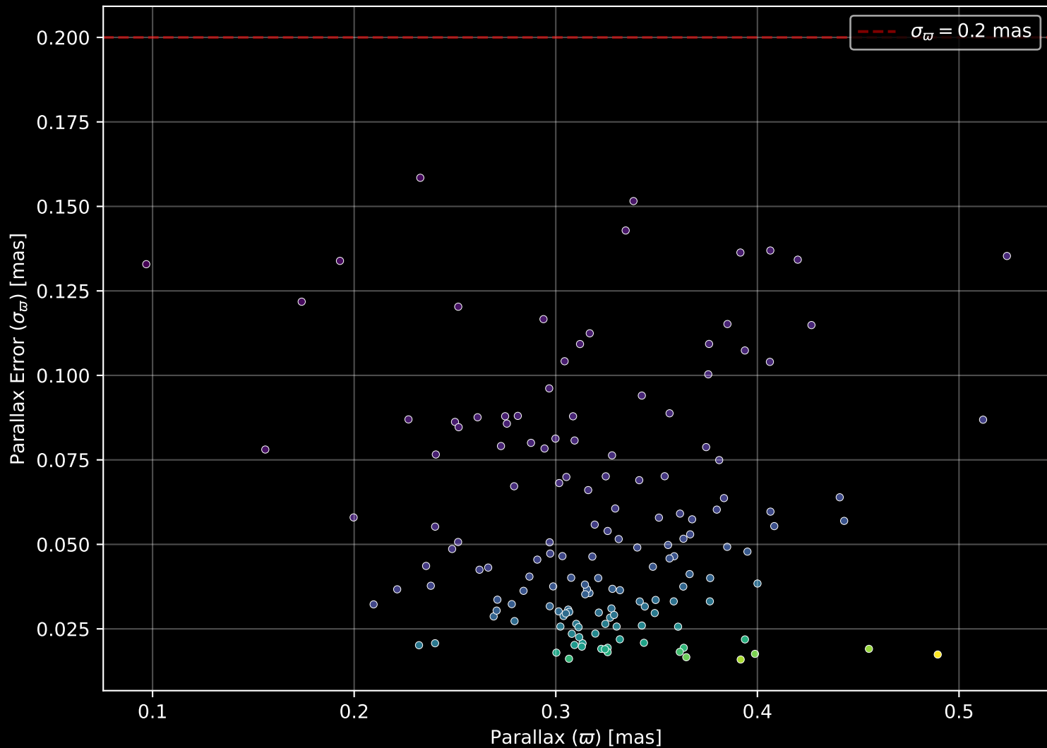
Gaia Cluster: [FSR_1180] Parallax Quality (n= 154)
