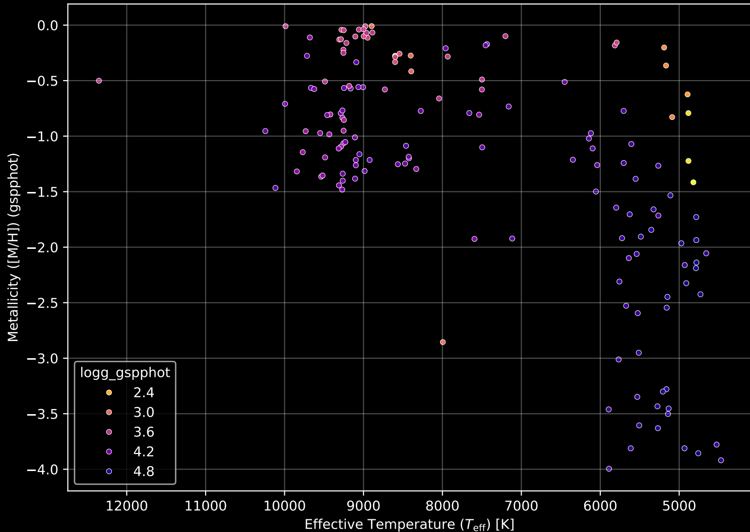
Gaia Cluster: [FSR_1180] Stellar Population Parameters (n= 154)
