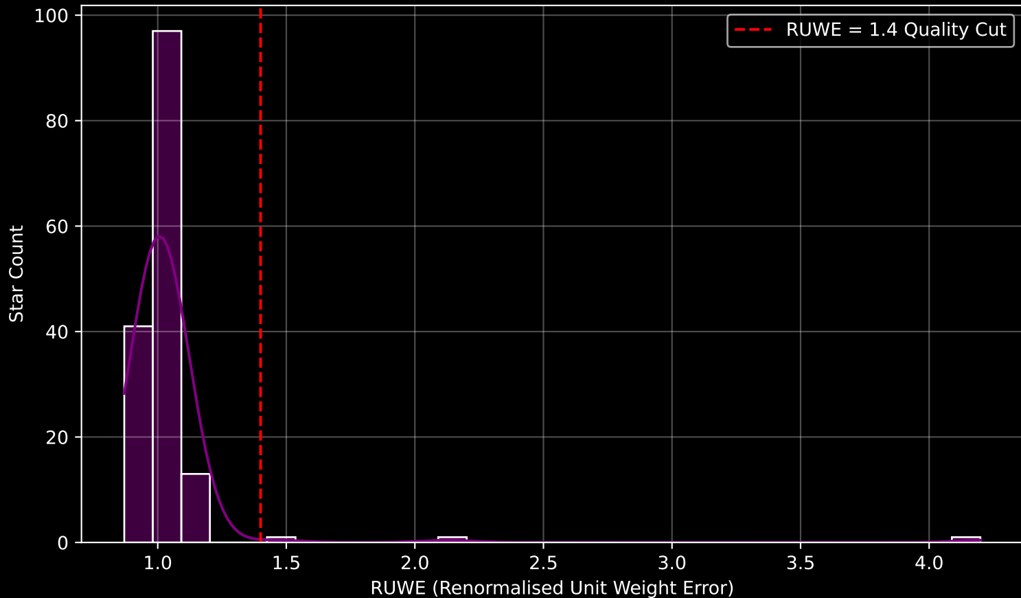
Gaia Cluster: [FSR_1180] RUWE Distribution (n= 154)
