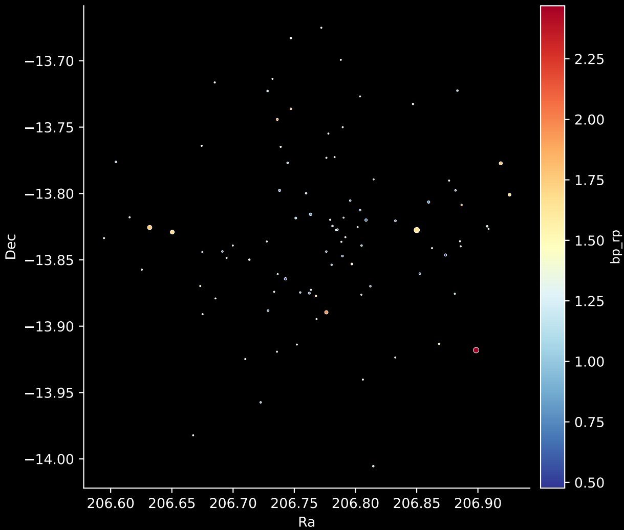
Gaia Cluster: [FSR_1209] Stars: 92
