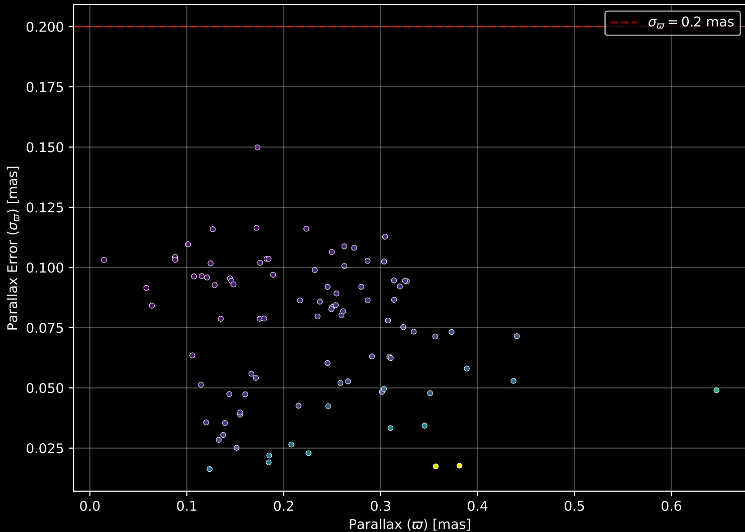
Gaia Cluster: [FSR_1209] Parallax Quality (n= 92)
