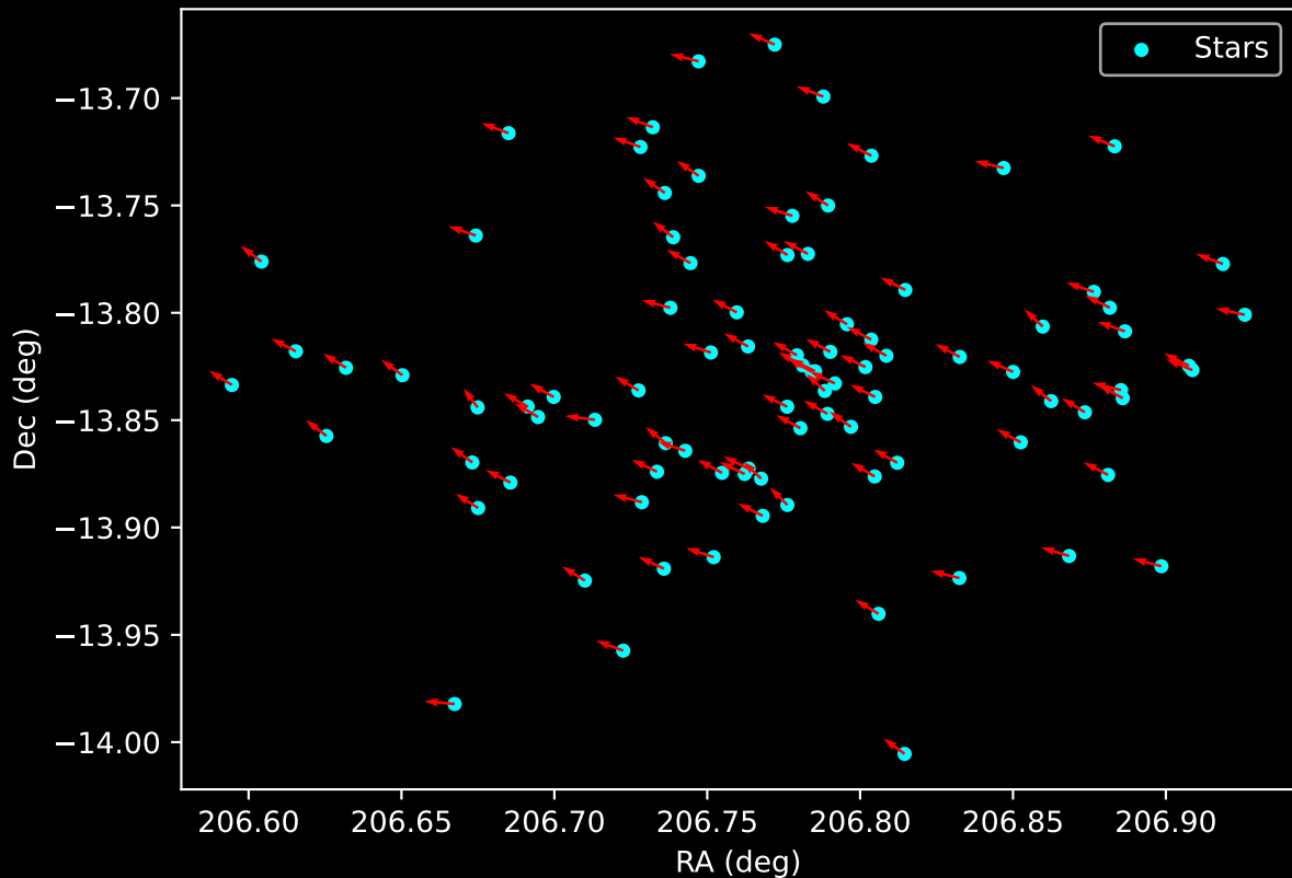
Gaia Cluster: [FSR_1209] Proper Motion Vectors for Gaia Star Field (n= 92)
