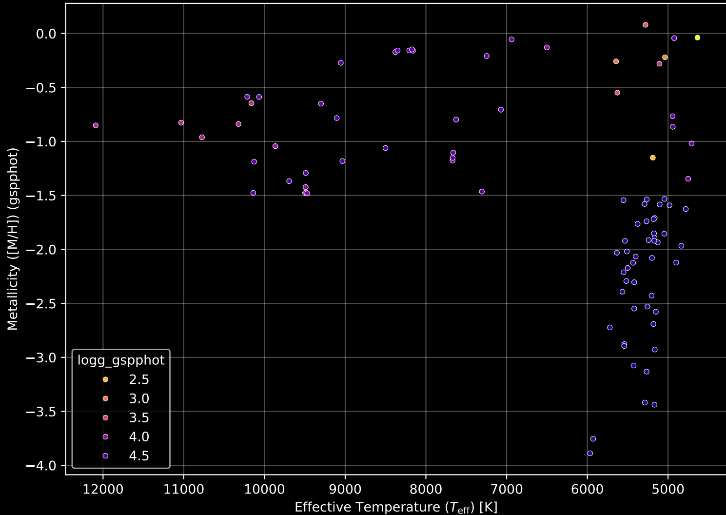
Gaia Cluster: [FSR_1209] Stellar Population Parameters (n= 92)
