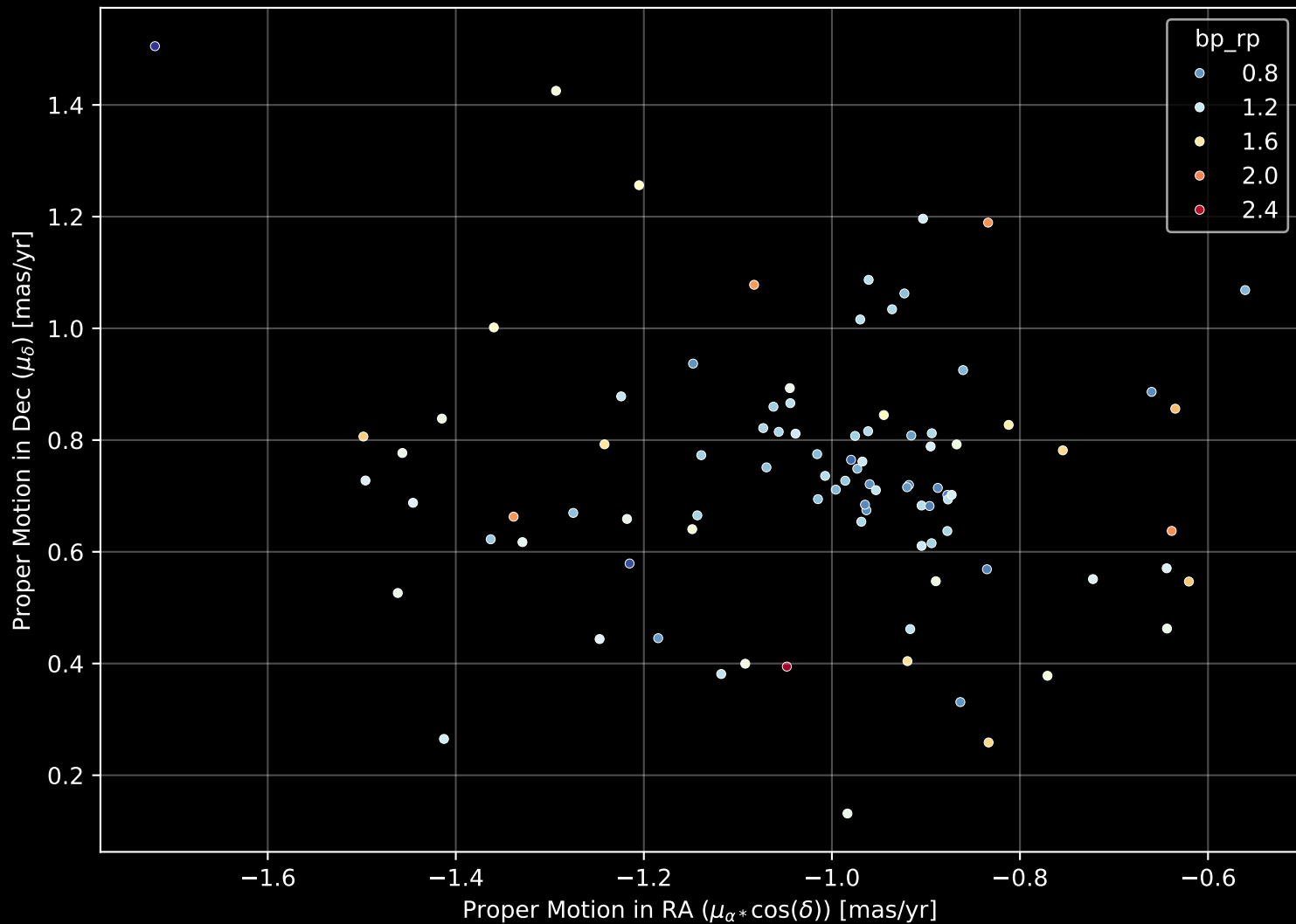
Gaia Cluster: [FSR_1209] Proper Motion Diagram (n= 92)
