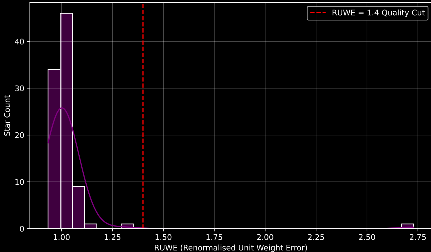
Gaia Cluster: [FSR_1209] RUWE Distribution (n= 92)
