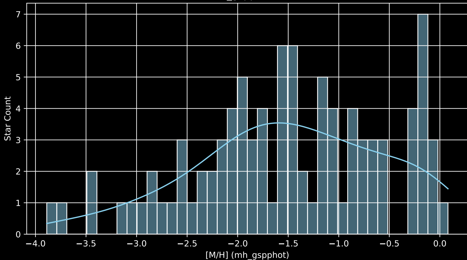
Gaia Cluster: [FSR_1209 [M/H] (mh_gspphot) (n= 92)
