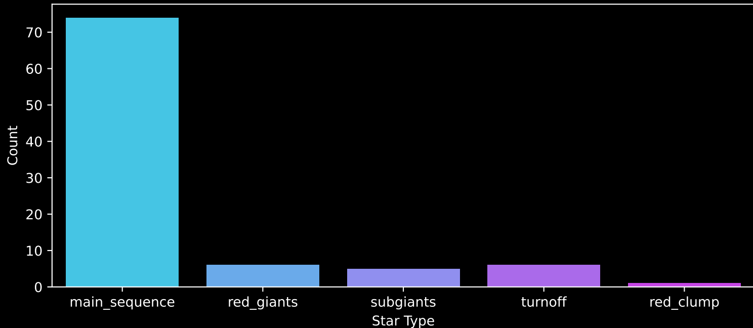
Gaia Cluster: [FSR_1209] Count plot of Star Type
