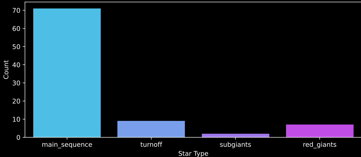
Gaia Cluster: [FSR_1211] Count plot of Star Type
