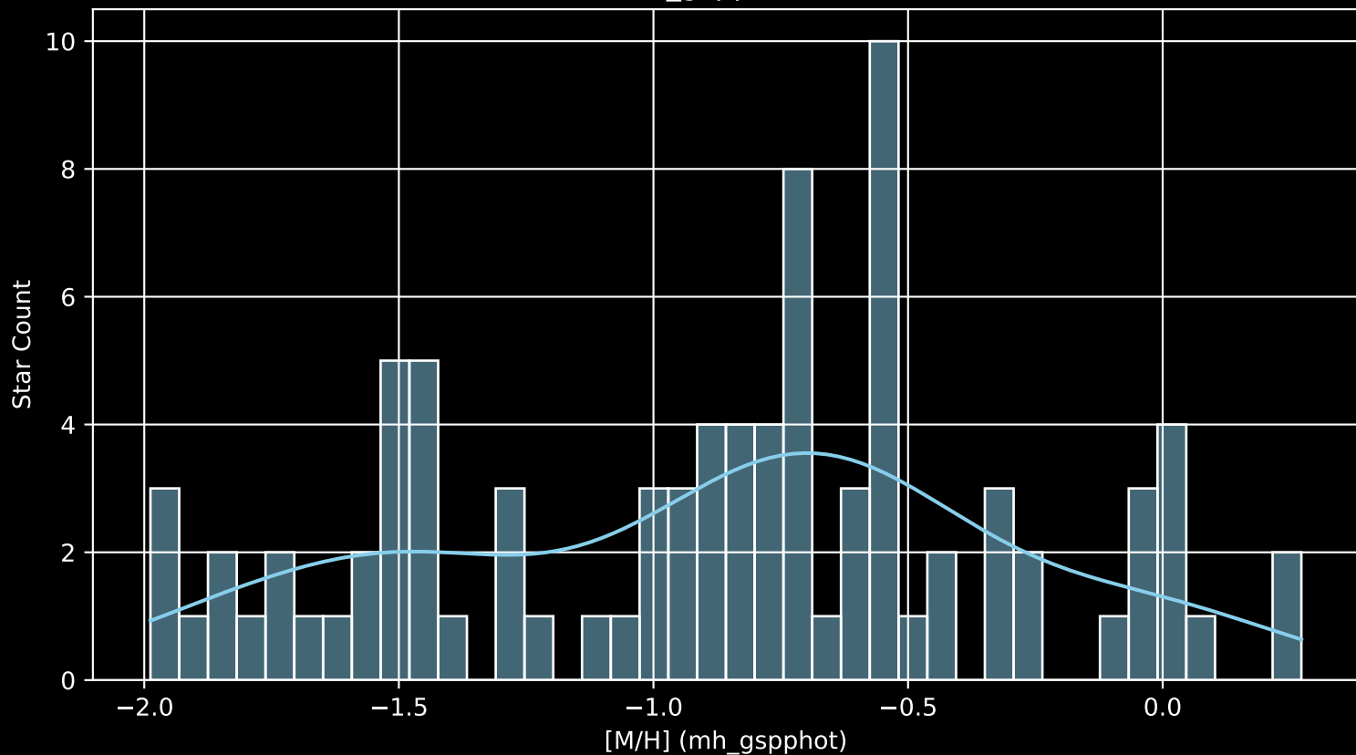
Gaia Cluster: [FSR_1211 [M/H] (mh_gspphot) (n= 89)
