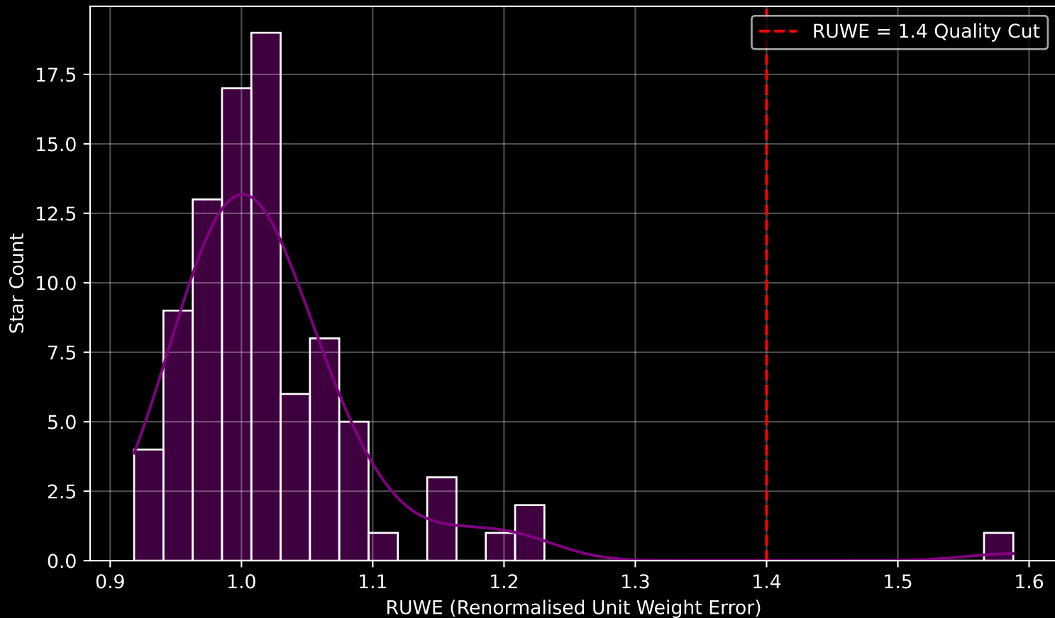
Gaia Cluster: [FSR_1211] RUWE Distribution (n= 89)
