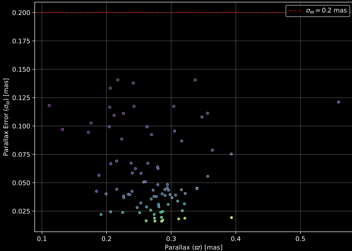
Gaia Cluster: [FSR_1211] Parallax Quality (n= 89)
