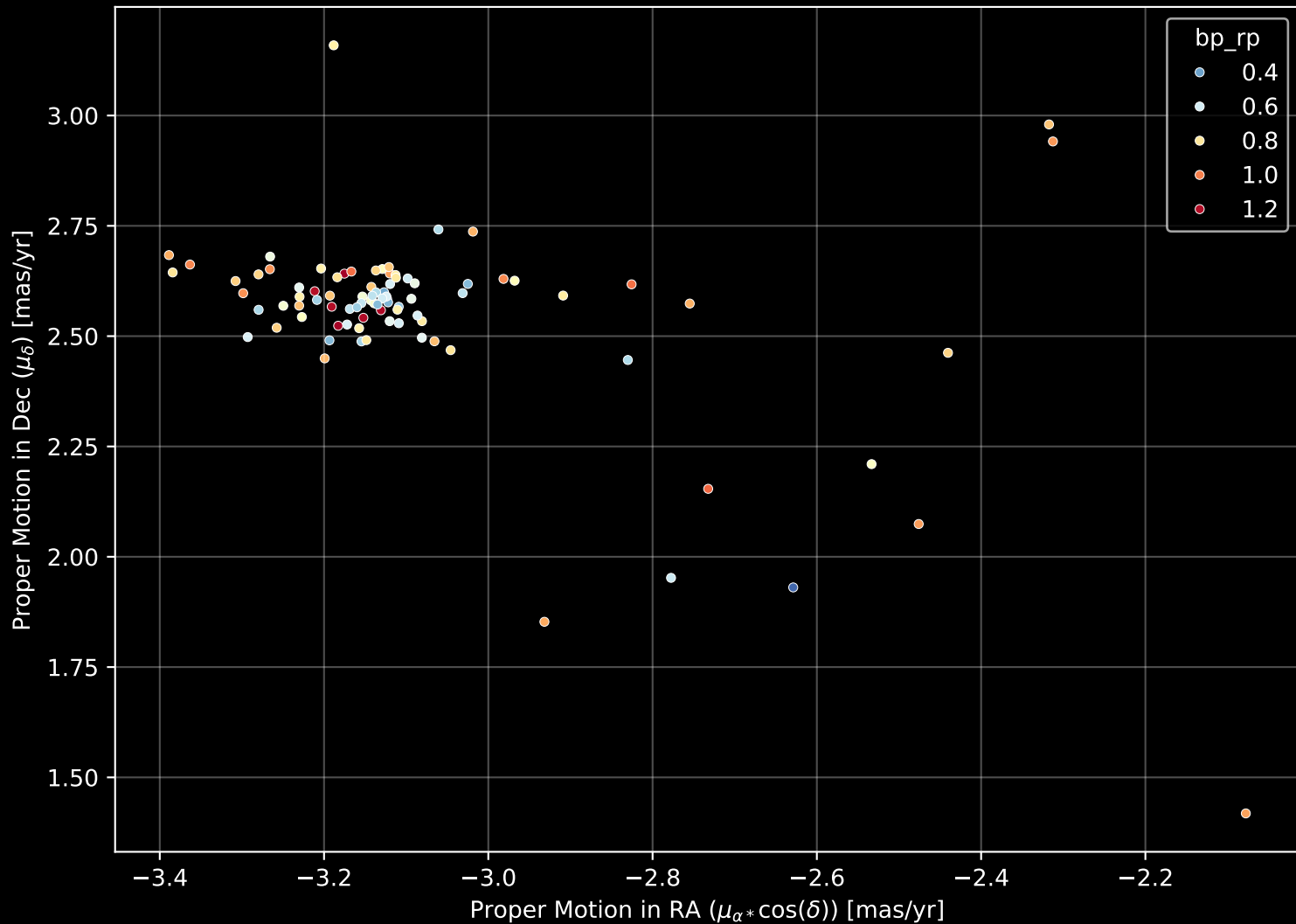
Gaia Cluster: [FSR_1211] Proper Motion Diagram (n= 89)
