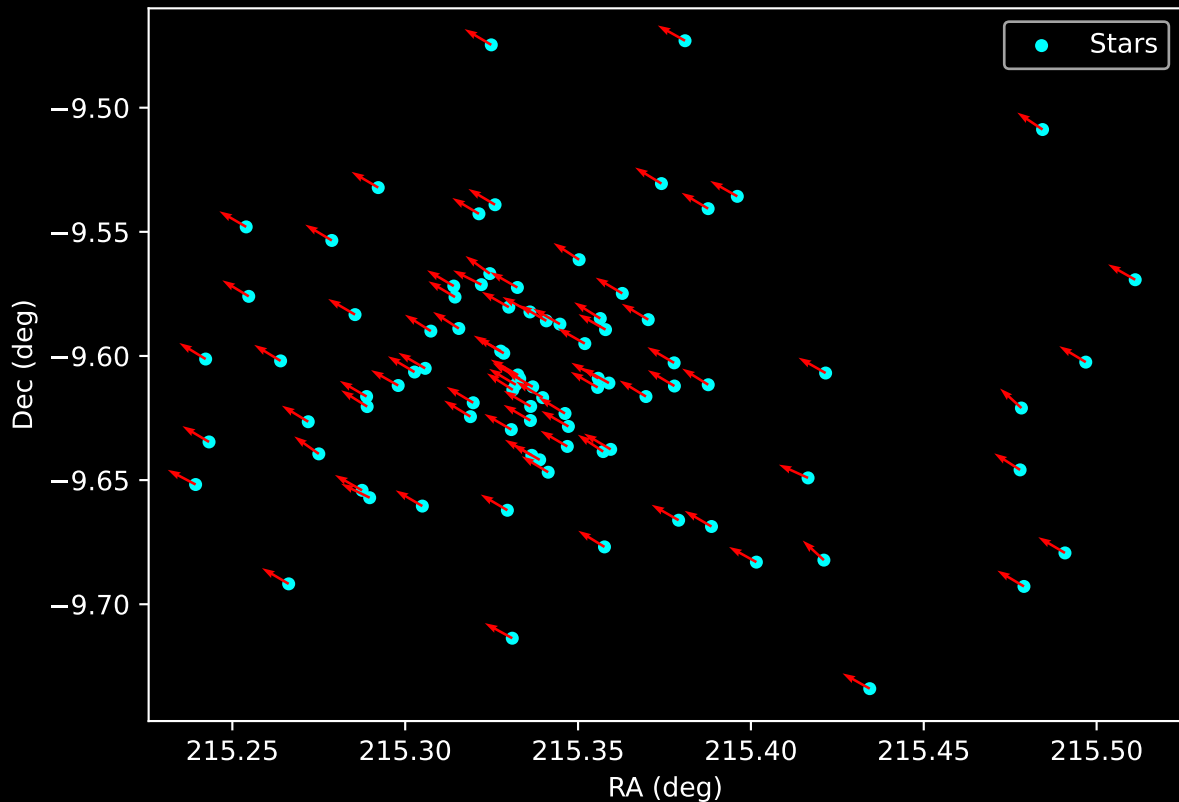
Gaia Cluster: [FSR_1211] Proper Motion Vectors for Gaia Star Field (n= 89)
