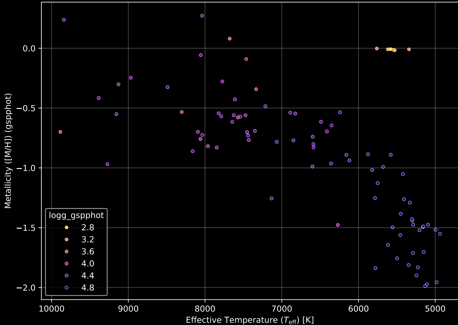
Gaia Cluster: [FSR_1211] Stellar Population Parameters (n= 89)
