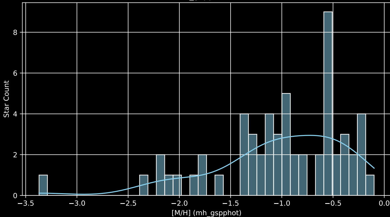
Gaia Cluster: [FSR_1260 [M/H] (mh_gspphot) (n= 58)
