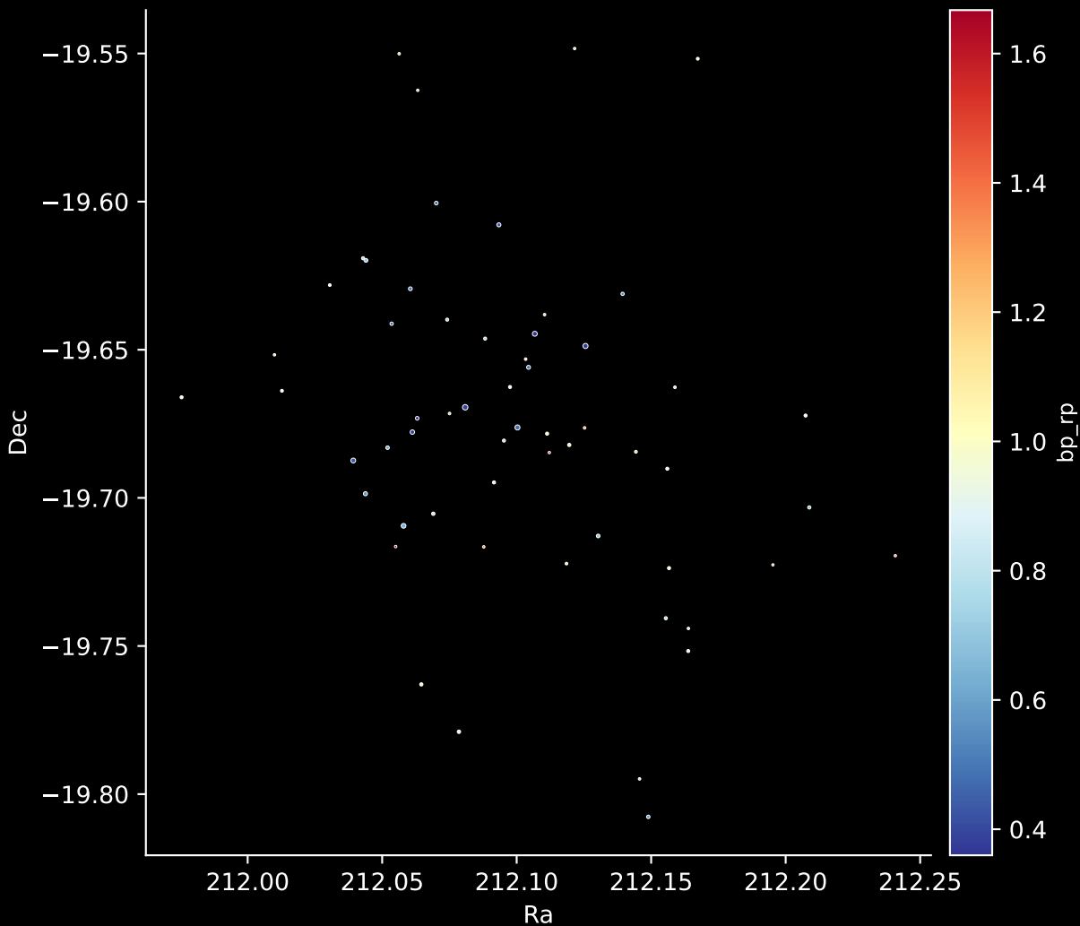
Gaia Cluster: [FSR_1260] Stars: 58
