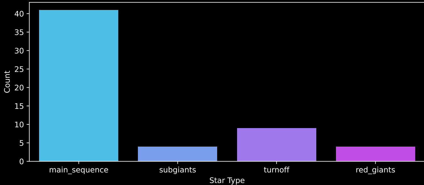
Gaia Cluster: [FSR_1260] Count plot of Star Type
