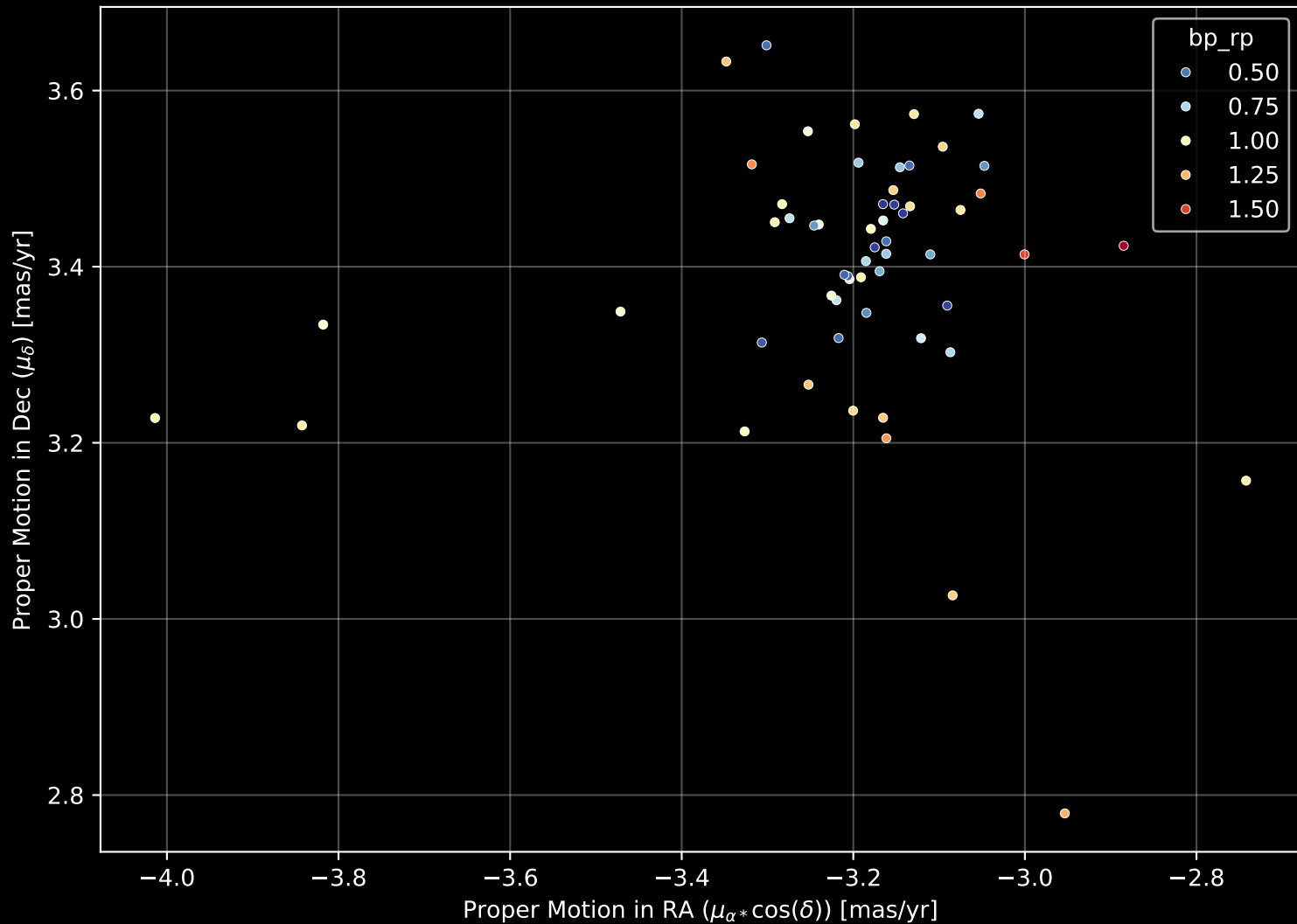
Gaia Cluster: [FSR_1260] Proper Motion Diagram (n= 58)
