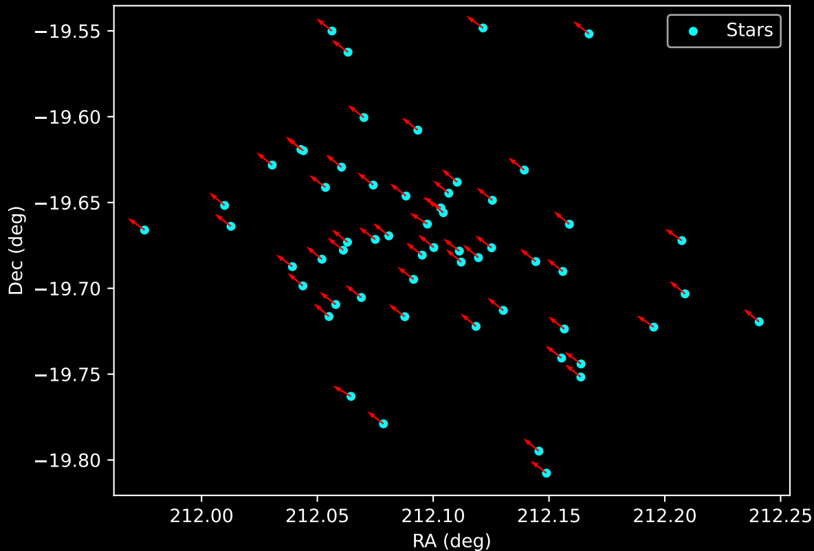
Gaia Cluster: [FSR_1260] Proper Motion Vectors for Gaia Star Field (n= 58)
