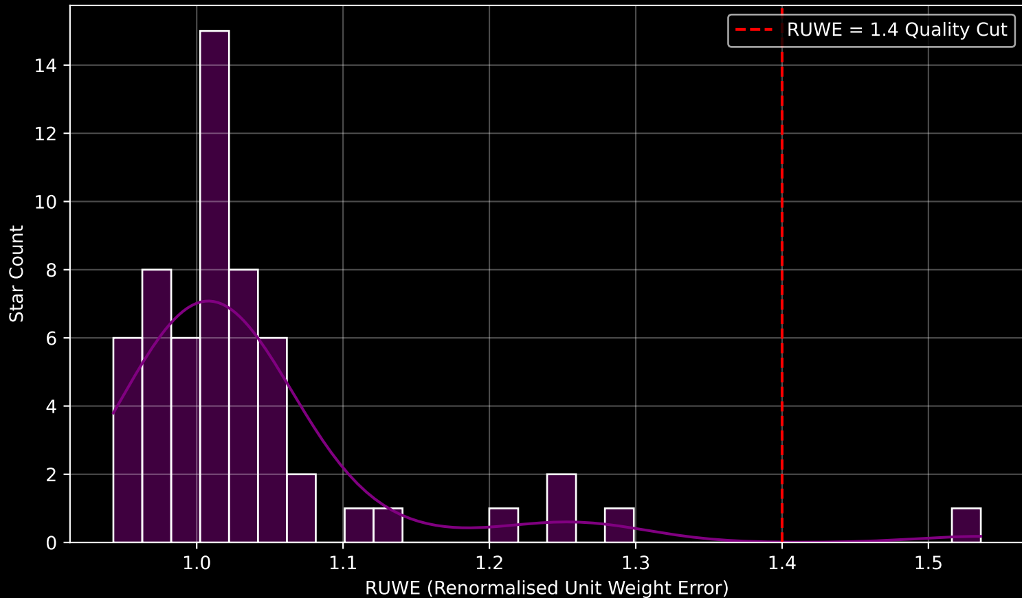
Gaia Cluster: [FSR_1260] RUWE Distribution (n= 58)
