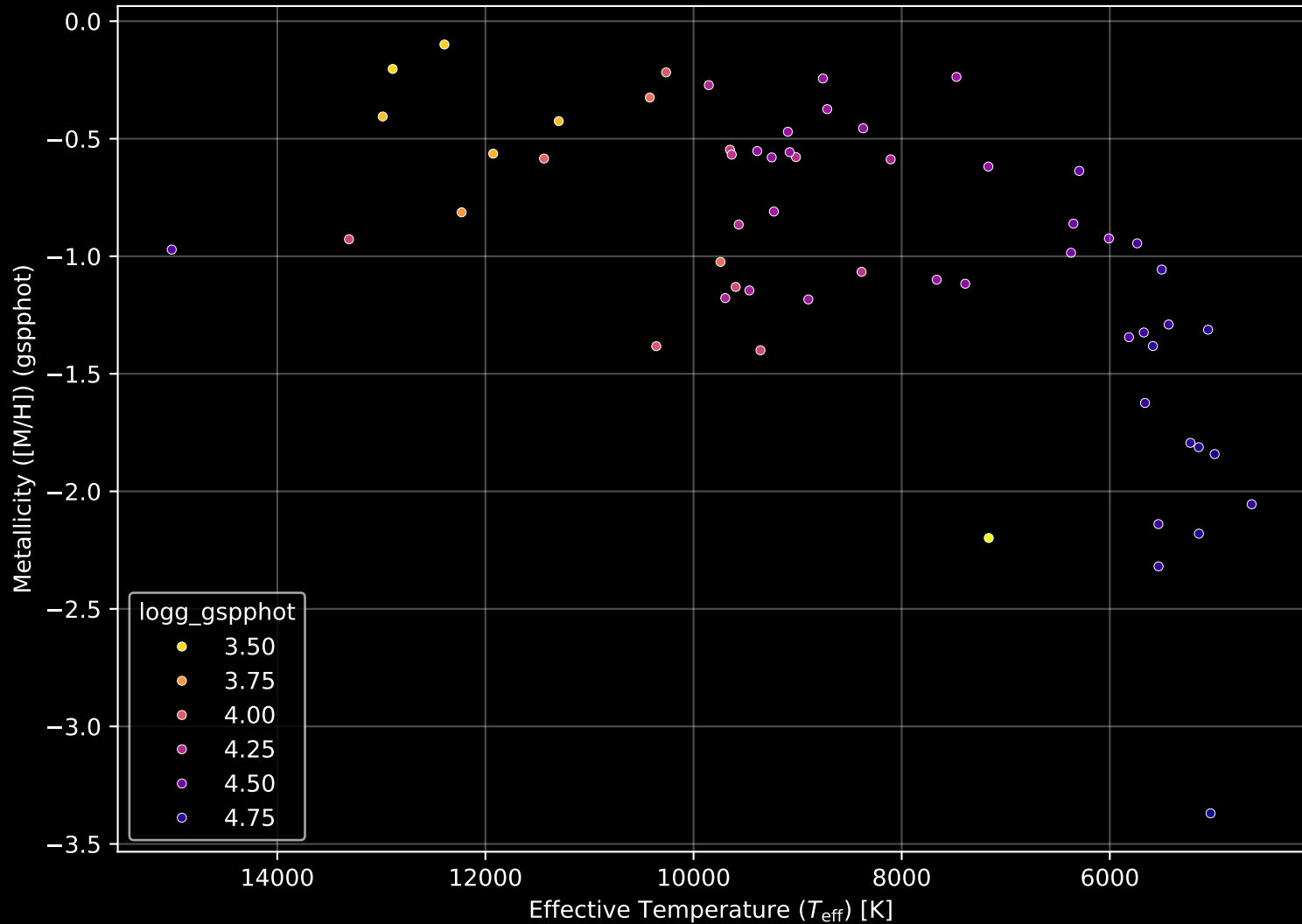
Gaia Cluster: [FSR_1260] Stellar Population Parameters (n= 58)
