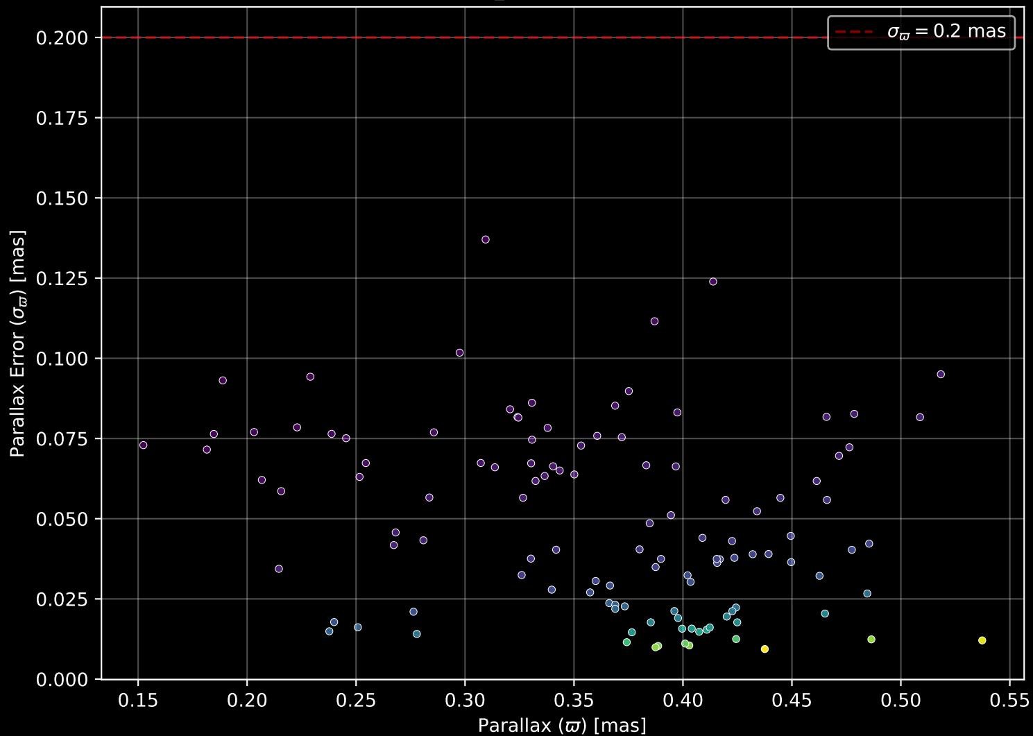
Gaia Cluster: [FSR_1360] Parallax Quality (n= 117)
