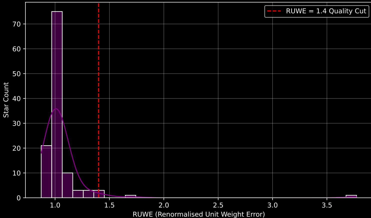
Gaia Cluster: [FSR_1360] RUWE Distribution (n= 117)
