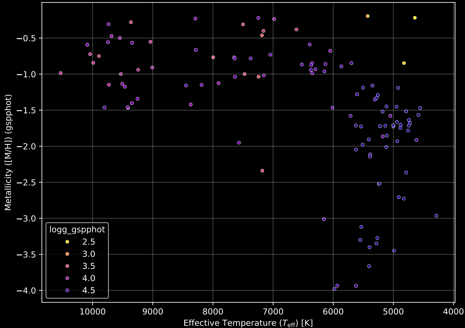
Gaia Cluster: [FSR_1360] Stellar Population Parameters (n= 117)
