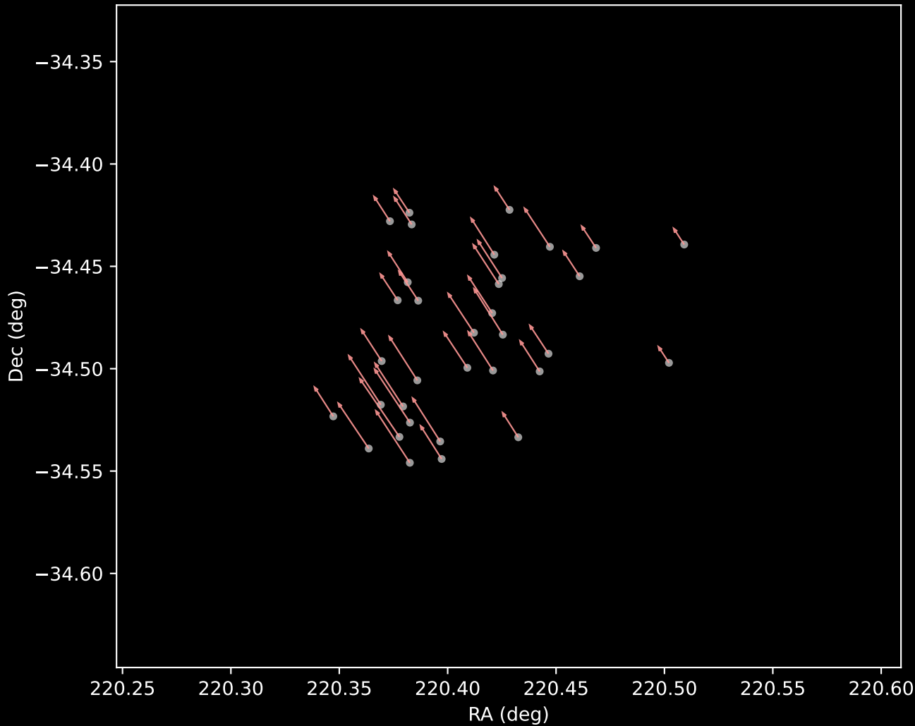
Gaia DR3 Cluster 7 Proper Motion Vectors (n=34)
