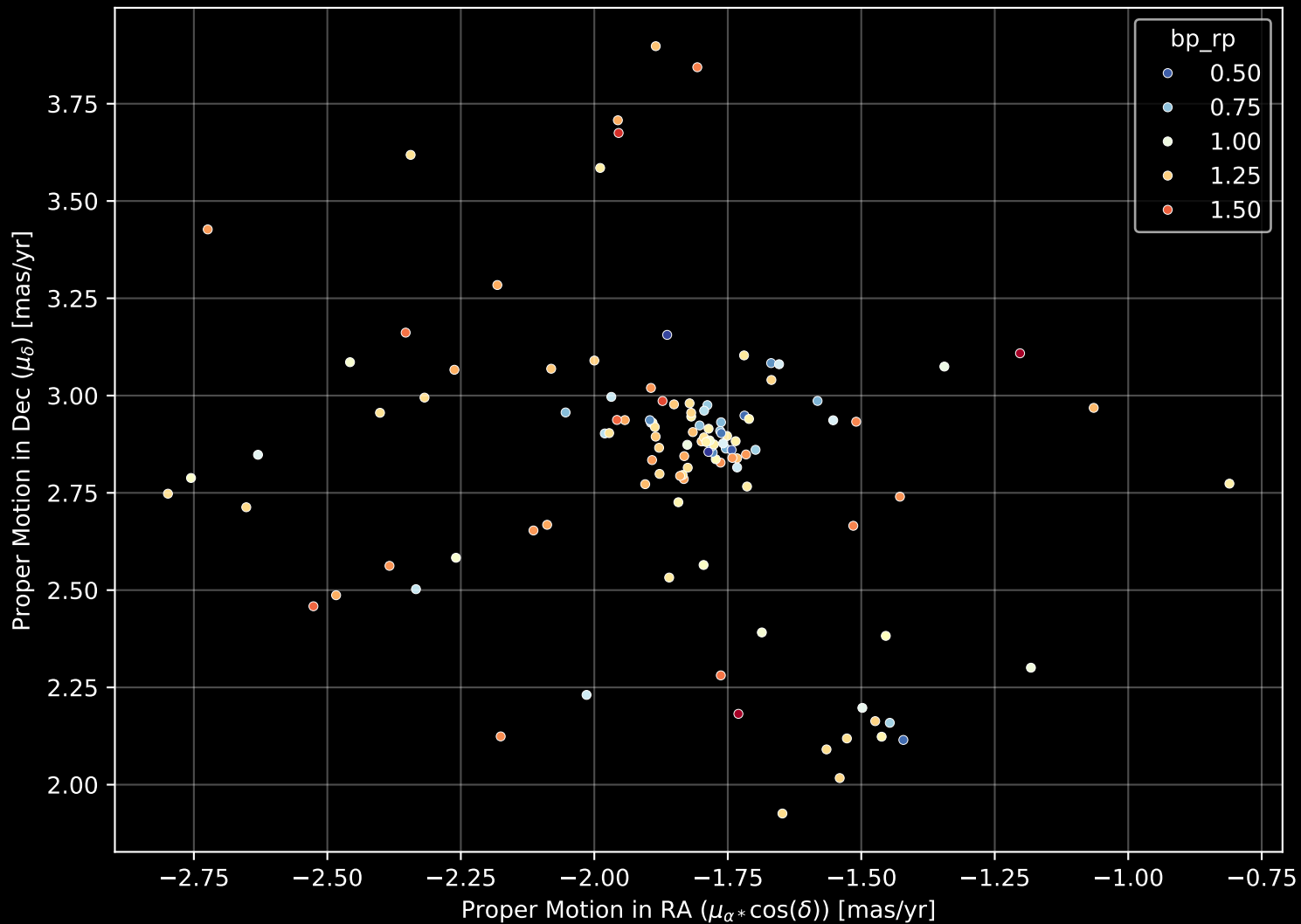
Gaia Cluster: [FSR_1360] Proper Motion Diagram (n= 117)
