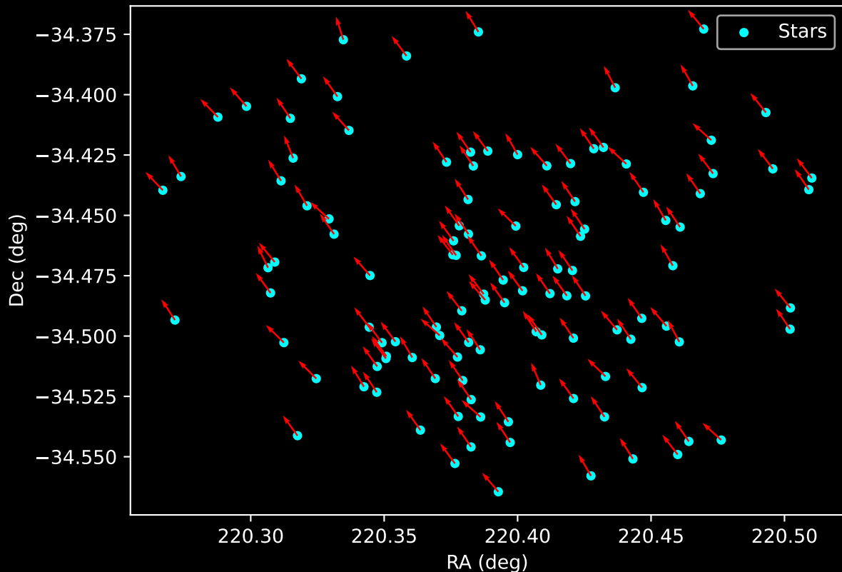
Gaia Cluster: [FSR_1360] Proper Motion Vectors for Gaia Star Field (n= 117)
