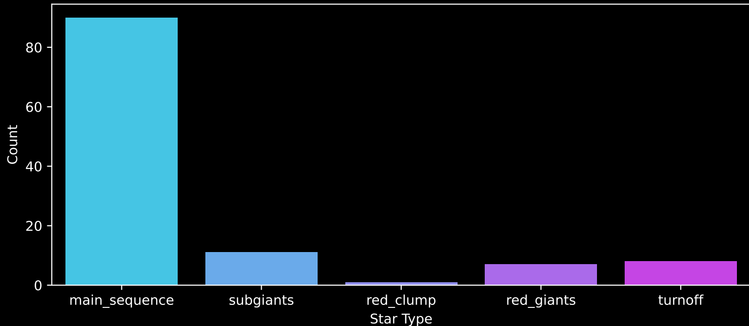
Gaia Cluster: [FSR_1360] Count plot of Star Type
