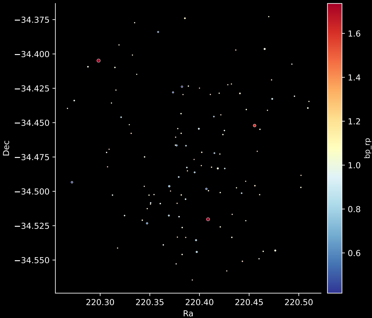
Gaia Cluster: [FSR_1360] Stars: 117
