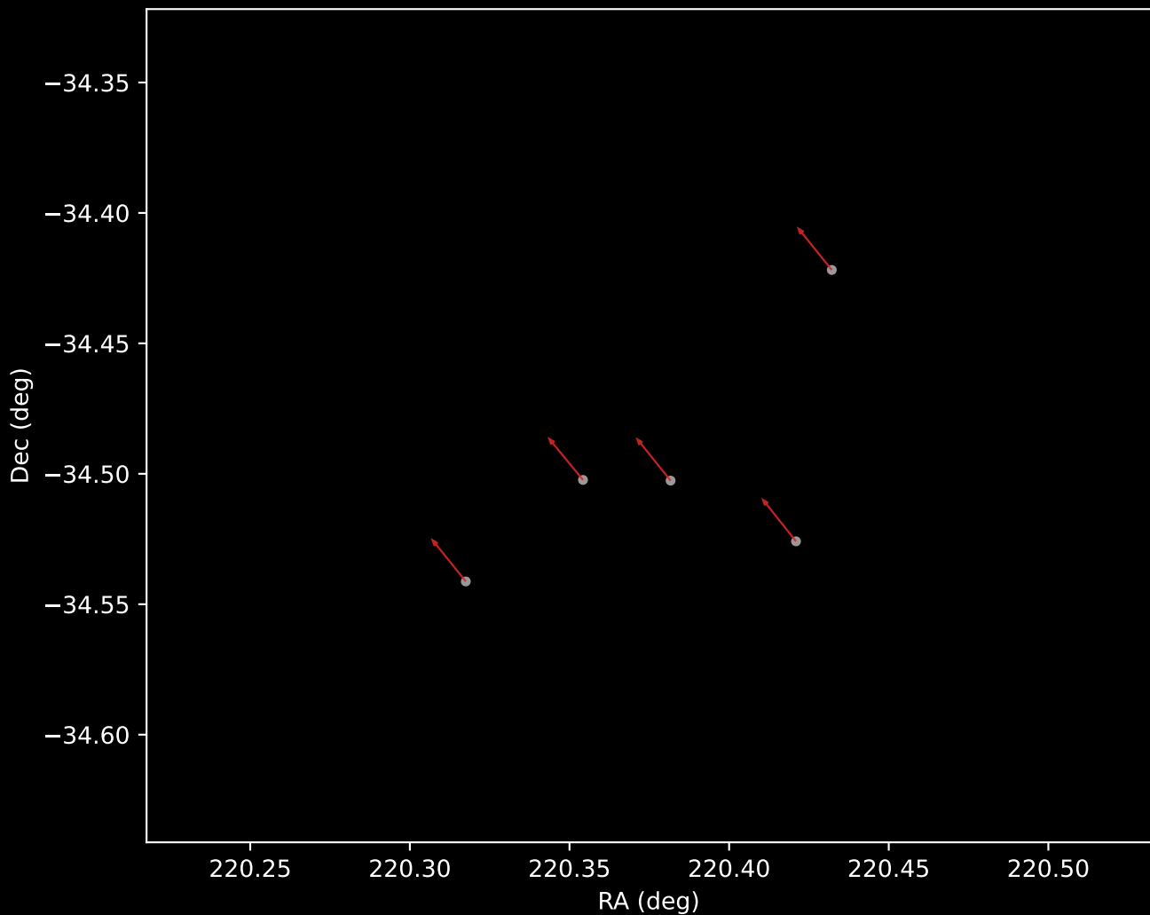
Gaia DR3 Cluster 6 Proper Motion Vectors (n=5)
