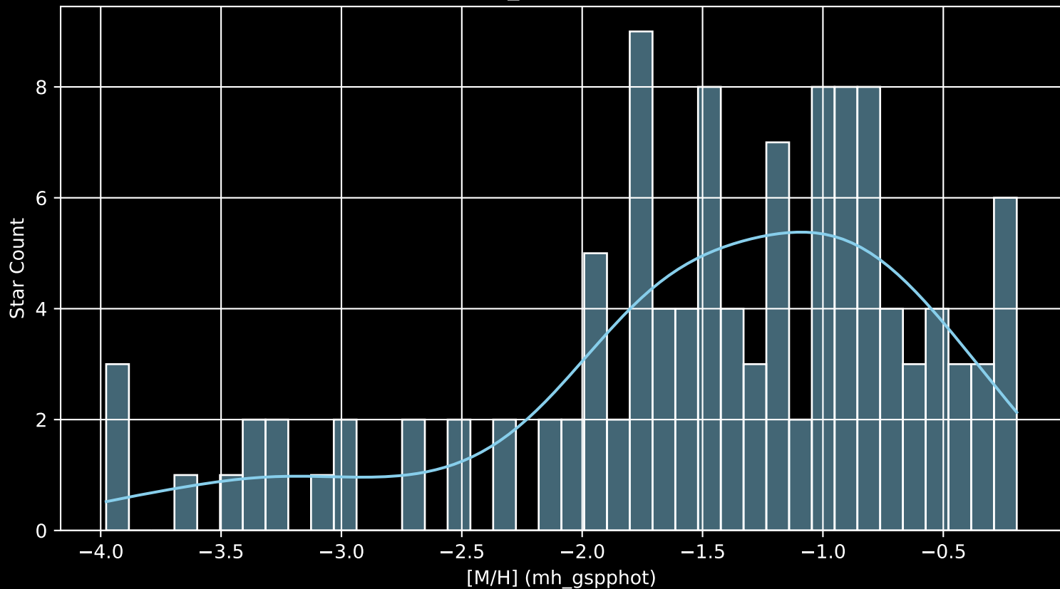
Gaia Cluster: [FSR_1360 [M/H] (mh_gspphot) (n= 117)
