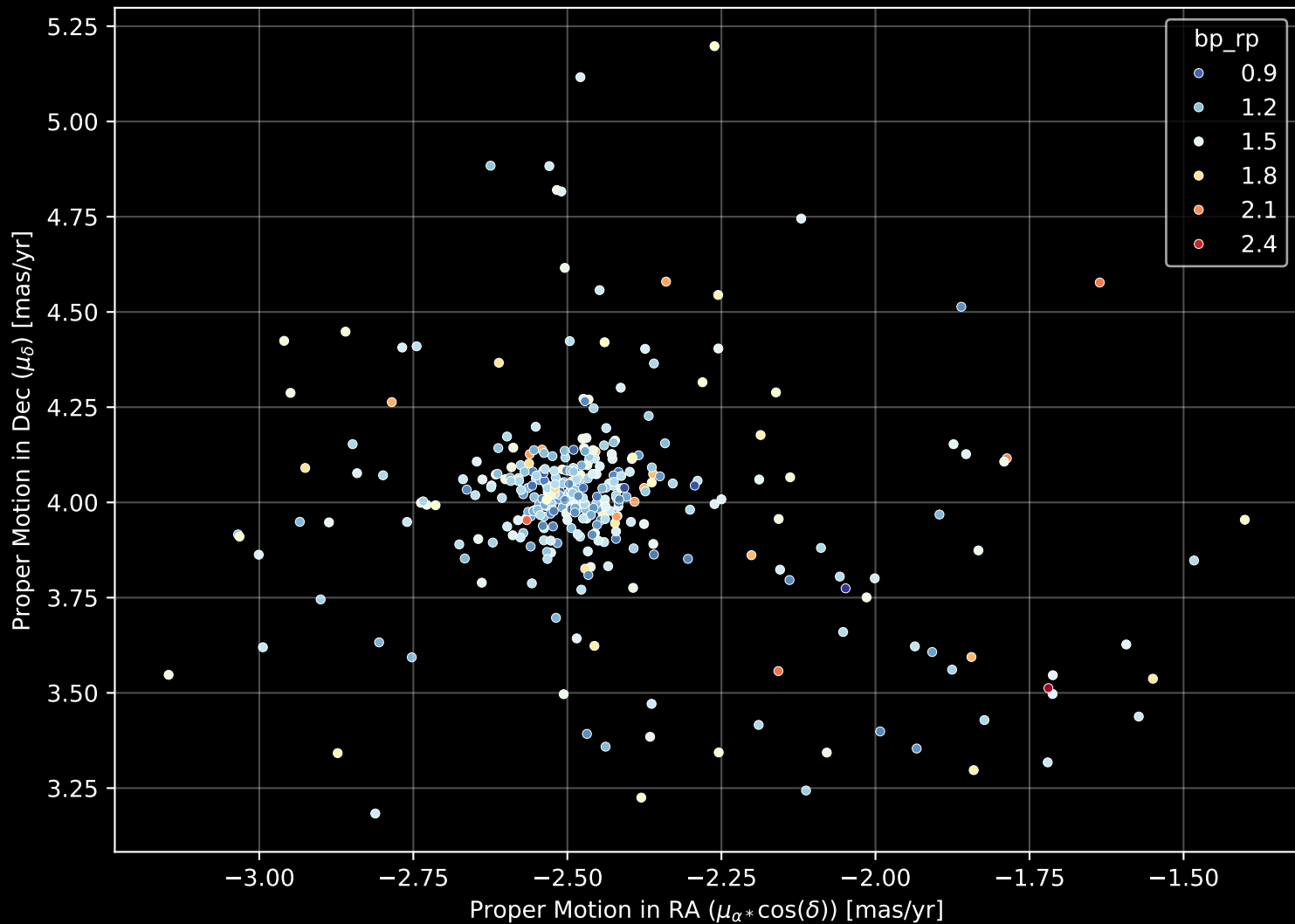
Gaia Cluster: [FSR_1361] Proper Motion Diagram (n= 361)
