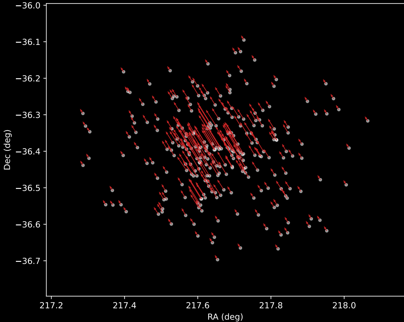
Gaia DR3 Cluster 6 Proper Motion Vectors (n=256)
