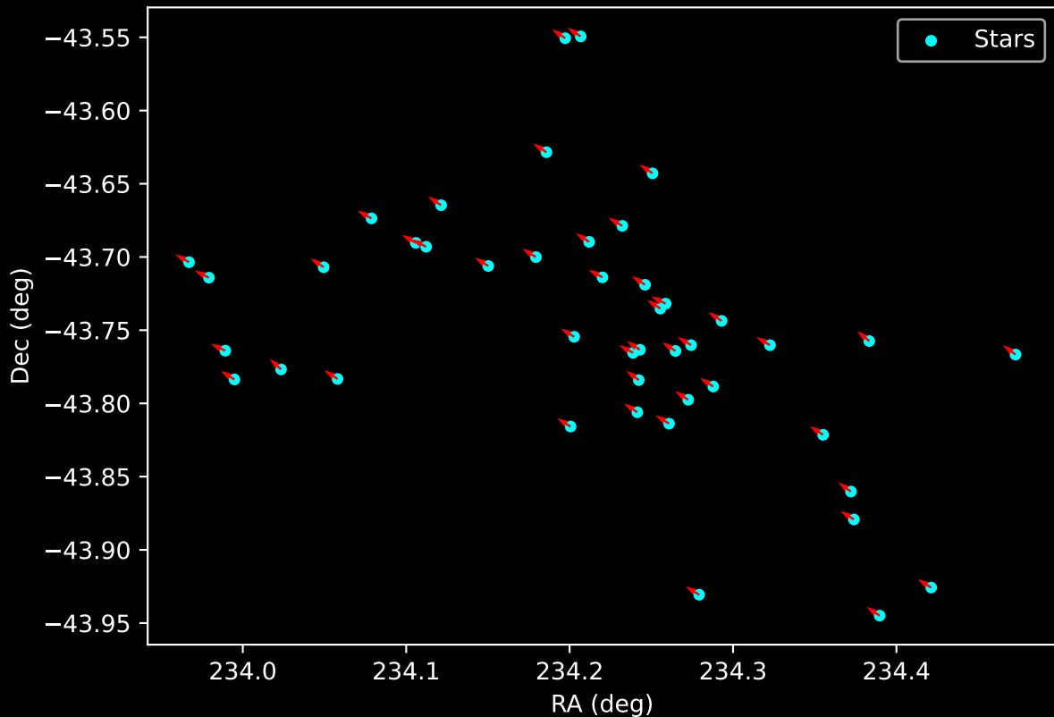
Gaia Cluster: [FSR_1435] Proper Motion Vectors for Gaia Star Field (n= 44)
