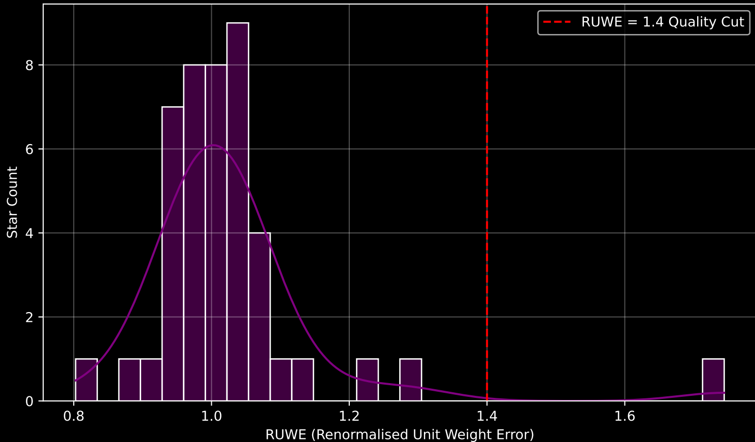
Gaia Cluster: [FSR_1435] RUWE Distribution (n= 44)
