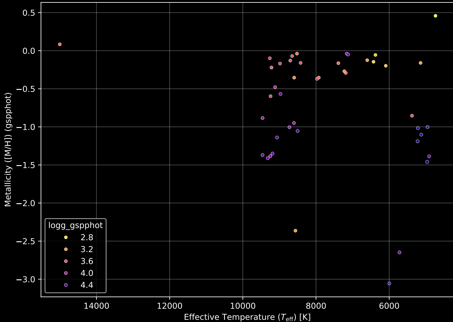
Gaia Cluster: [FSR_1435] Stellar Population Parameters (n= 44)
