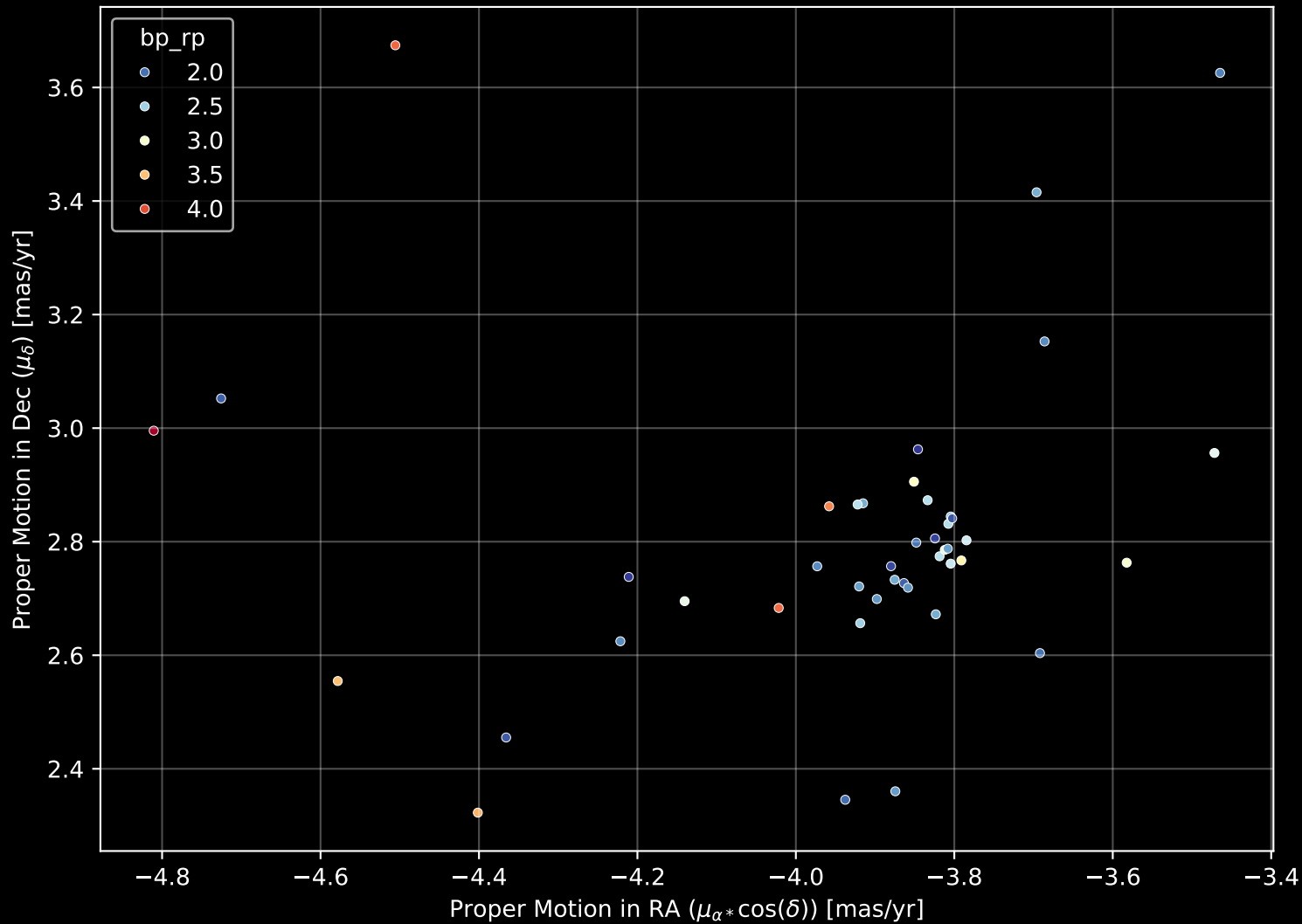
Gaia Cluster: [FSR_1435] Proper Motion Diagram (n= 44)
