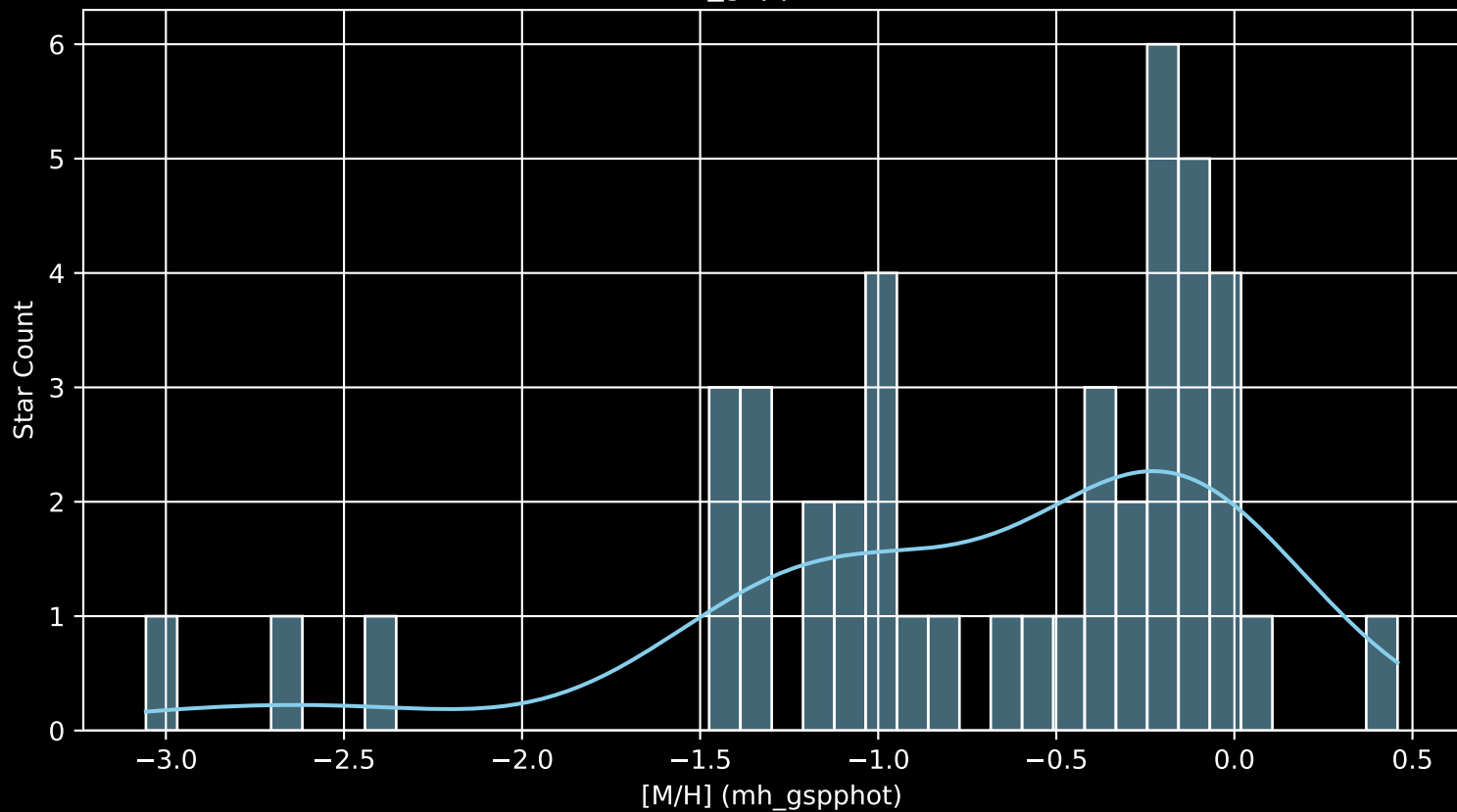
Gaia Cluster: [FSR_1435 [M/H] (mh_gspphot) (n= 44)
