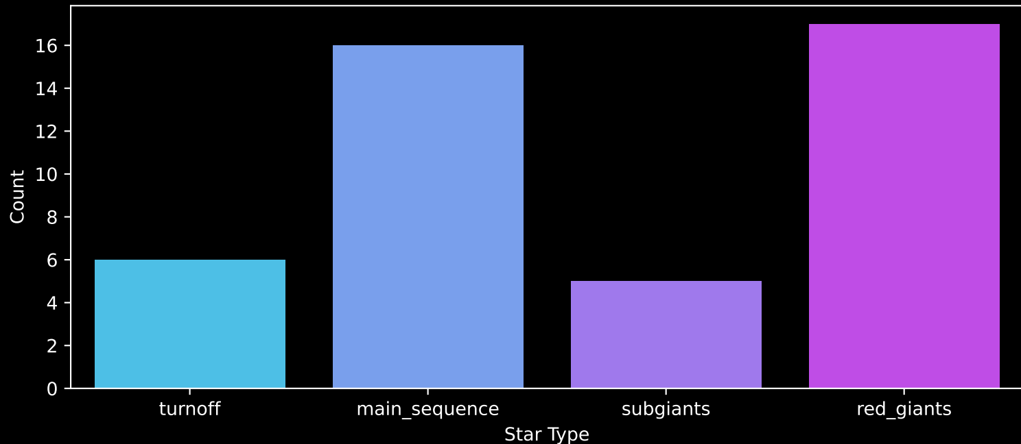
Gaia Cluster: [FSR_1435] Count plot of Star Type
