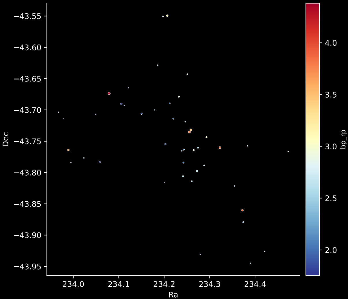
Gaia Cluster: [FSR_1435] Stars: 44
