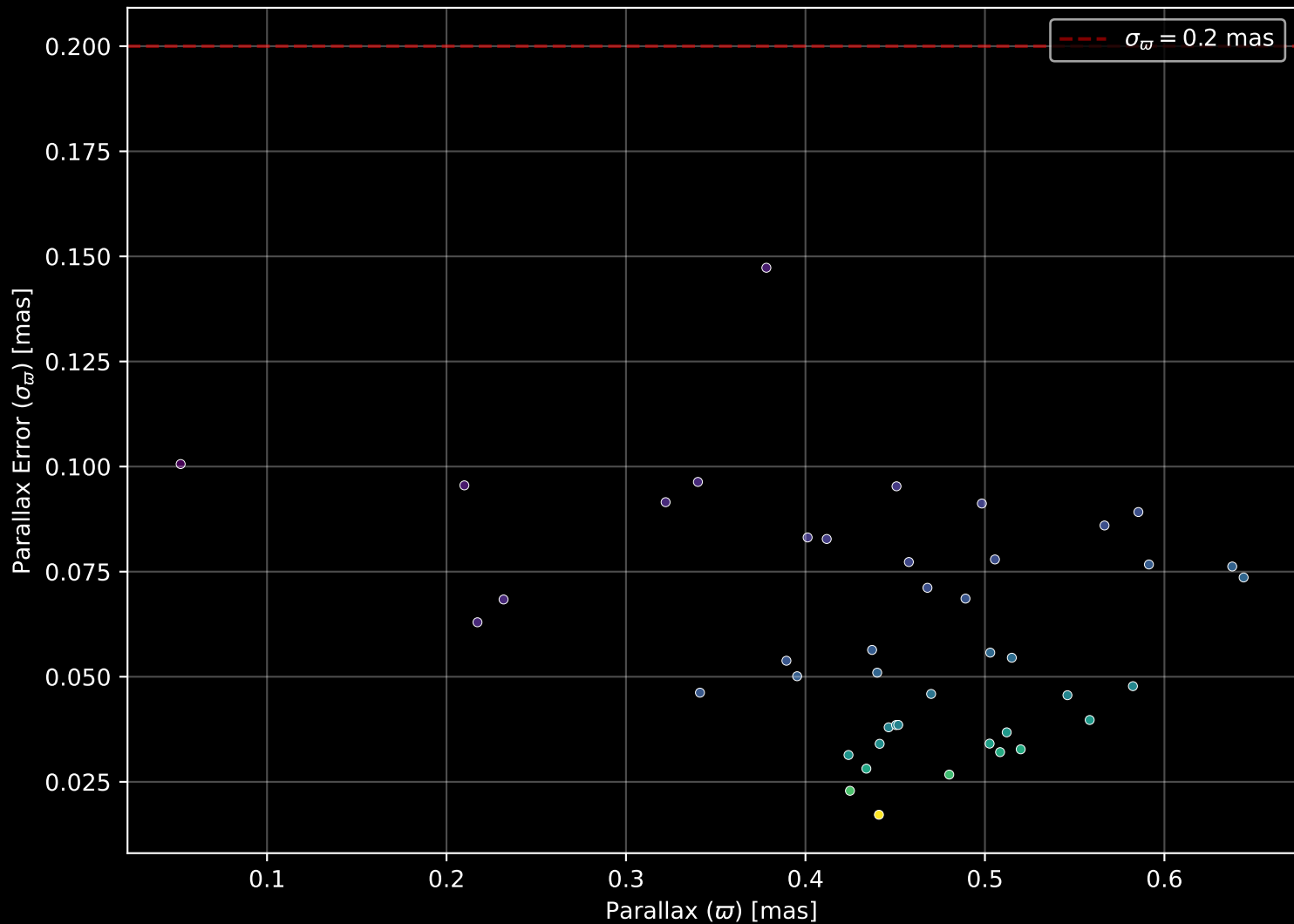
Gaia Cluster: [FSR_1435] Parallax Quality (n= 44)
