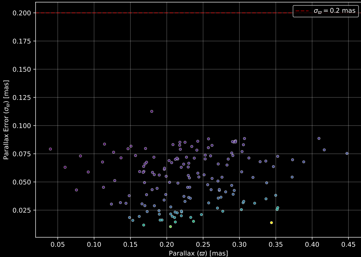
Gaia Cluster: [FSR_1441] Parallax Quality (n= 155)
