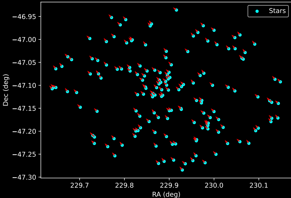
Gaia Cluster: [FSR_1441] Proper Motion Vectors for Gaia Star Field (n= 155)
