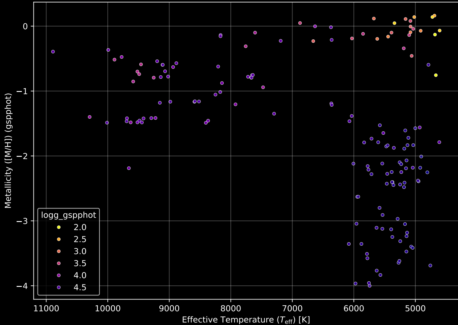
Gaia Cluster: [FSR_1441] Stellar Population Parameters (n= 155)
