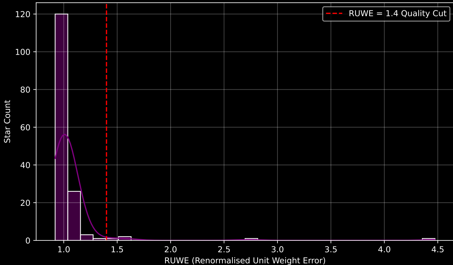
Gaia Cluster: [FSR_1441] RUWE Distribution (n= 155)
