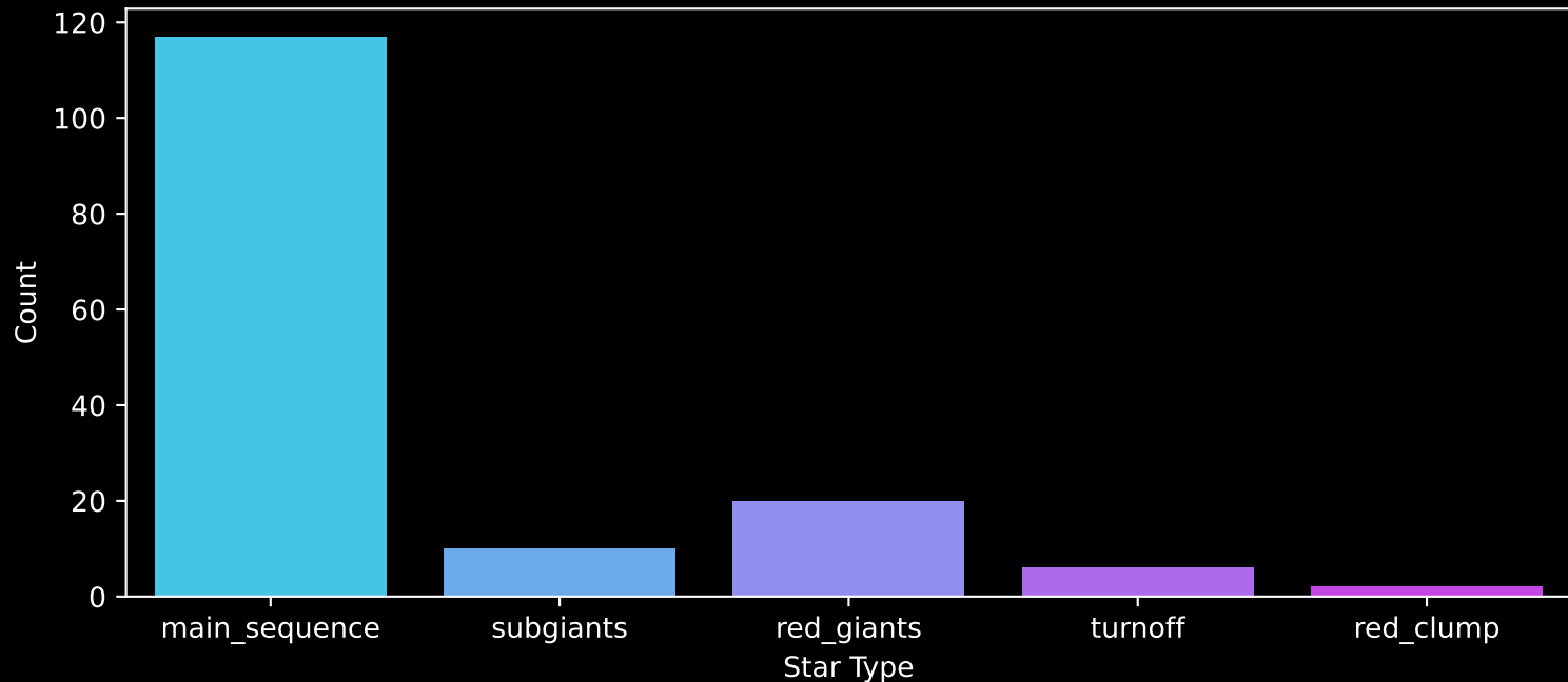
Gaia Cluster: [FSR_1441] Count plot of Star Type
