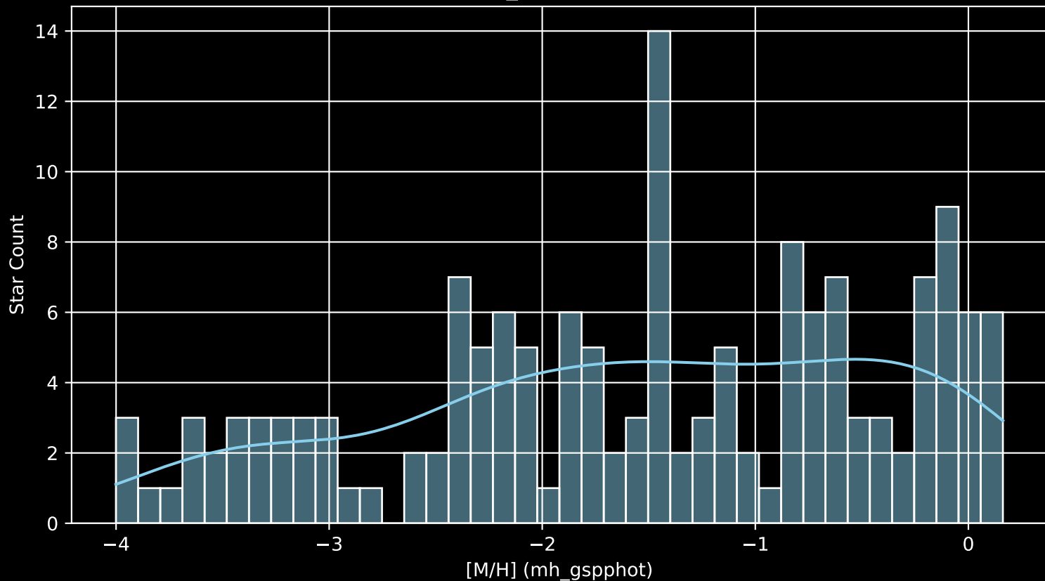
Gaia Cluster: [FSR_1441 [M/H] (mh_gspphot) (n= 155)
