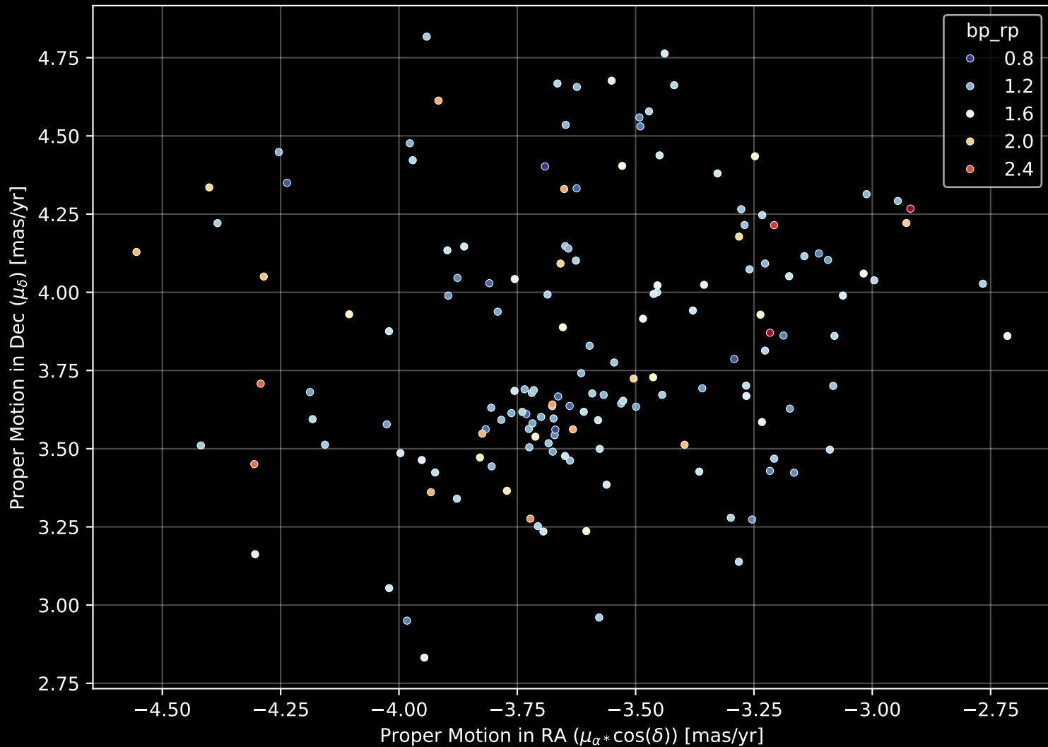
Gaia Cluster: [FSR_1441] Proper Motion Diagram (n= 155)
