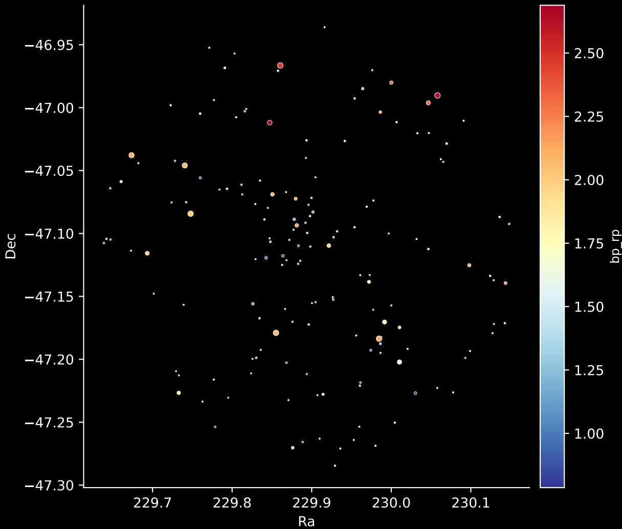
Gaia Cluster: [FSR_1441] Stars: 155
