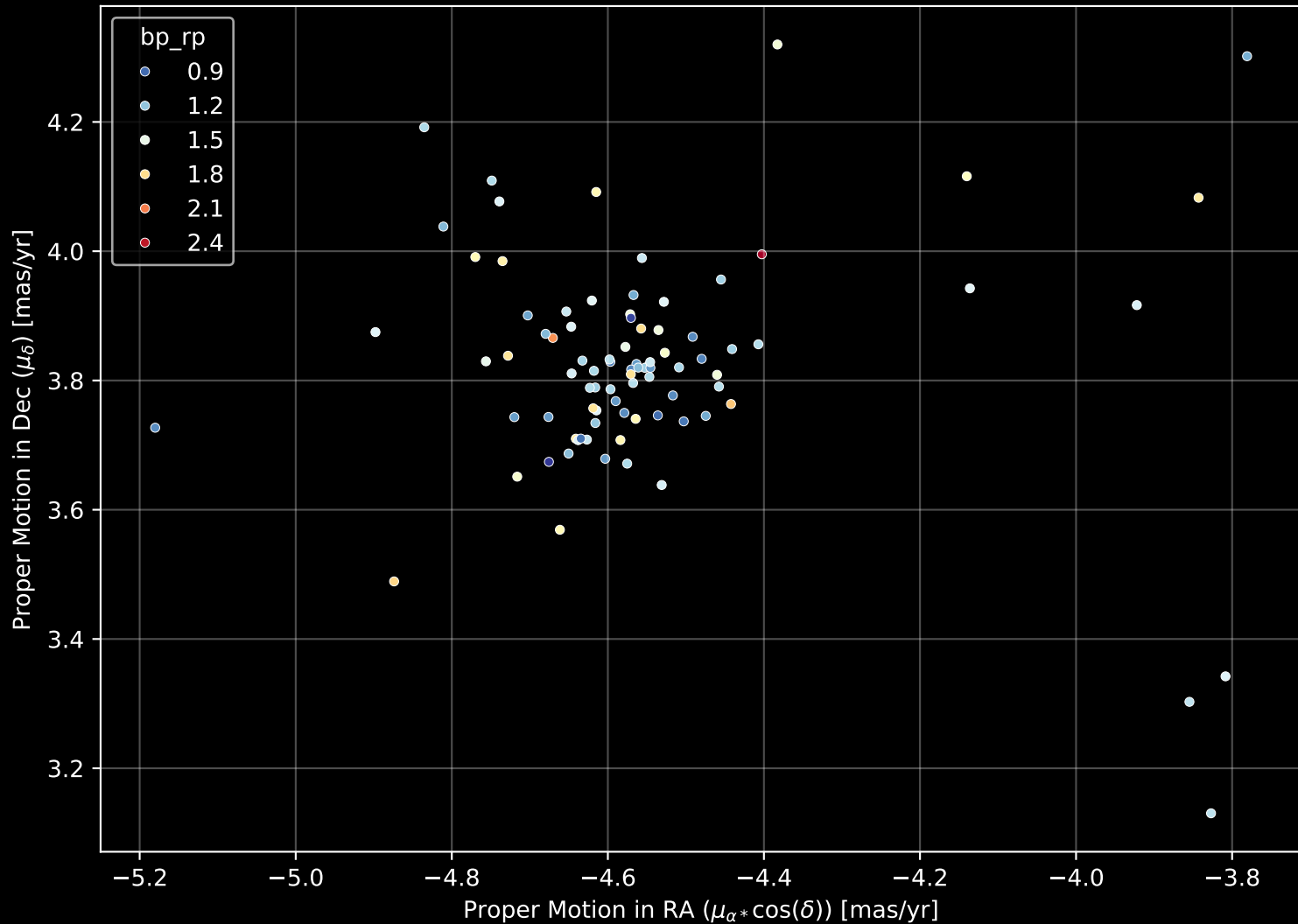
Gaia Cluster: [FSR_1452] Proper Motion Diagram (n= 88)
