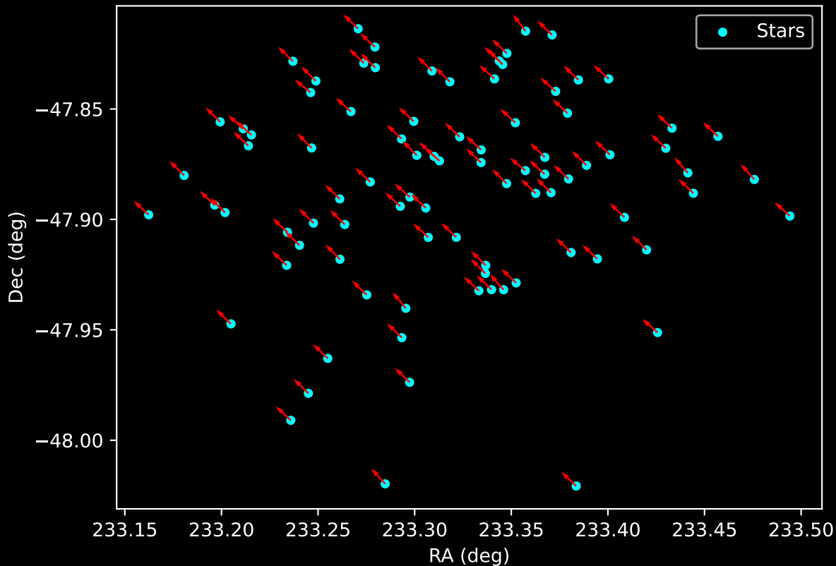
Gaia Cluster: [FSR_1452] Proper Motion Vectors for Gaia Star Field (n= 88)
