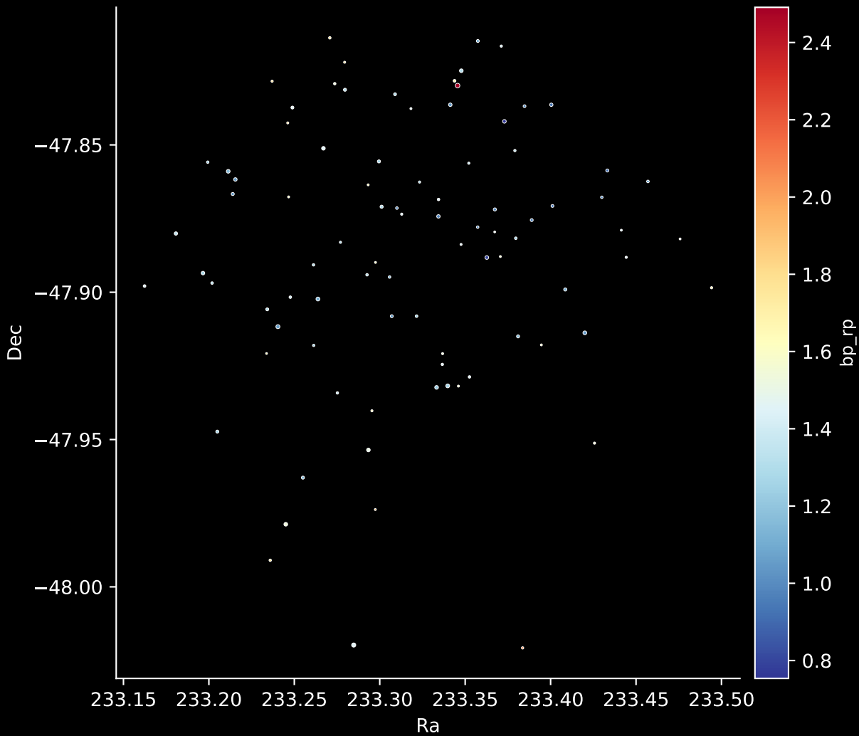
Gaia Cluster: [FSR_1452] Stars: 88
