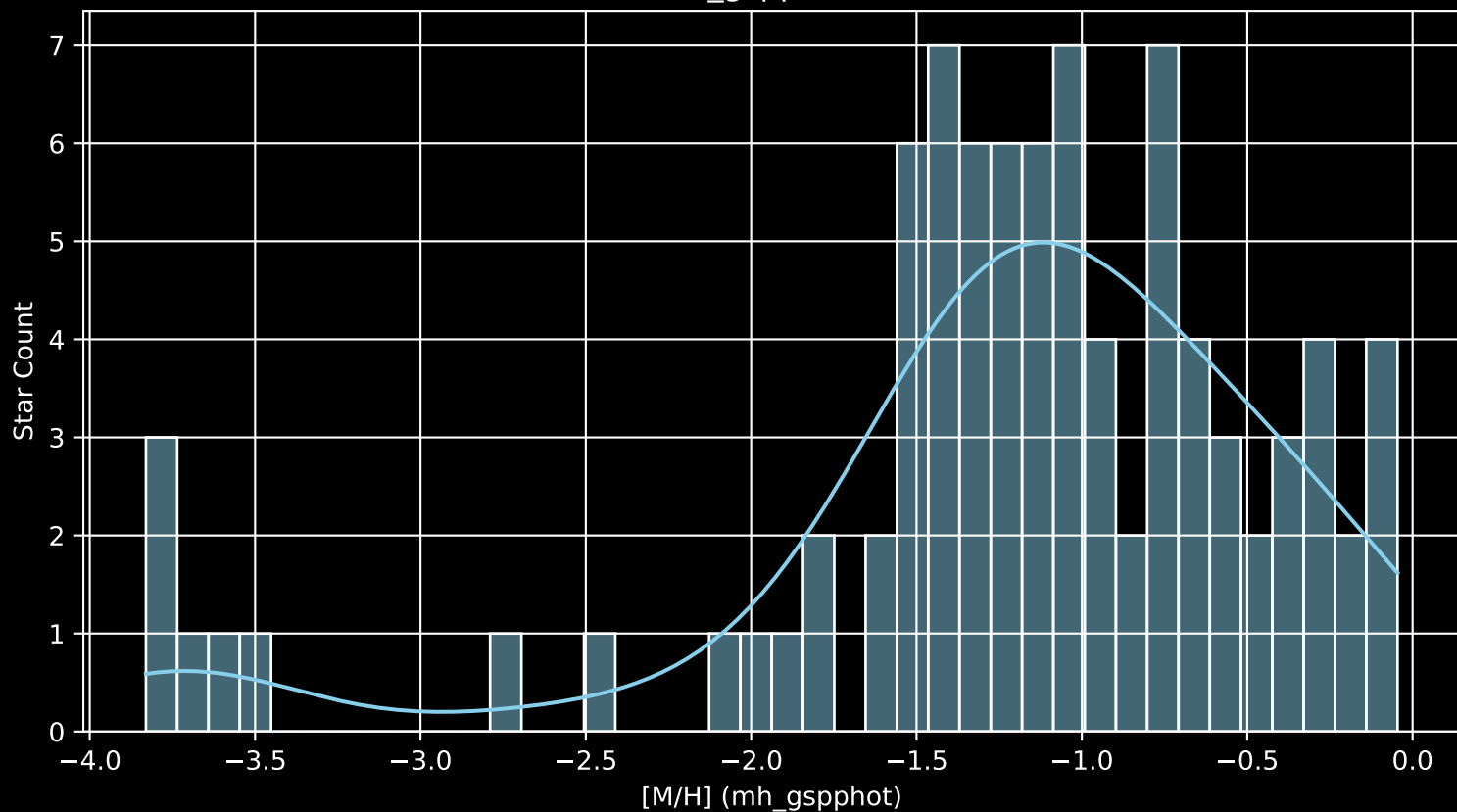
Gaia Cluster: [FSR_1452 [M/H] (mh_gspphot) (n= 88)
