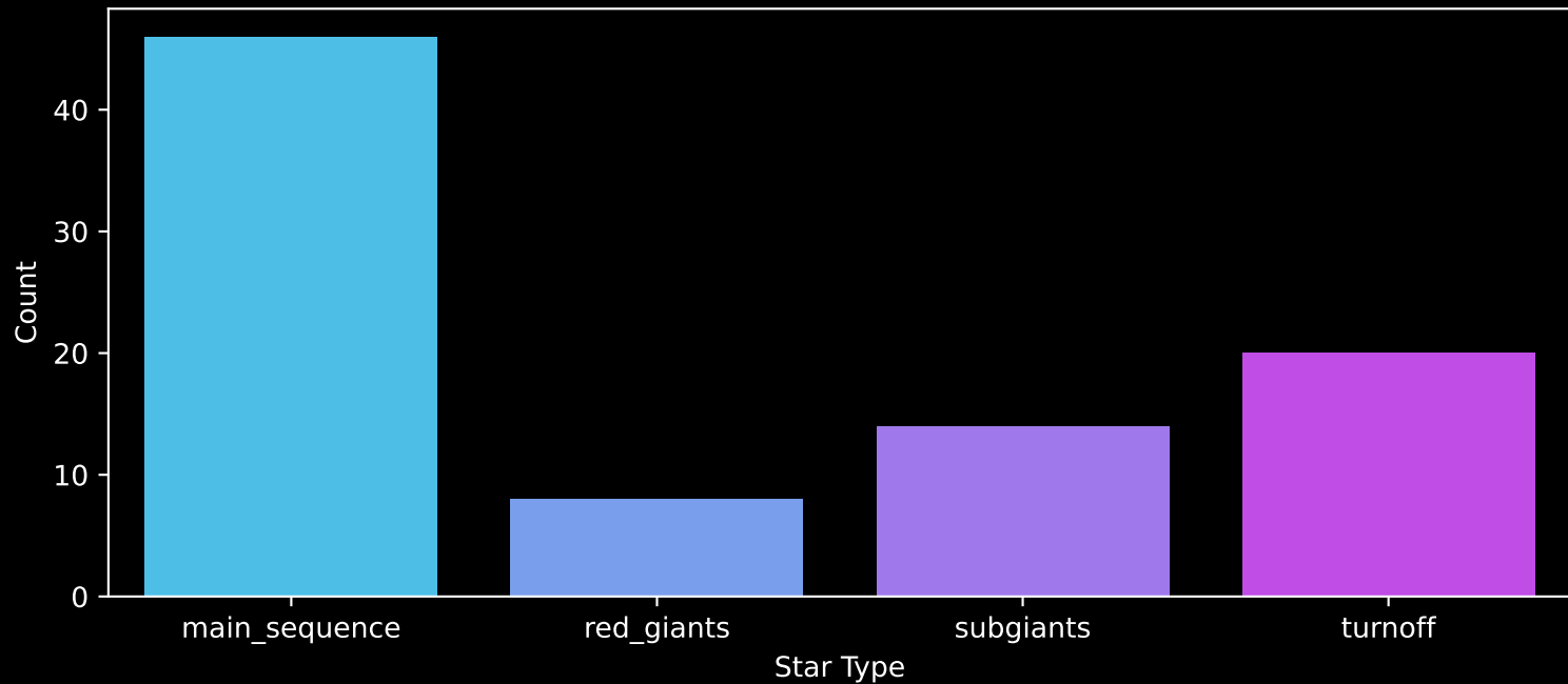
Gaia Cluster: [FSR_1452] Count plot of Star Type
