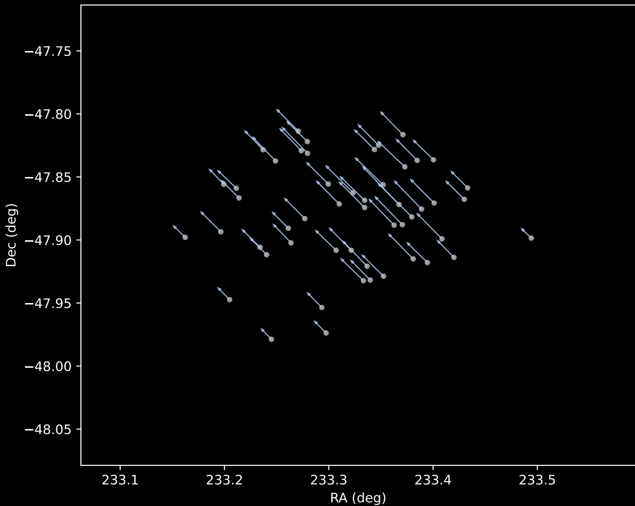
Gaia DR3 Cluster 1 Proper Motion Vectors (n=51)
