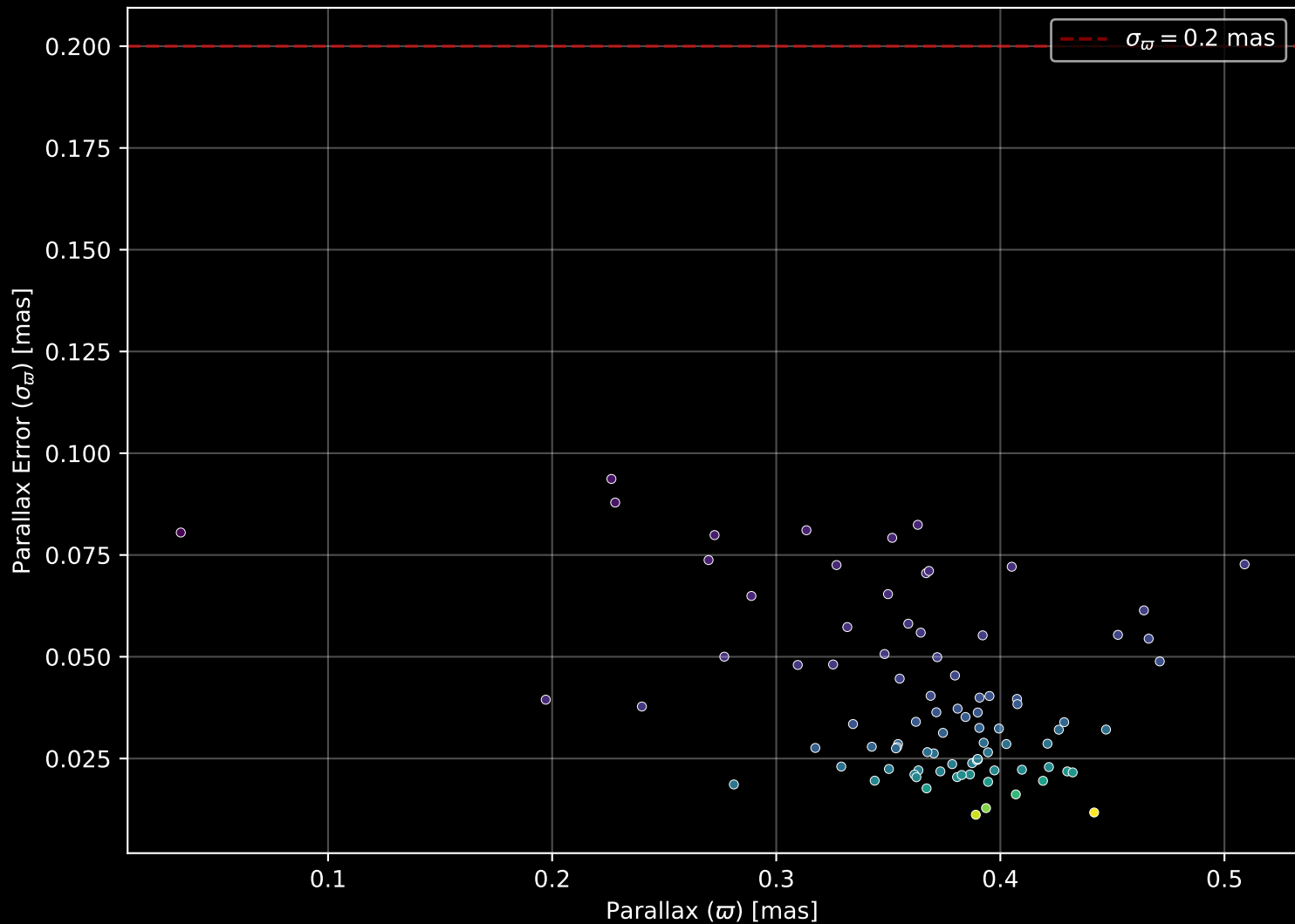
Gaia Cluster: [FSR_1452] Parallax Quality (n= 88)
