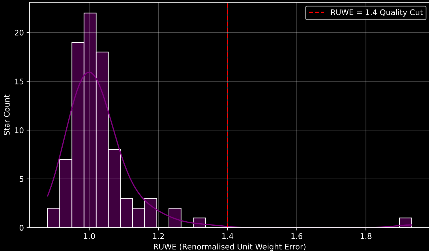
Gaia Cluster: [FSR_1452] RUWE Distribution (n= 88)
