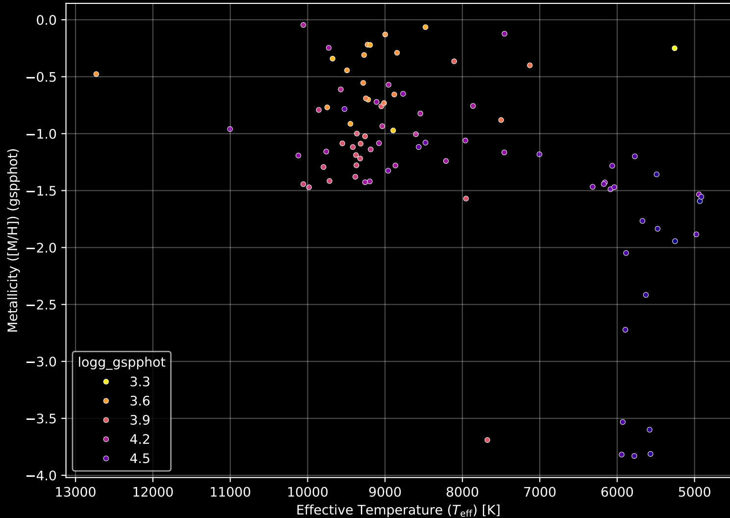
Gaia Cluster: [FSR_1452] Stellar Population Parameters (n= 88)
