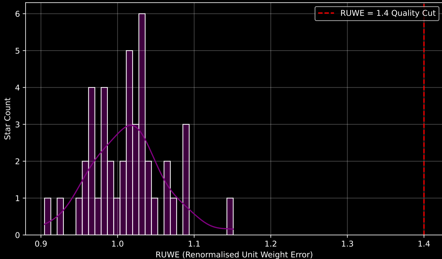
Gaia Cluster: [FSR_1484] RUWE Distribution (n= 43)
