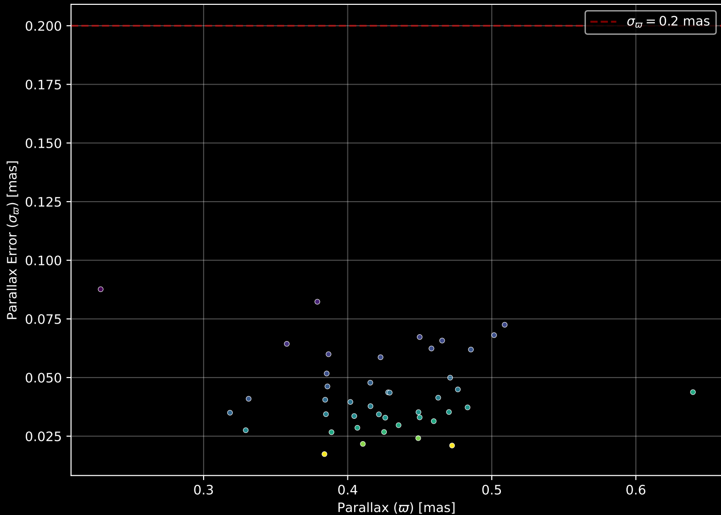
Gaia Cluster: [FSR_1484] Parallax Quality (n= 43)
