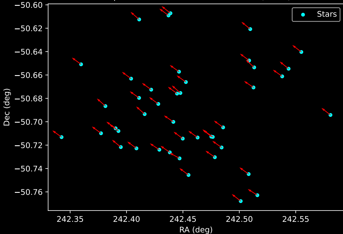
Gaia Cluster: [FSR_1484] Proper Motion Vectors for Gaia Star Field (n= 43)
