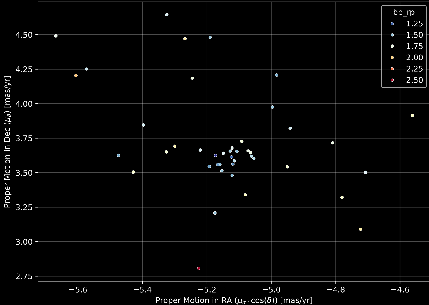
Gaia Cluster: [FSR_1484] Proper Motion Diagram (n= 43)
