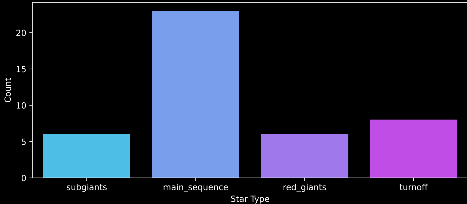
Gaia Cluster: [FSR_1484] Count plot of Star Type
