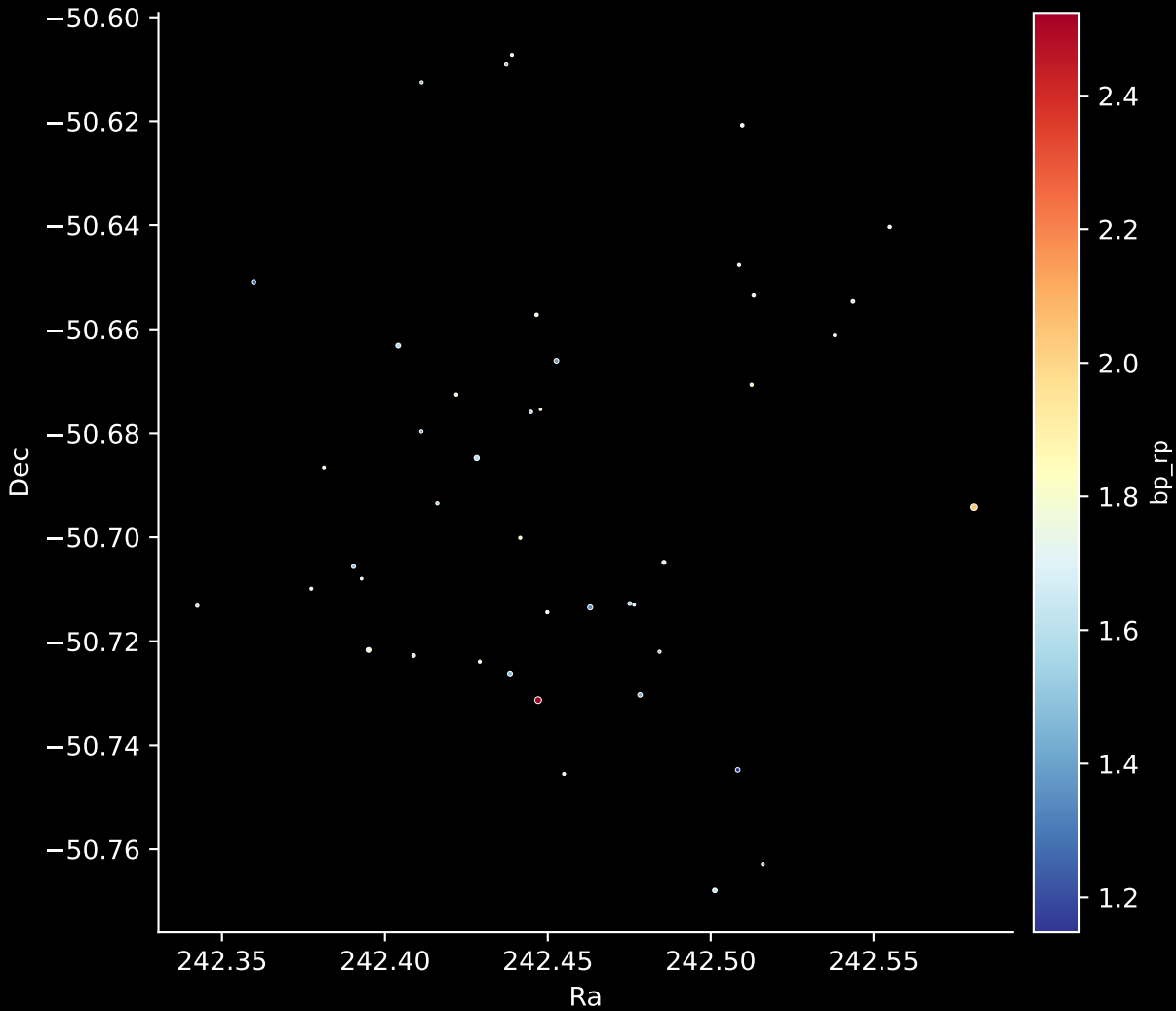
Gaia Cluster: [FSR_1484] Stars: 43
