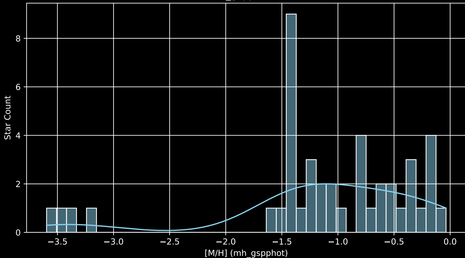
Gaia Cluster: [FSR_1484 [M/H] (mh_gspphot) (n= 43)
