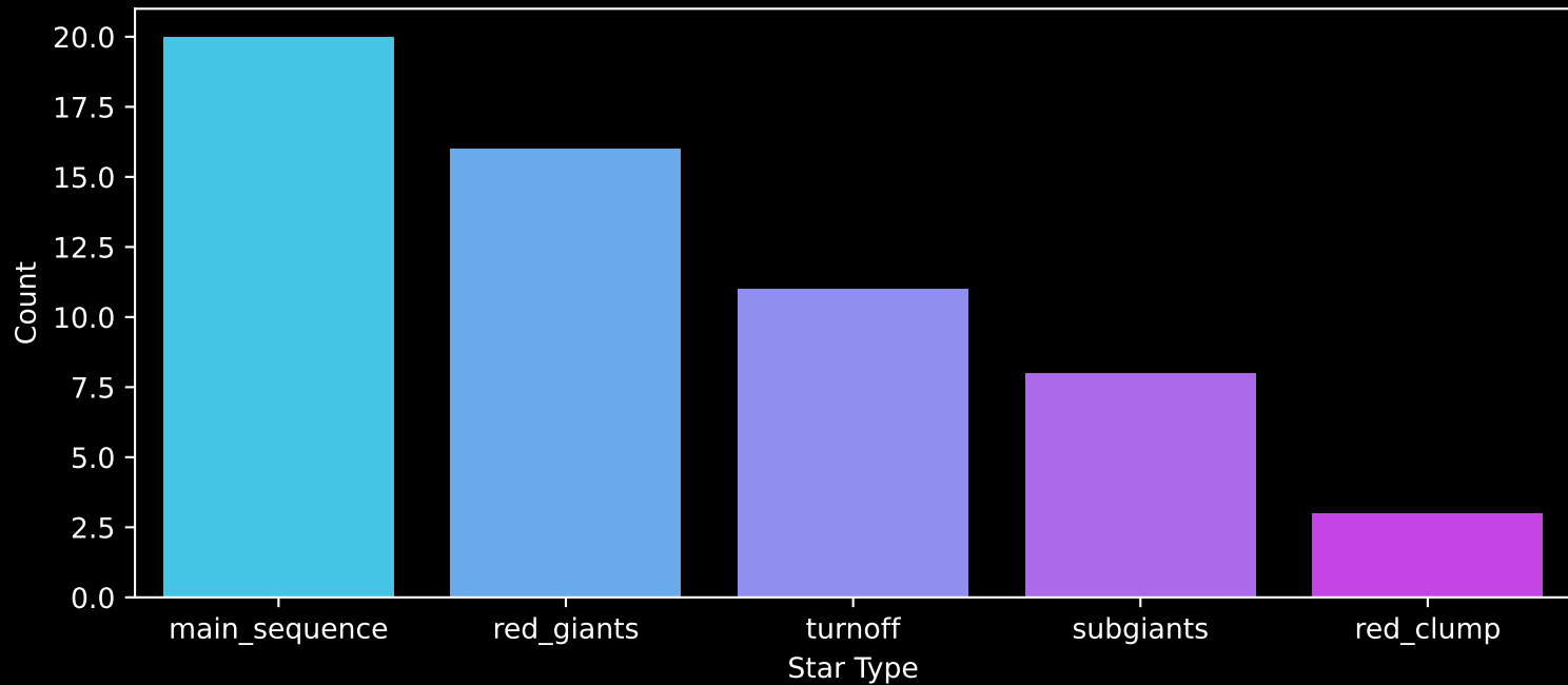
Gaia Cluster: [FSR_1530] Count plot of Star Type
