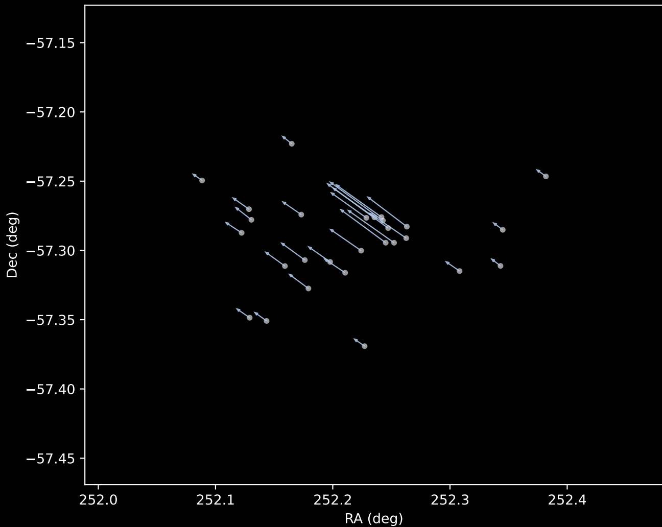
Gaia DR3 Cluster 1 Proper Motion Vectors (n=28)
