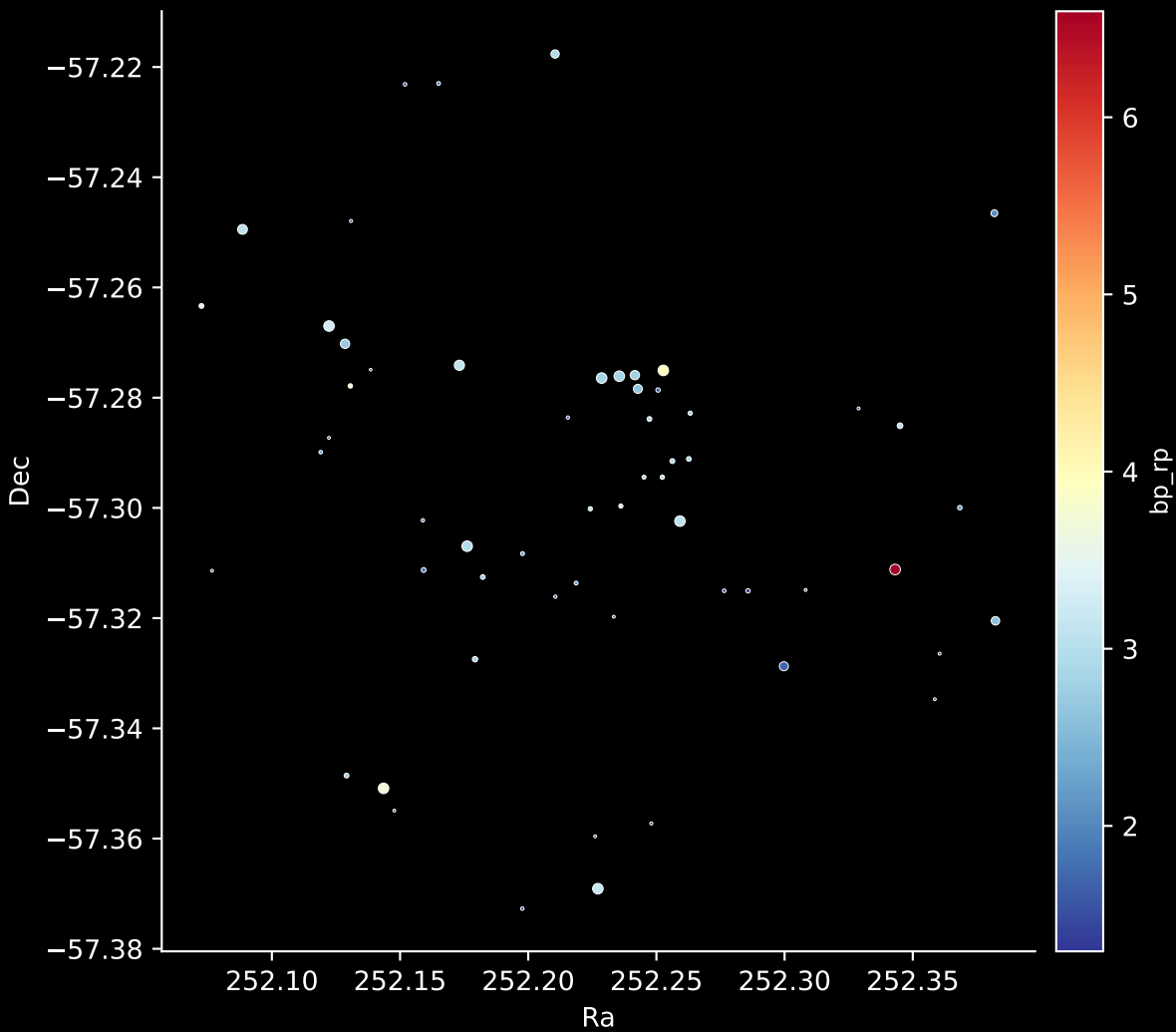
Gaia Cluster: [FSR_1530] Stars: 58
