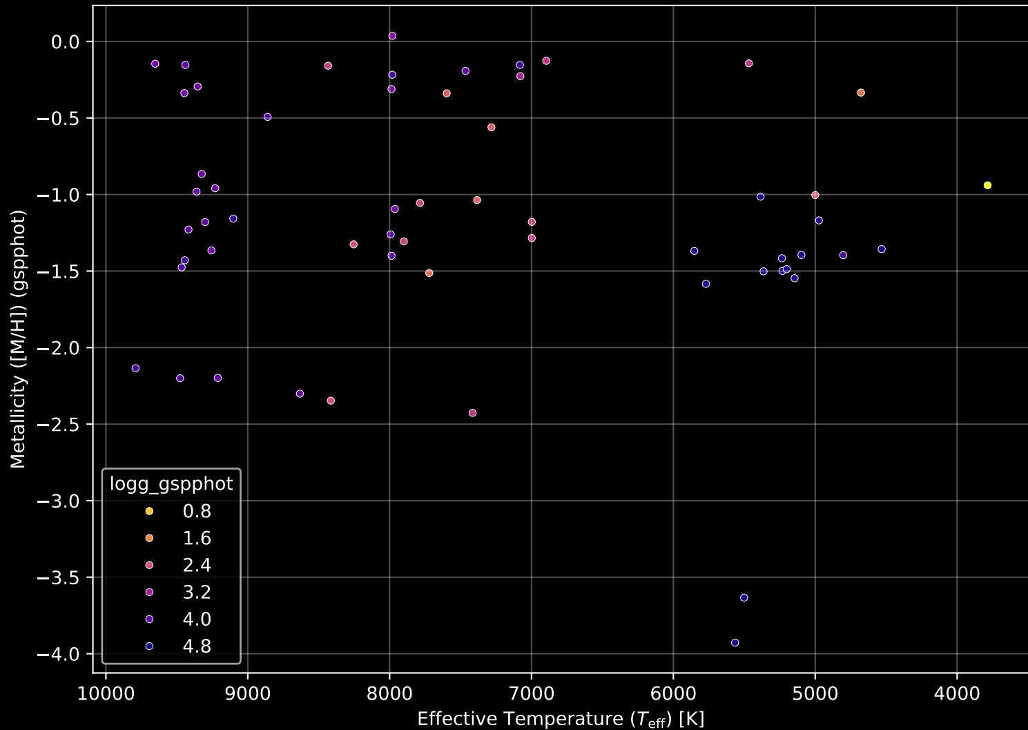
Gaia Cluster: [FSR_1530] Stellar Population Parameters (n= 58)
