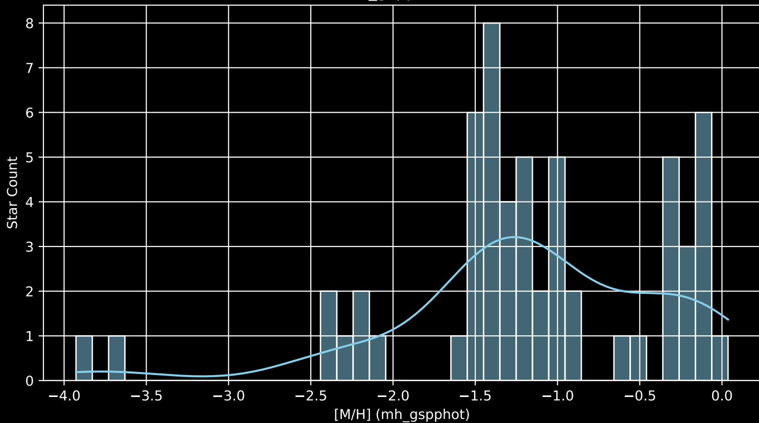
Gaia Cluster: [FSR_1530 [M/H] (mh_gspphot) (n= 58)
