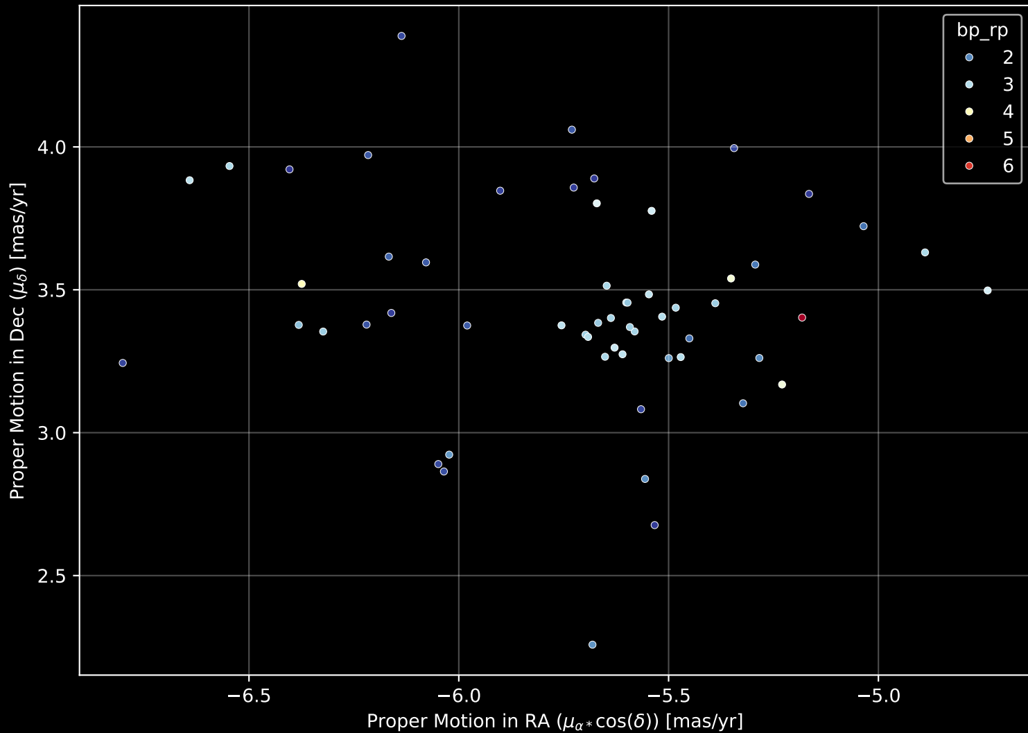
Gaia Cluster: [FSR_1530] Proper Motion Diagram (n= 58)
