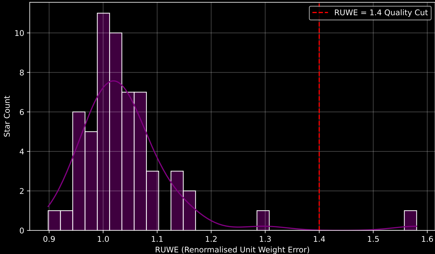
Gaia Cluster: [FSR_1530] RUWE Distribution (n= 58)
