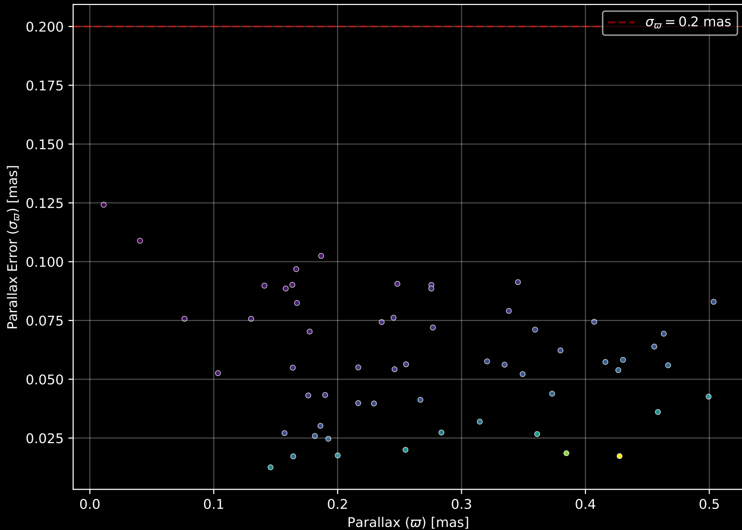
Gaia Cluster: [FSR_1530] Parallax Quality (n= 58)
