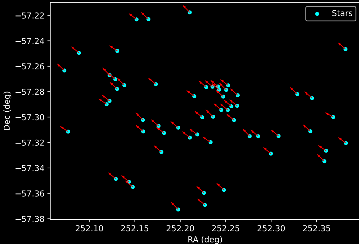
Gaia Cluster: [FSR_1530] Proper Motion Vectors for Gaia Star Field (n= 58)
