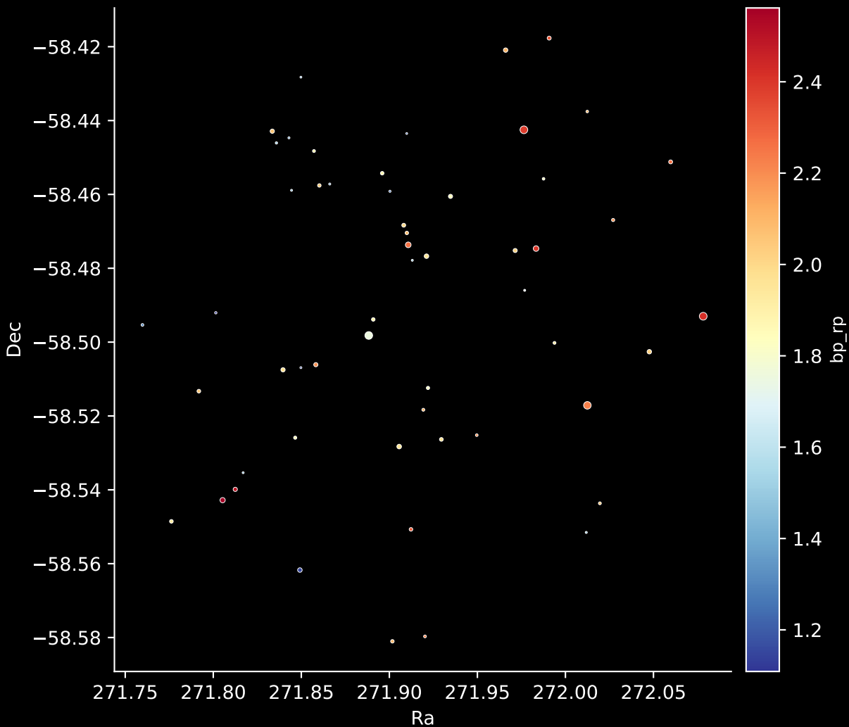
Gaia Cluster: [FSR_1580] Stars: 55
