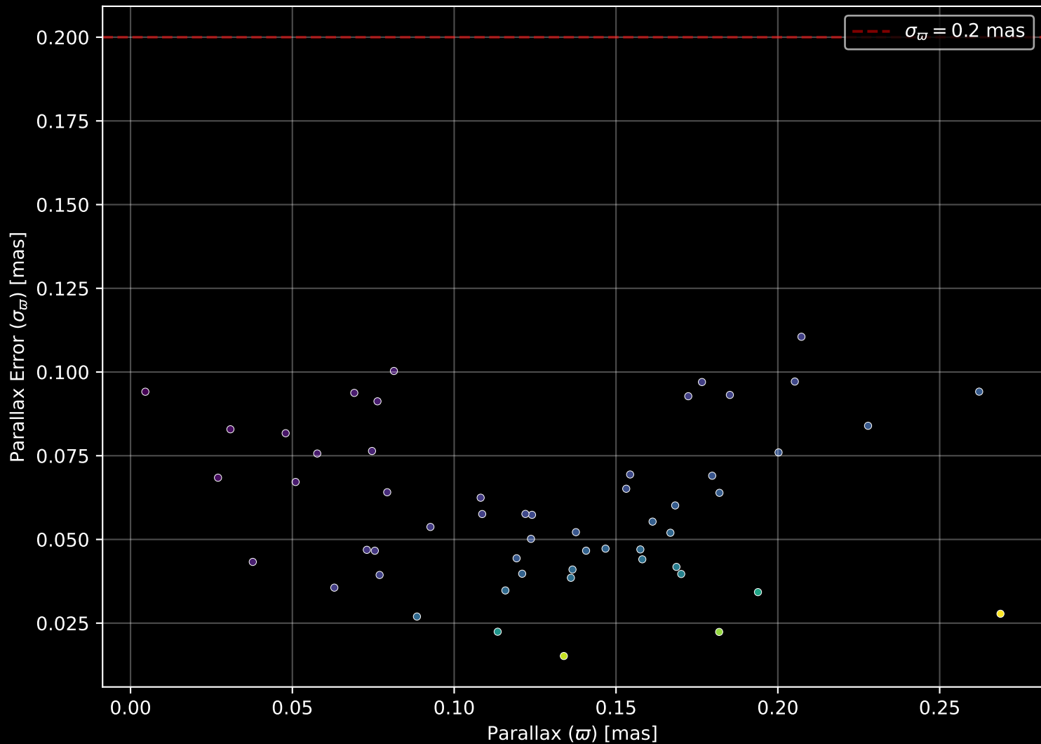
Gaia Cluster: [FSR_1580] Parallax Quality (n= 55)
