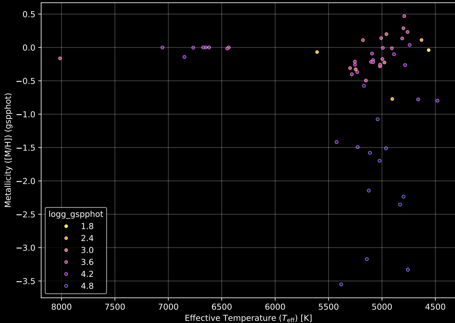
Gaia Cluster: [FSR_1580] Stellar Population Parameters (n= 55)
