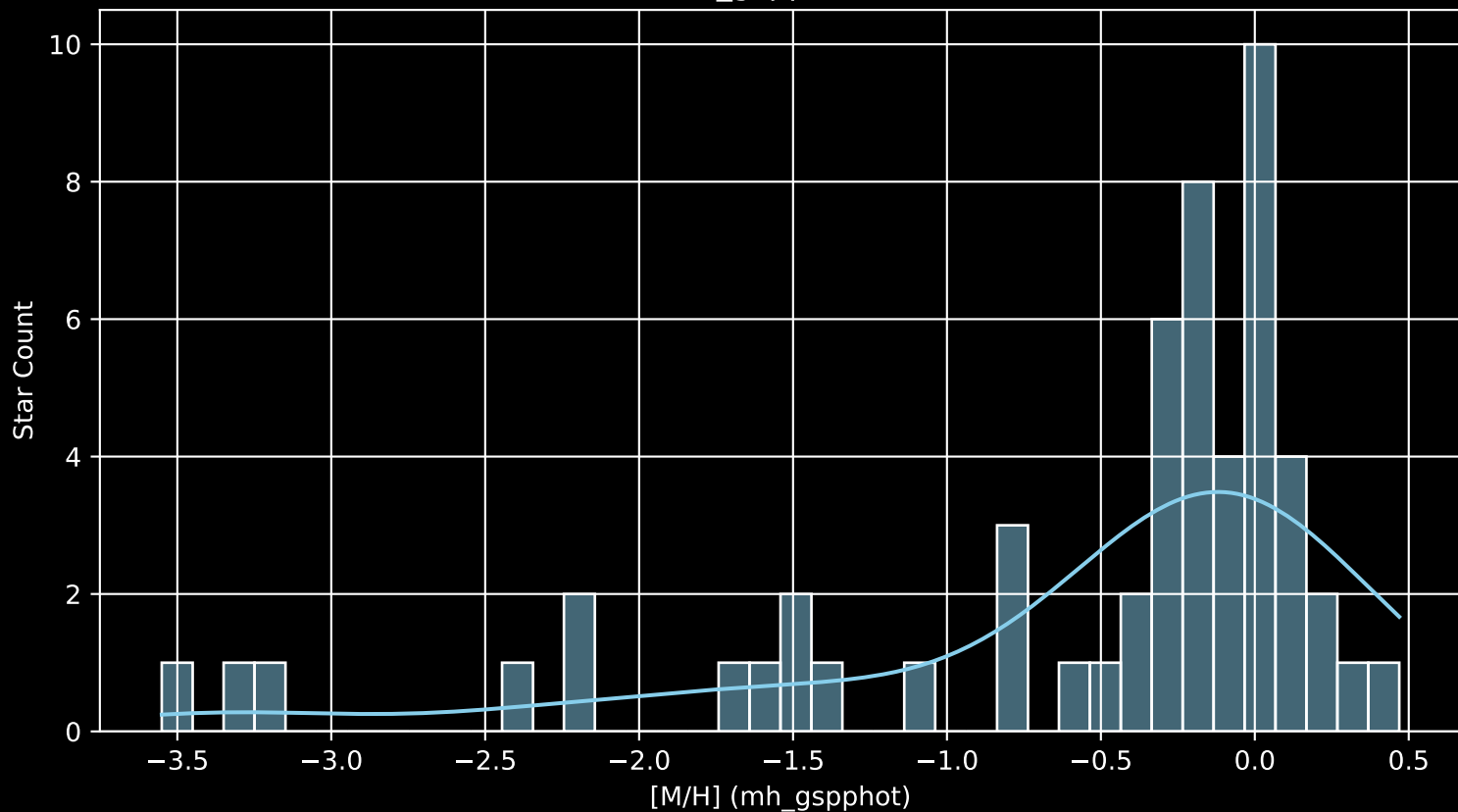
Gaia Cluster: [FSR_1580 [M/H] (mh_gspphot) (n= 55)
