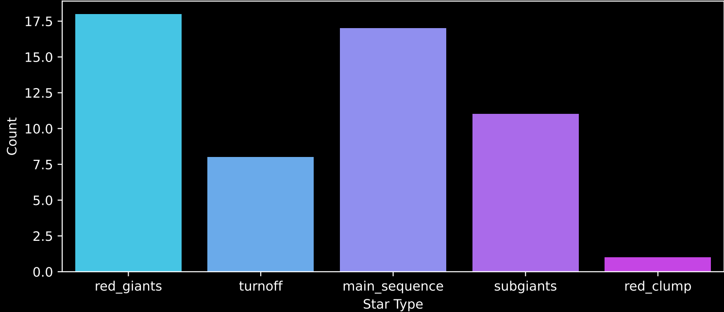
Gaia Cluster: [FSR_1580] Count plot of Star Type
