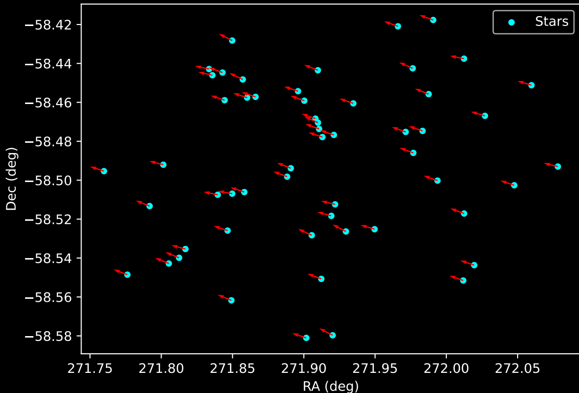
Gaia Cluster: [FSR_1580] Proper Motion Vectors for Gaia Star Field (n= 55)
