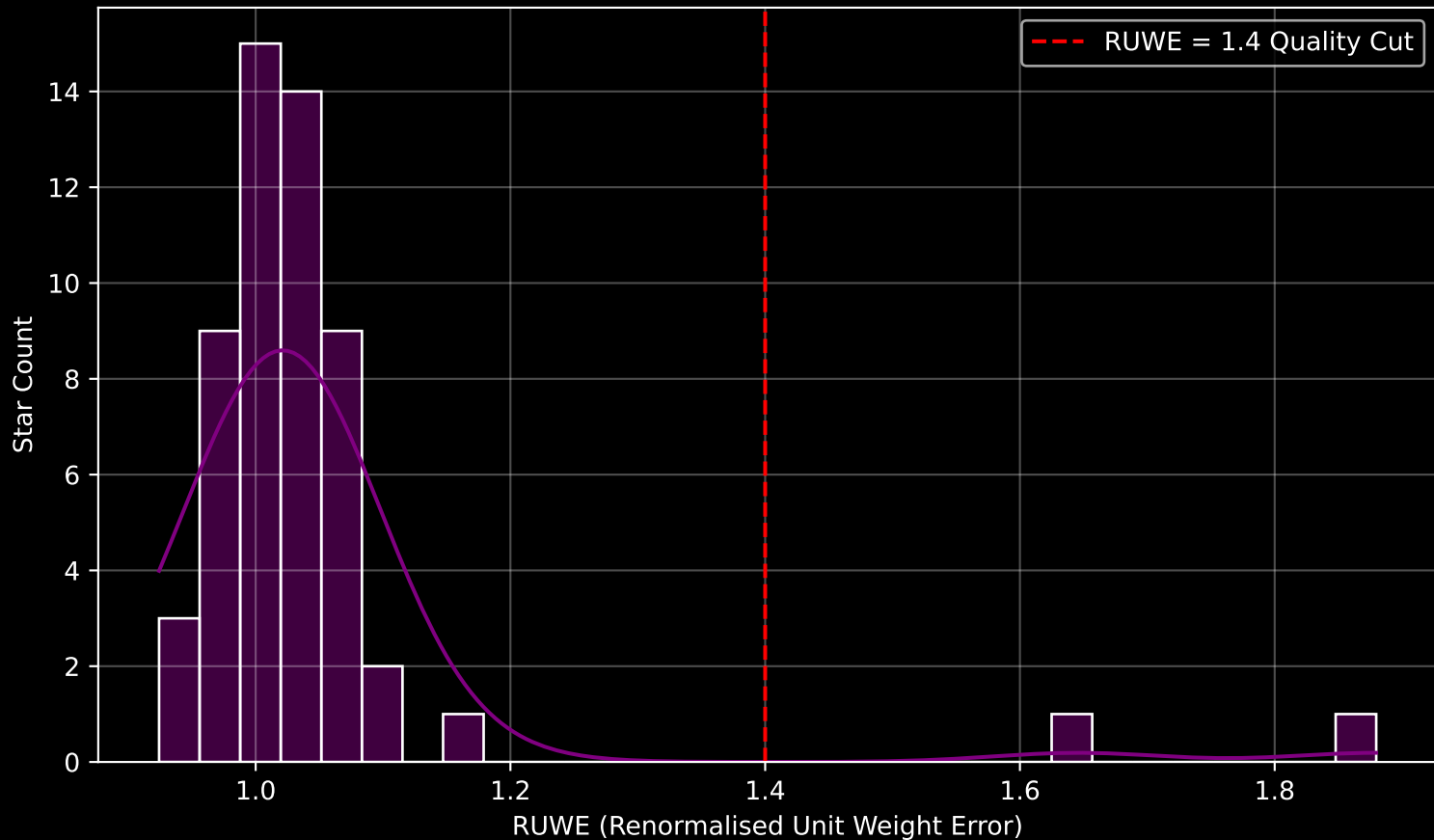
Gaia Cluster: [FSR_1580] RUWE Distribution (n= 55)
