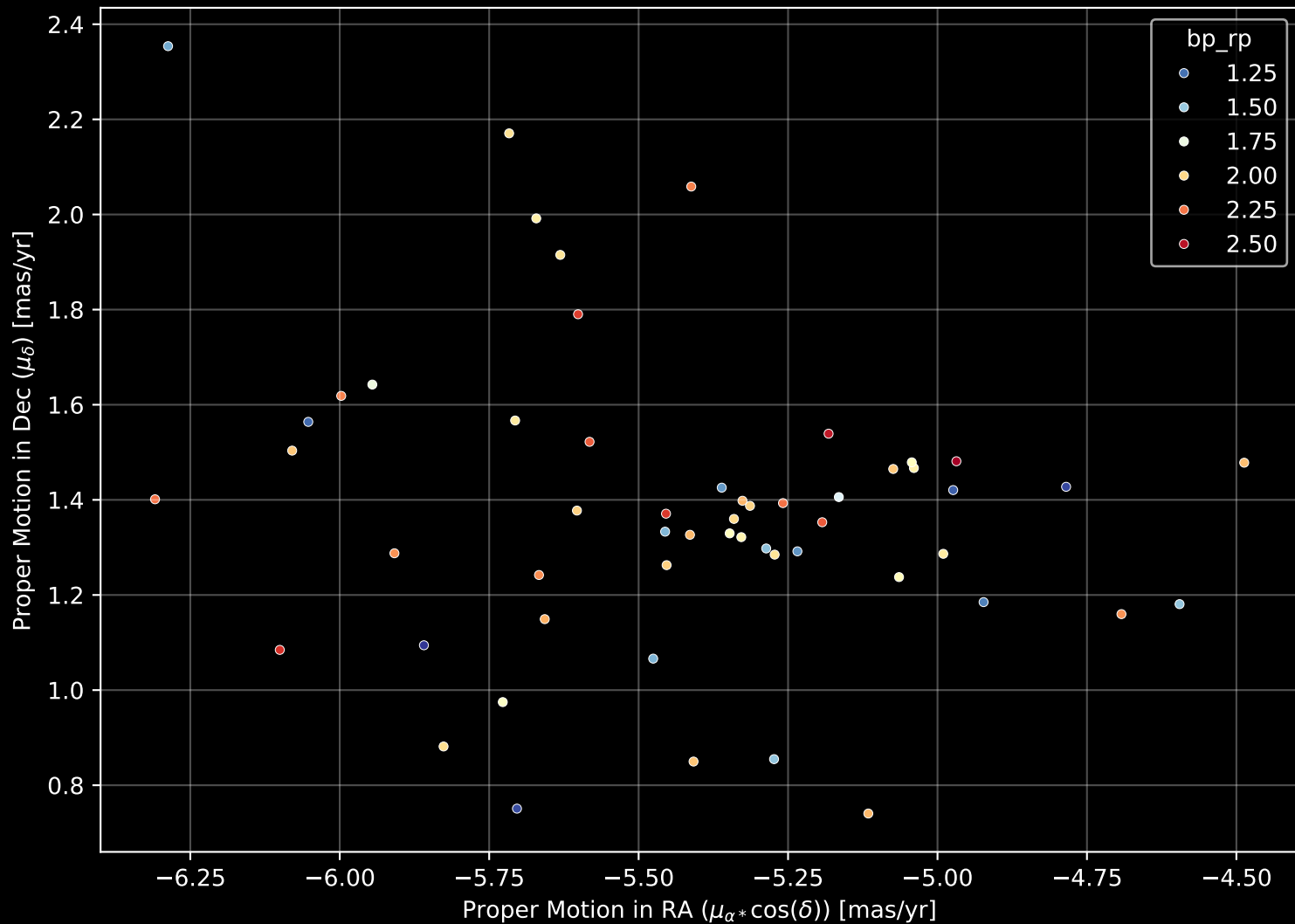
Gaia Cluster: [FSR_1580] Proper Motion Diagram (n= 55)
