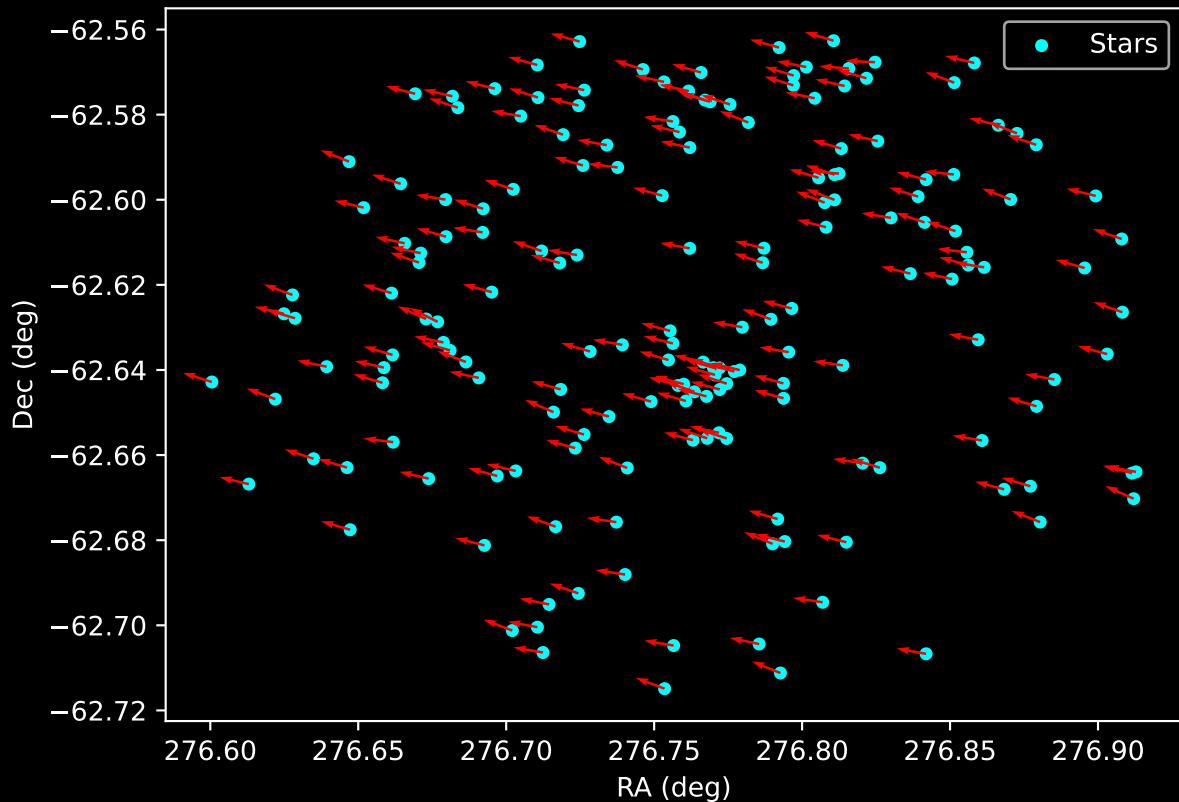
Gaia Cluster: [FSR_1595] Proper Motion Vectors for Gaia Star Field (n= 175)
