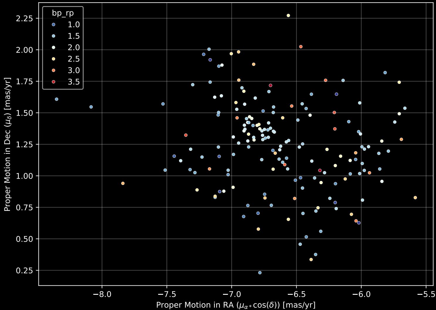
Gaia Cluster: [FSR_1595] Proper Motion Diagram (n= 175)
