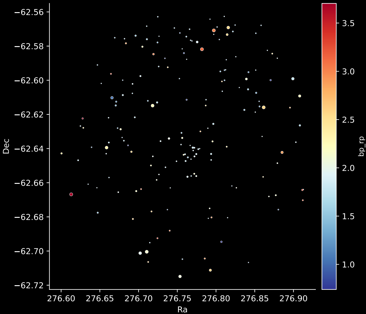
Gaia Cluster: [FSR_1595] Stars: 175
