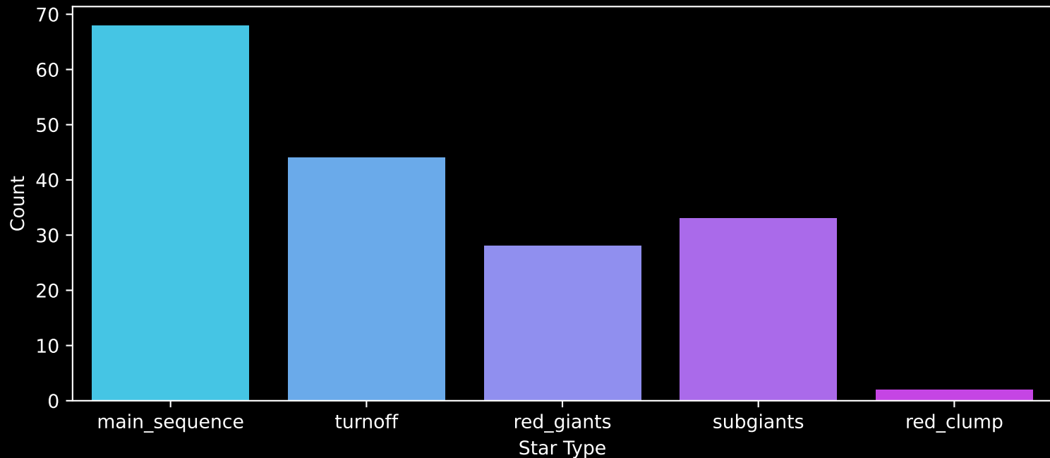
Gaia Cluster: [FSR_1595] Count plot of Star Type
