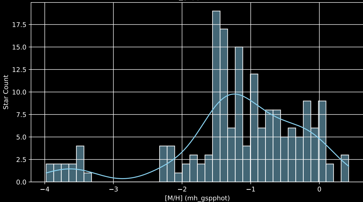
Gaia Cluster: [FSR_1595 [M/H] (mh_gspphot) (n= 172)
