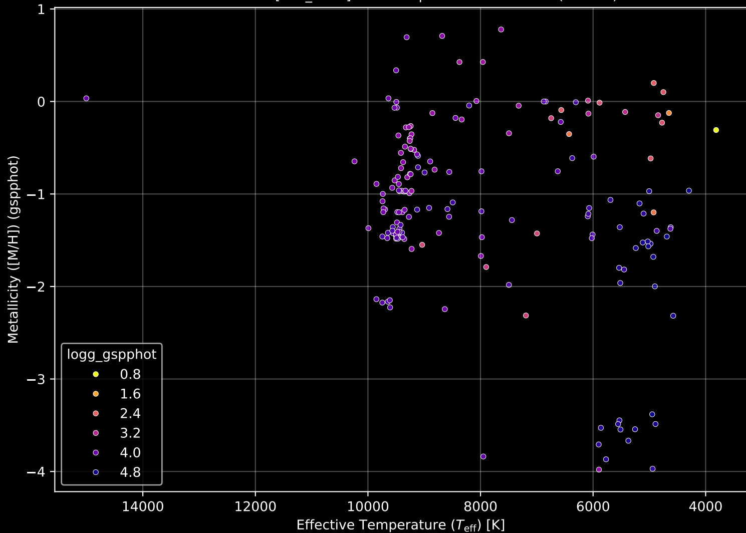
Gaia Cluster: [FSR_1595] Stellar Population Parameters (n= 175)
