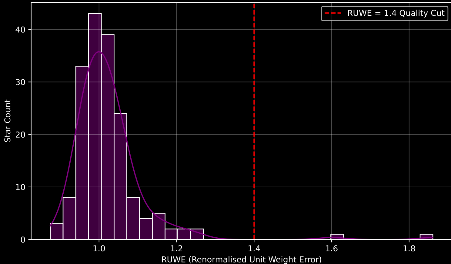
Gaia Cluster: [FSR_1595] RUWE Distribution (n= 175)
