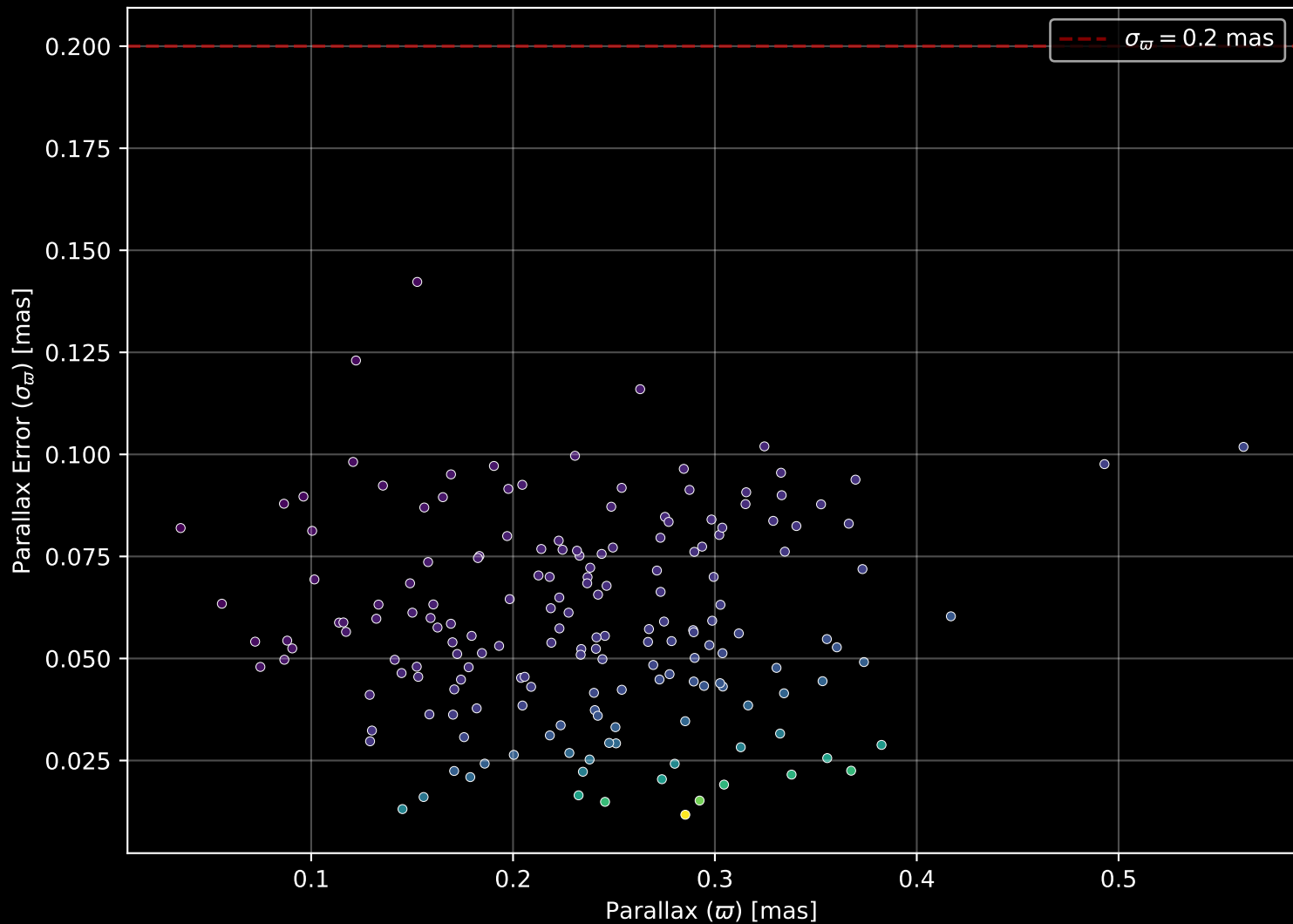
Gaia Cluster: [FSR_1595] Parallax Quality (n= 175)
