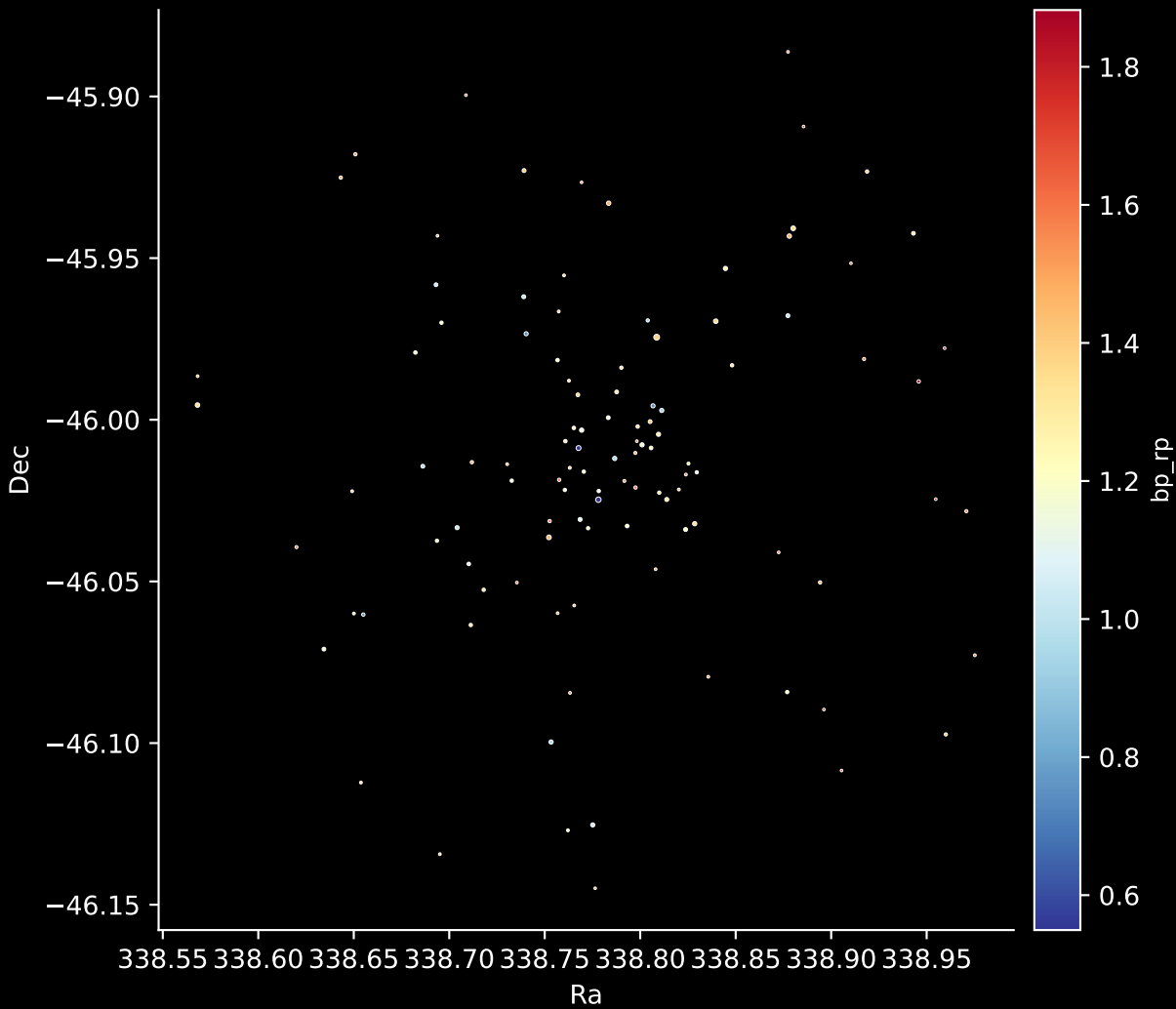
Gaia Cluster: [FSR_1723] Stars: 108
