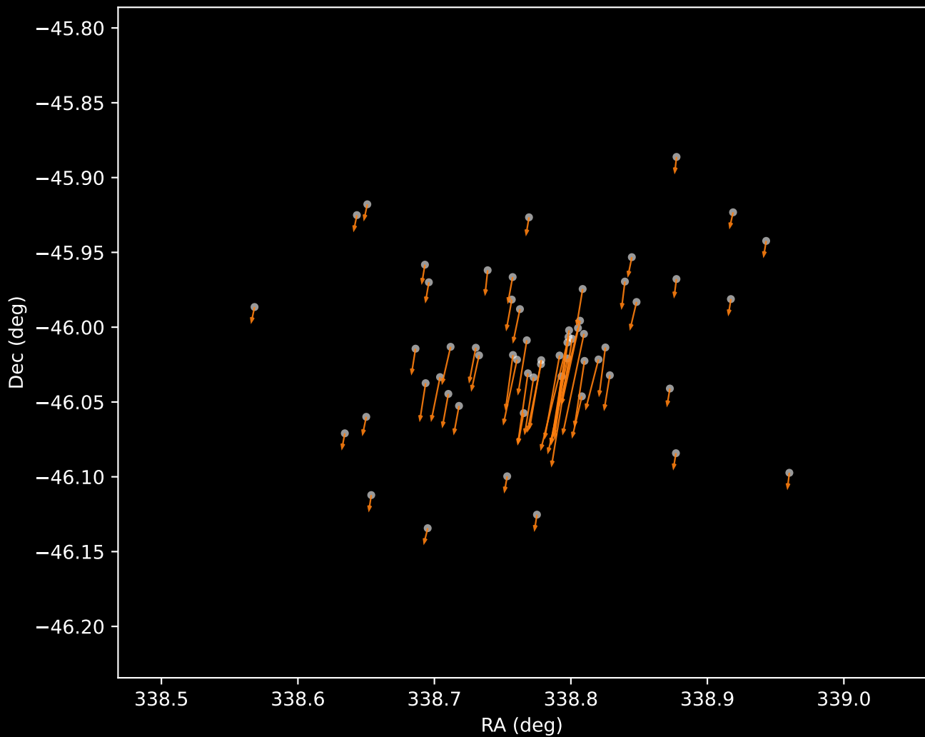
Gaia DR3 Cluster 2 Proper Motion Vectors (n=59)
