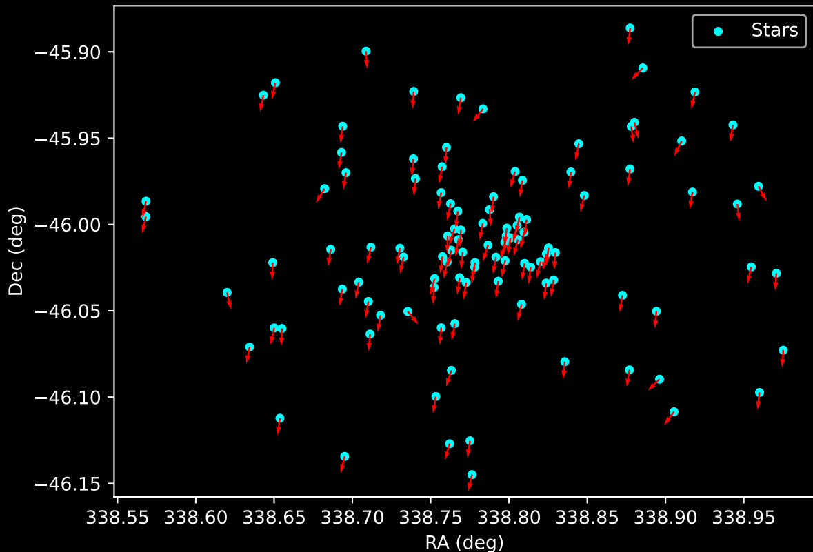
Gaia Cluster: [FSR_1723] Proper Motion Vectors for Gaia Star Field (n= 108)
