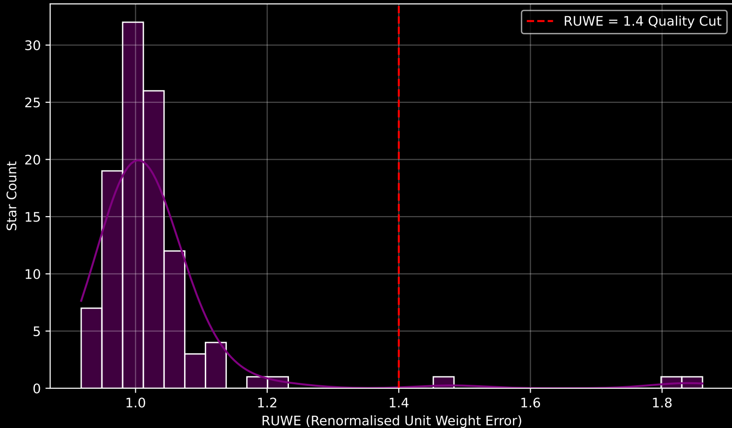
Gaia Cluster: [FSR_1723] RUWE Distribution (n= 108)
