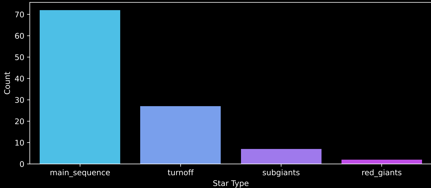
Gaia Cluster: [FSR_1723] Count plot of Star Type
