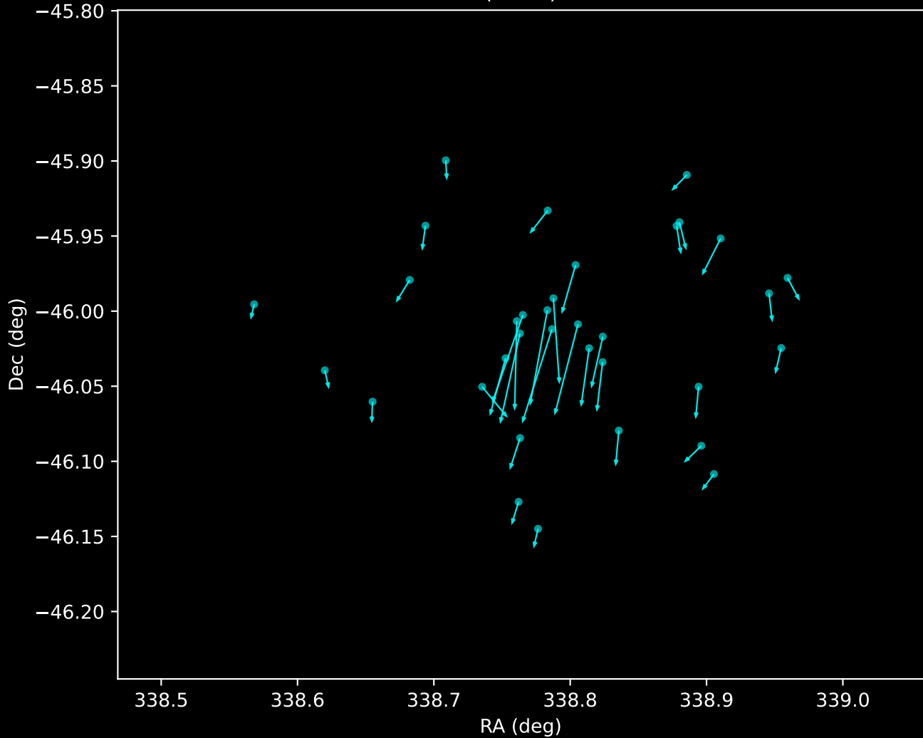
Gaia DR3 Noise Stream Proper Motion Vectors (n=34)
