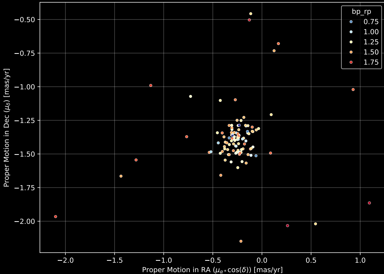
Gaia Cluster: [FSR_1723] Proper Motion Diagram (n= 108)
