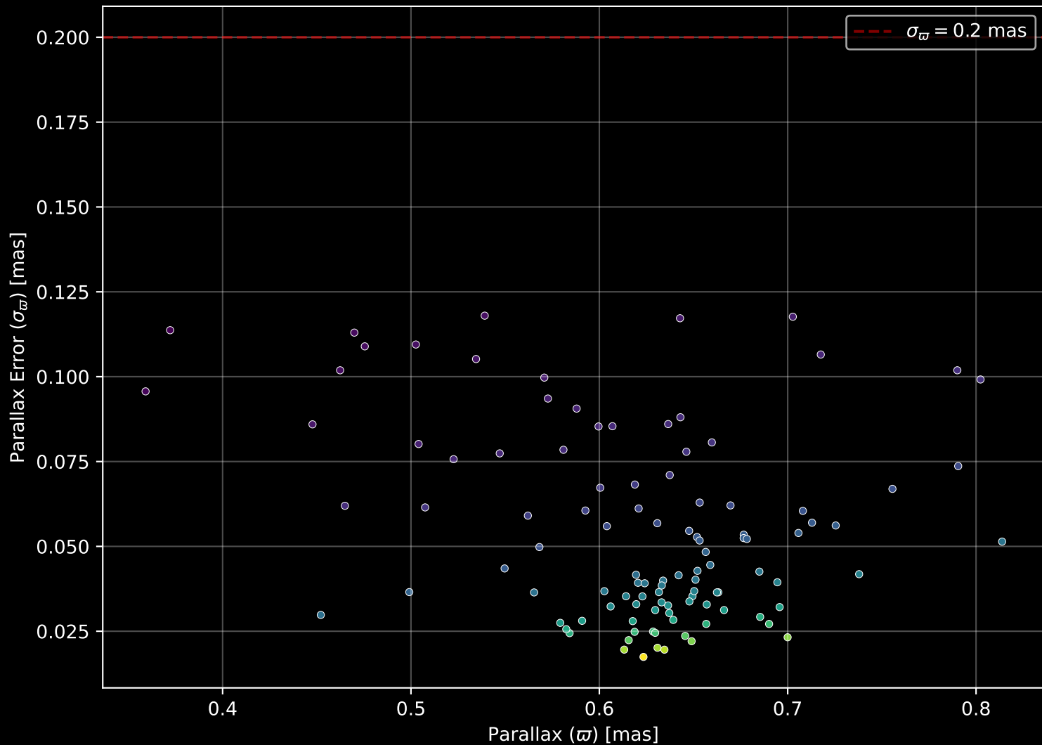
Gaia Cluster: [FSR_1723] Parallax Quality (n= 108)
