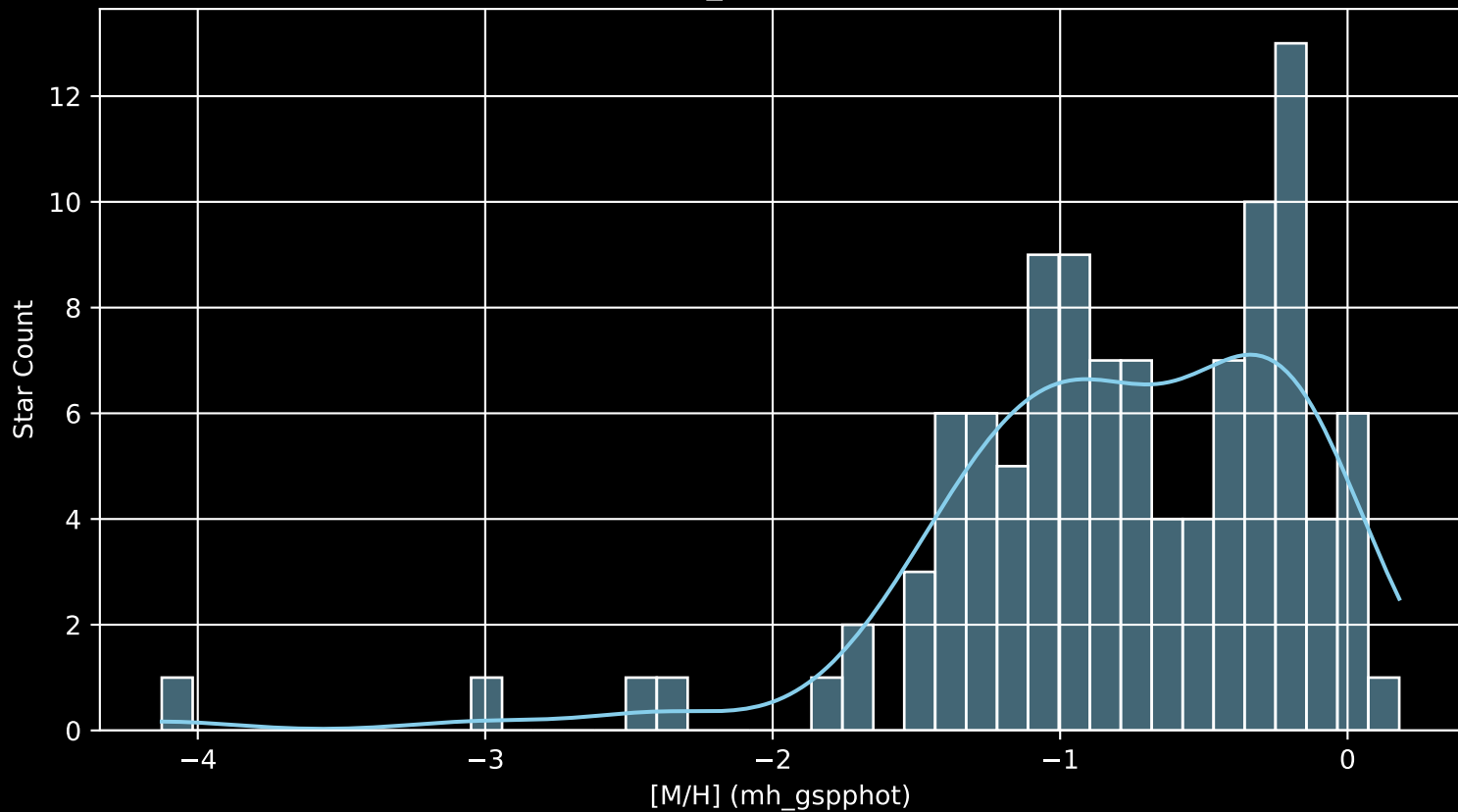
Gaia Cluster: [FSR_1723 [M/H] (mh_gspphot) (n= 108)
