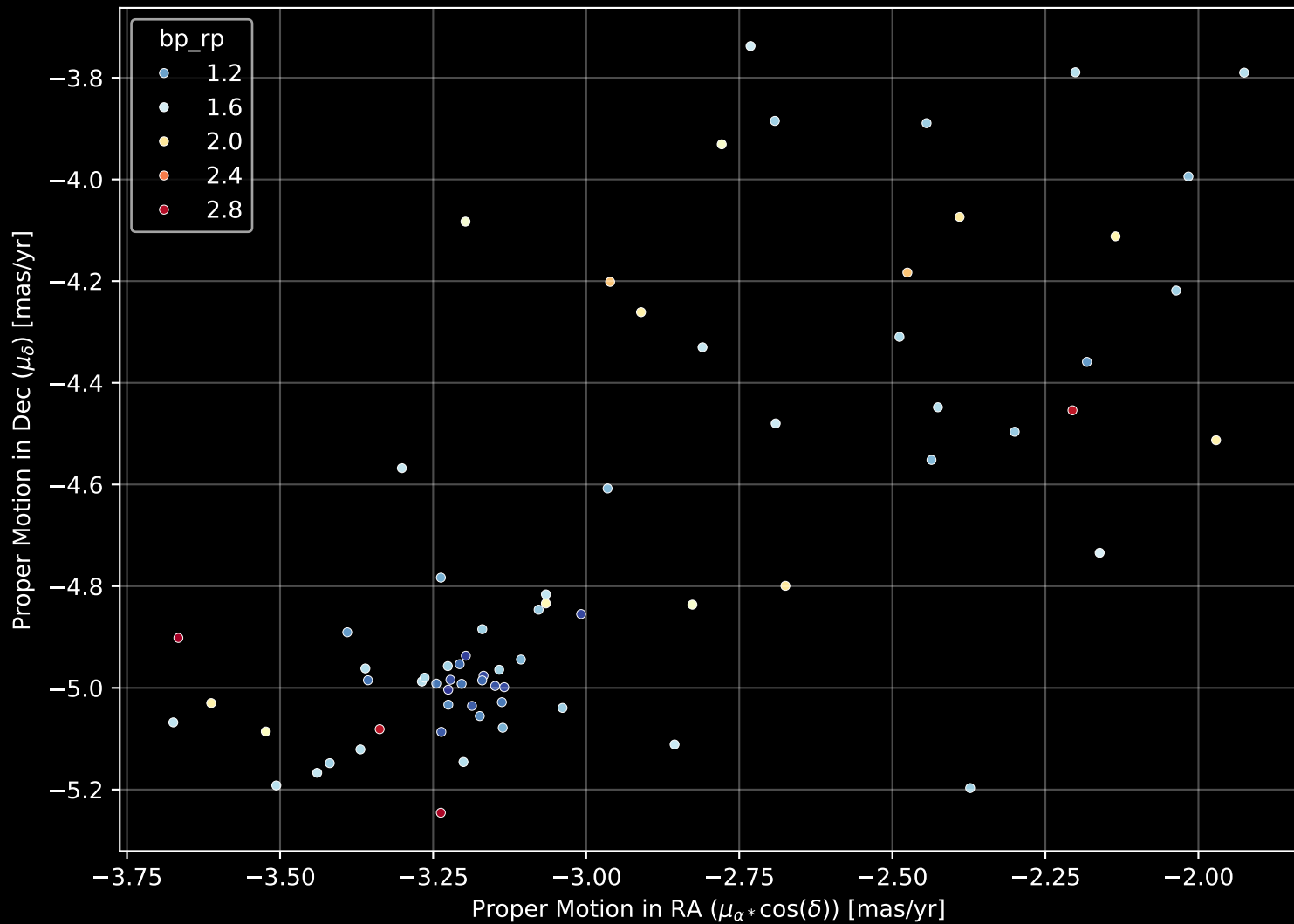
Gaia Cluster: [Feibelman_1] Proper Motion Diagram (n= 72)
