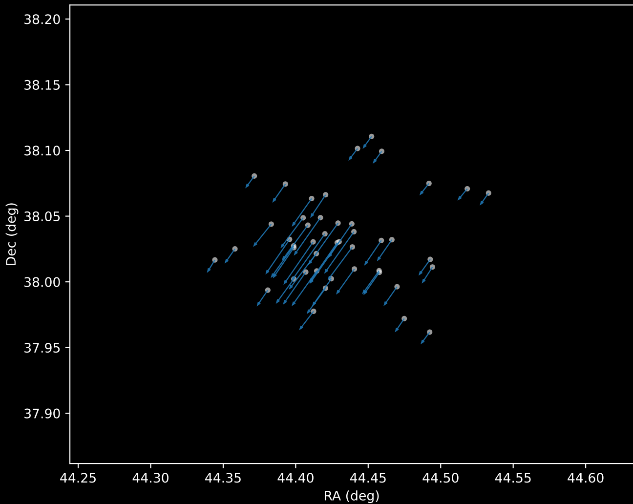
Gaia DR3 Cluster 0 Proper Motion Vectors (n=45)
