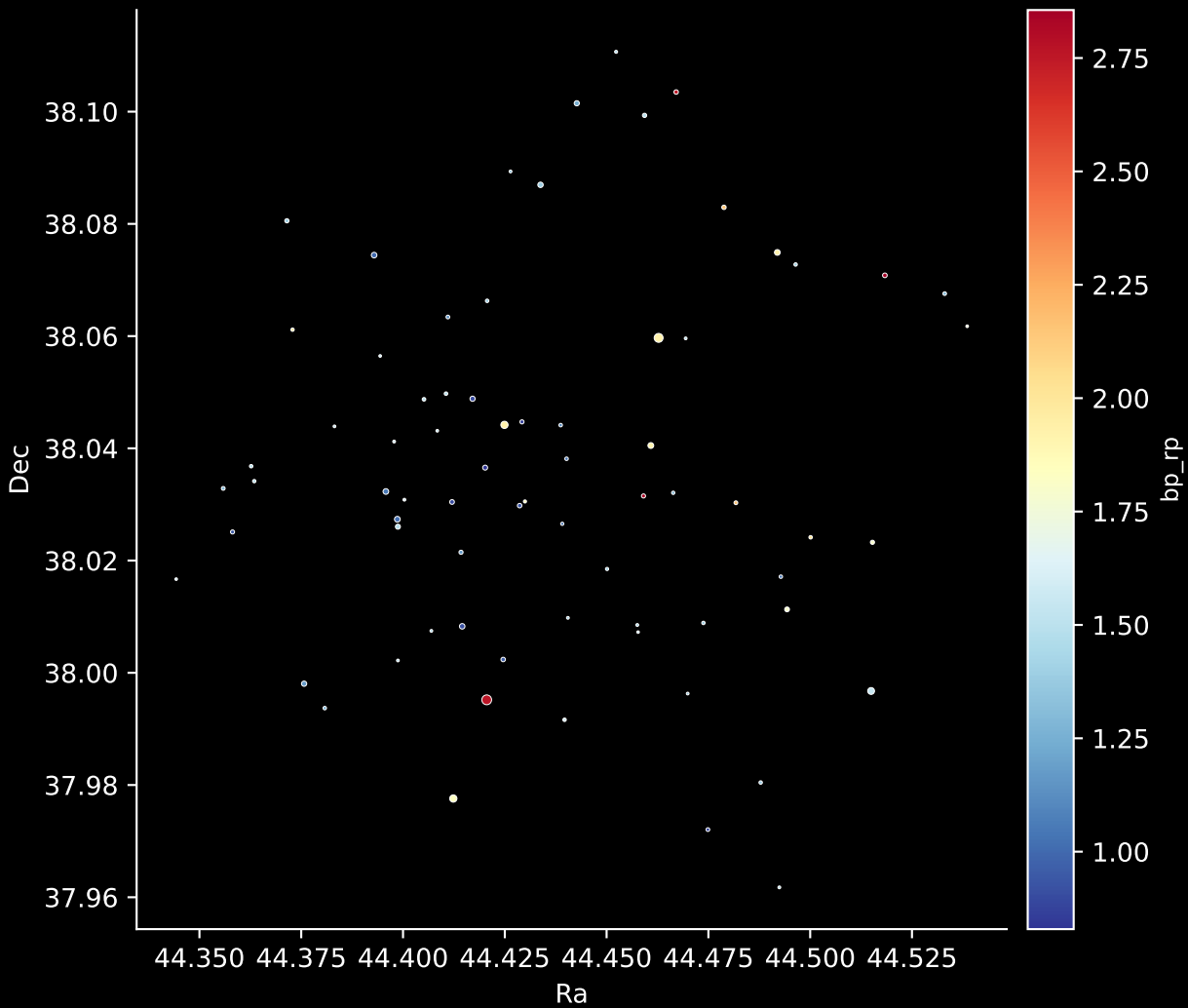
Gaia Cluster: [Feibelman_1] Stars: 72
