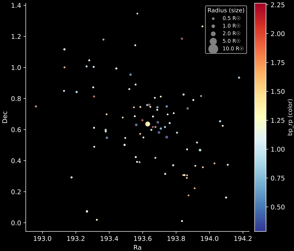
Gaia Cluster: [Ferrero_11] Stars: 90
