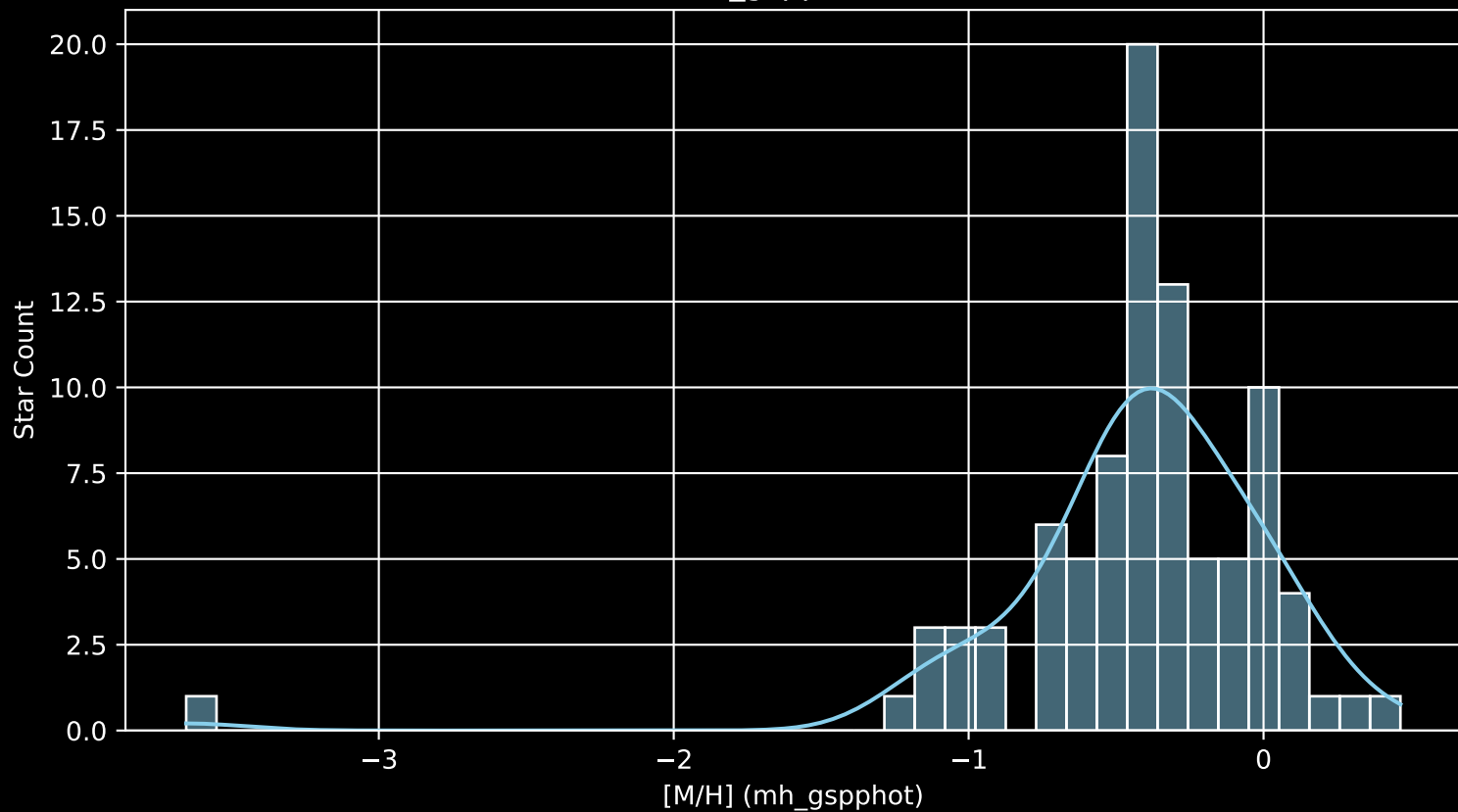
Gaia Cluster: [Ferrero_11 [M/H] (mh_gspphot) (n= 90)
