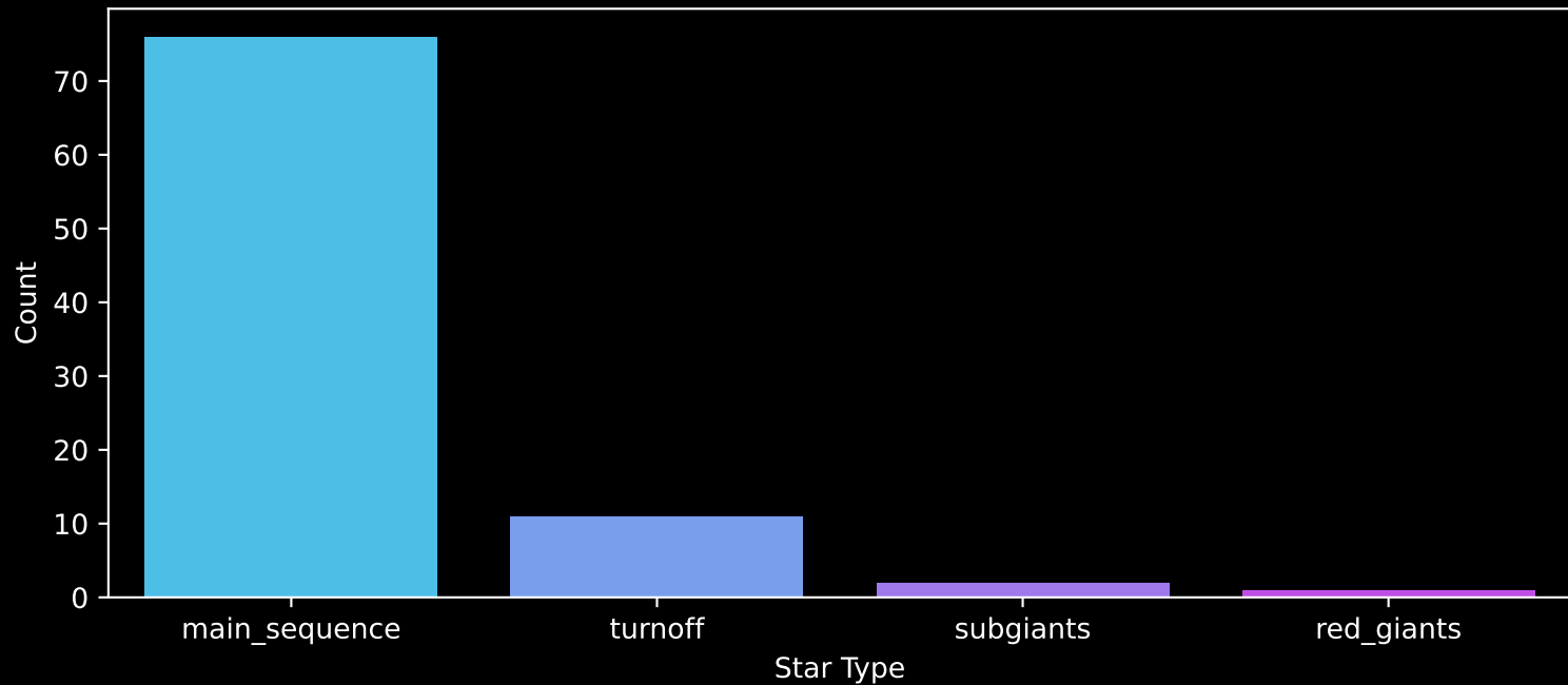
Gaia Cluster: [Ferrero_11] Count plot of Star Type
