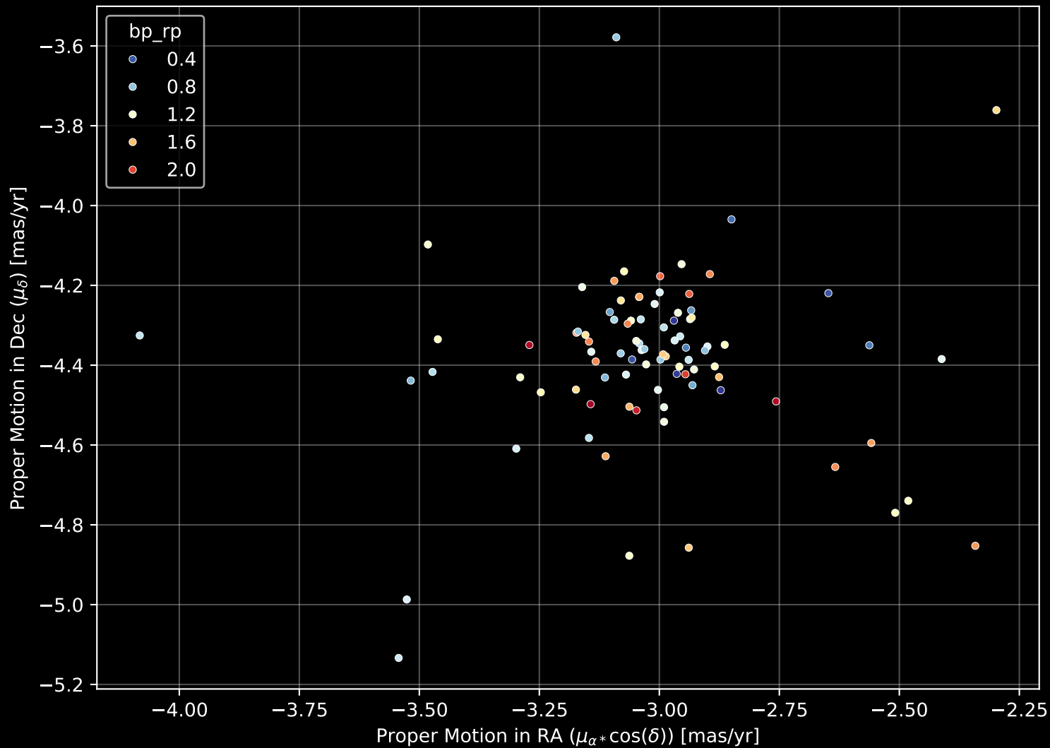
Gaia Cluster: [Ferrero_11] Proper Motion Diagram (n= 90)
