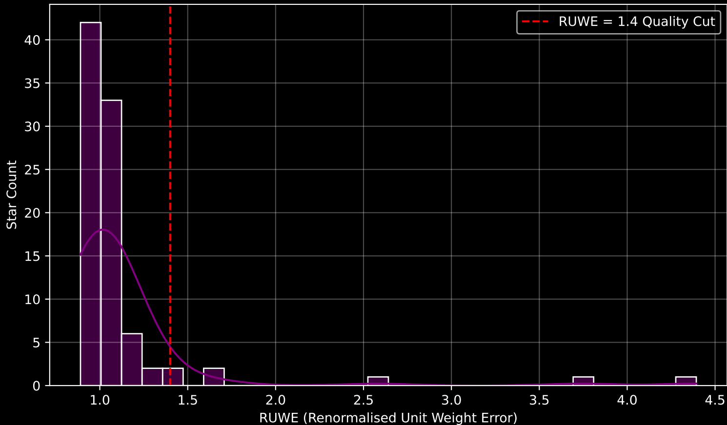
Gaia Cluster: [Ferrero_11] RUWE Distribution (n= 90)
