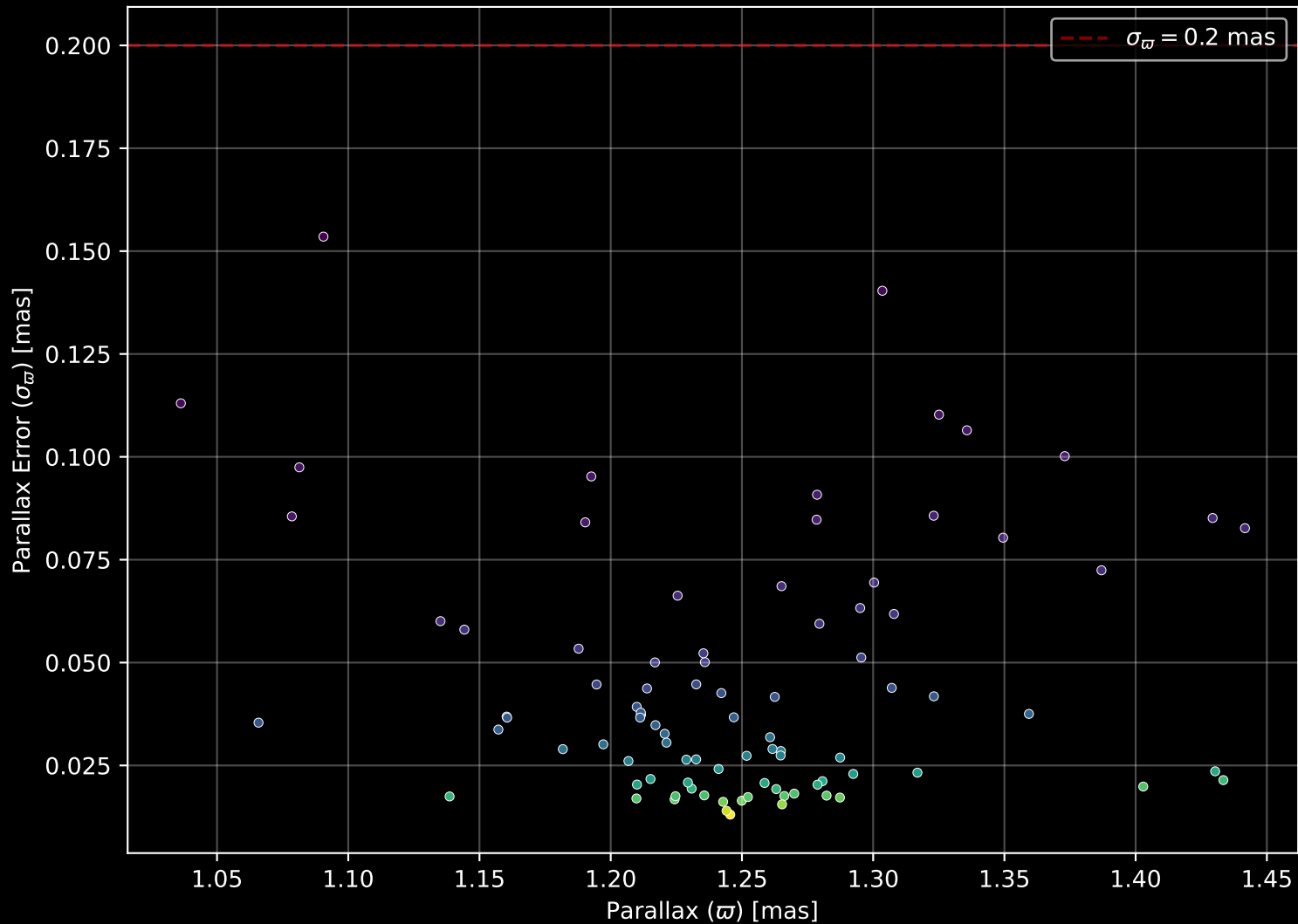
Gaia Cluster: [Ferrero_11] Parallax Quality (n= 90)
