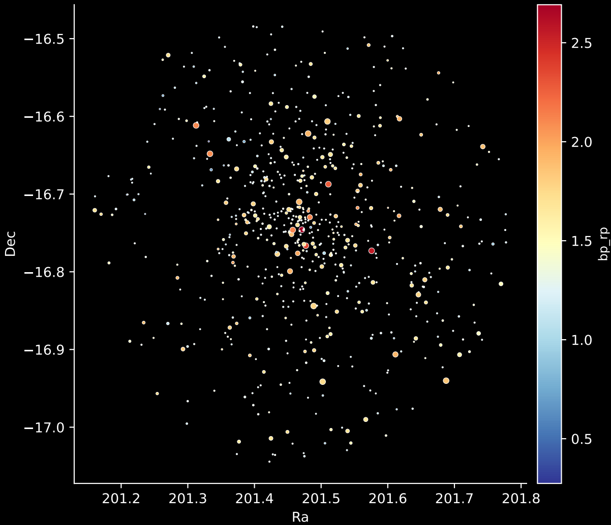
Gaia Cluster: [Gaia_1] Stars: 663
