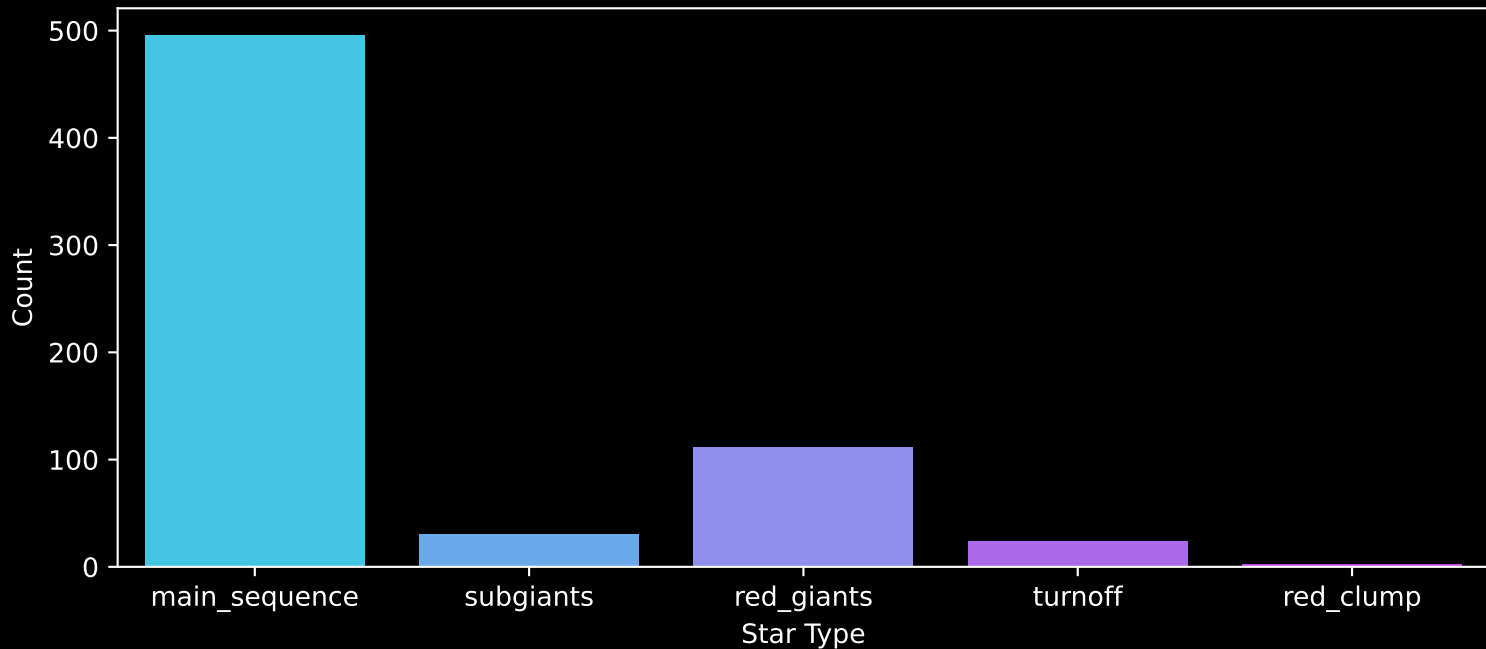
Gaia Cluster: [Gaia_1] Count plot of Star Type
