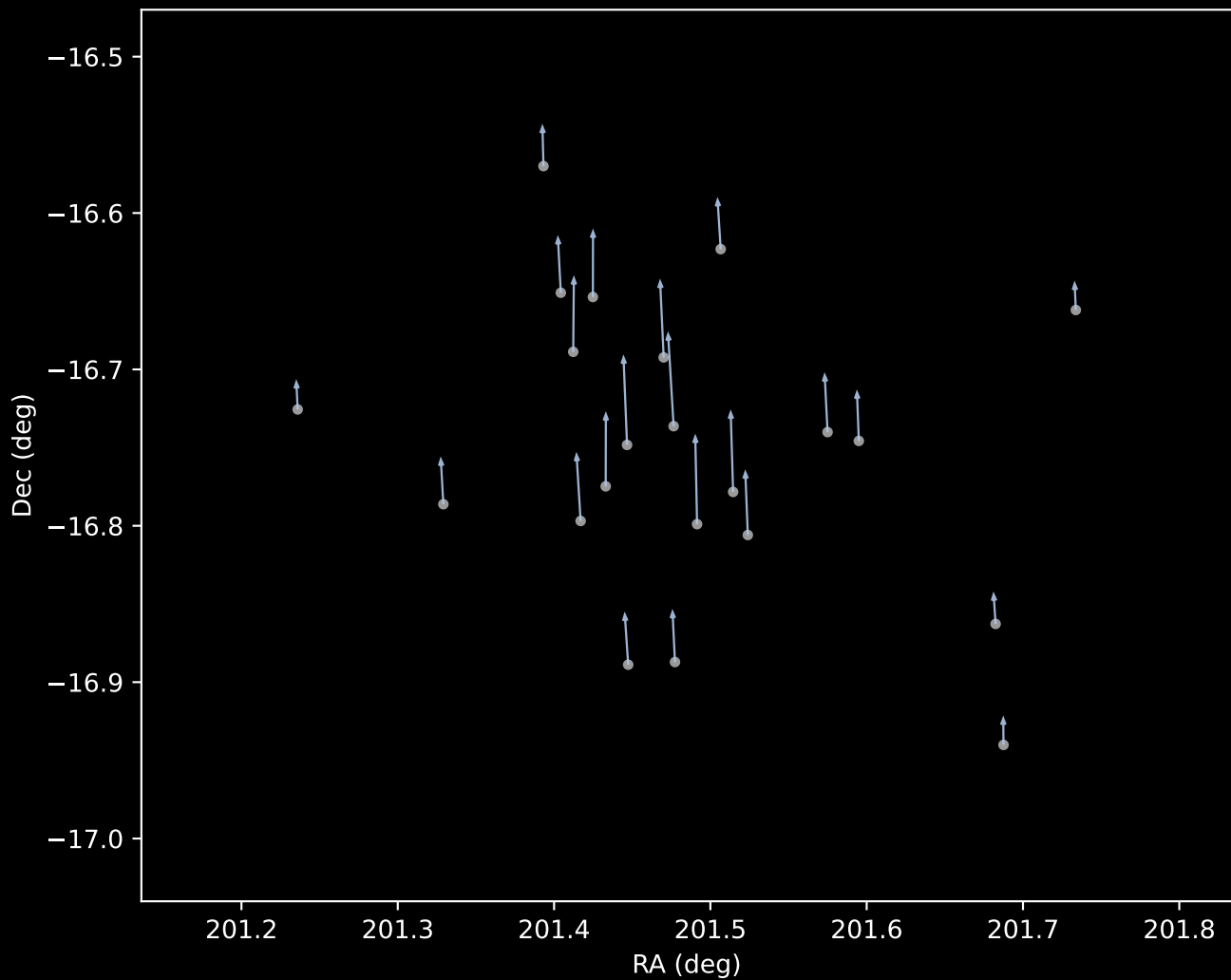
Gaia DR3 Cluster 21 Proper Motion Vectors (n=22)
