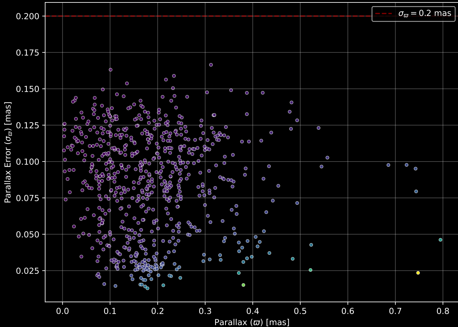
Gaia Cluster: [Gaia_1] Parallax Quality (n= 663)
