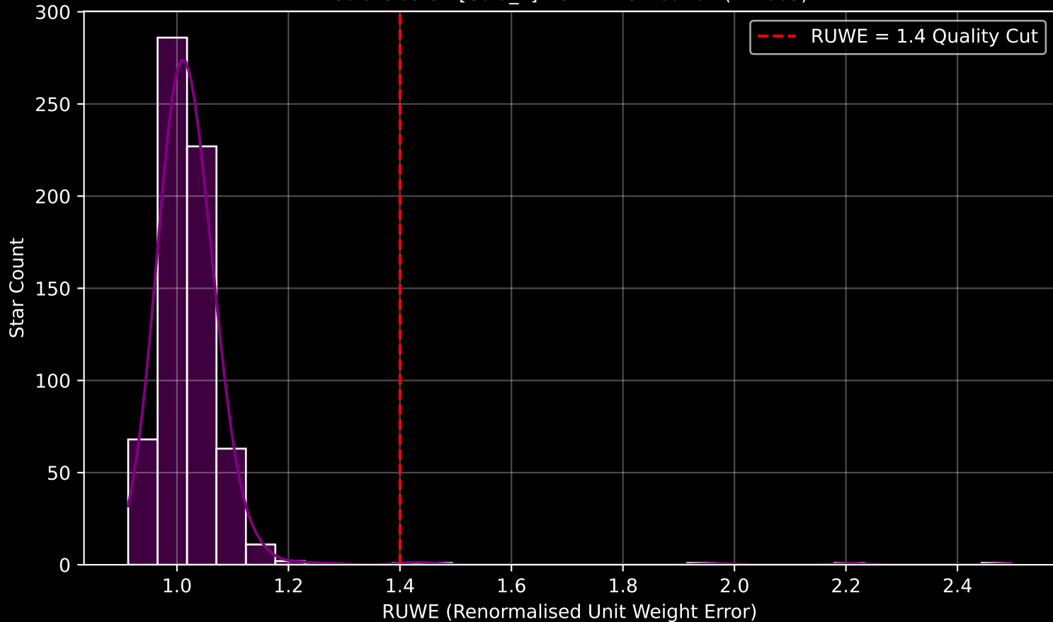
Gaia Cluster: [Gaia_1] RUWE Distribution (n= 663)
