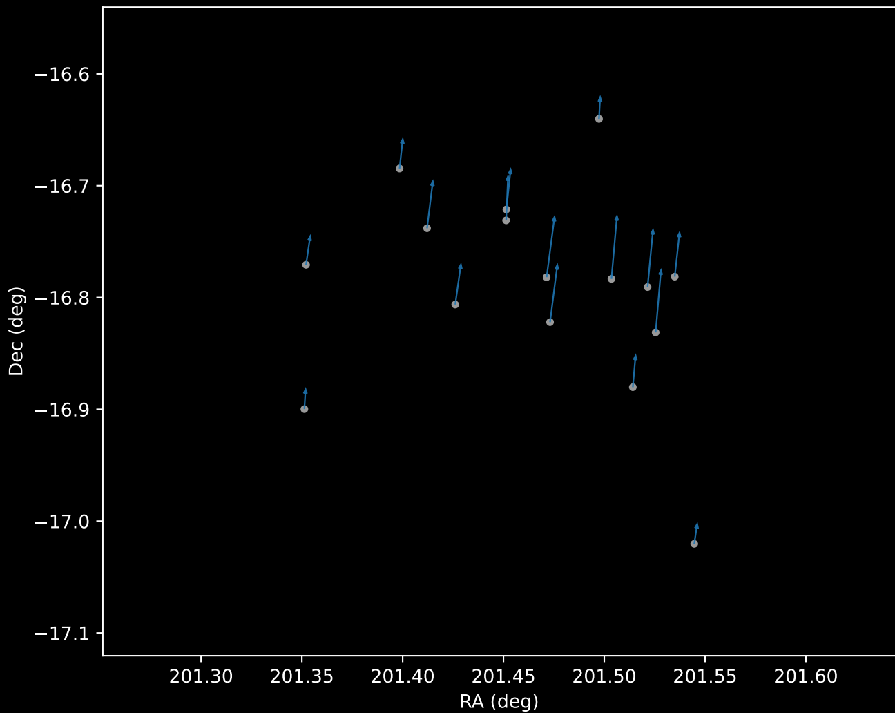
Gaia DR3 Cluster 20 Proper Motion Vectors (n=16)
