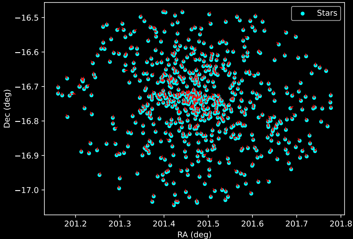
Gaia Cluster: [Gaia_1] Proper Motion Vectors for Gaia Star Field (n= 663)
