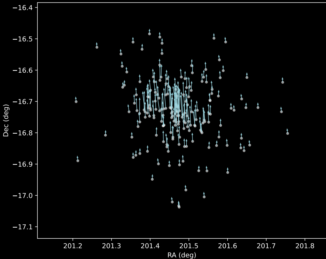
Gaia DR3 Cluster 19 Proper Motion Vectors (n=186)
