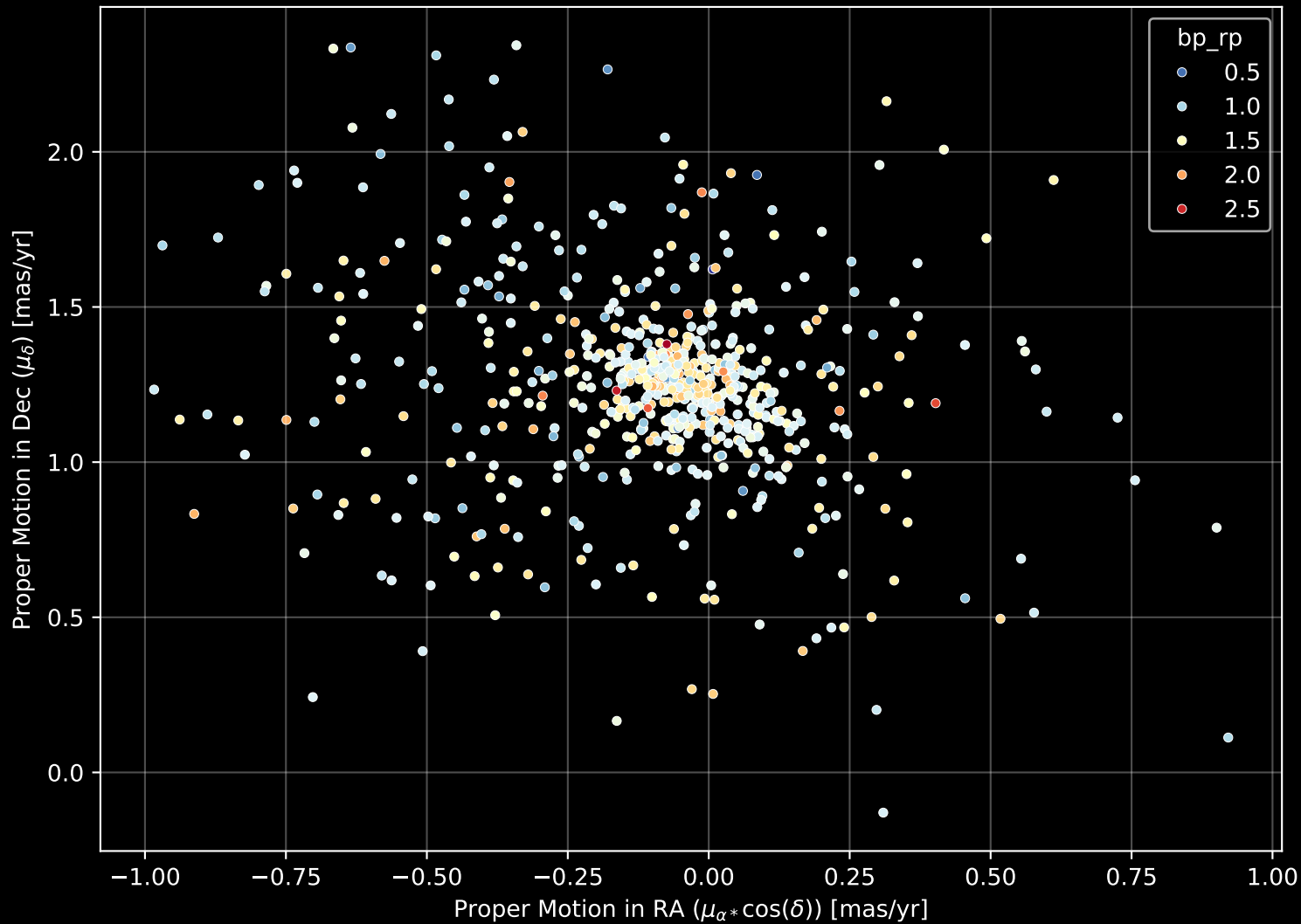
Gaia Cluster: [Gaia_1] Proper Motion Diagram (n= 663)
