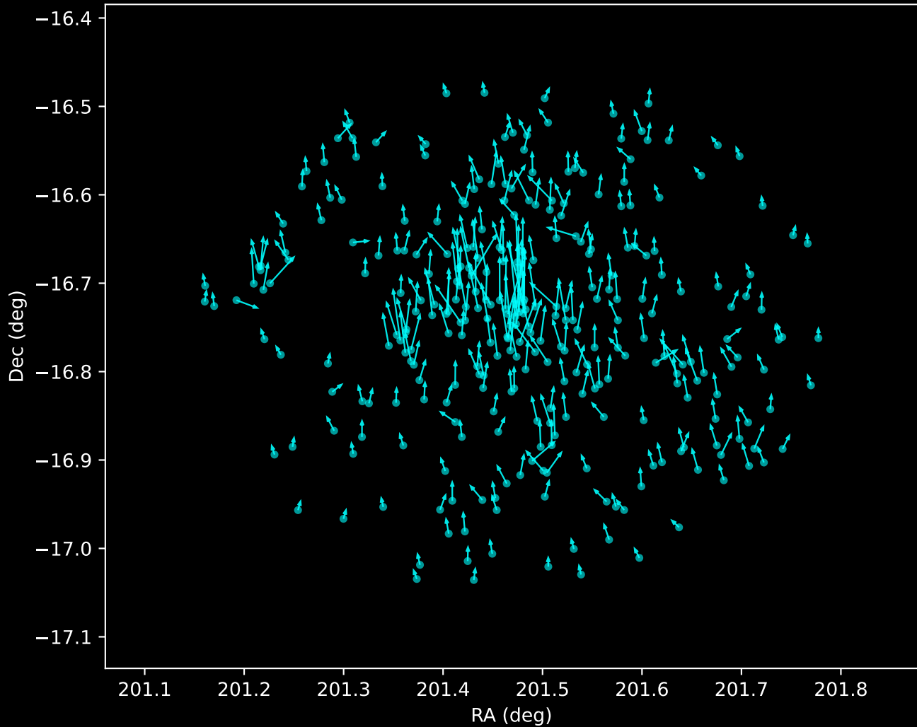
Gaia DR3 Noise Stream Proper Motion Vectors (n=301)
