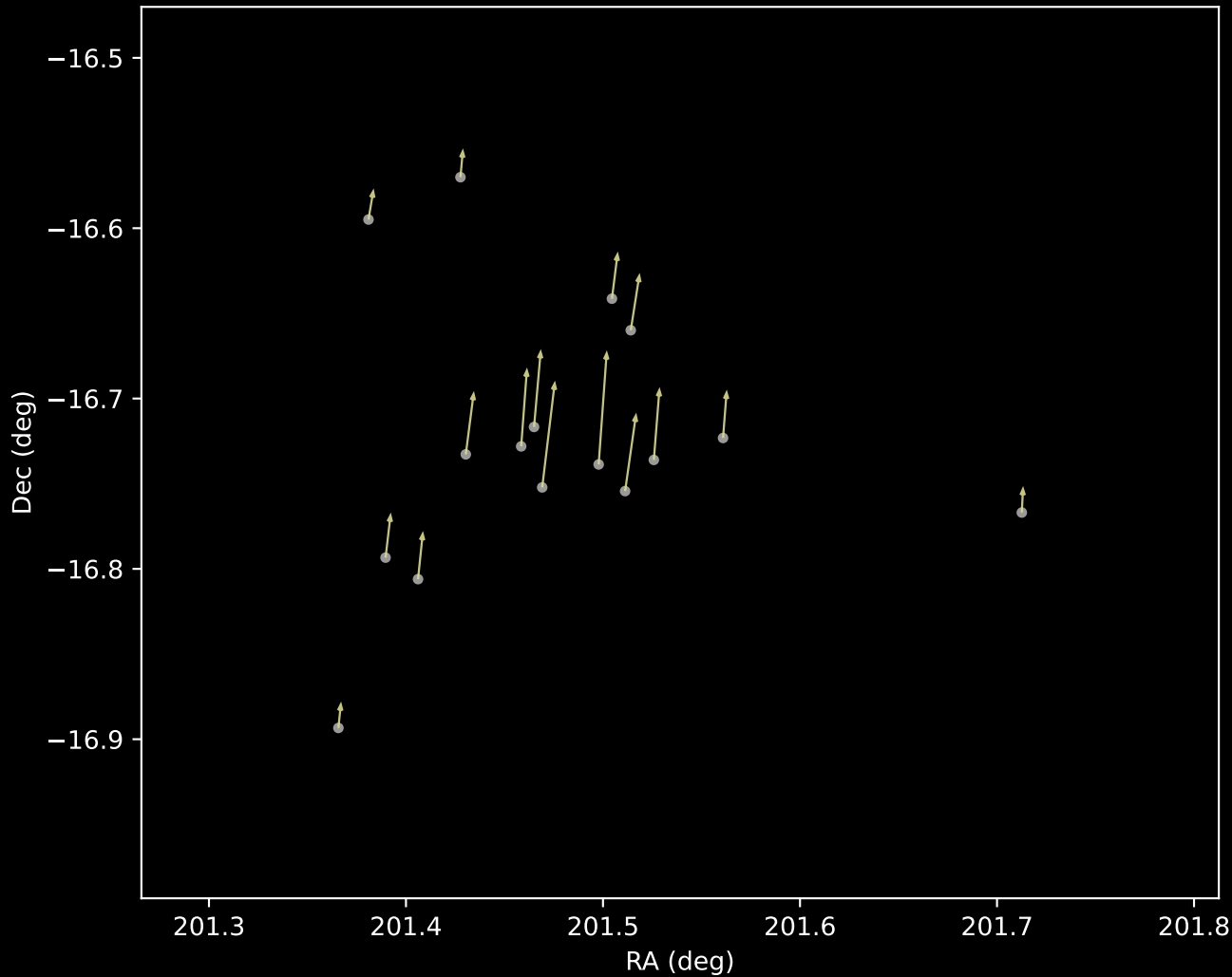
Gaia DR3 Cluster 17 Proper Motion Vectors (n=16)
