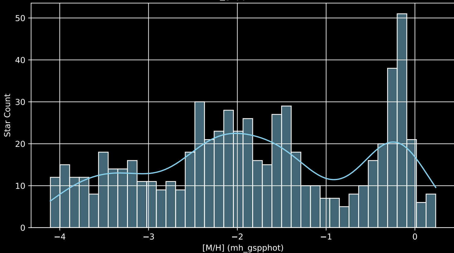
Gaia Cluster: [Gaia_1 [M/H] (mh_gspphot) (n= 663)
