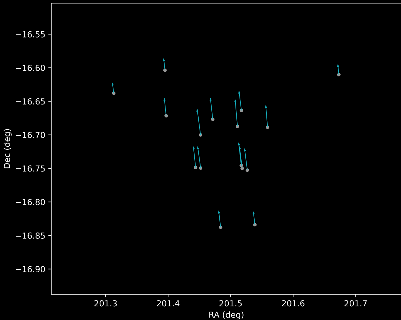
Gaia DR3 Cluster 18 Proper Motion Vectors (n=16)
