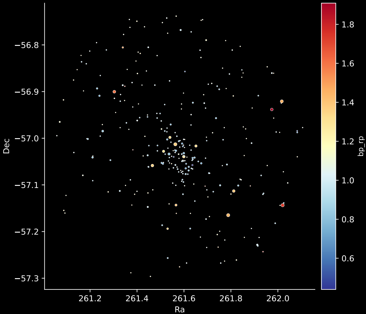
Gaia Cluster: [Gulliver_1] Stars: 291
