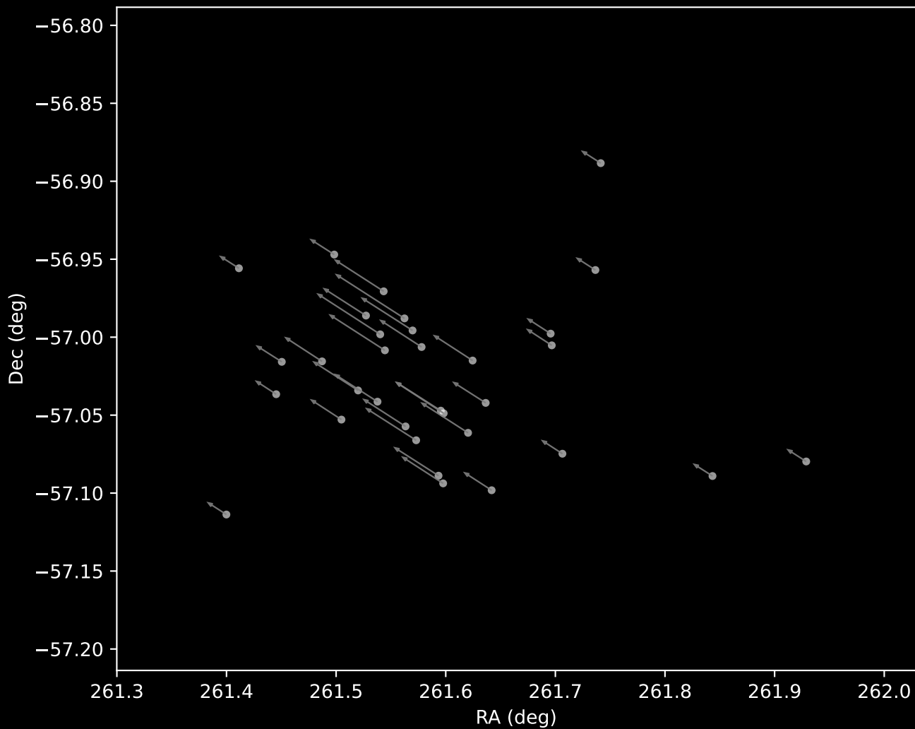
Gaia DR3 Cluster 14 Proper Motion Vectors (n=33)
