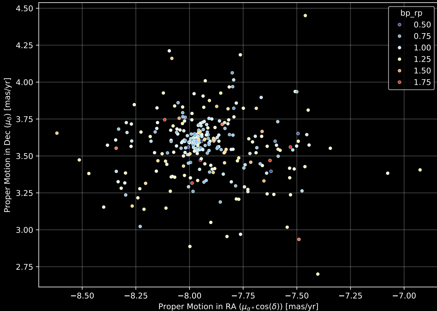
Gaia Cluster: [Gulliver_1] Proper Motion Diagram (n= 291)
