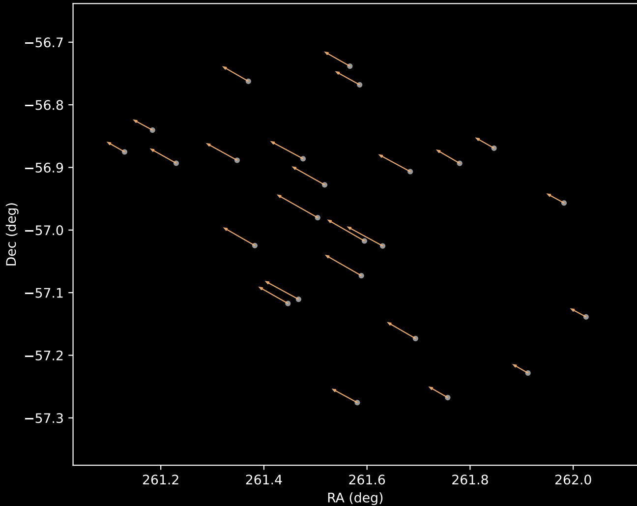
Gaia DR3 Cluster 3 Proper Motion Vectors (n=25)
