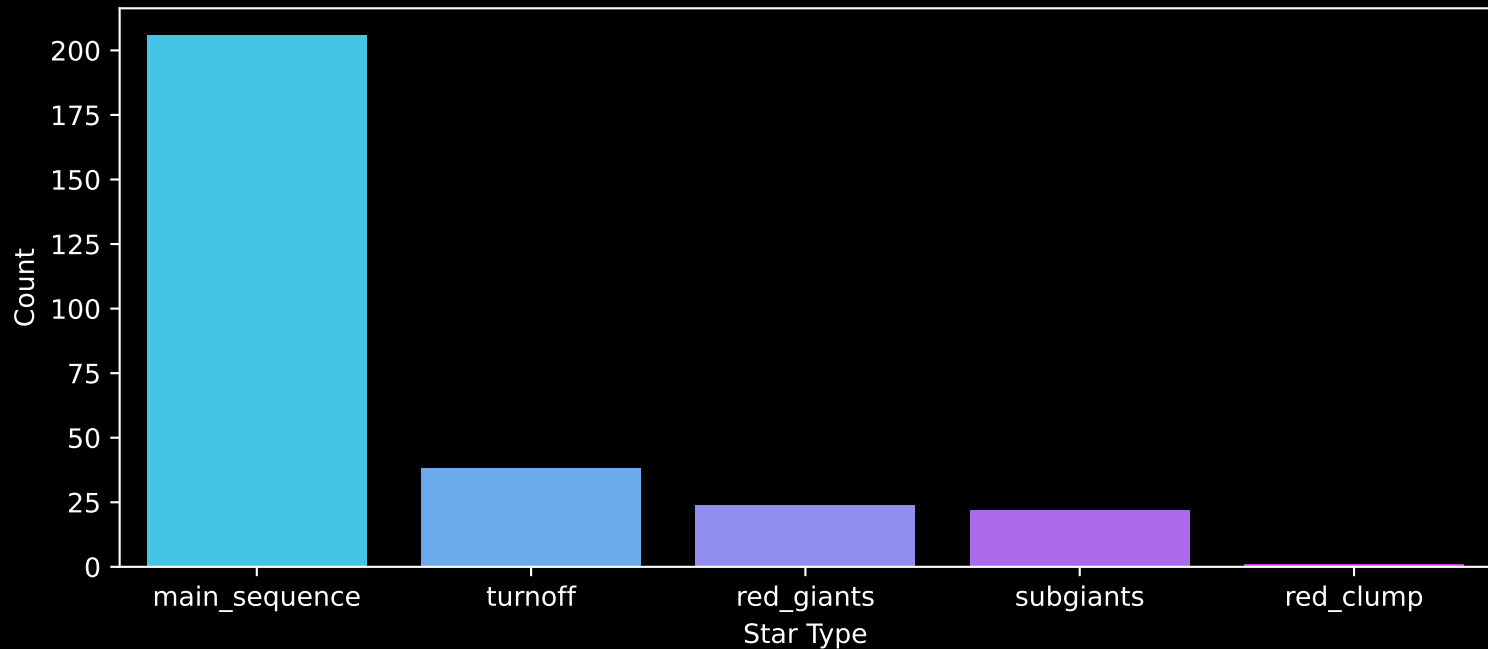
Gaia Cluster: [Gulliver_1] Count plot of Star Type
