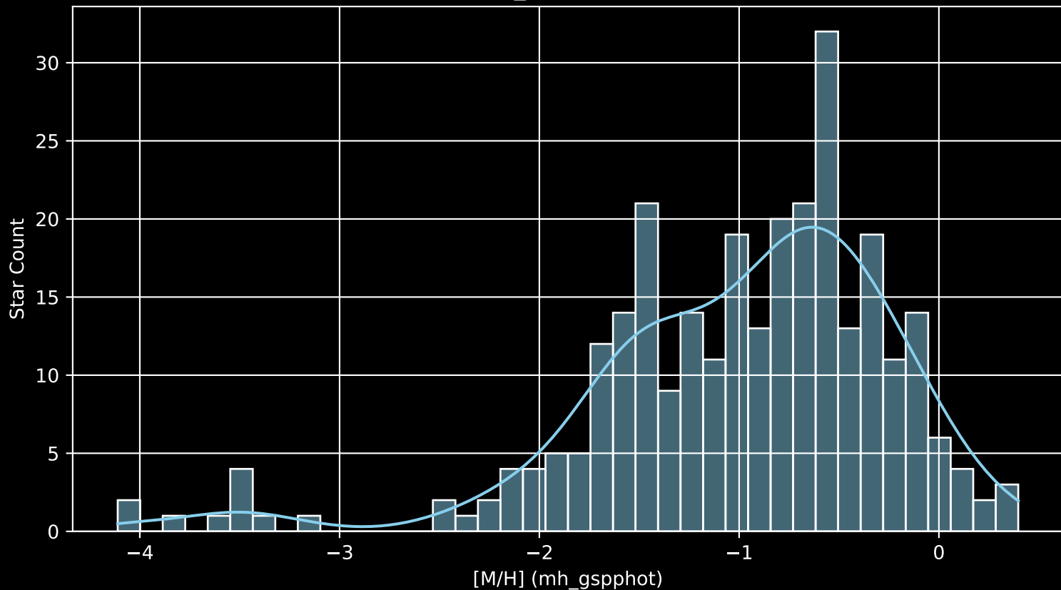
Gaia Cluster: [Gulliver_1 [M/H] (mh_gspphot) (n= 291)
