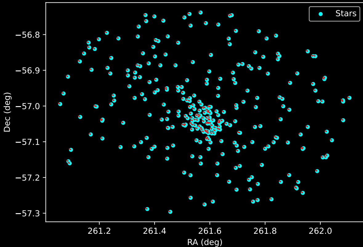
Gaia Cluster: [Gulliver_1] Proper Motion Vectors for Gaia Star Field (n= 291)
