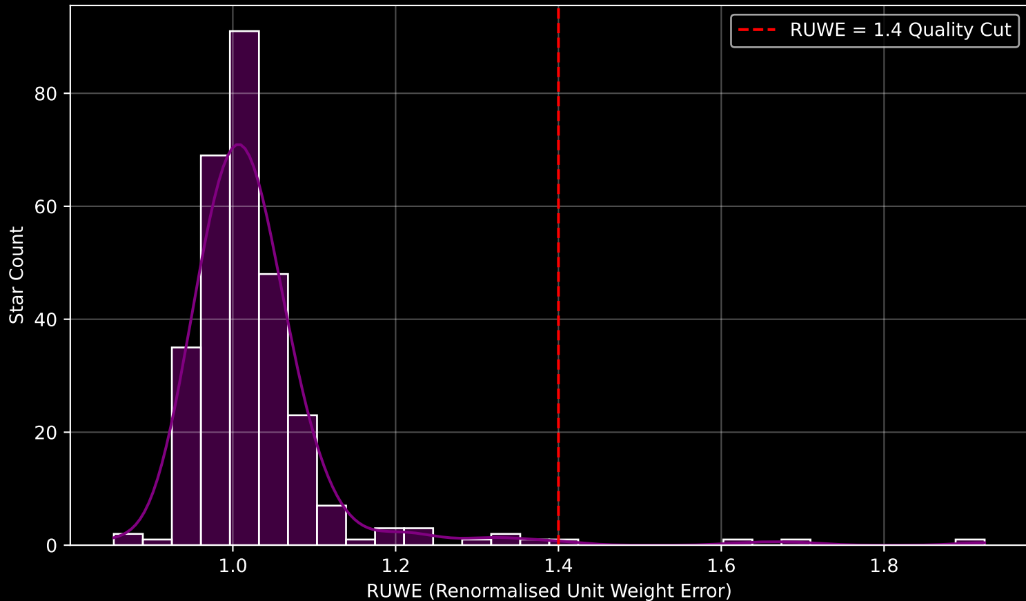
Gaia Cluster: [Gulliver_1] RUWE Distribution (n= 291)
