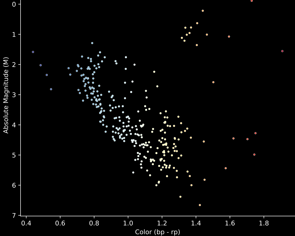
Gaia Cluster: [Gulliver_1] Stars (n= 291) Hertzprung-Russel Diagram
