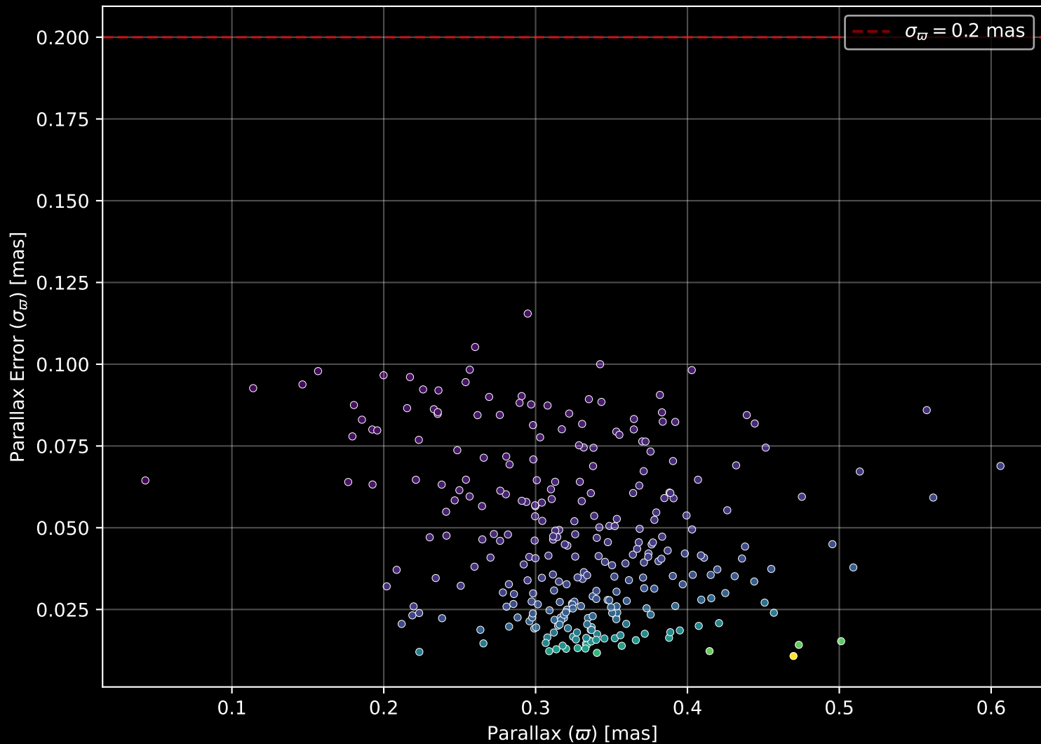
Gaia Cluster: [Gulliver_1] Parallax Quality (n= 291)
