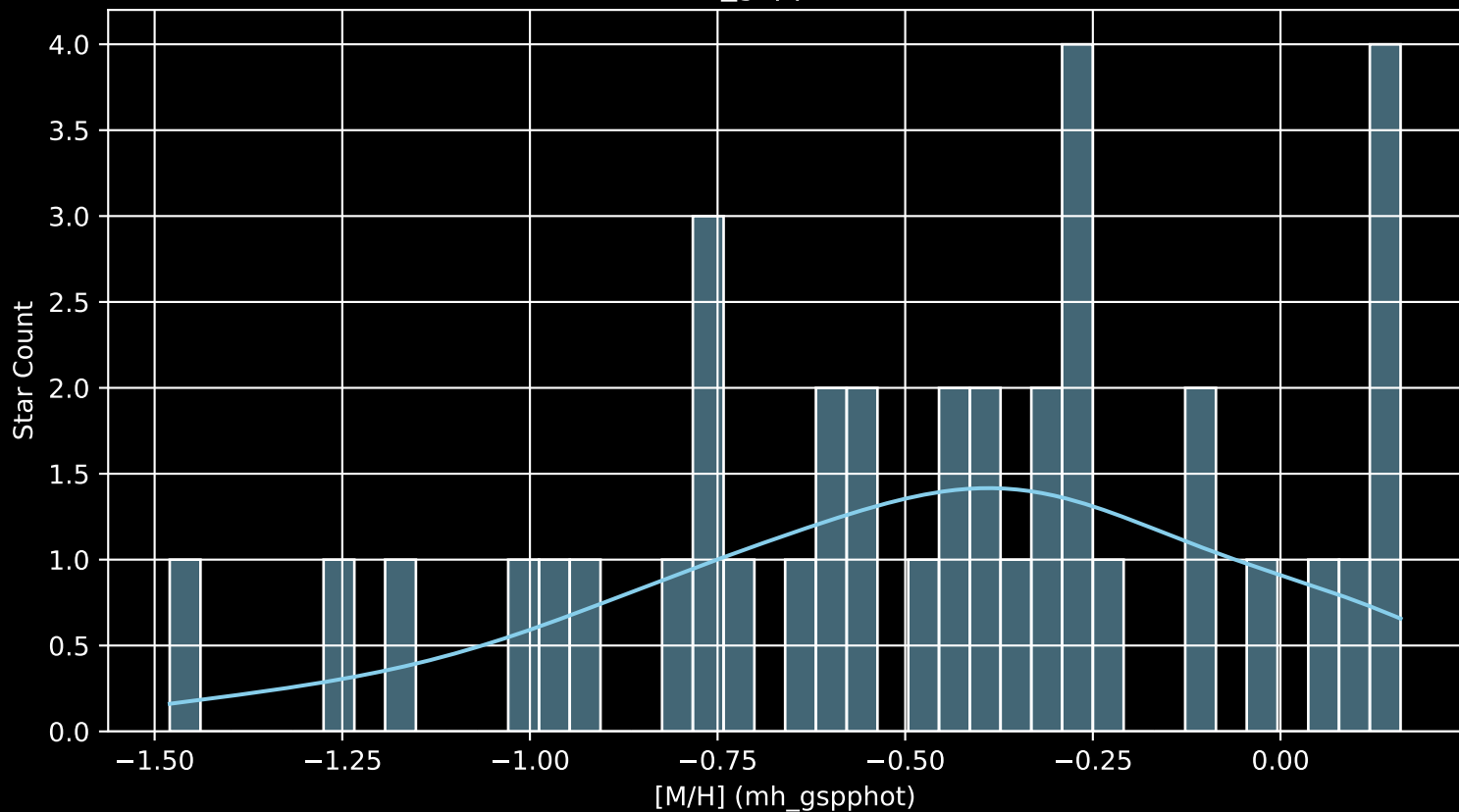
Gaia Cluster: [Gulliver_10 [M/H] (mh_gspphot) (n= 38)
