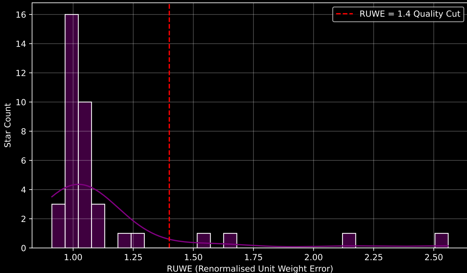
Gaia Cluster: [Gulliver_10] RUWE Distribution (n= 38)
