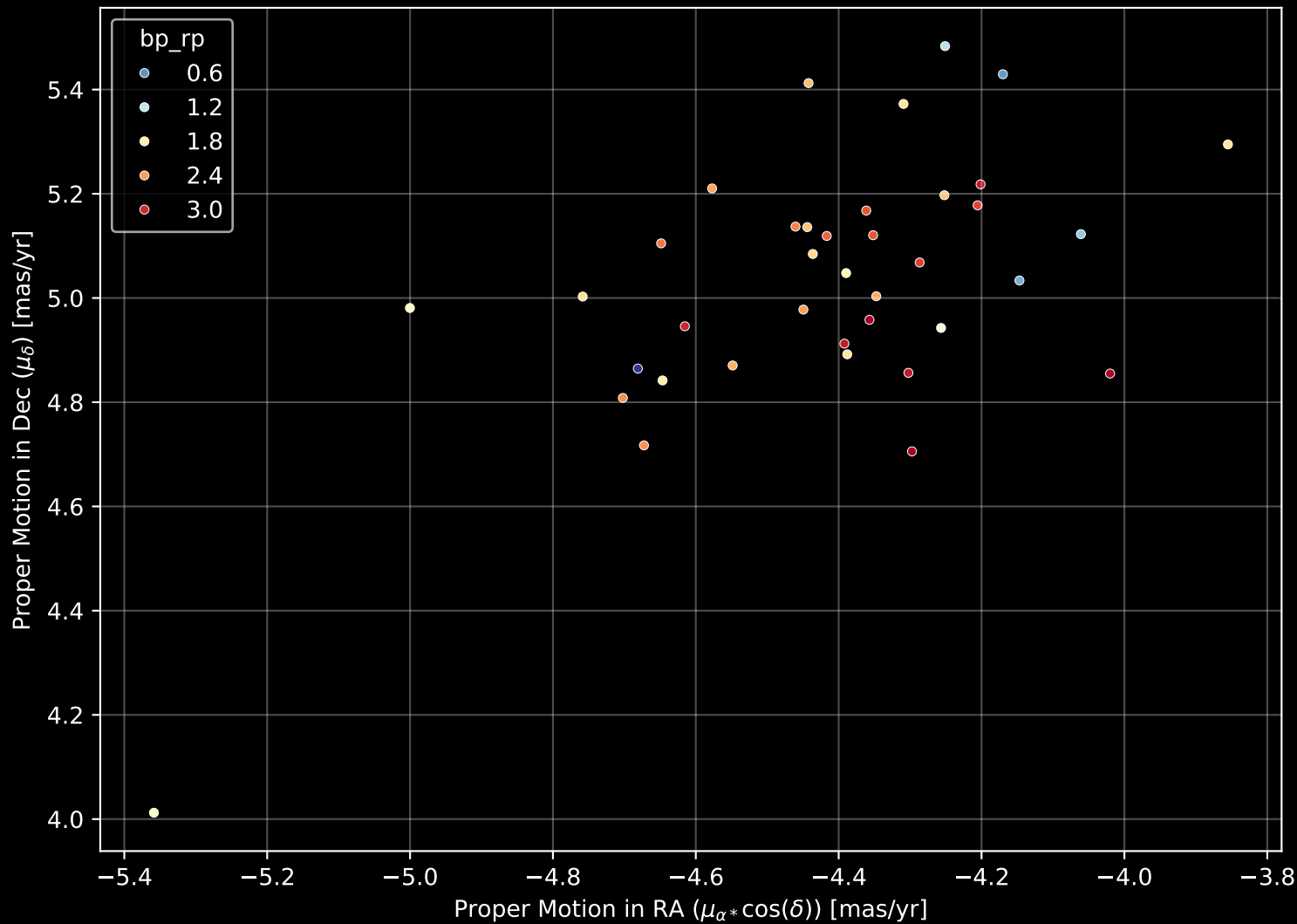
Gaia Cluster: [Gulliver_10] Proper Motion Diagram (n= 38)
