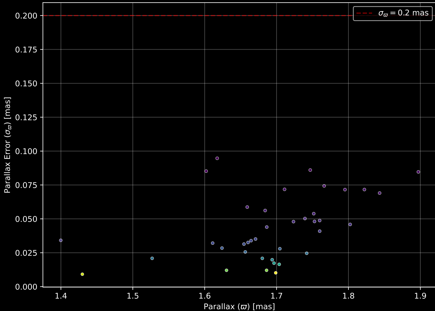
Gaia Cluster: [Gulliver_10] Parallax Quality (n= 38)
