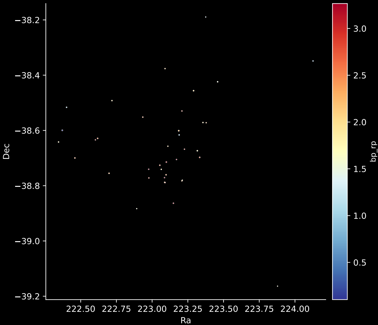
Gaia Cluster: [Gulliver_10] Stars: 38
