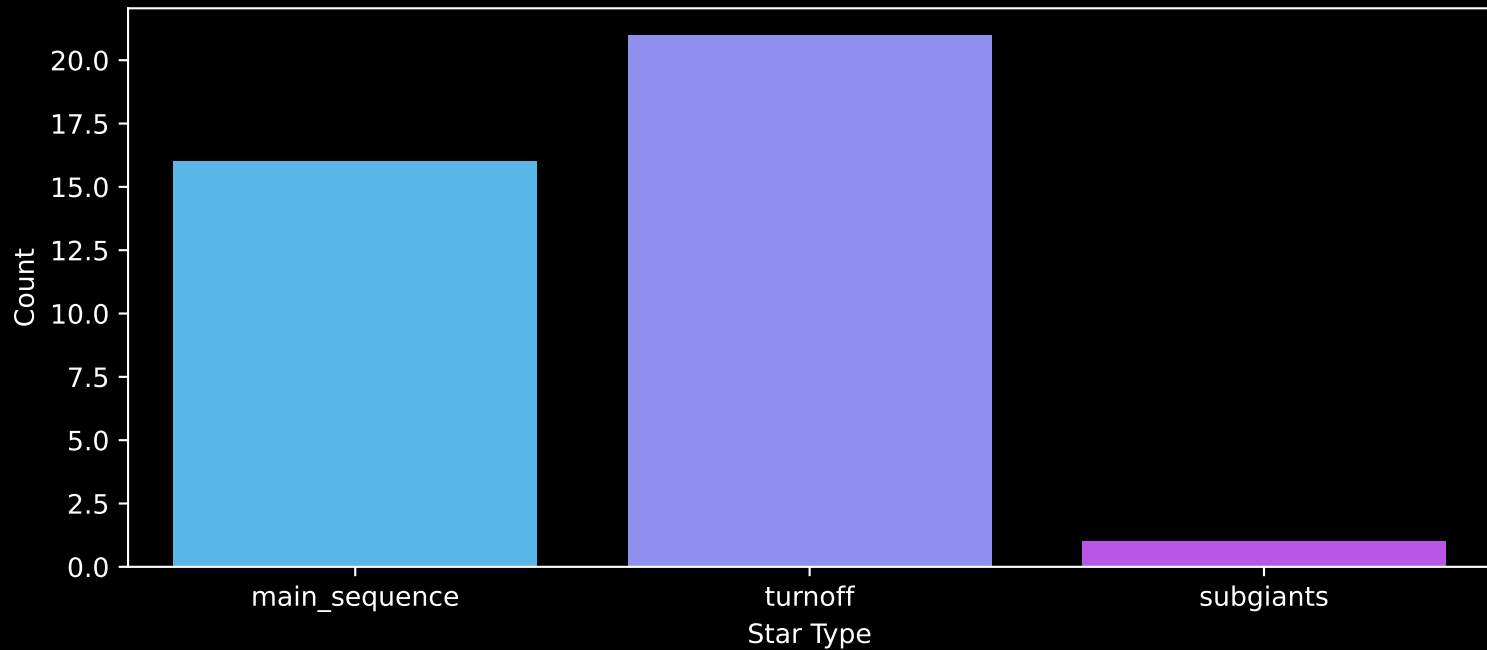
Gaia Cluster: [Gulliver_10] Count plot of Star Type
