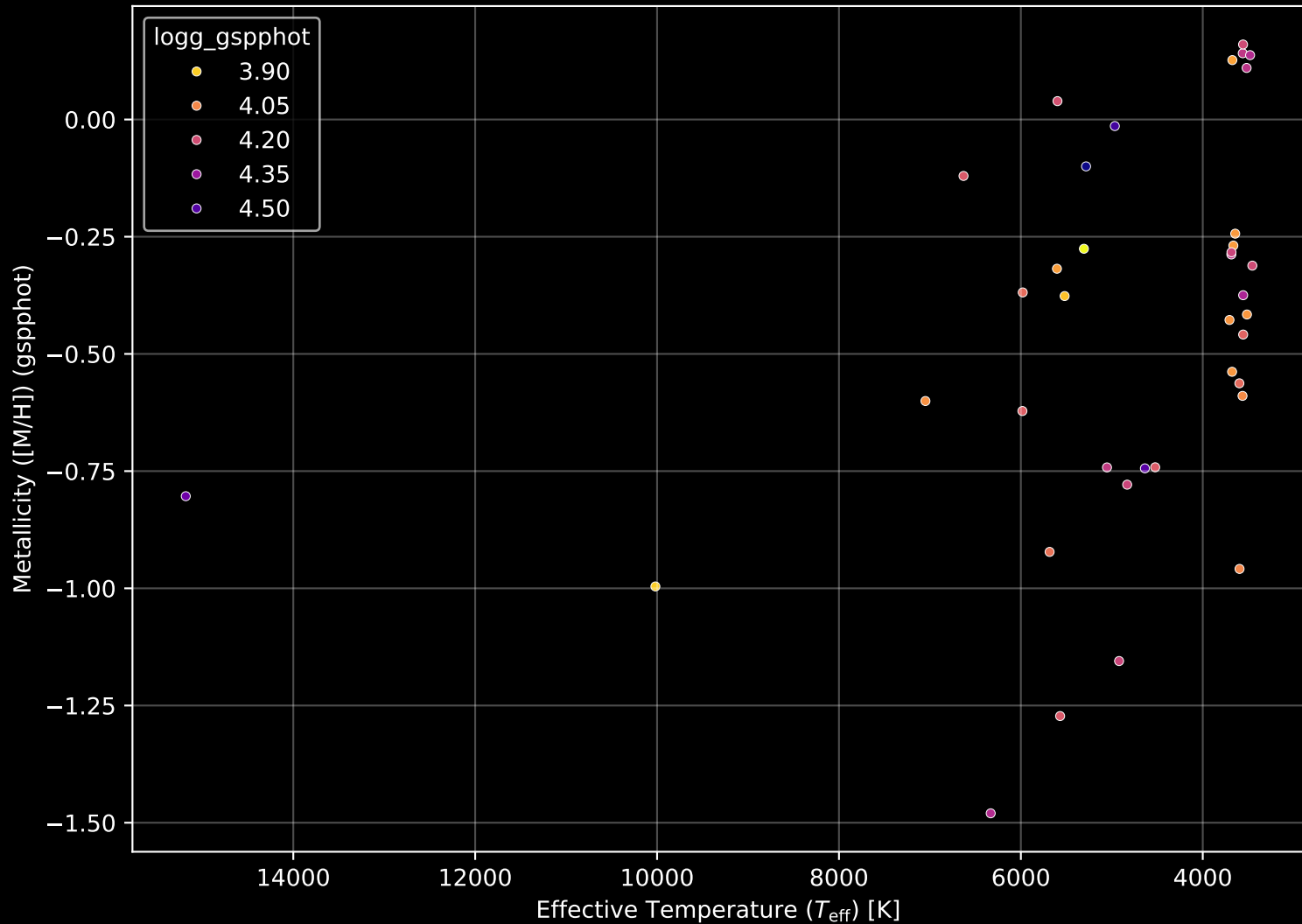
Gaia Cluster: [Gulliver_10] Stellar Population Parameters (n= 38)
