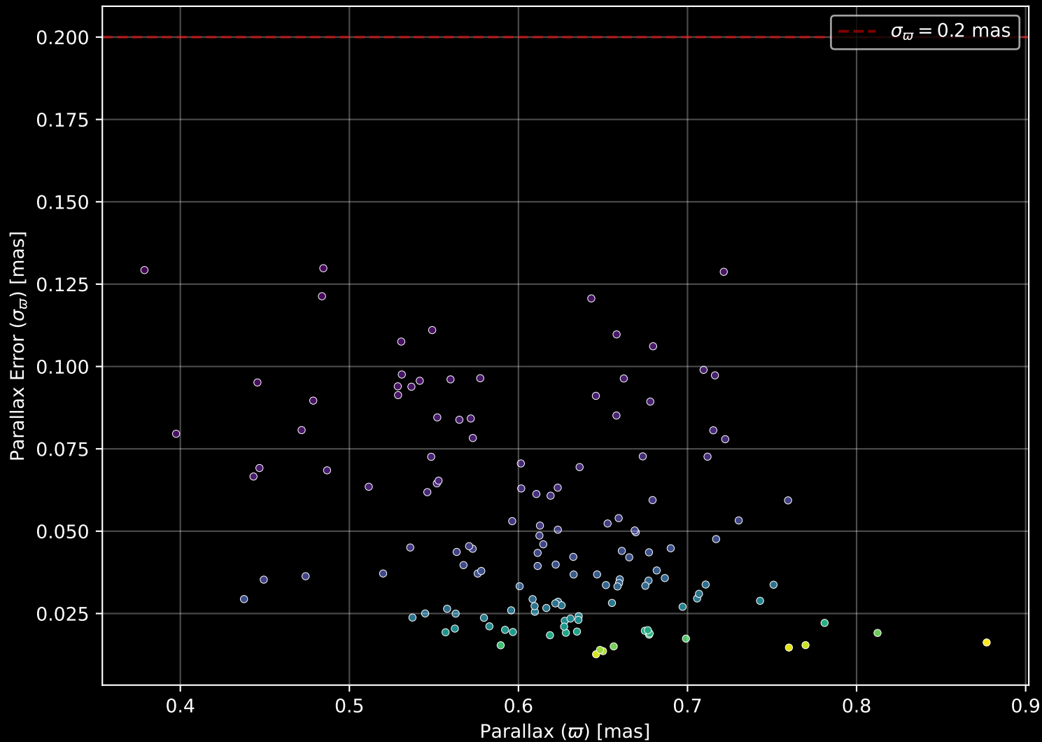
Gaia Cluster: [Gulliver_13] Parallax Quality (n= 139)
