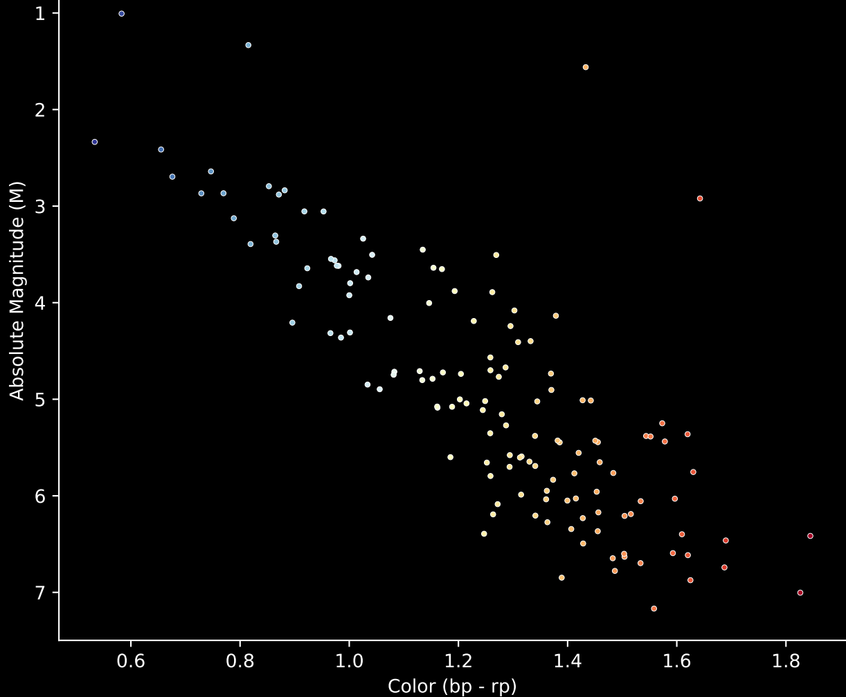
Gaia Cluster: [Gulliver_13] Stars (n= 139) Hertzsprung-Russel Diagram
