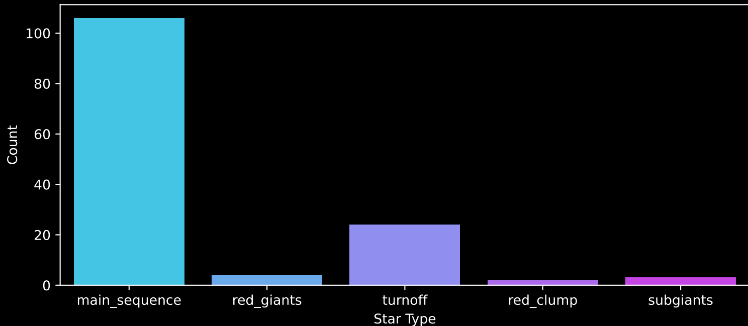
Gaia Cluster: [Gulliver_13] Count plot of Star Type
