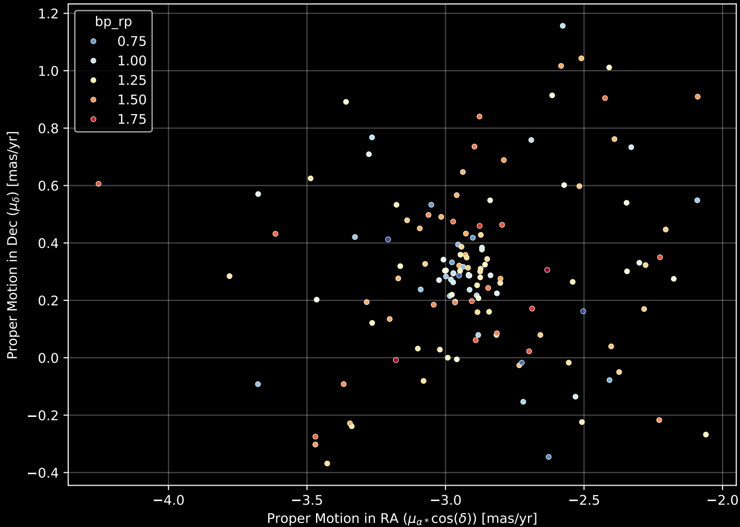
Gaia Cluster: [Gulliver_13] Proper Motion Diagram (n= 139)
