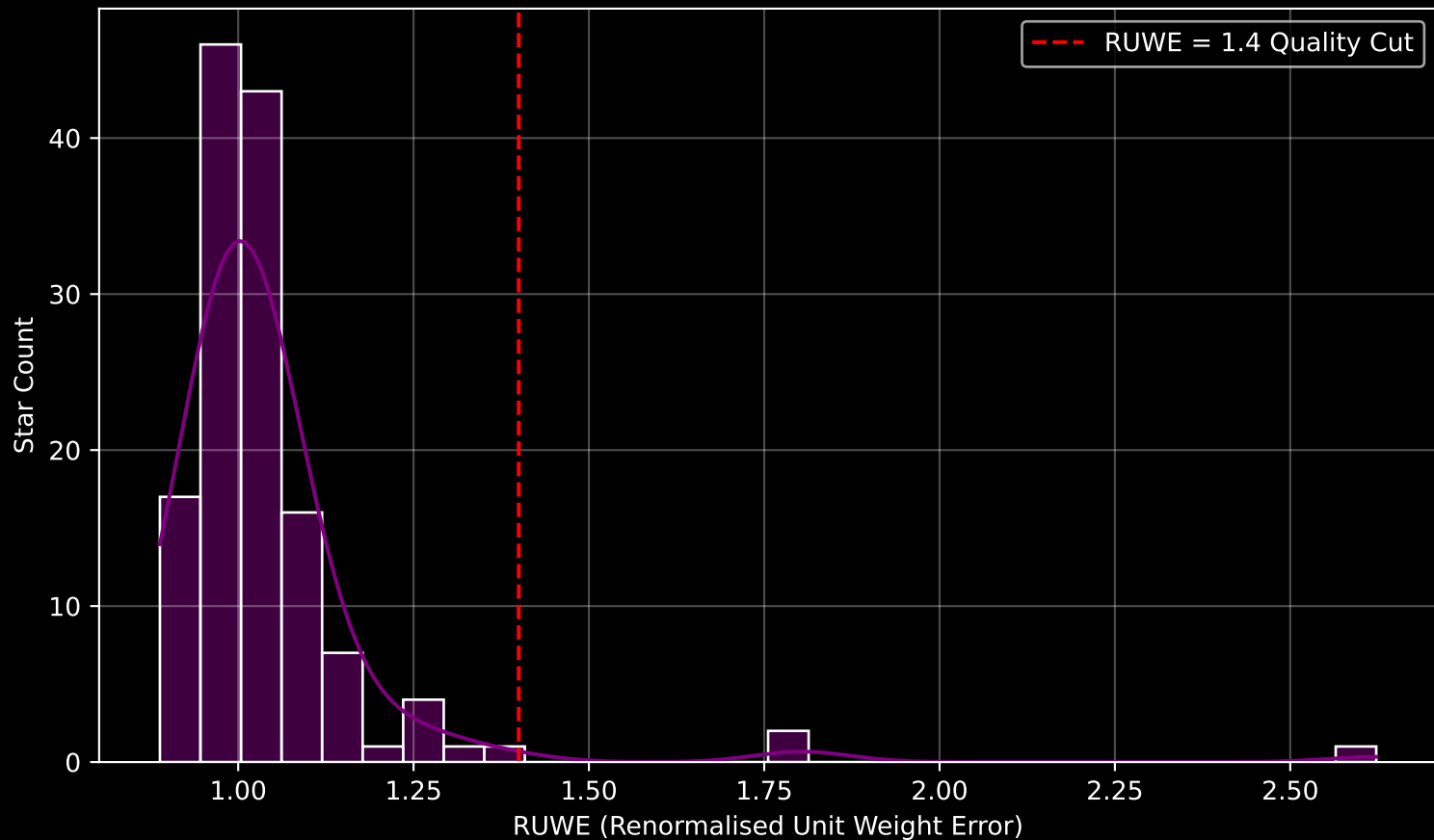
Gaia Cluster: [Gulliver_13] RUWE Distribution (n= 139)
