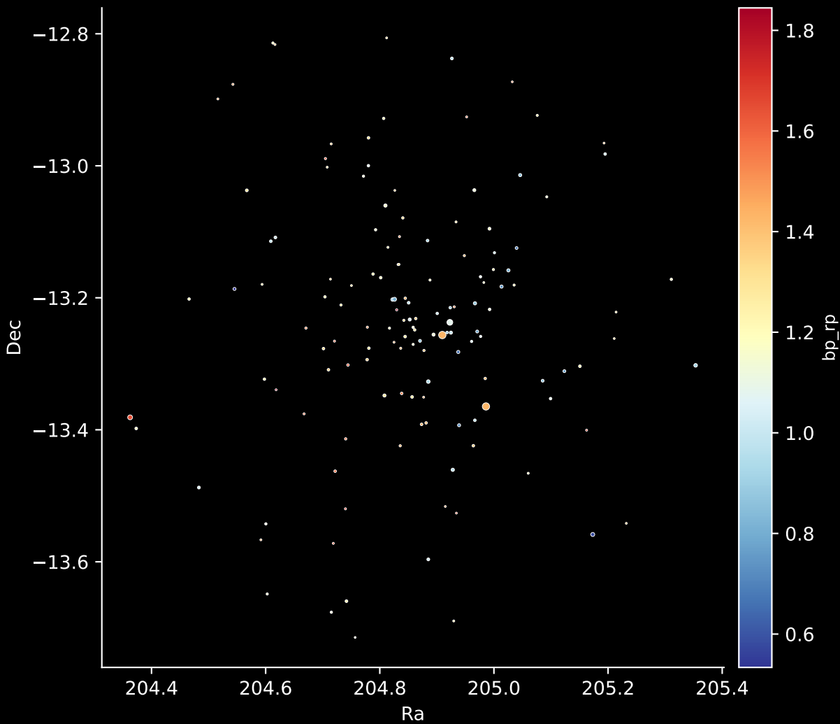
Gaia Cluster: [Gulliver_13] Stars: 139
