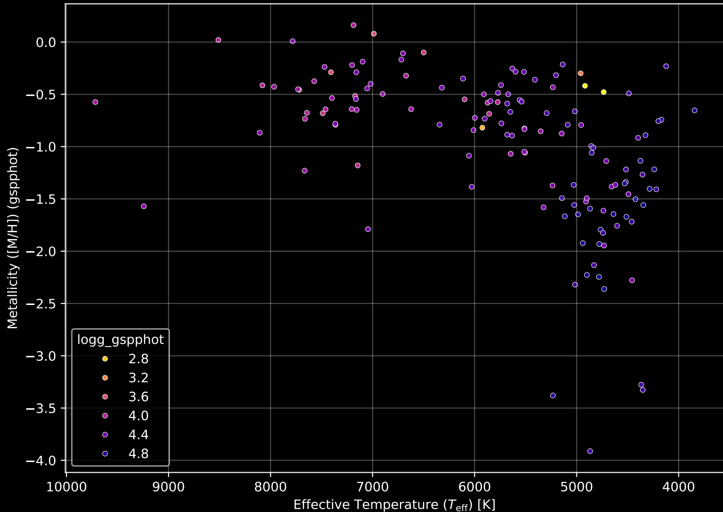
Gaia Cluster: [Gulliver_13] Stellar Population Parameters (n= 139)
