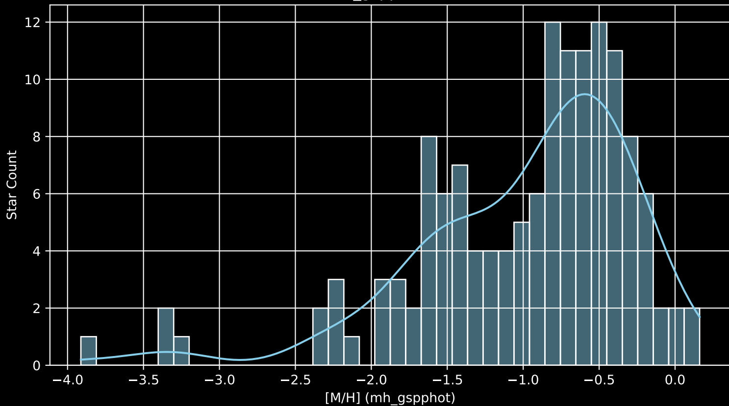
Gaia Cluster: [Gulliver_13 [M/H] (mh_gspphot) (n= 139)
