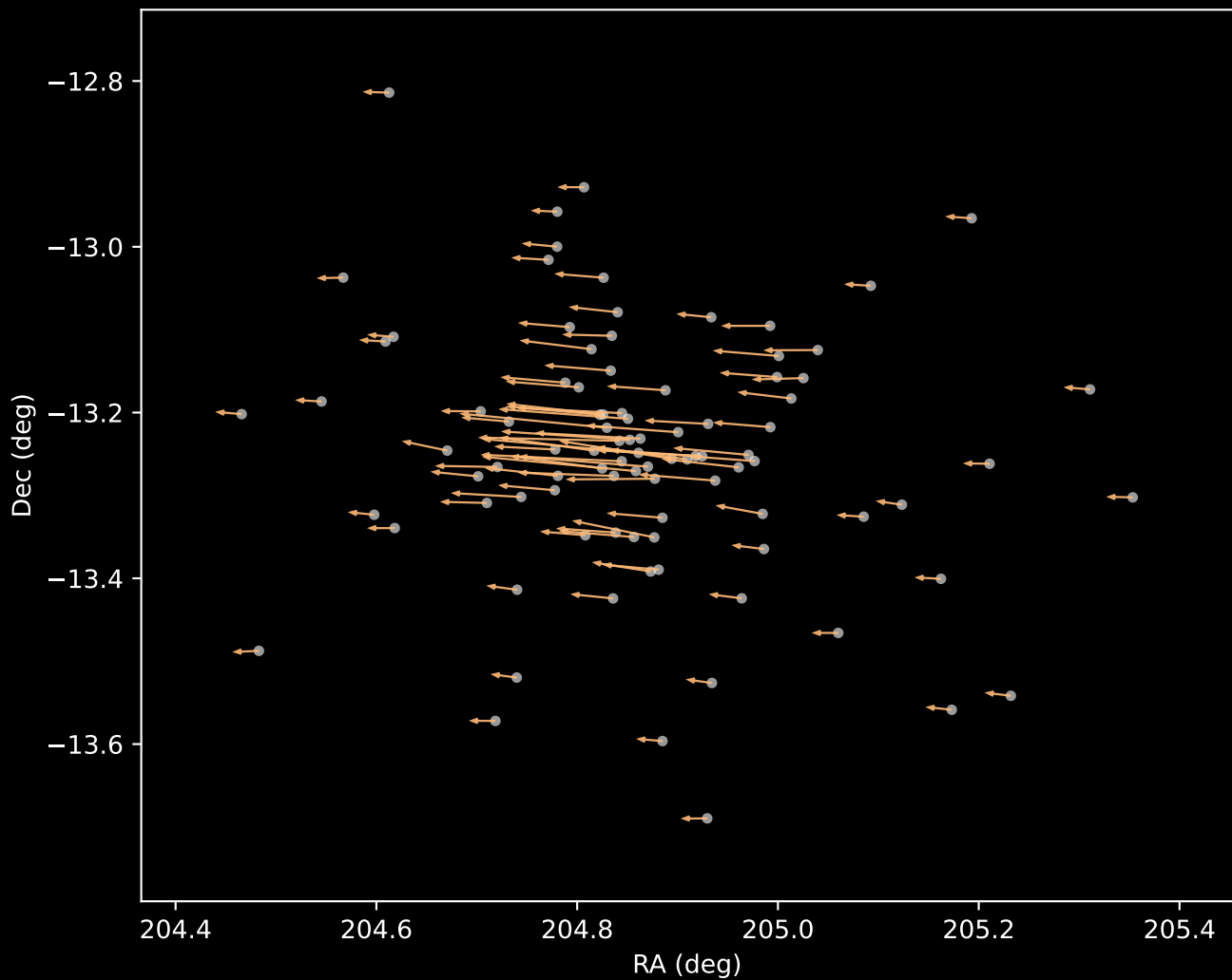
Gaia DR3 Cluster 3 Proper Motion Vectors (n=94)
