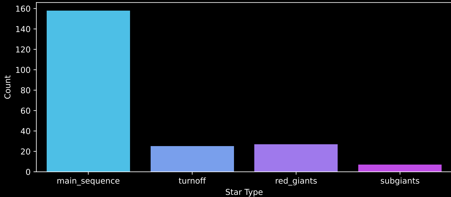
Gaia Cluster: [Gulliver_16] Count plot of Star Type
