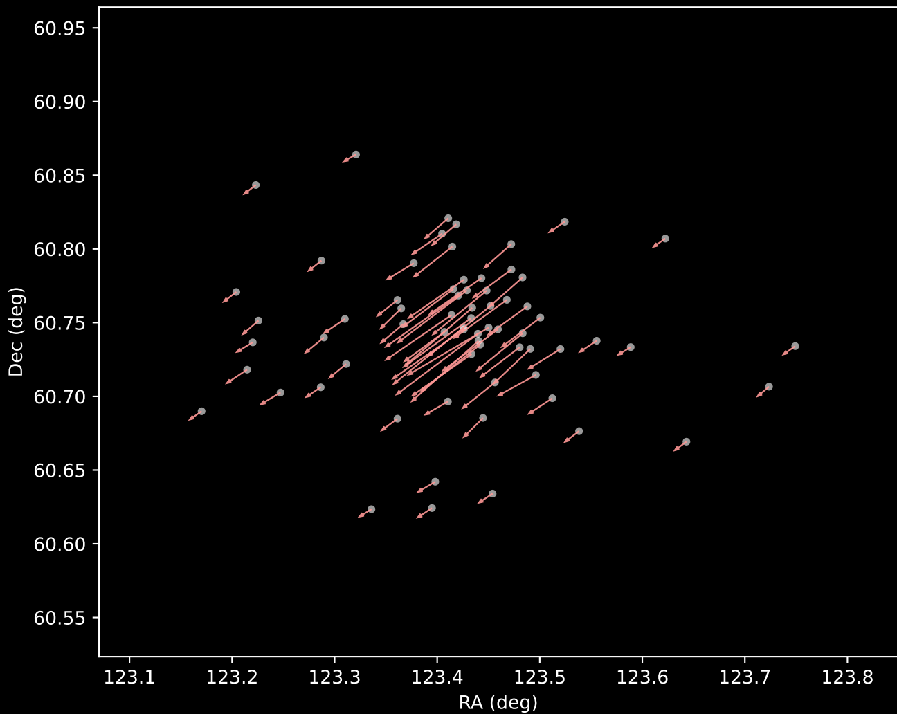
Gaia DR3 Cluster 7 Proper Motion Vectors (n=68)
