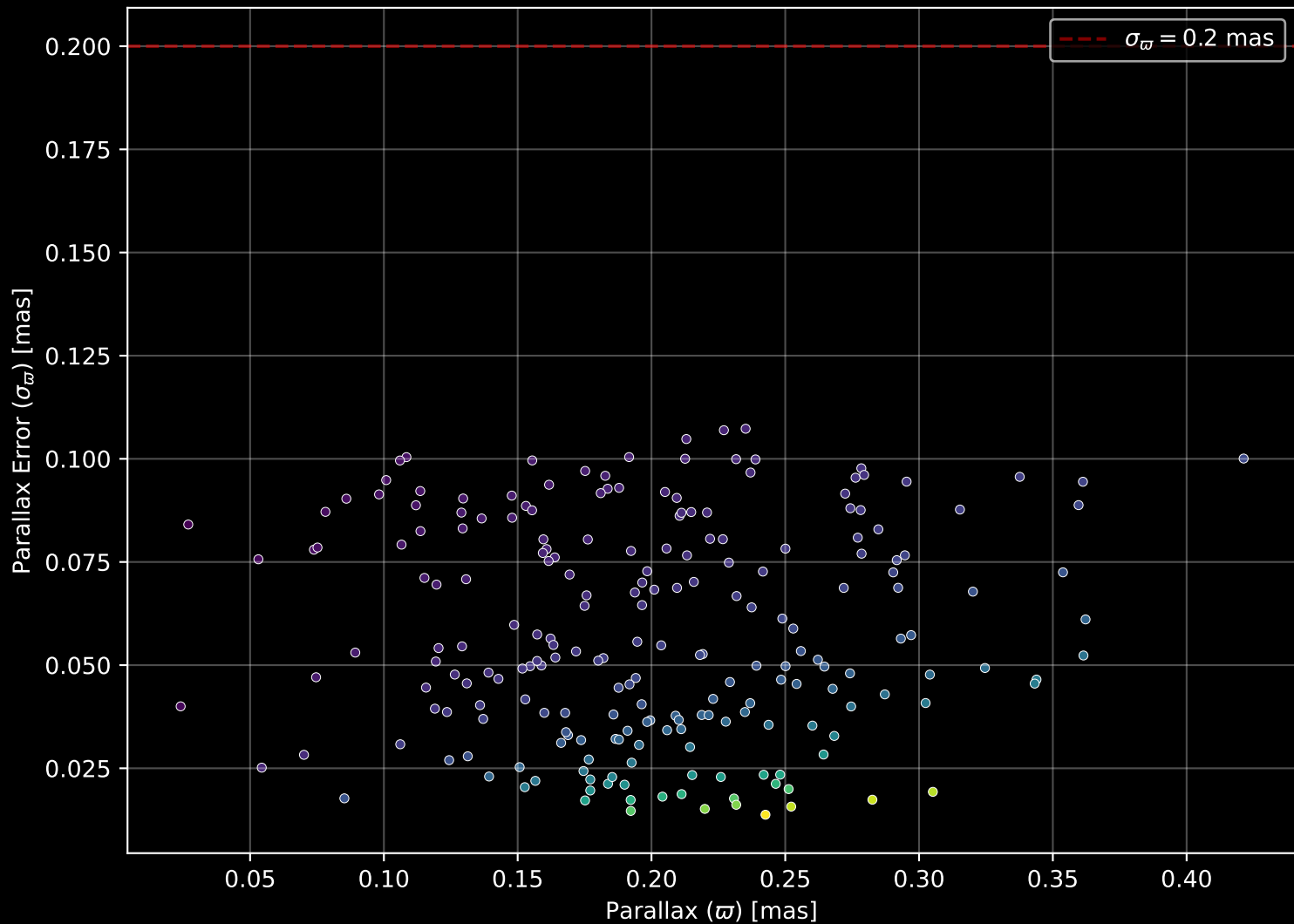
Gaia Cluster: [Gulliver_16] Parallax Quality (n= 217)
