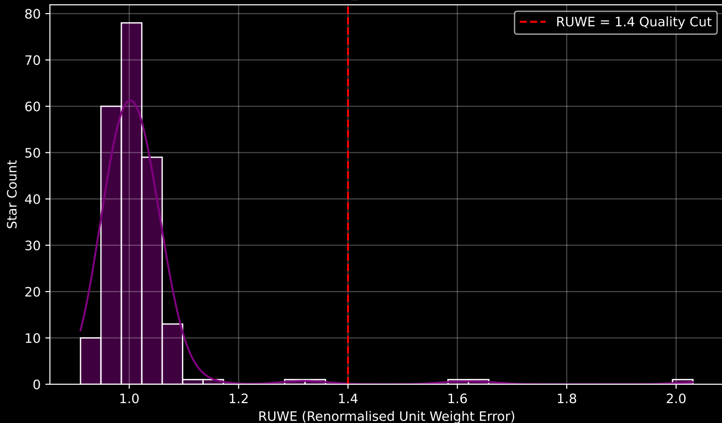
Gaia Cluster: [Gulliver_16] RUWE Distribution (n= 217)
