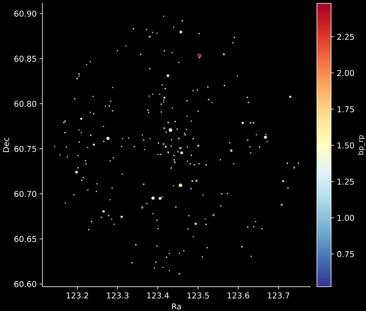
Gaia Cluster: [Gulliver_16] Stars: 217
