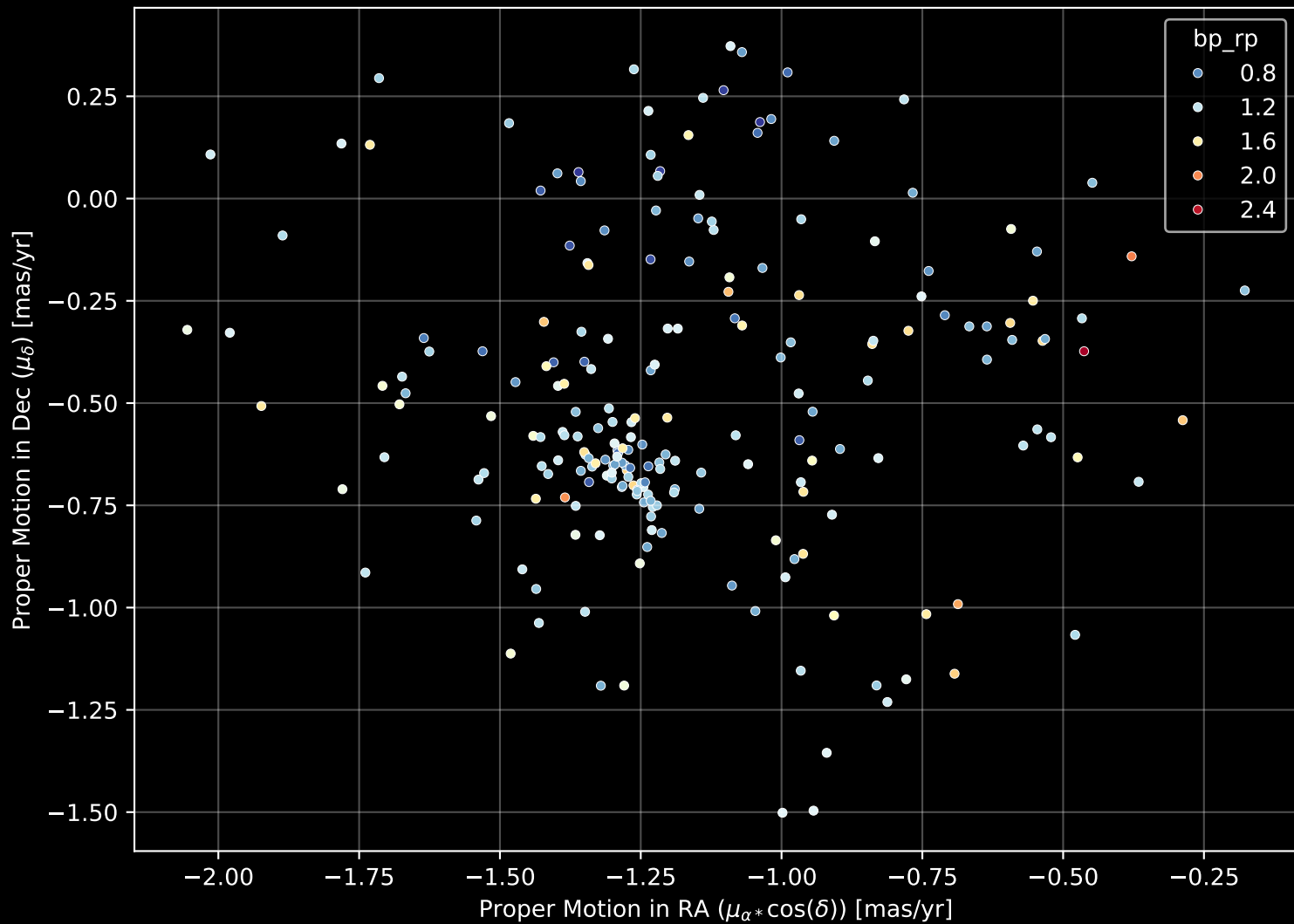
Gaia Cluster: [Gulliver_16] Proper Motion Diagram (n= 217)
