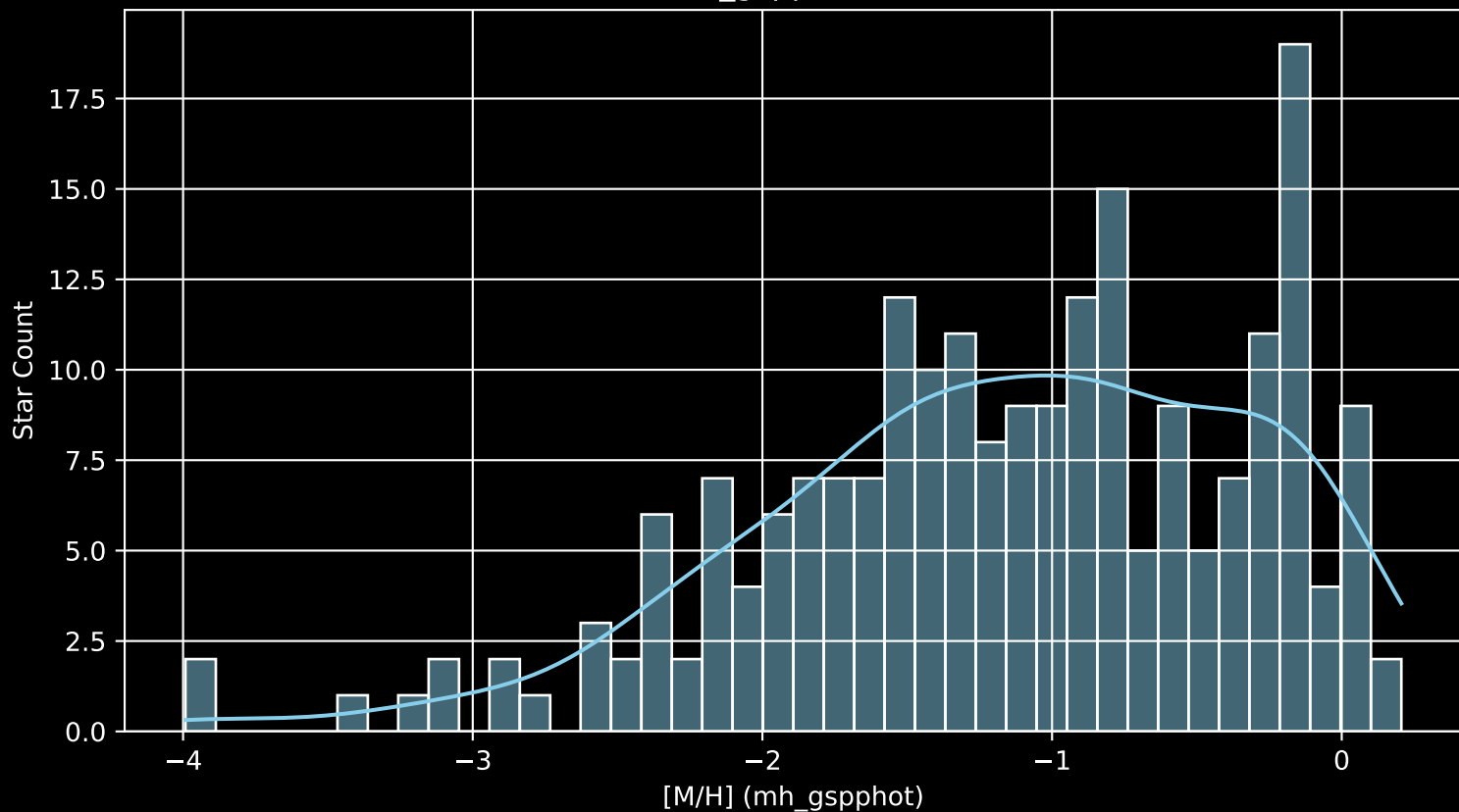
Gaia Cluster: [Gulliver_16 [M/H] (mh_gspphot) (n= 217)
