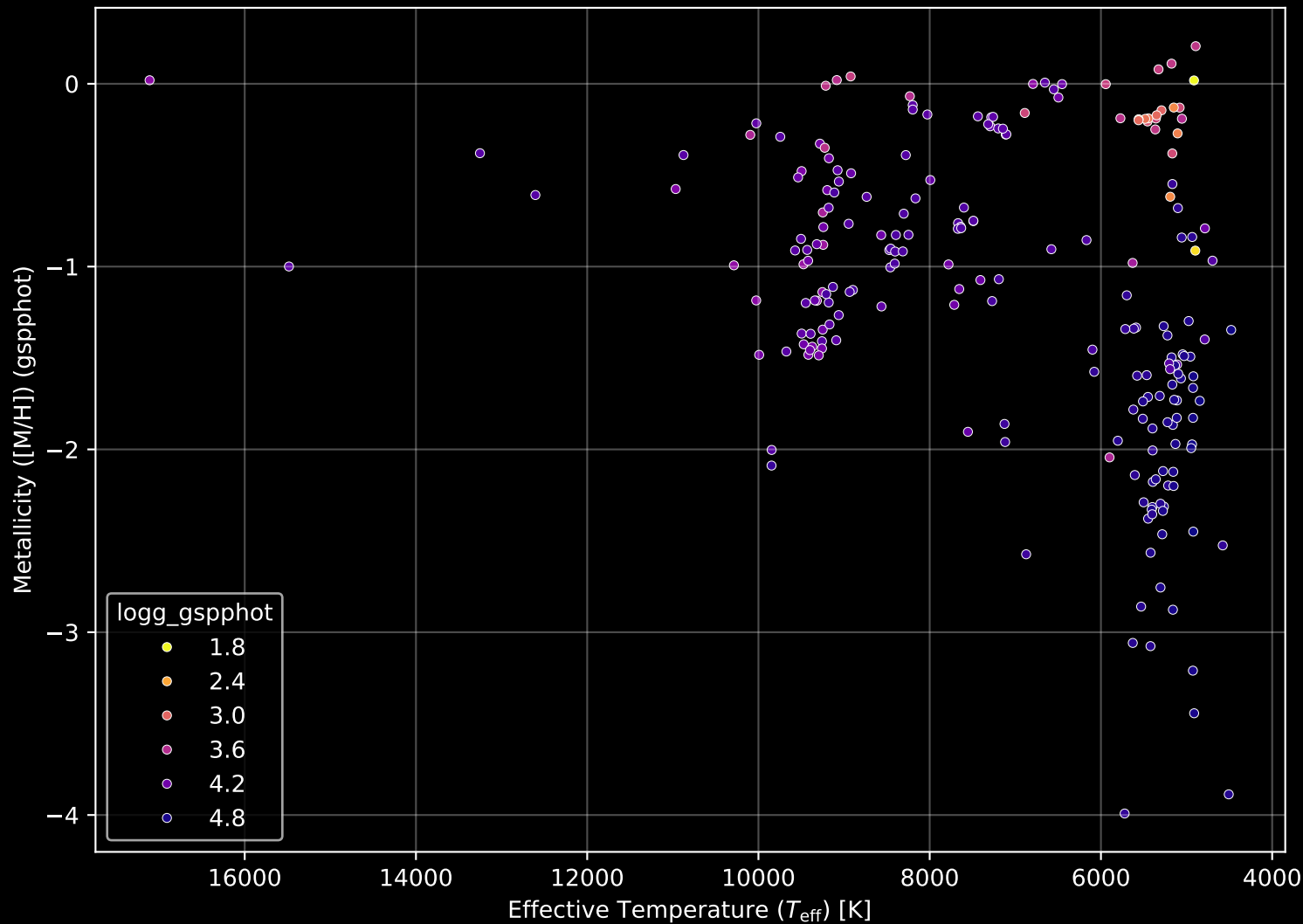
Gaia Cluster: [Gulliver_16] Stellar Population Parameters (n= 217)
