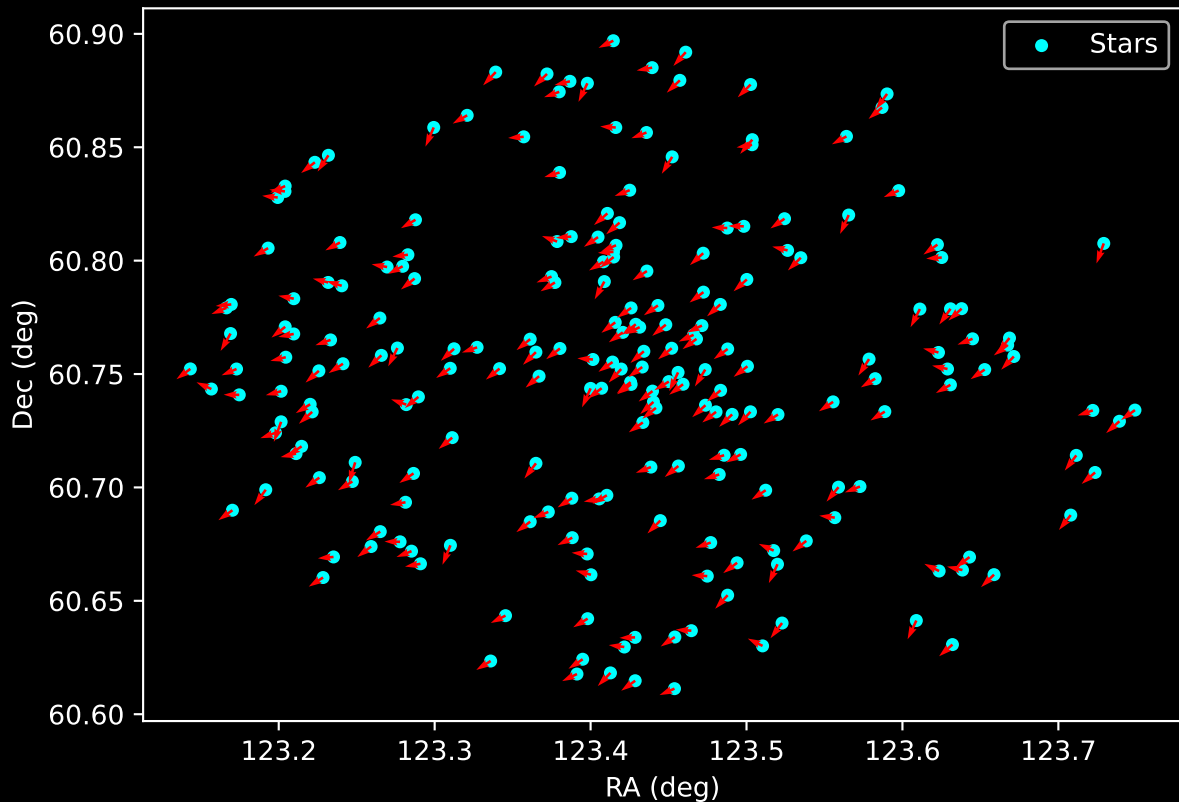
Gaia Cluster: [Gulliver_16] Proper Motion Vectors for Gaia Star Field (n= 217)
