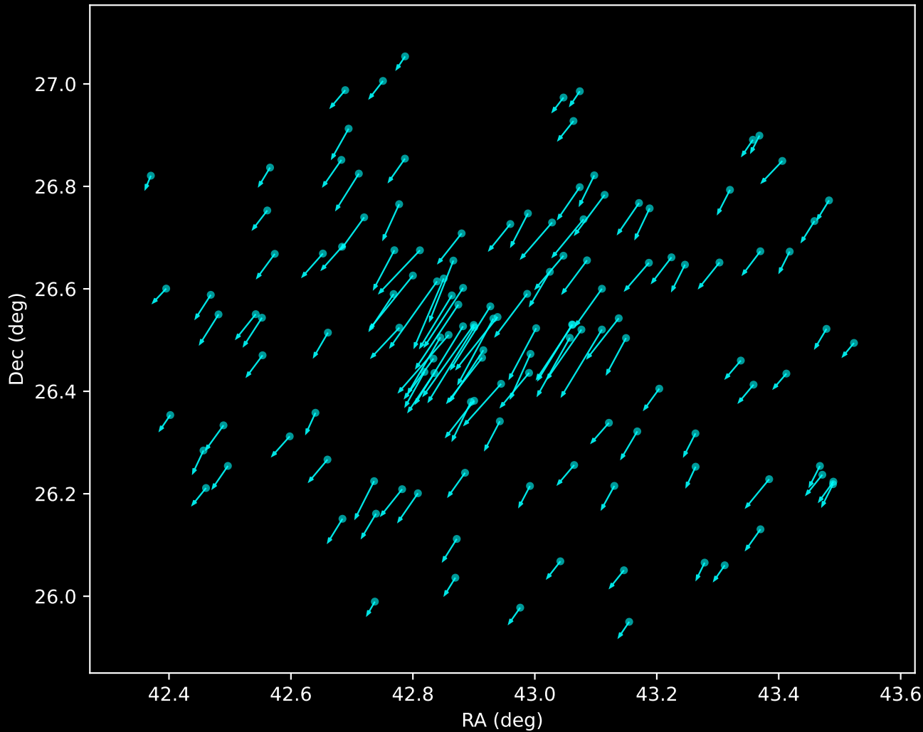
Gaia DR3 Noise Stream Proper Motion Vectors (n=132)
