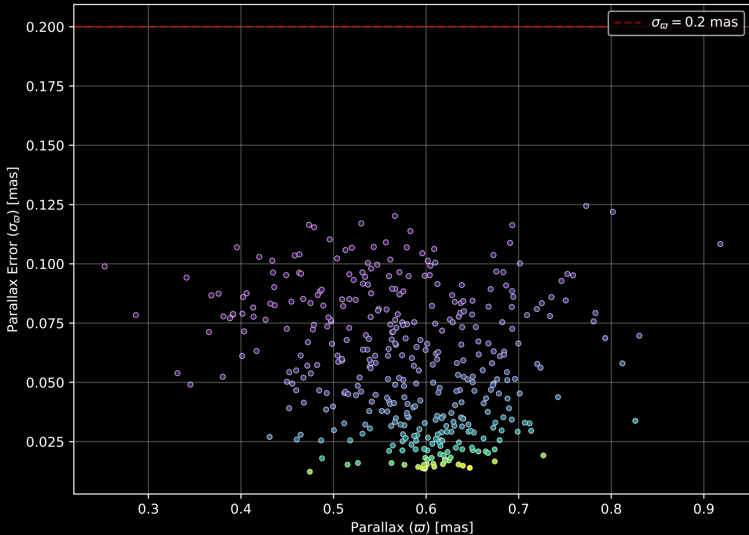
Gaia Cluster: [Gulliver_18] Parallax Quality (n= 385)
