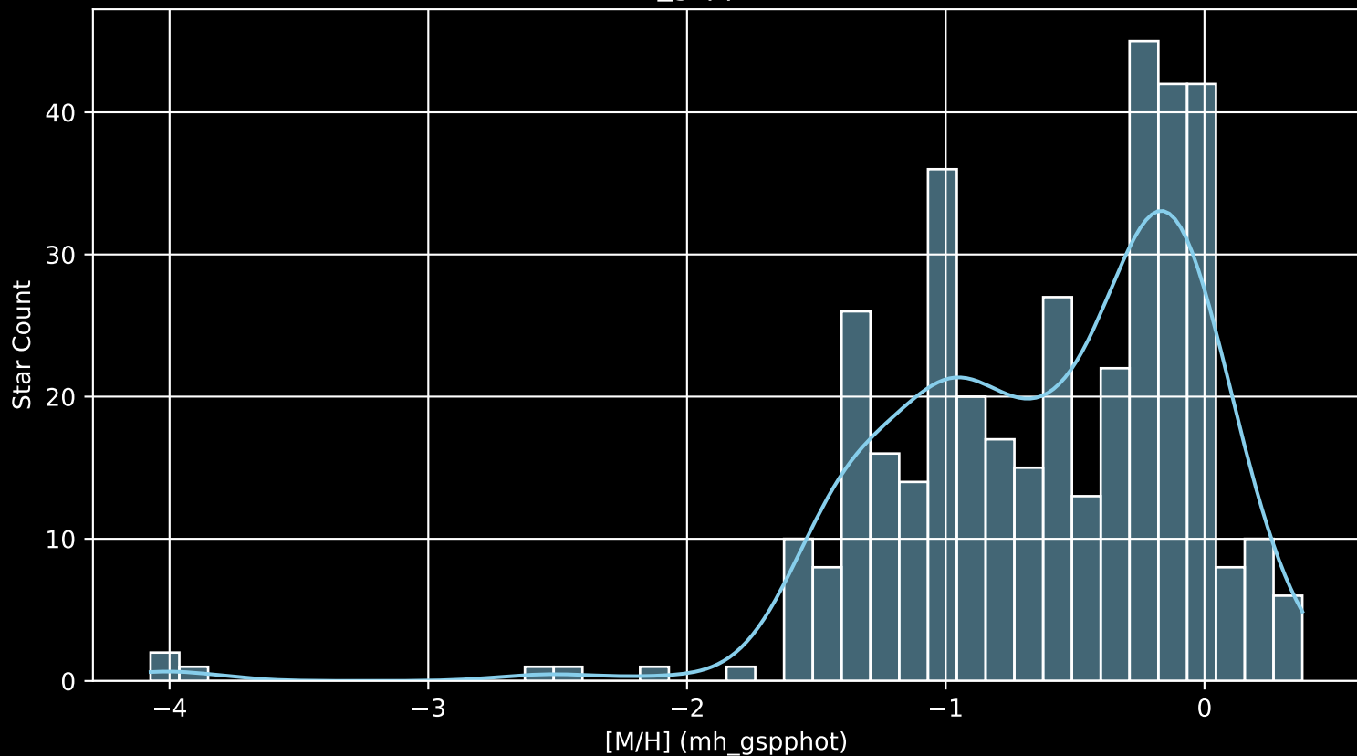
Gaia Cluster: [Gulliver_18 [M/H] (mh_gspphot) (n= 384)
