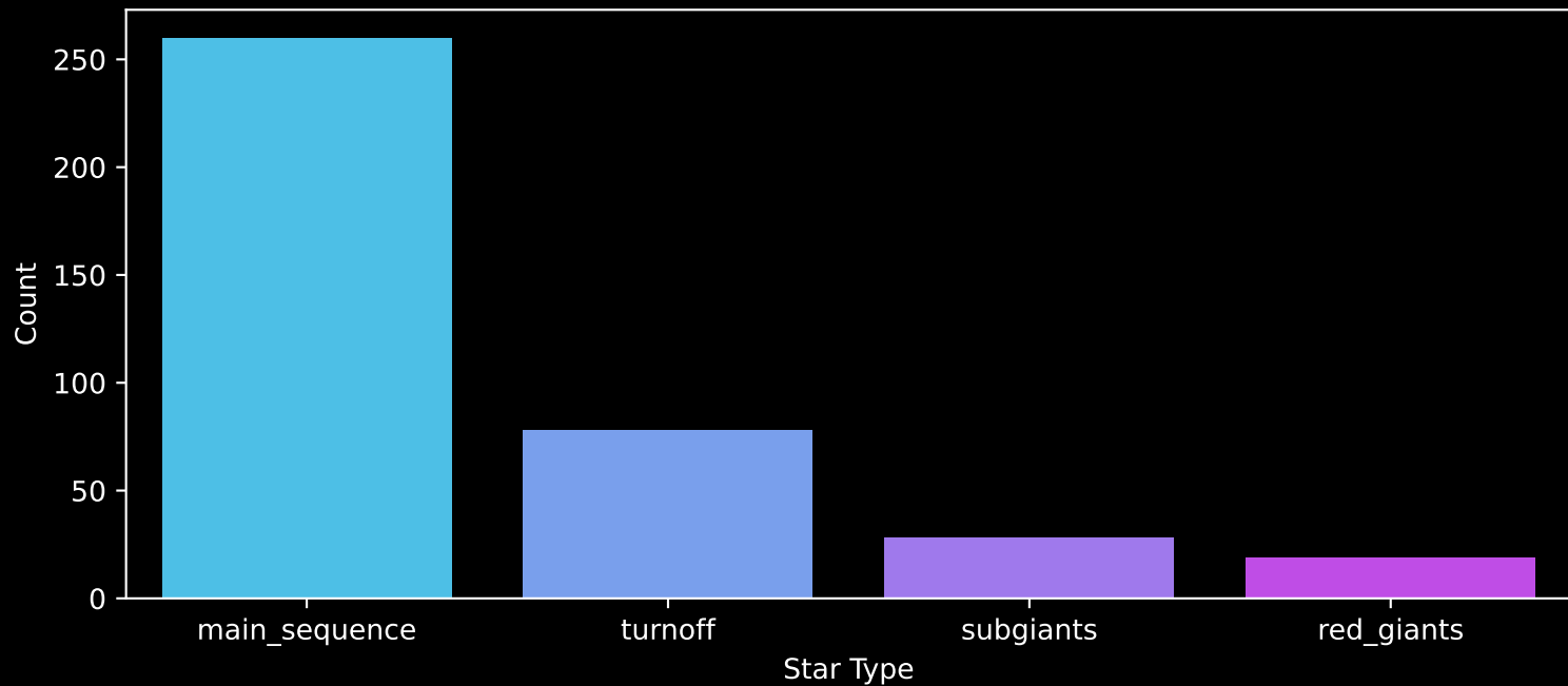
Gaia Cluster: [Gulliver_18] Count plot of Star Type
