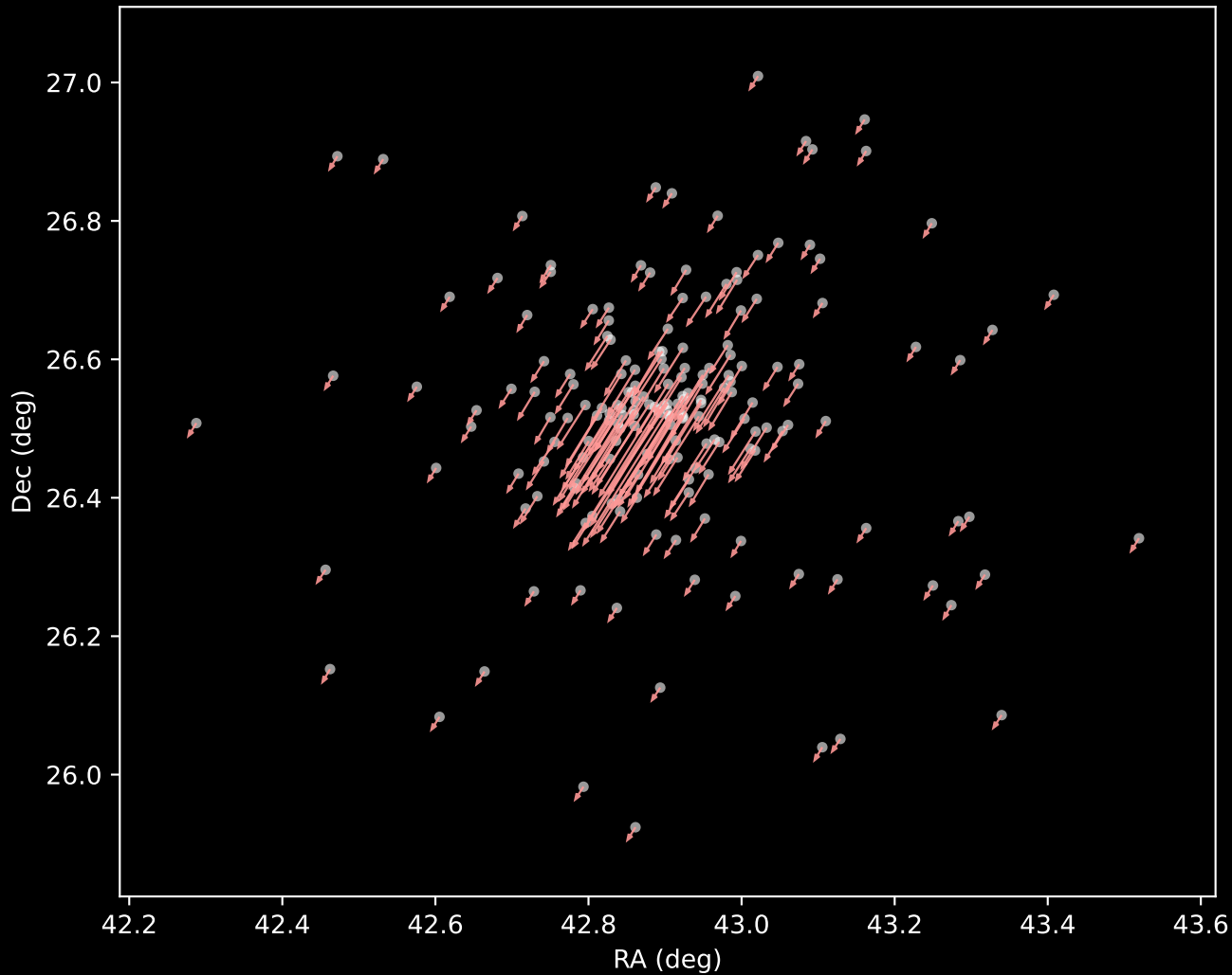
Gaia DR3 Cluster 7 Proper Motion Vectors (n=183)
