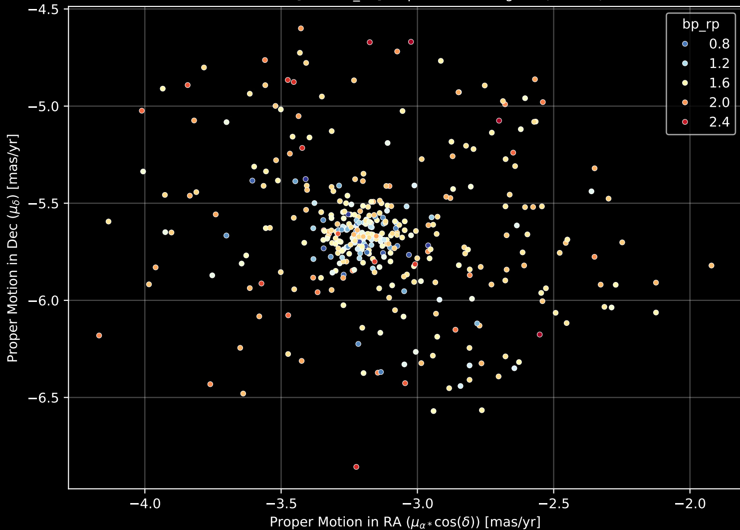
Gaia Cluster: [Gulliver_18] Proper Motion Diagram (n= 385)
