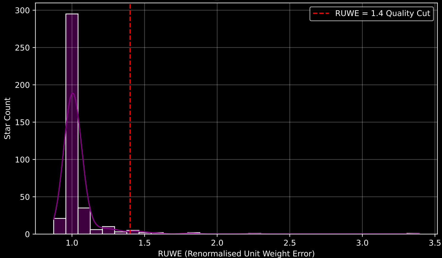
Gaia Cluster: [Gulliver_18] RUWE Distribution (n= 383)
