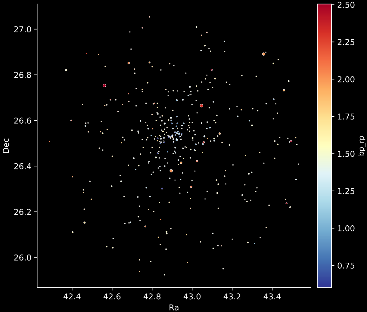
Gaia Cluster: [Gulliver_18] Stars: 385
