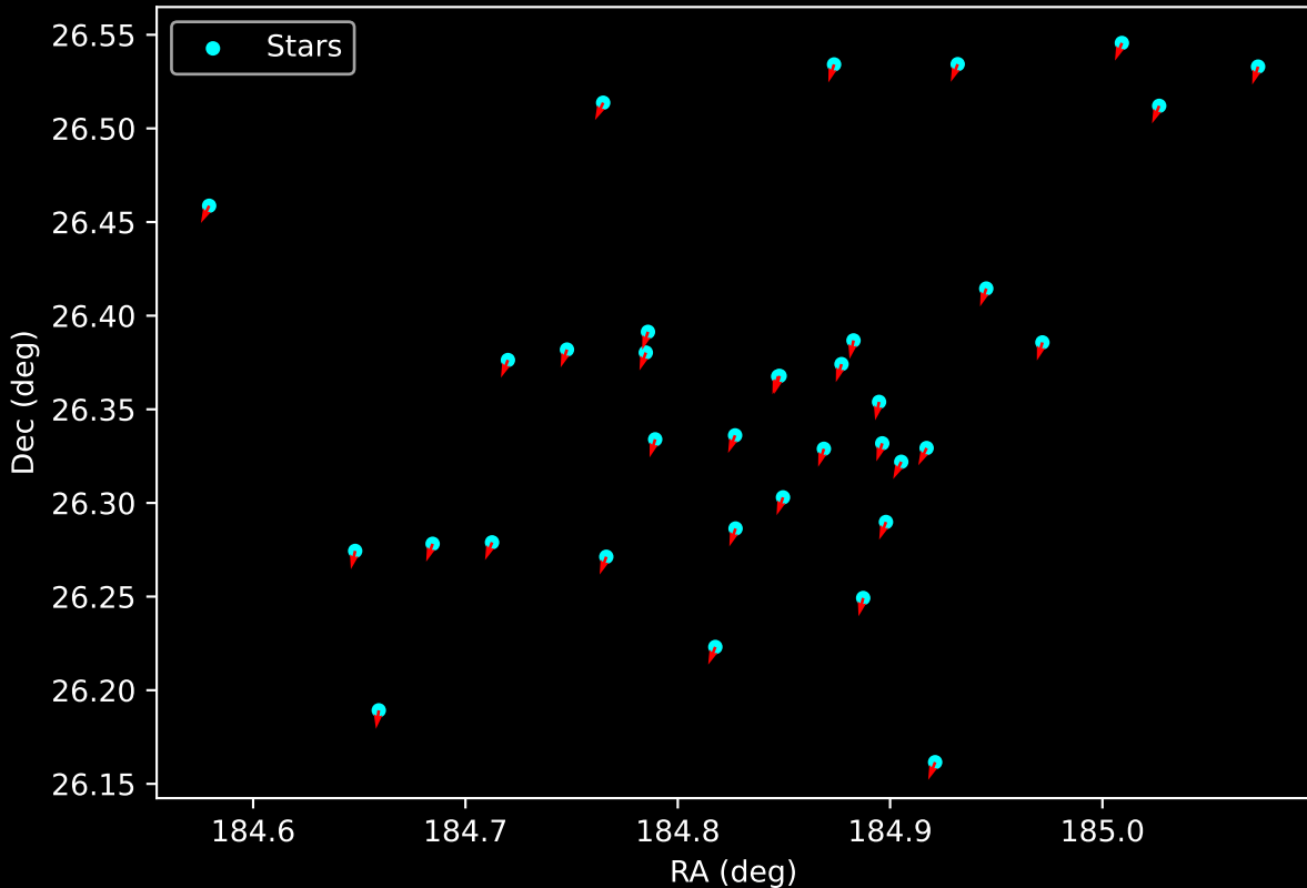
Gaia Cluster: [Gulliver_22] Proper Motion Vectors for Gaia Star Field (n= 35)
