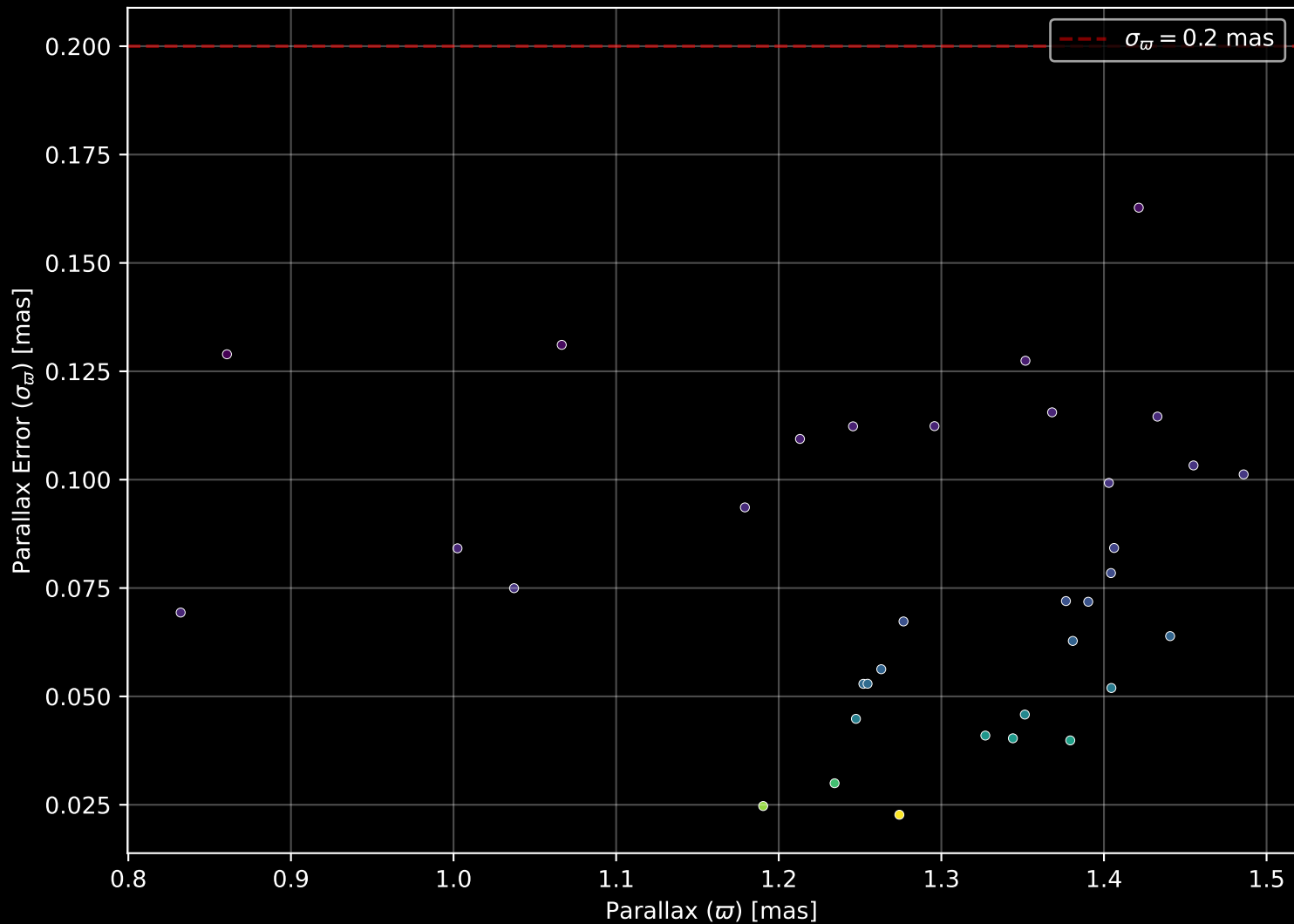
Gaia Cluster: [Gulliver 22] Parallax Quality (n= 35)
