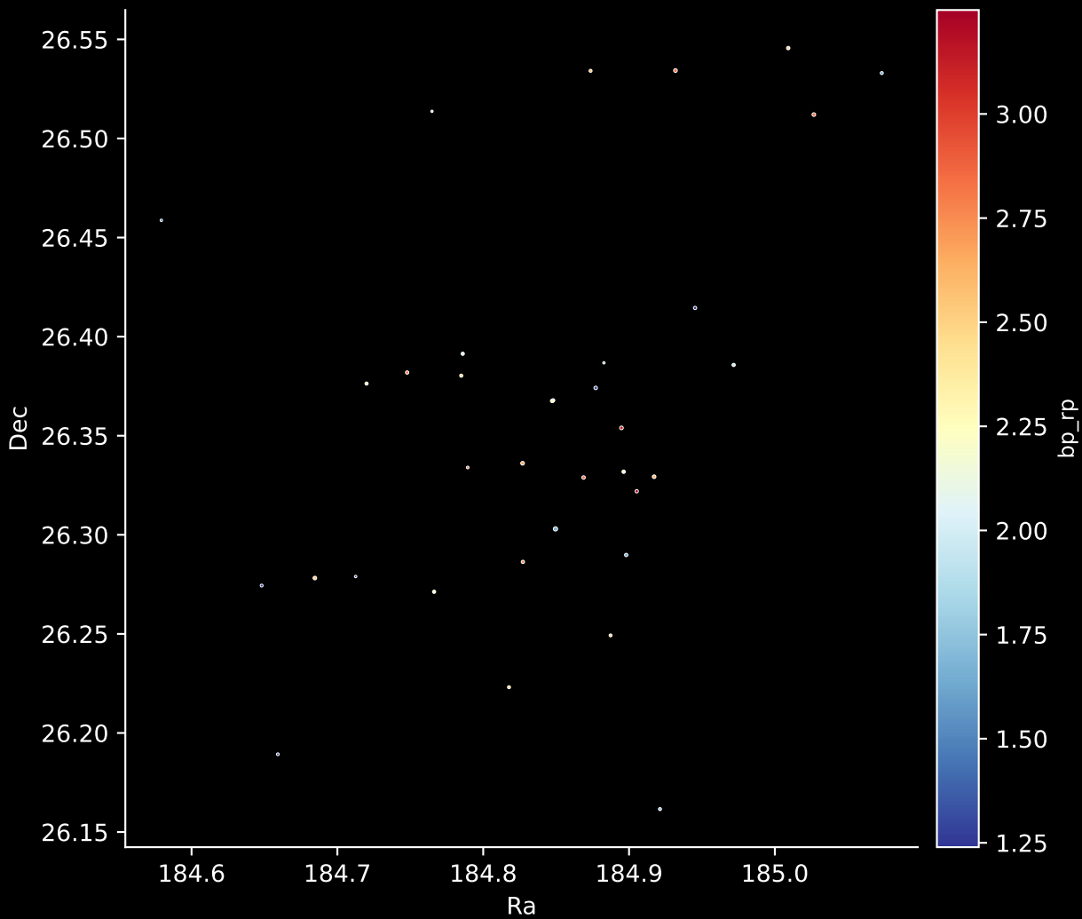
Gaia Cluster: [Gulliver_22] Stars: 35
