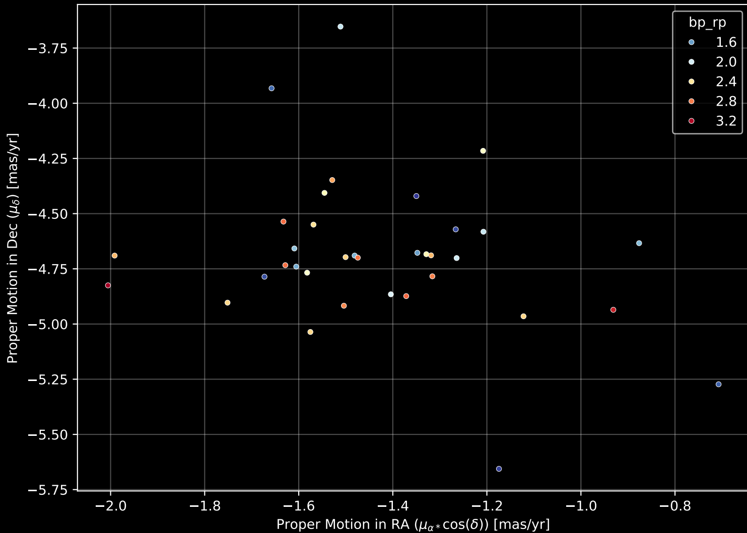
Gaia Cluster: [Gulliver_22] Proper Motion Diagram (n= 35)
