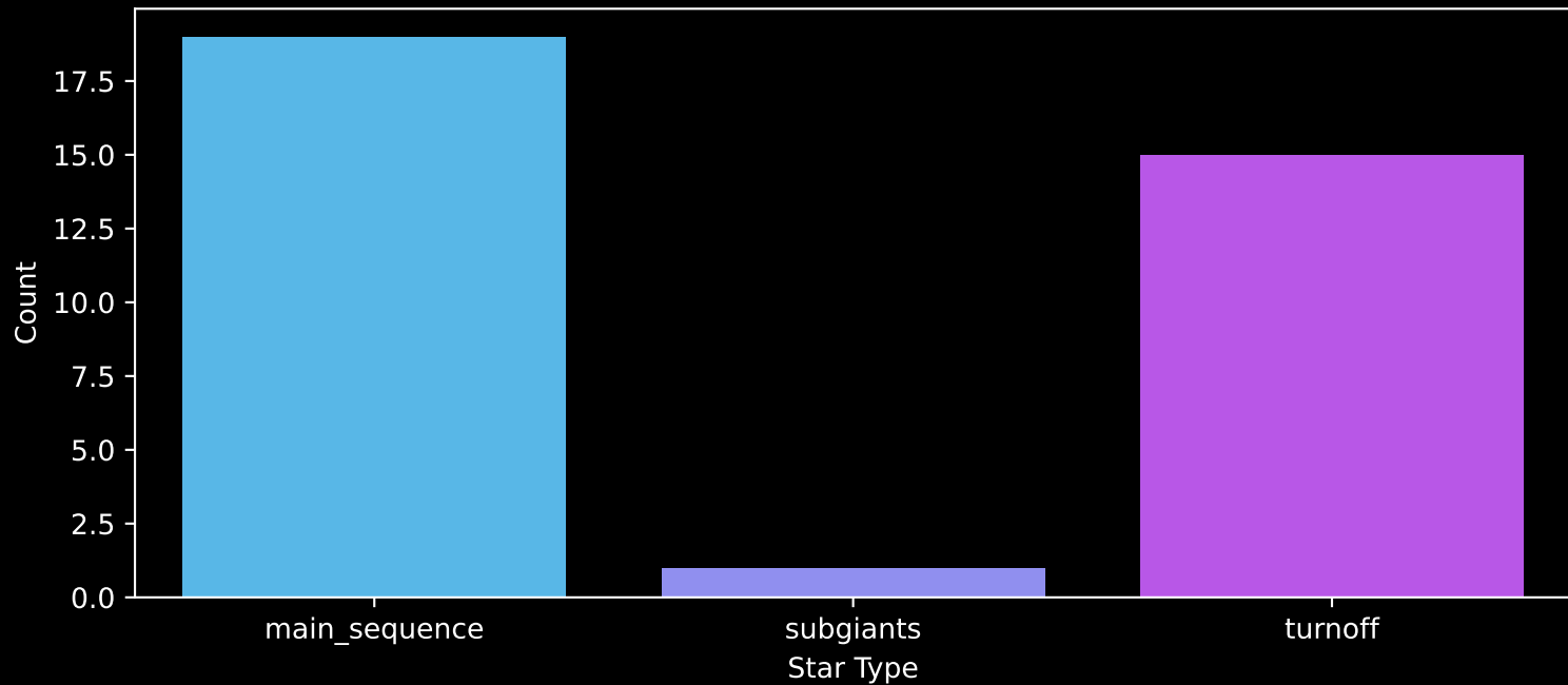
Gaia Cluster: [Gulliver_22] Count plot of Star Type
