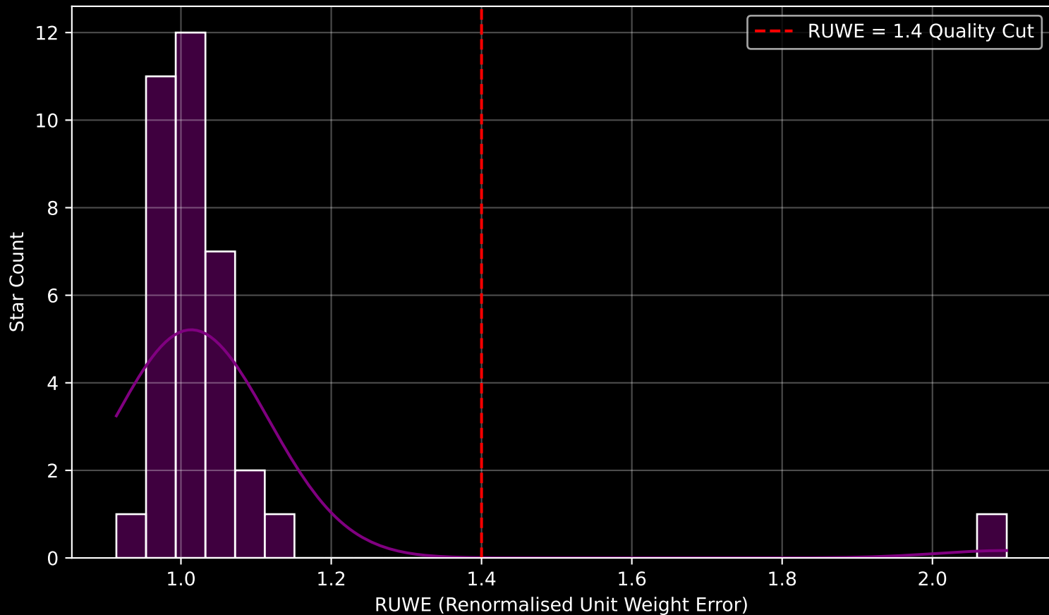
Gaia Cluster: [Gulliver_22] RUWE Distribution (n= 35)
