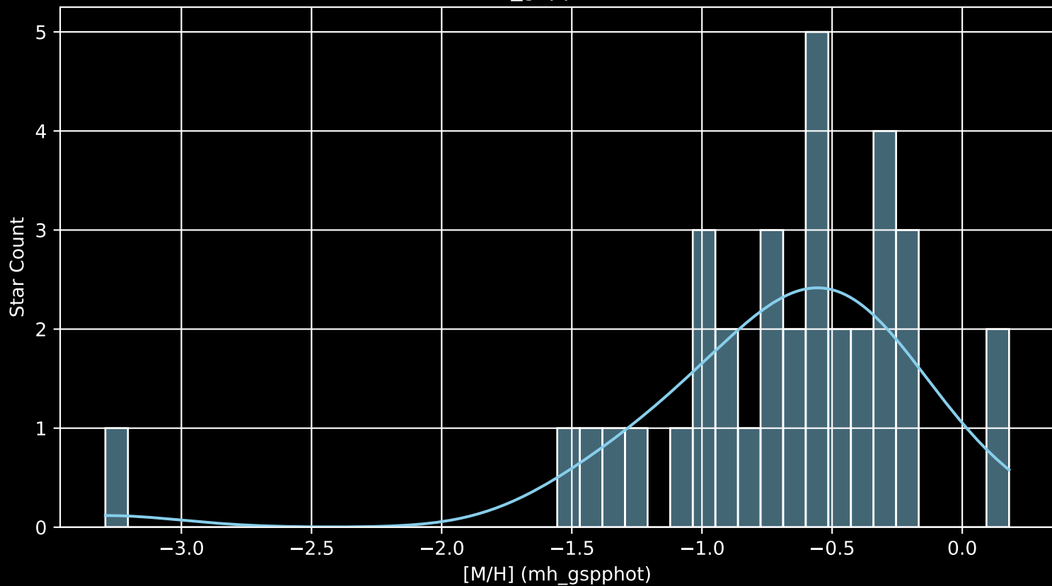
Gaia Cluster: [Gulliver_22 [M/H] (mh_gspphot) (n= 35)
