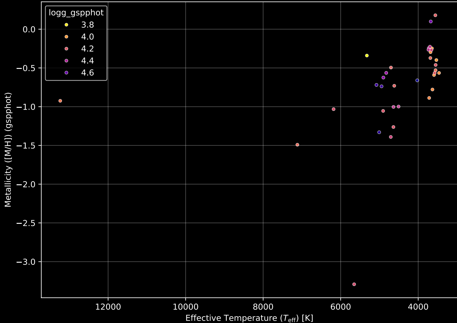
Gaia Cluster: [Gulliver_22] Stellar Population Parameters (n= 35)
