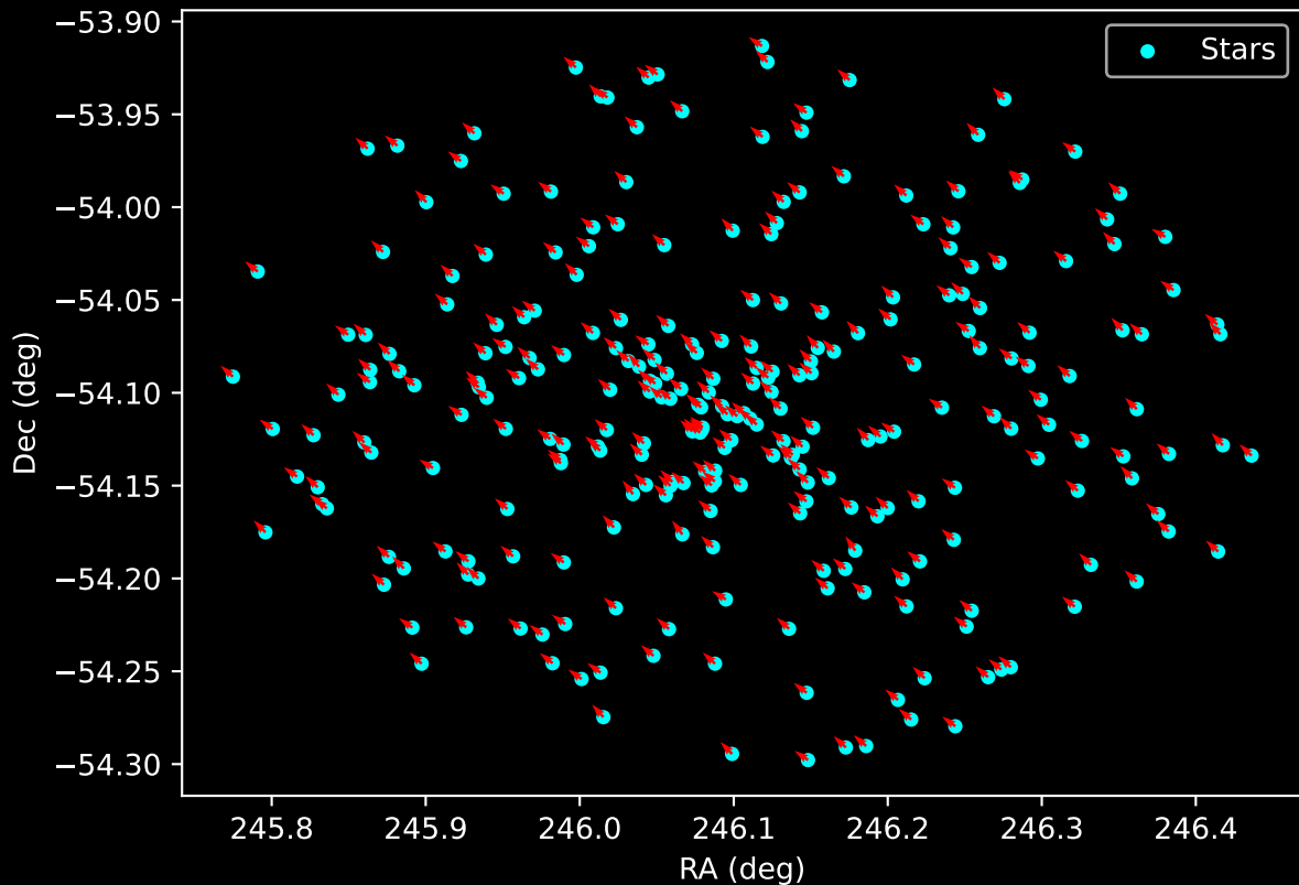
Gaia Cluster: [Gulliver_27] Proper Motion Vectors for Gaia Star Field (n= 269)
