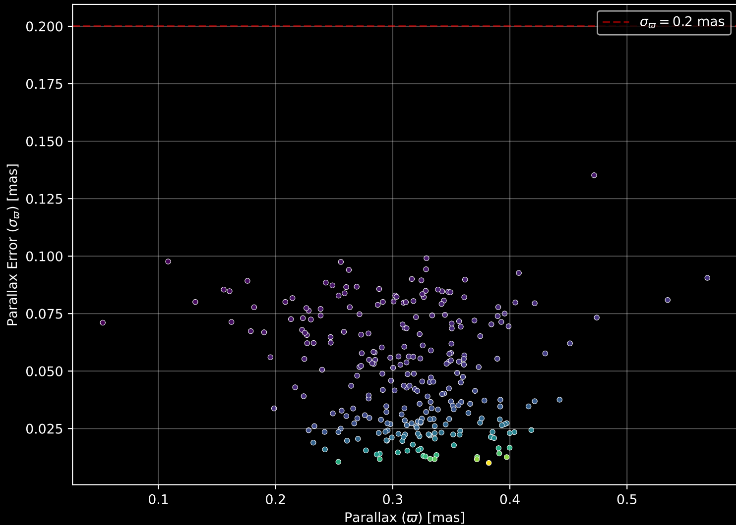
Gaia Cluster: [Gulliver_27] Parallax Quality (n= 269)
