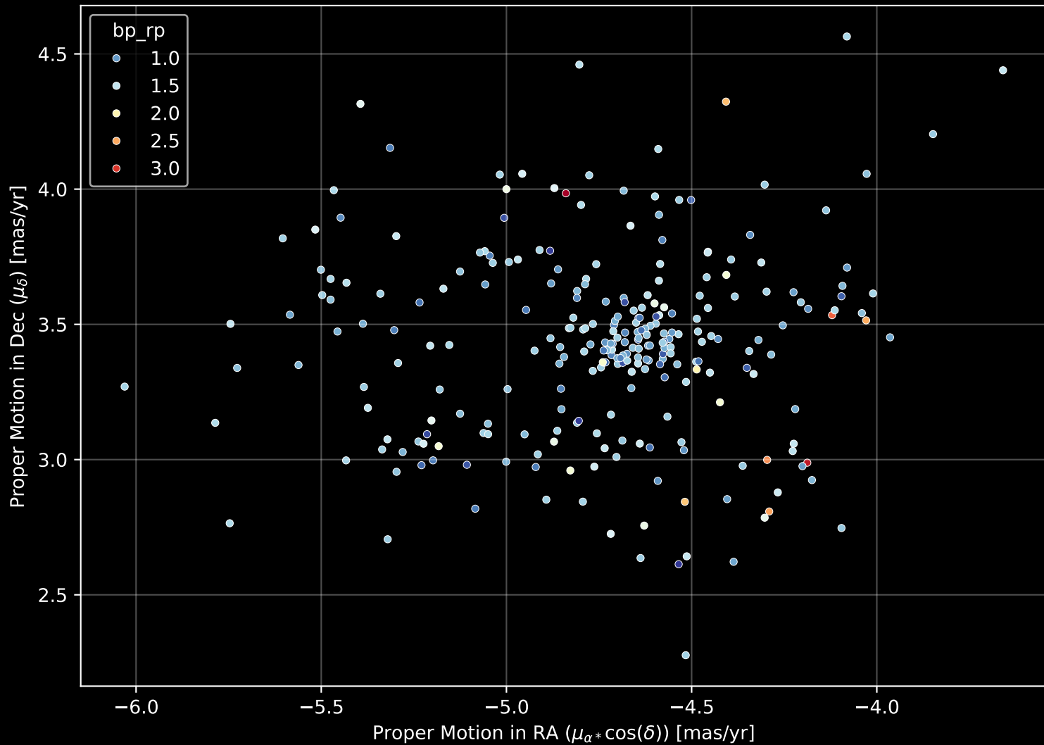
Gaia Cluster: [Gulliver_27] Proper Motion Diagram (n= 269)
