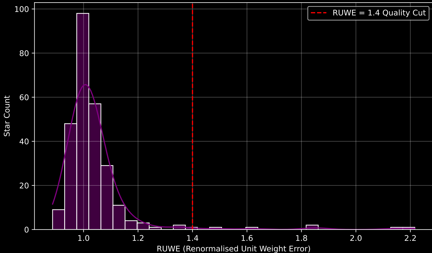
Gaia Cluster: [Gulliver_27] RUWE Distribution (n= 269)
