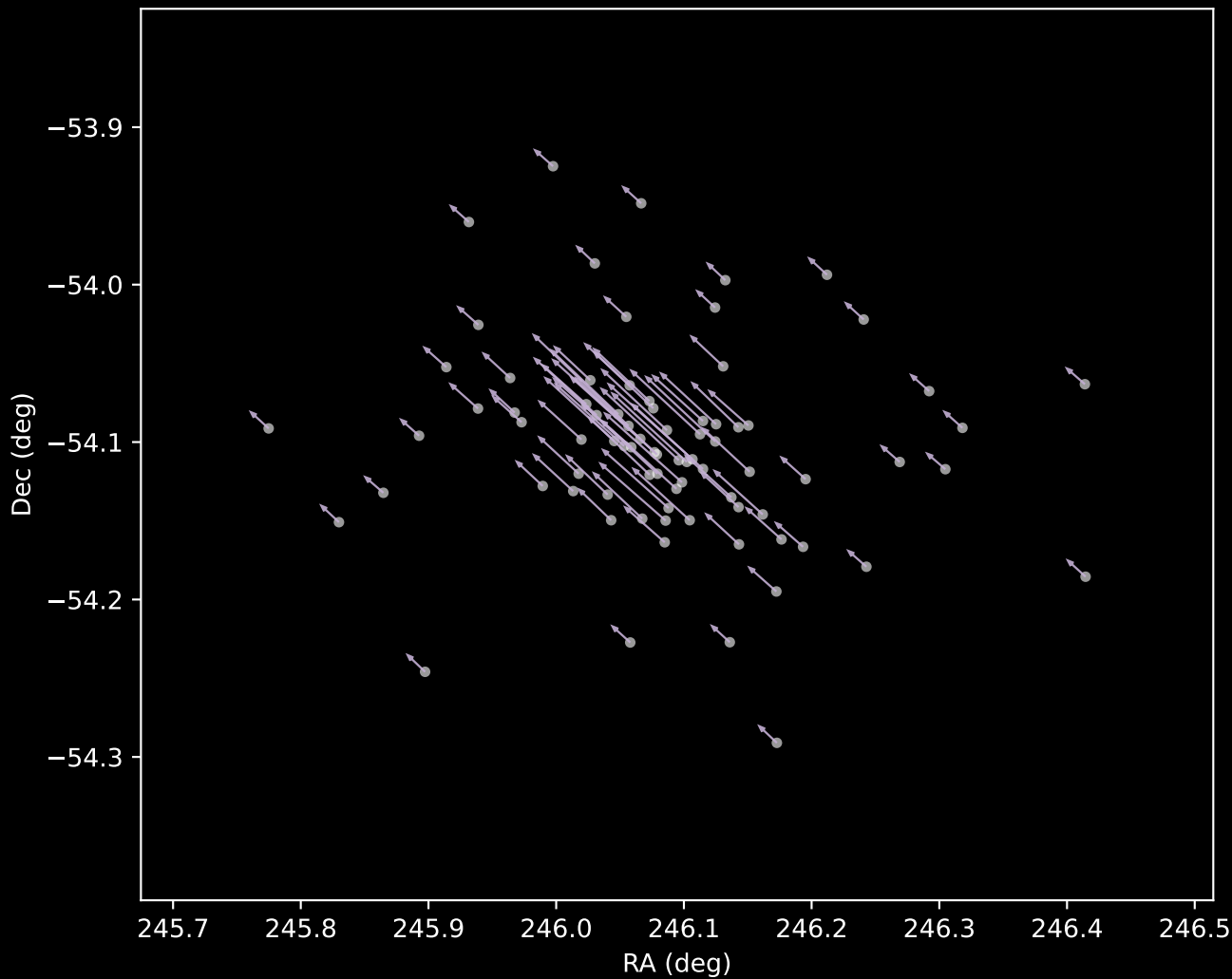
Gaia DR3 Cluster 9 Proper Motion Vectors (n=80)
