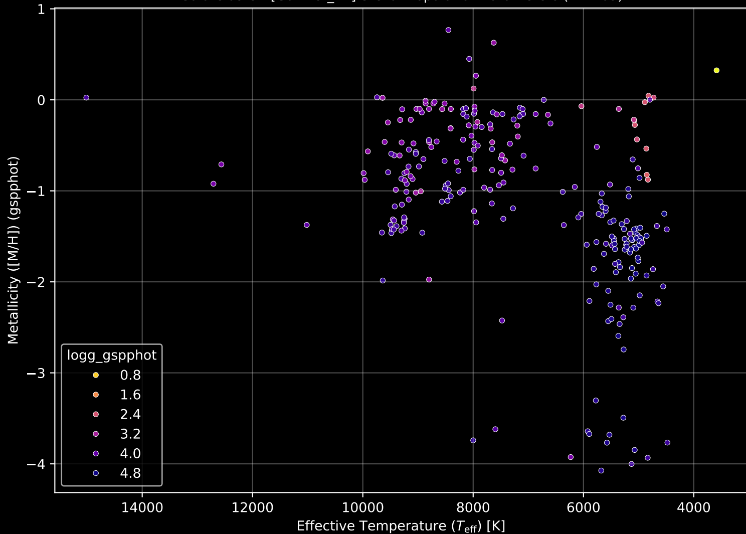
Gaia Cluster: [Gulliver_27] Stellar Population Parameters (n= 269)
