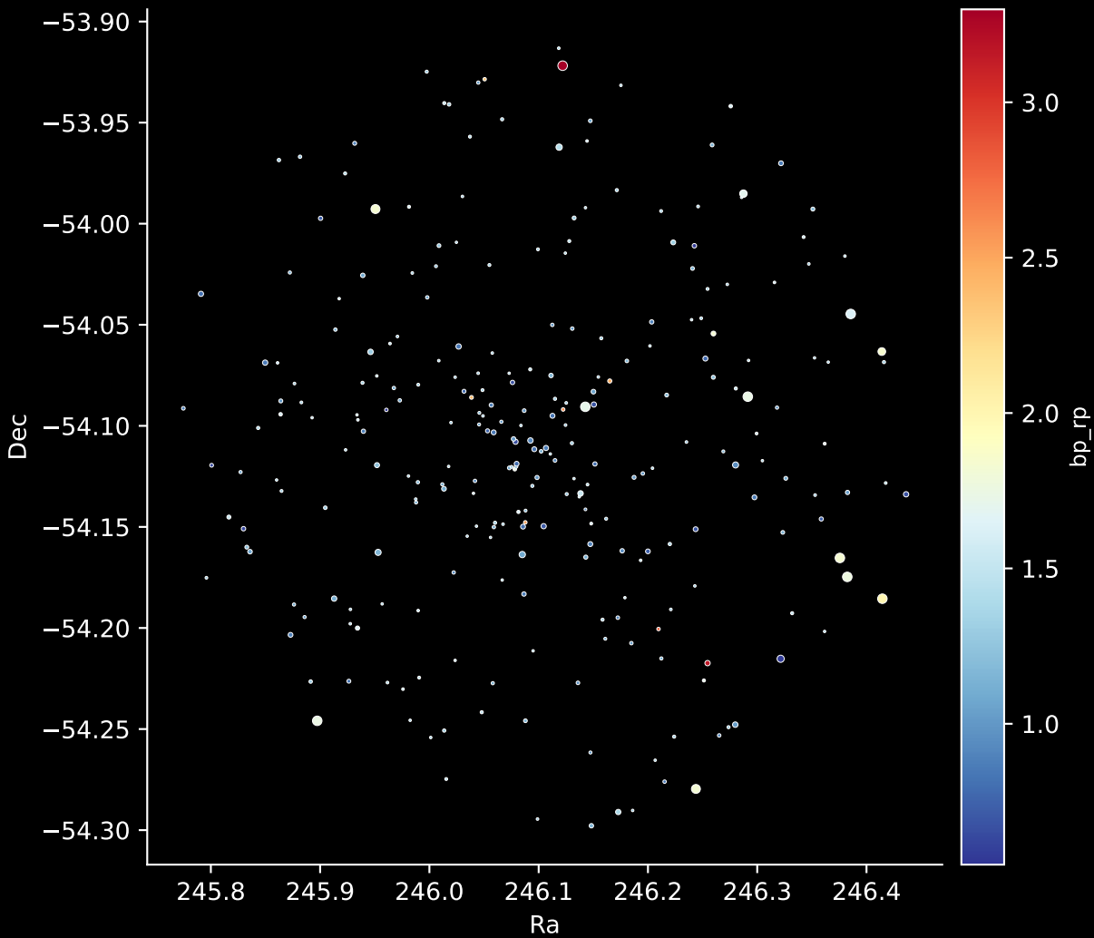
Gaia Cluster: [Gulliver_27] Stars: 269
