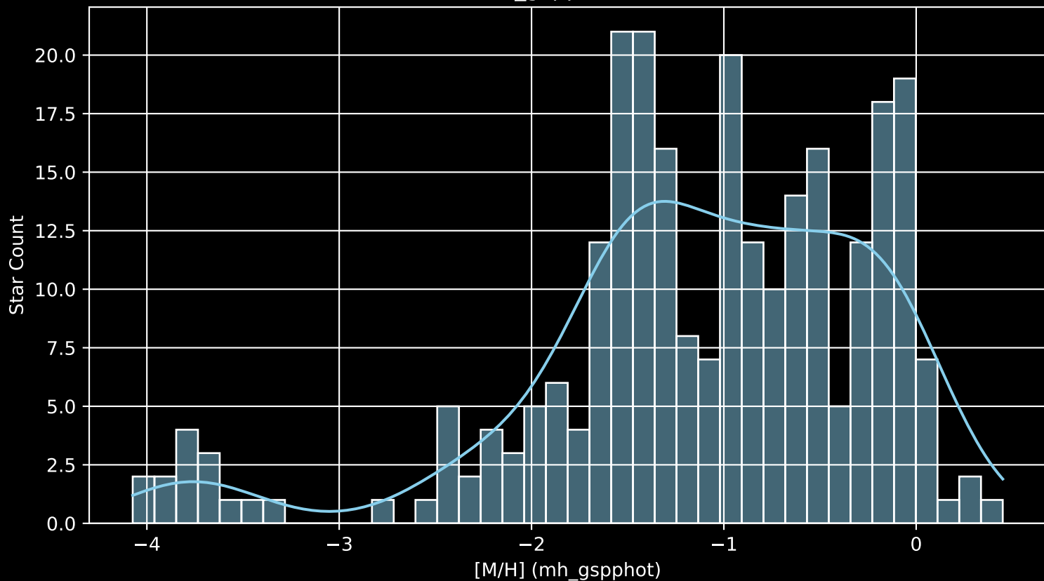
Gaia Cluster: [Gulliver_27 [M/H] (mh_gspphot) (n= 267)
