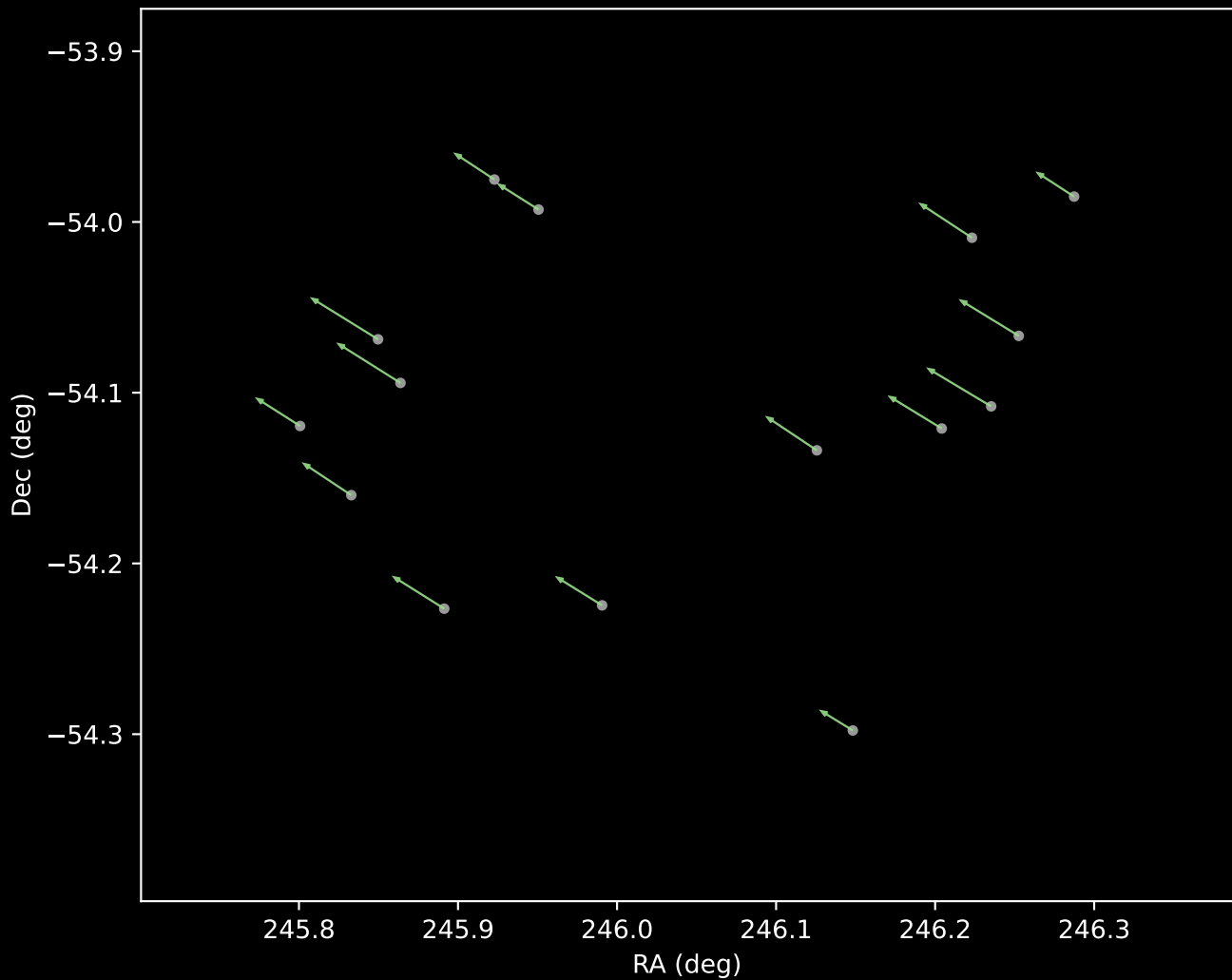
Gaia DR3 Cluster 5 Proper Motion Vectors (n=15)
