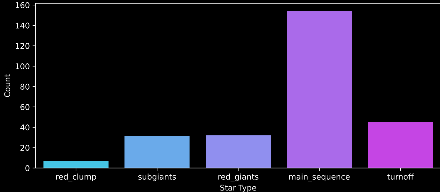
Gaia Cluster: [Gulliver_27] Count plot of Star Type
