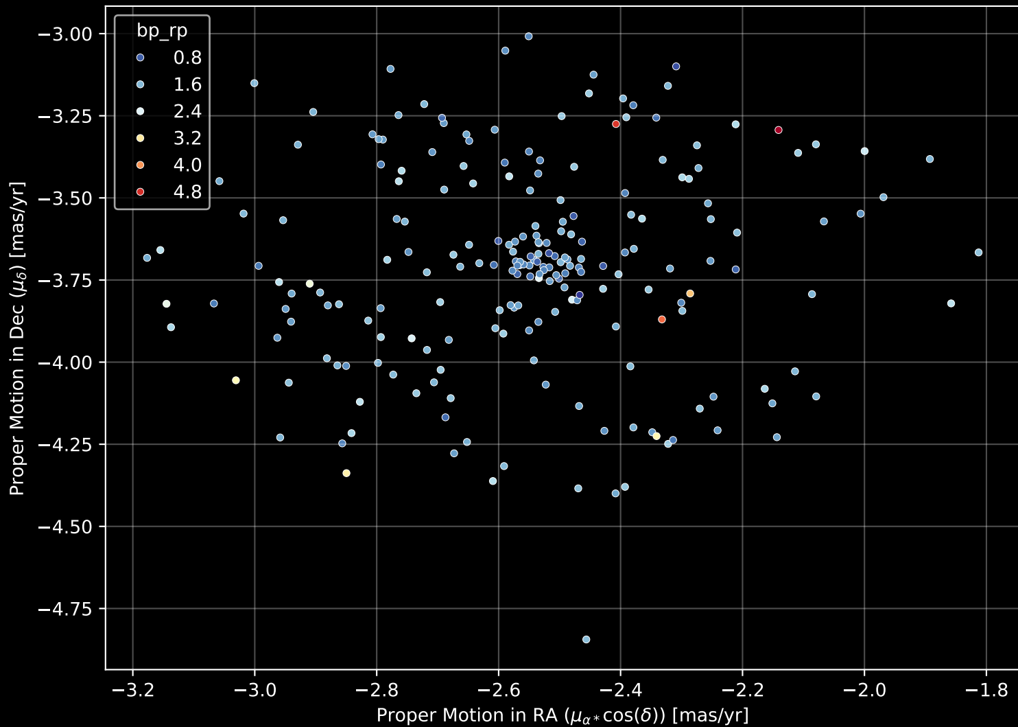
Gaia Cluster: [Gulliver_30] Proper Motion Diagram (n= 215)
