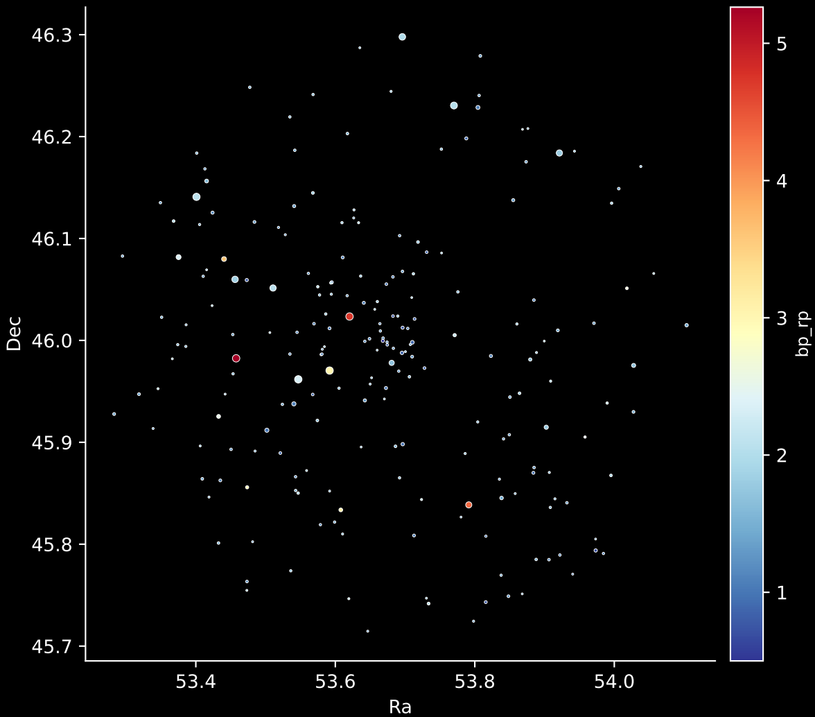
Gaia Cluster: [Gulliver_30] Stars: 215
