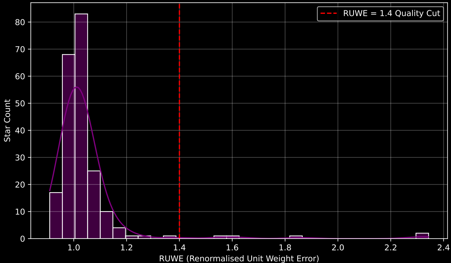
Gaia Cluster: [Gulliver_30] RUWE Distribution (n= 215)
