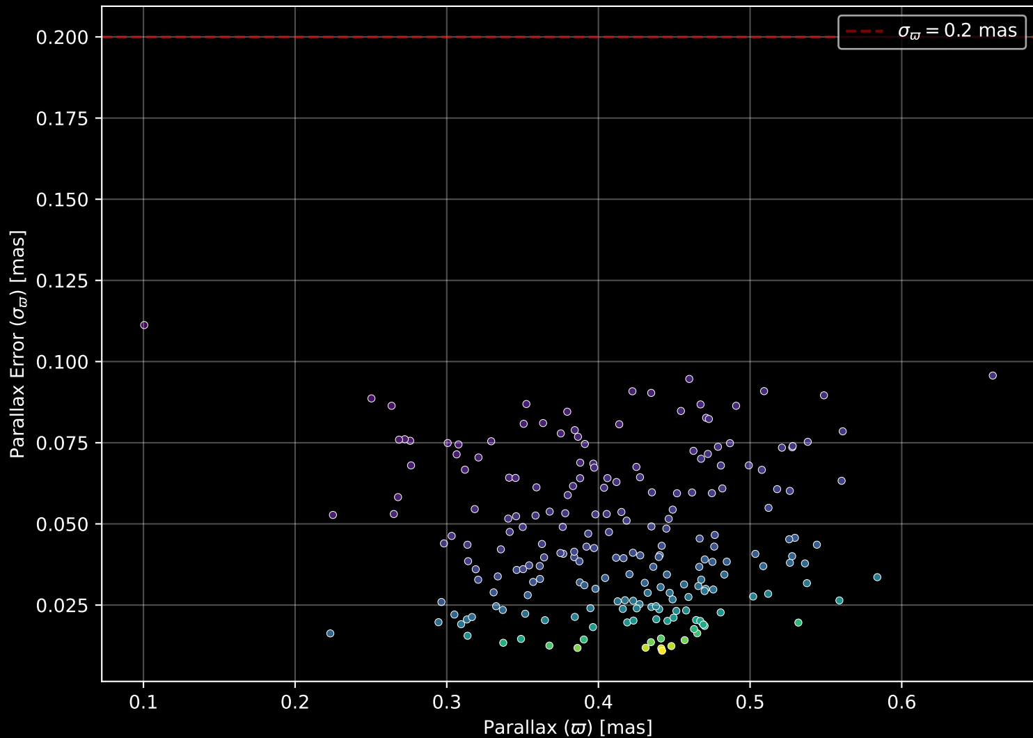
Gaia Cluster: [Gulliver_30] Parallax Quality (n= 215)
