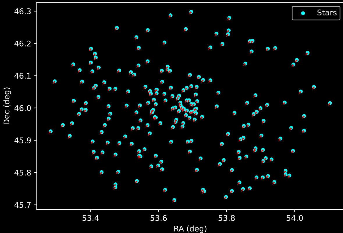
Gaia Cluster: [Gulliver_30] Proper Motion Vectors for Gaia Star Field (n= 215)
