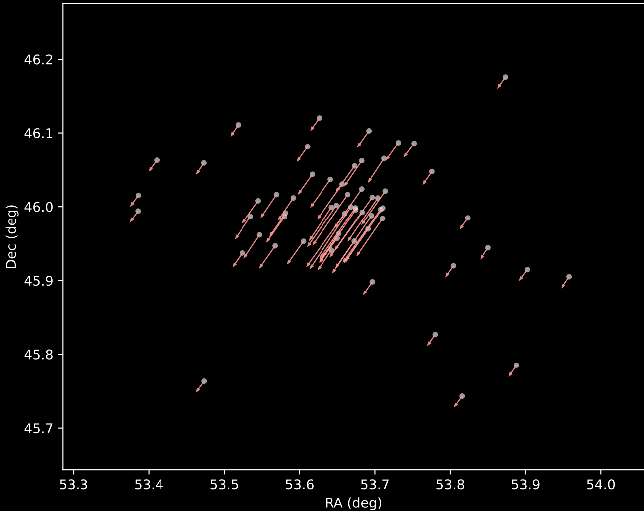
Gaia DR3 Cluster 7 Proper Motion Vectors (n=59)
