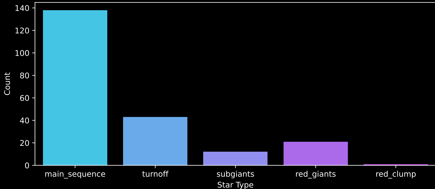
Gaia Cluster: [Gulliver_30] Count plot of Star Type
