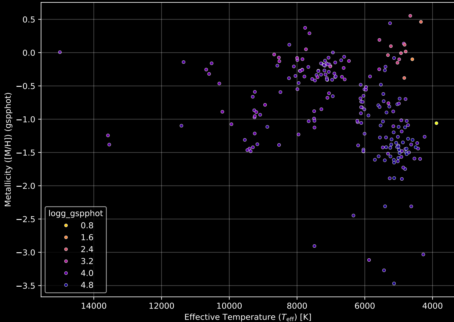
Gaia Cluster: [Gulliver_30] Stellar Population Parameters (n= 215)
