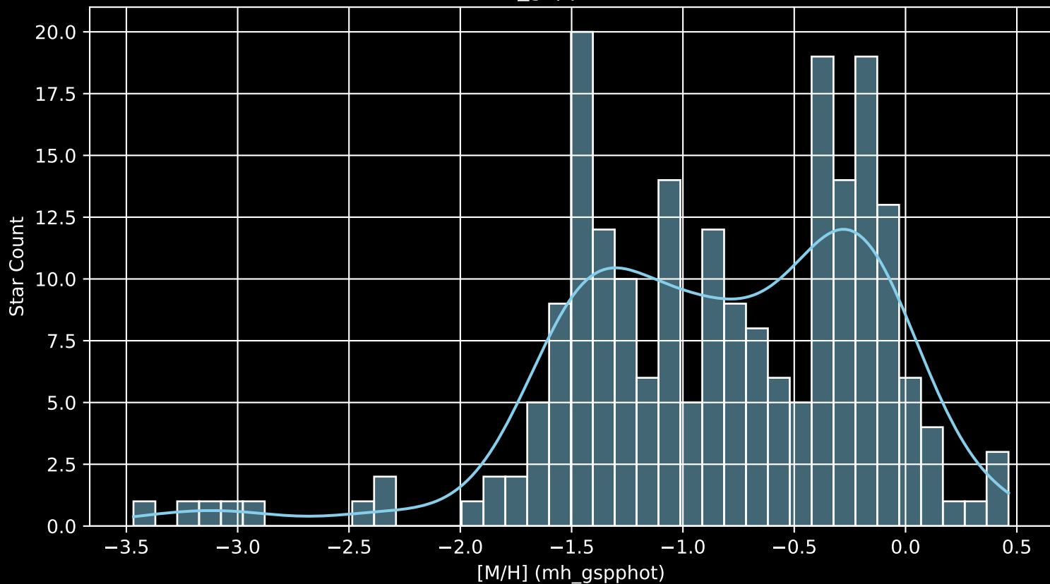
Gaia Cluster: [Gulliver_30 [M/H] (mh_gspphot) (n= 214)
