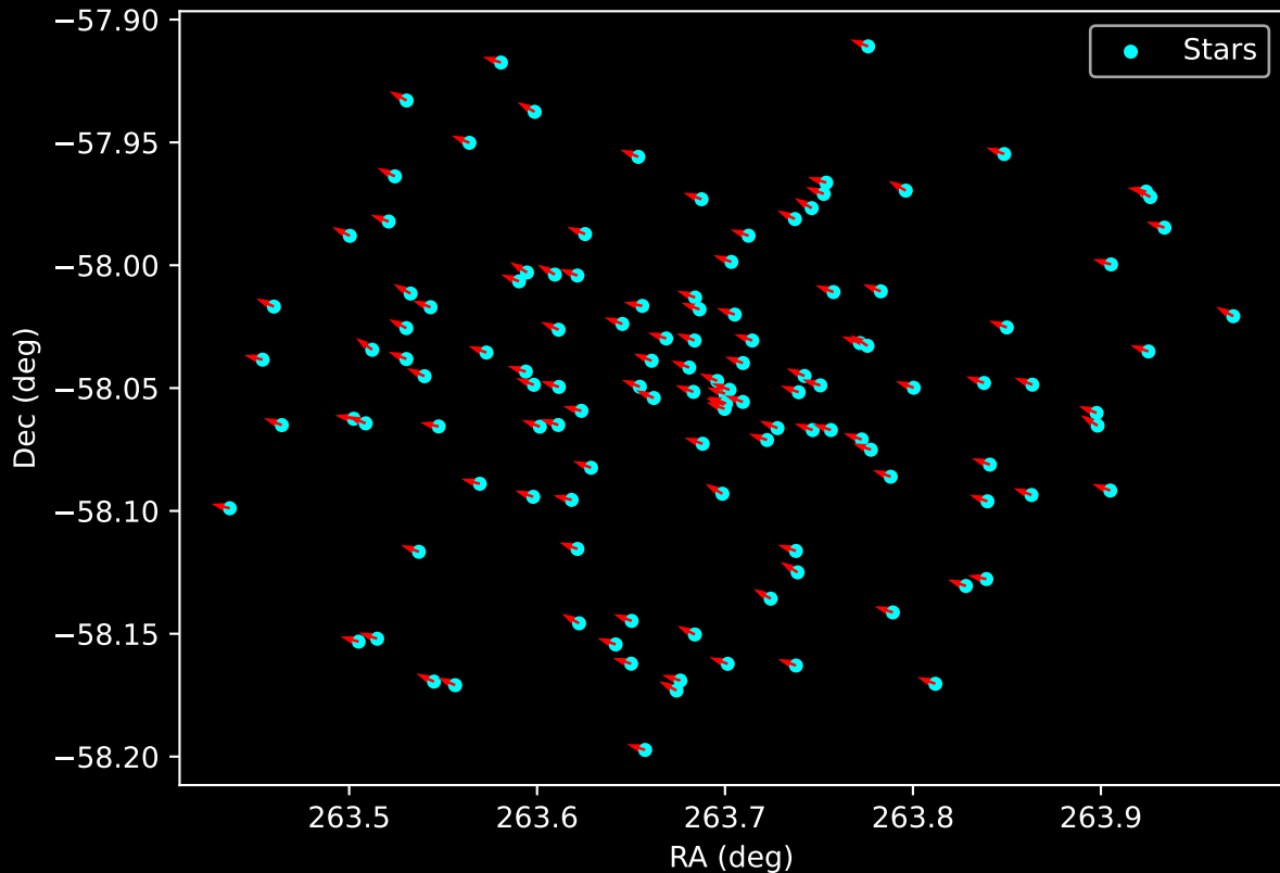
Gaia Cluster: [Gulliver_39] Proper Motion Vectors for Gaia Star Field (n= 124)
