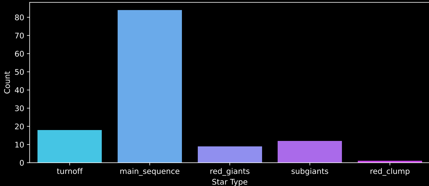
Gaia Cluster: [Gulliver_39] Count plot of Star Type
