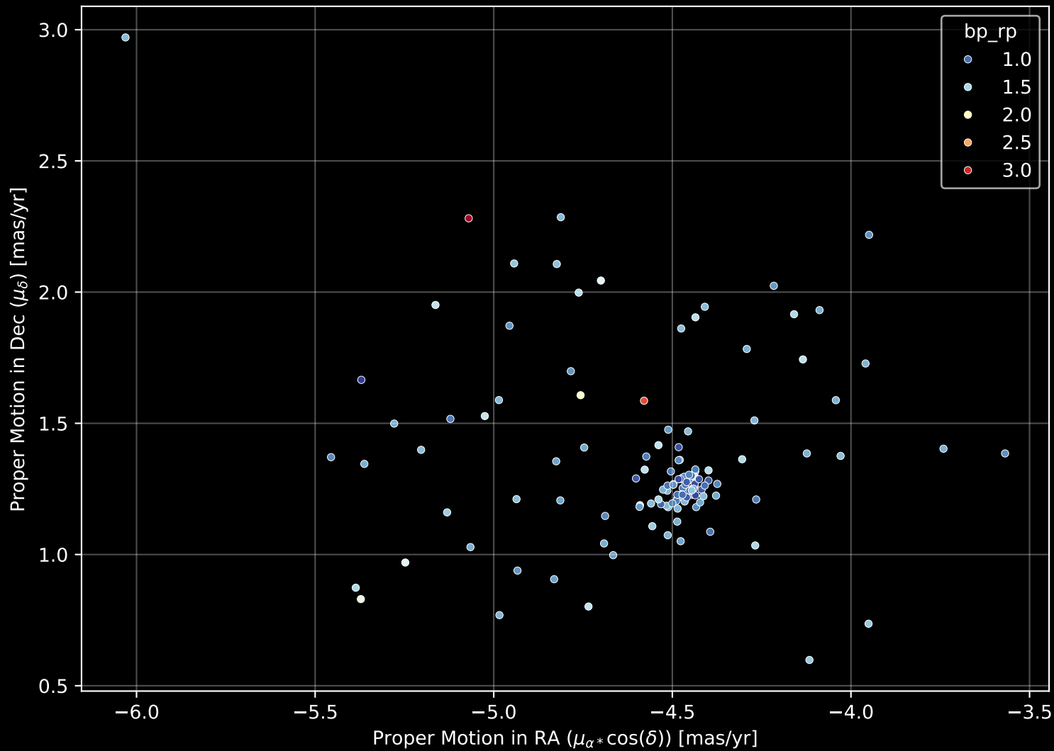
Gaia Cluster: [Gulliver_39] Proper Motion Diagram (n= 124)
