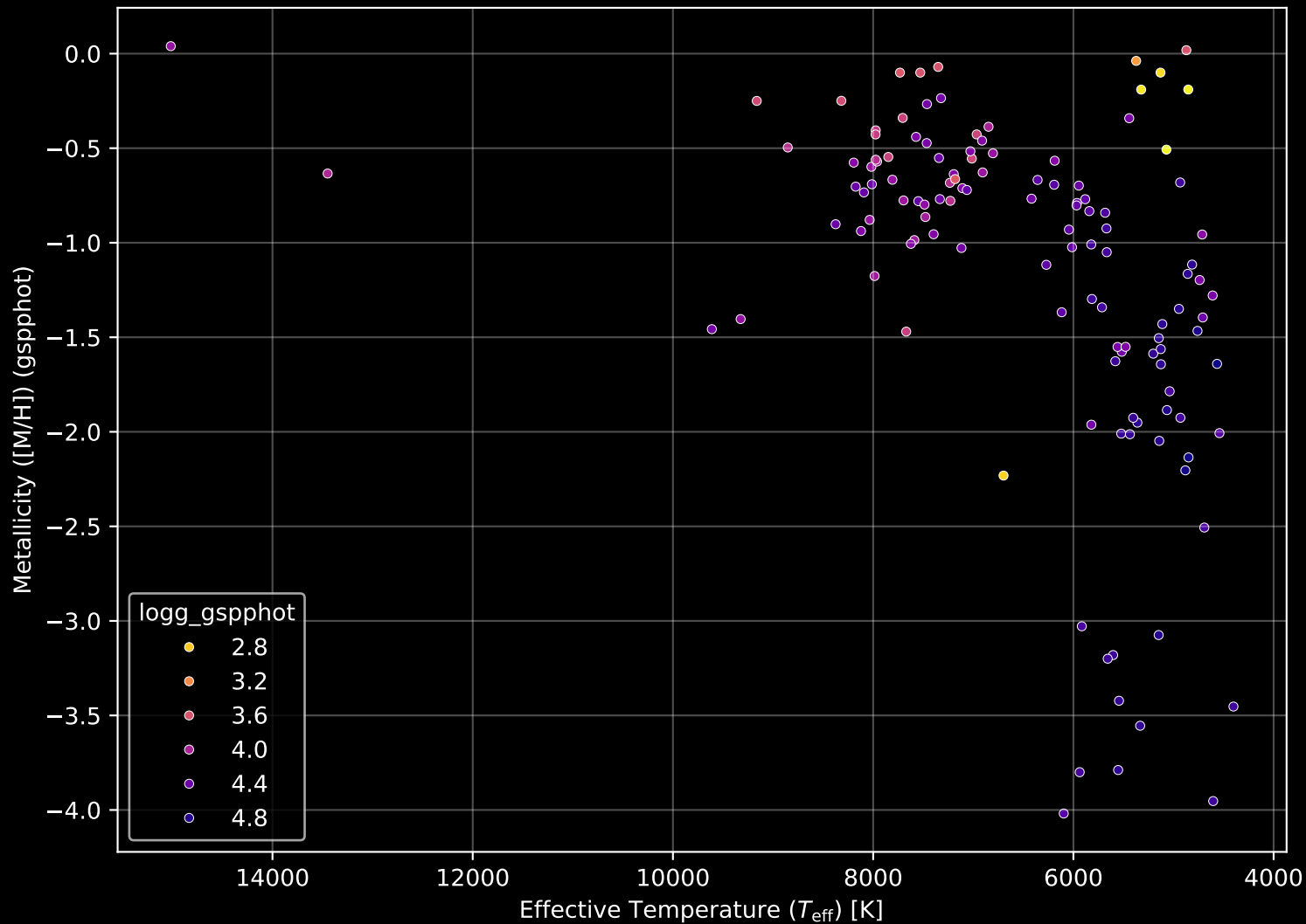
Gaia Cluster: [Gulliver_39] Stellar Population Parameters (n= 124)
