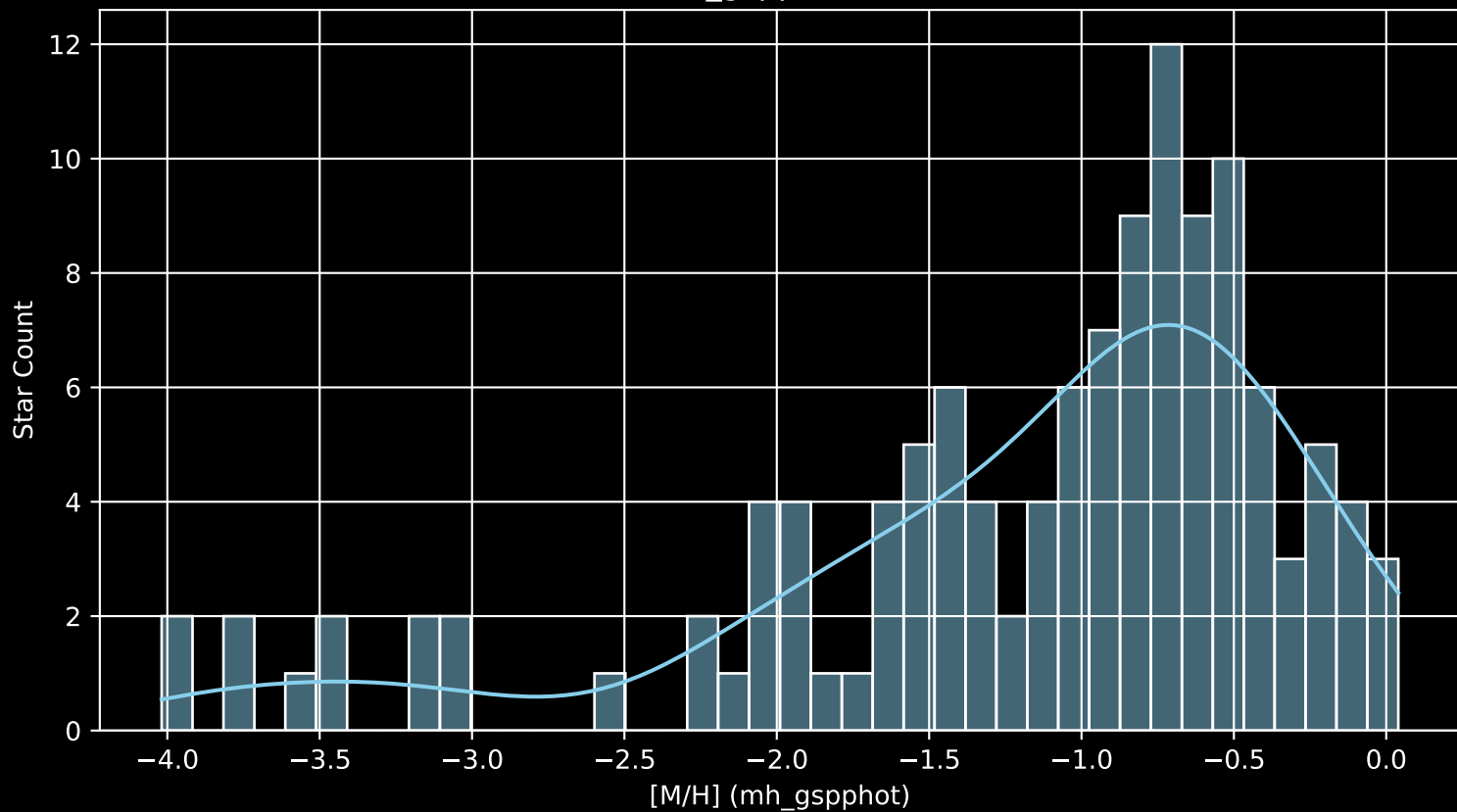
Gaia Cluster: [Gulliver_39 [M/H] (mh_gspphot) (n= 124)
