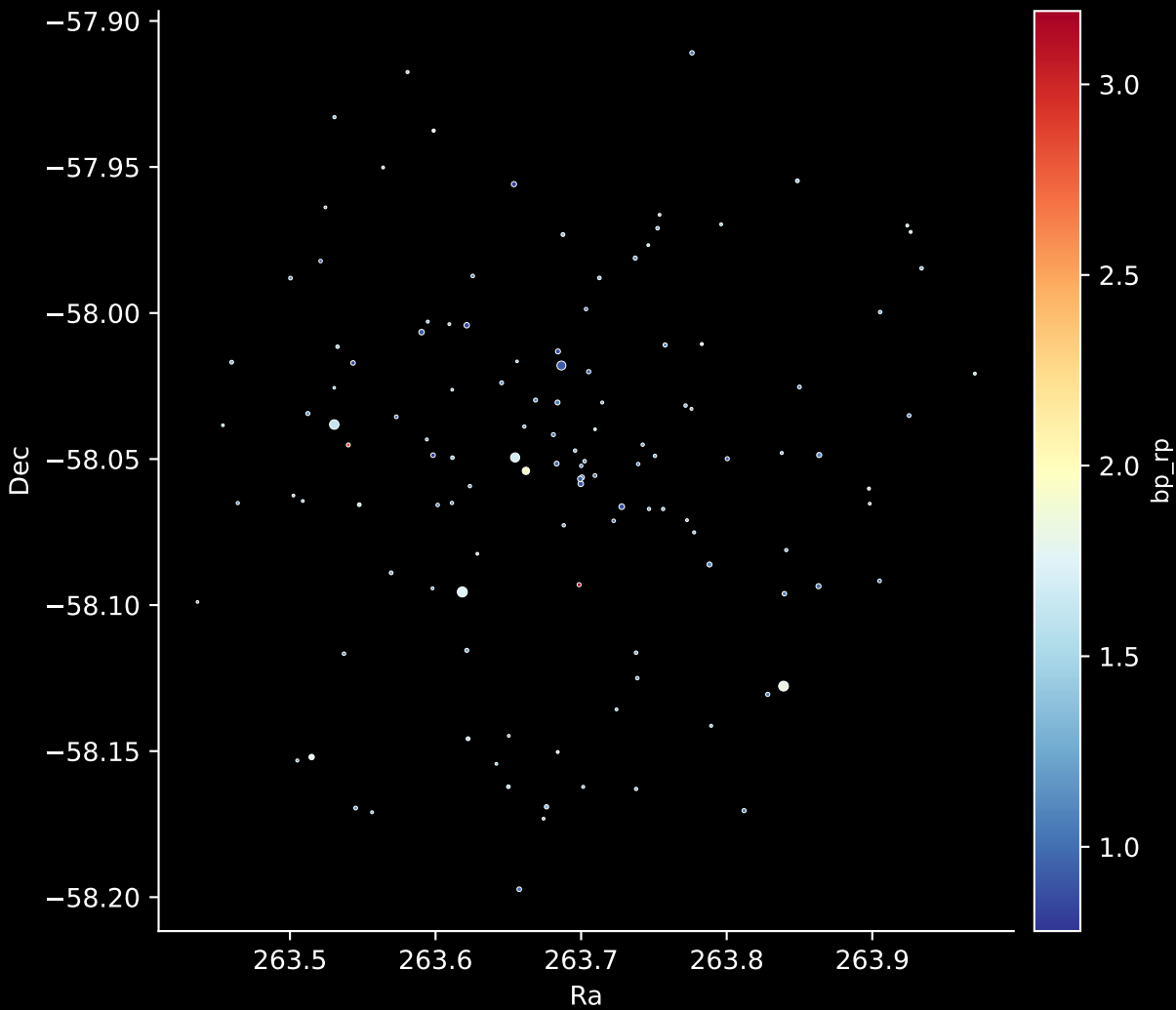
Gaia Cluster: [Gulliver_39] Stars: 124
