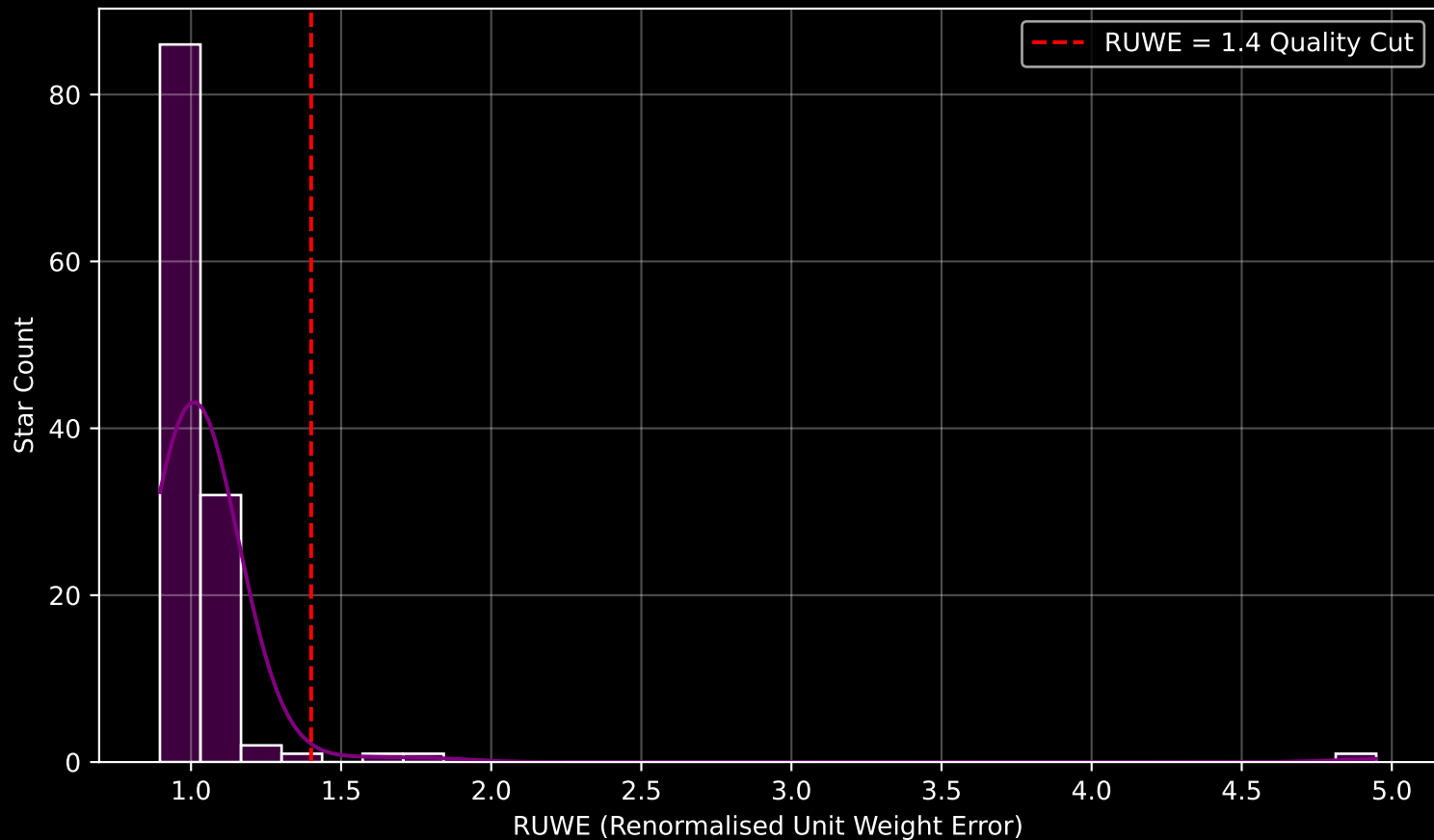
Gaia Cluster: [Gulliver_39] RUWE Distribution (n= 124)
