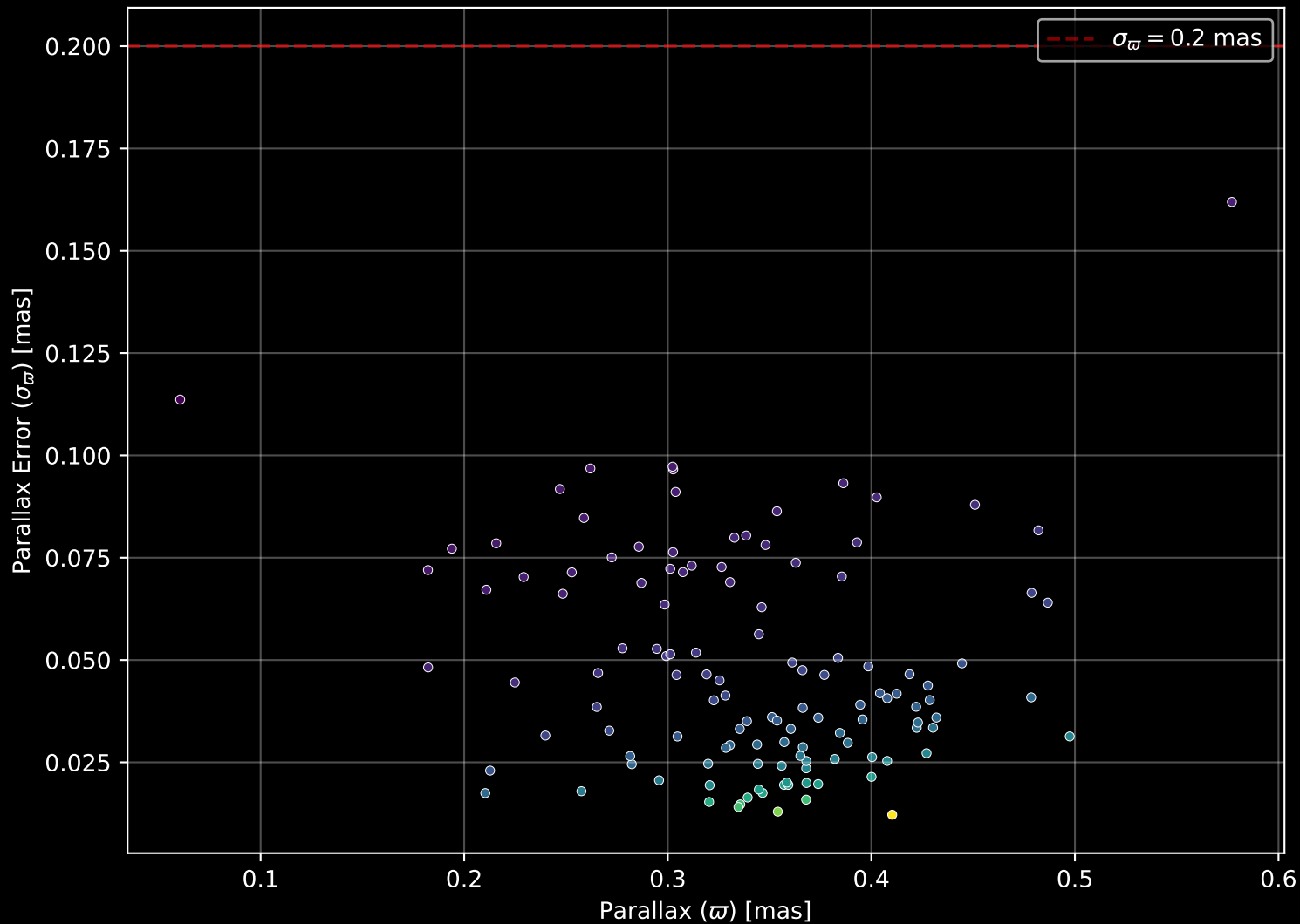
Gaia Cluster: [Gulliver_39] Parallax Quality (n= 124)
