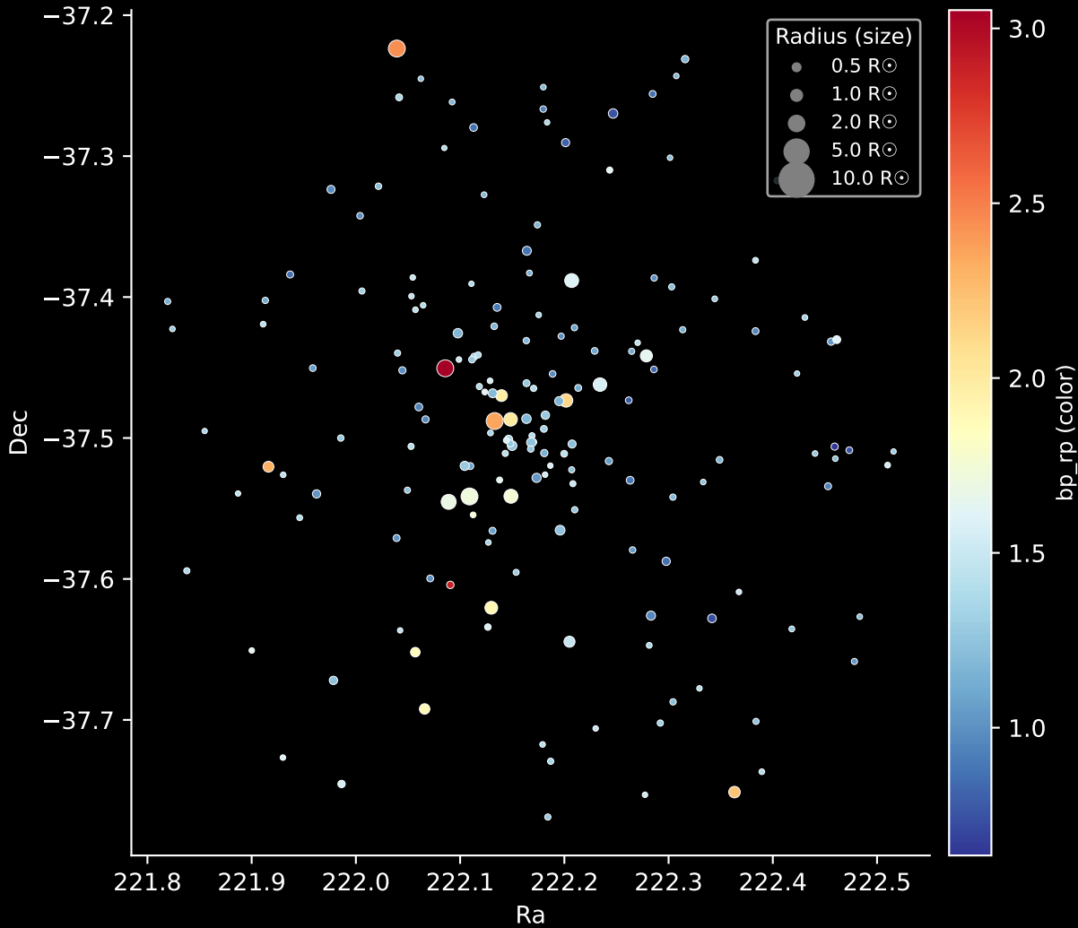
Gaia Cluster: [Gulliver_4] Stars: 171
