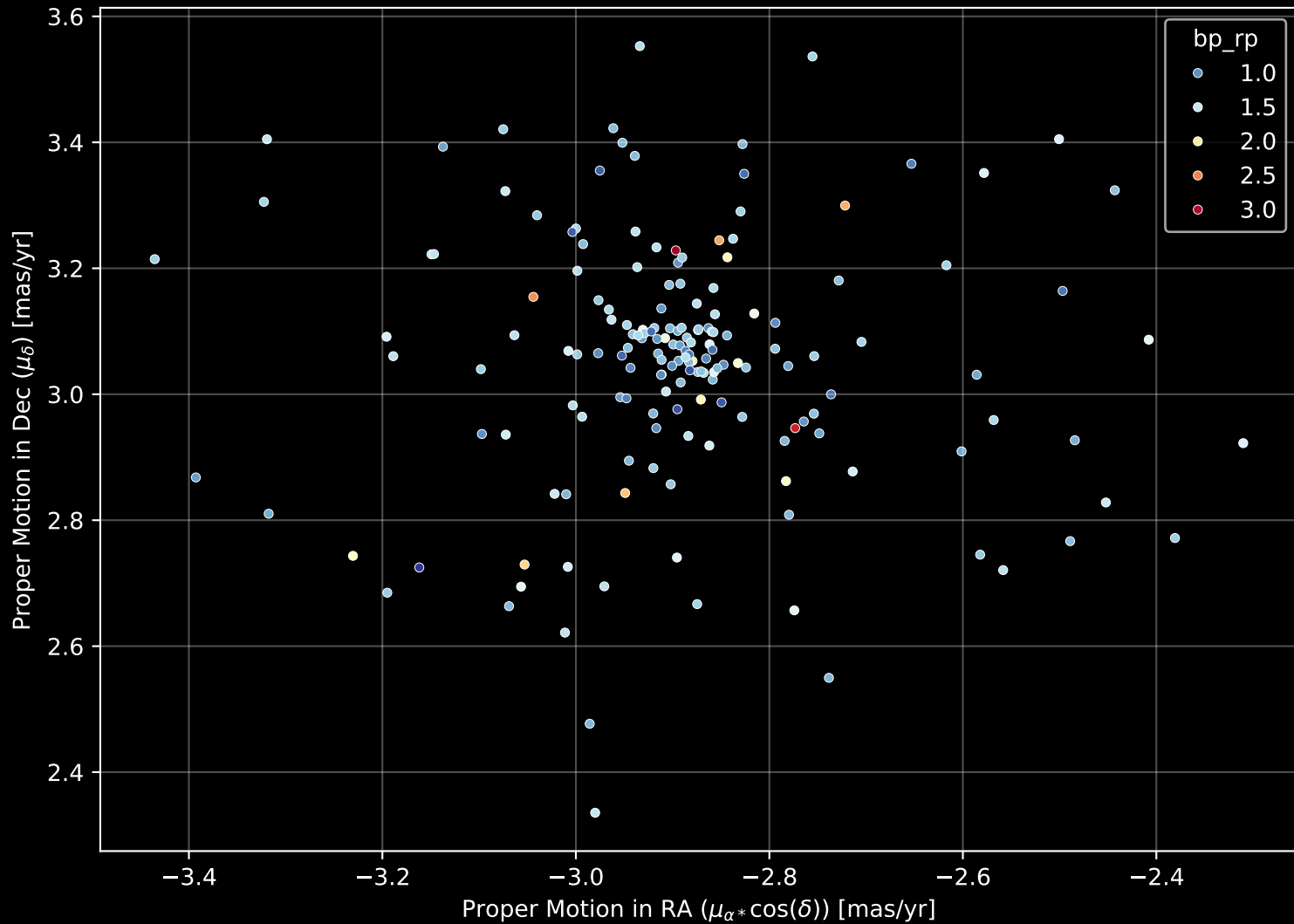
Gaia Cluster: [Gulliver_4] Proper Motion Diagram (n= 171)
