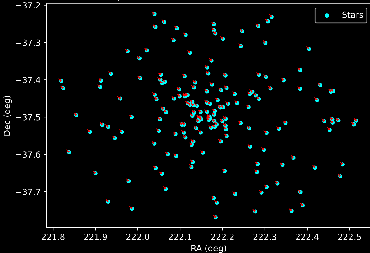
Gaia Cluster: [Gulliver_4] Proper Motion Vectors for Gaia Star Field (n= 171)
