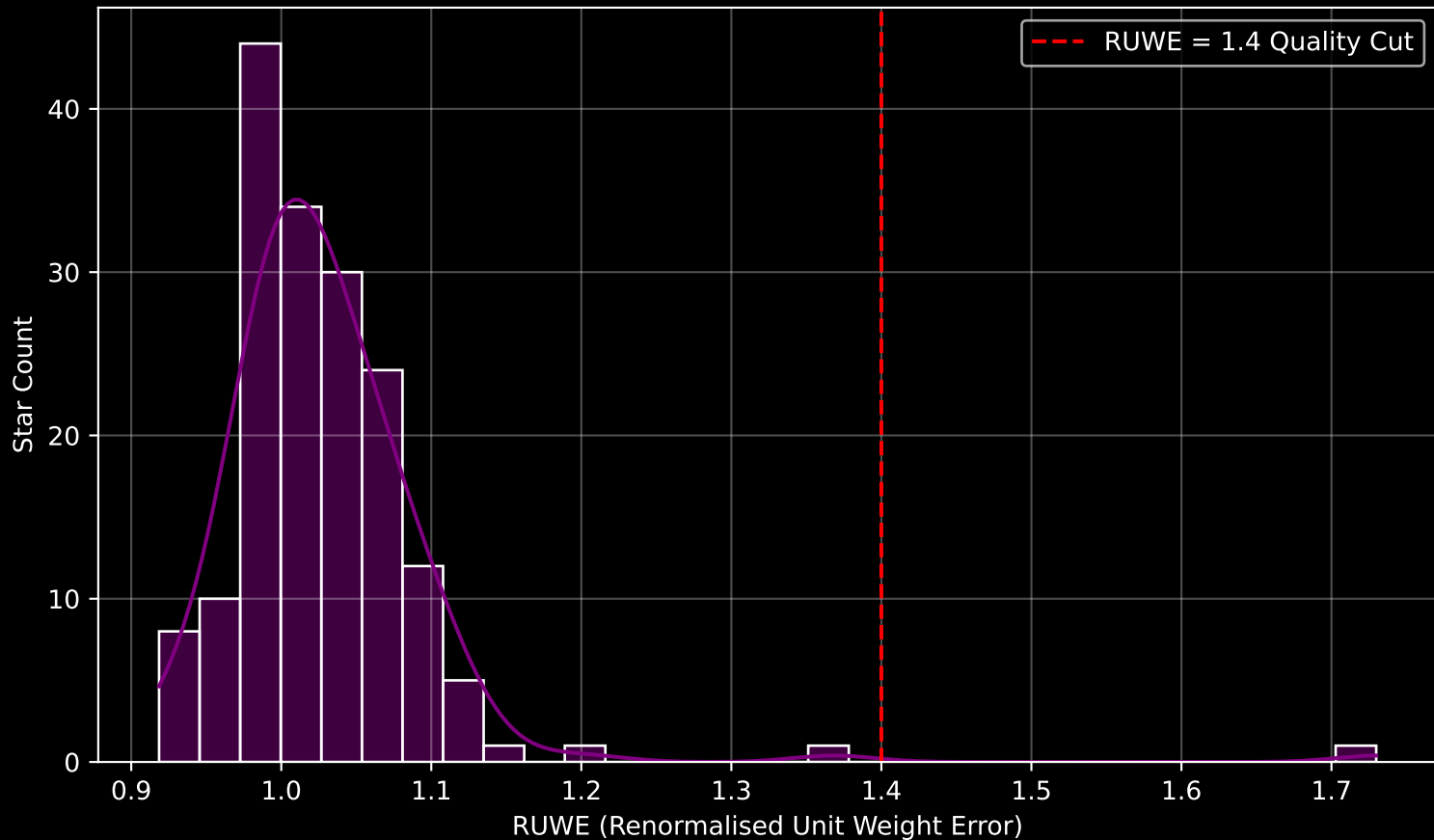
Gaia Cluster: [Gulliver_4] RUWE Distribution (n= 171)
