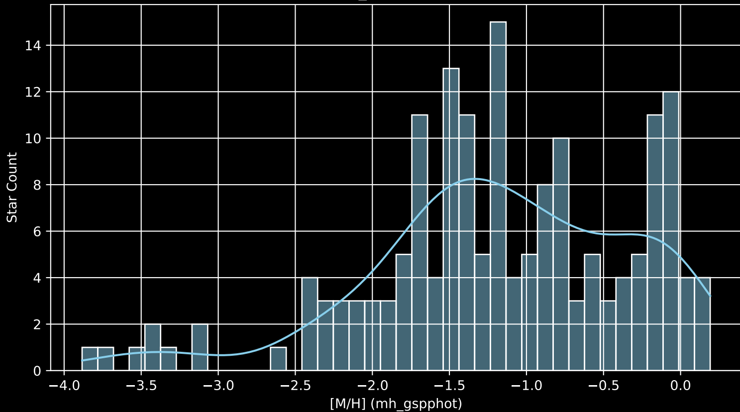
Gaia Cluster: [Gulliver_4 [M/H] (mh_gspphot) (n= 170)
