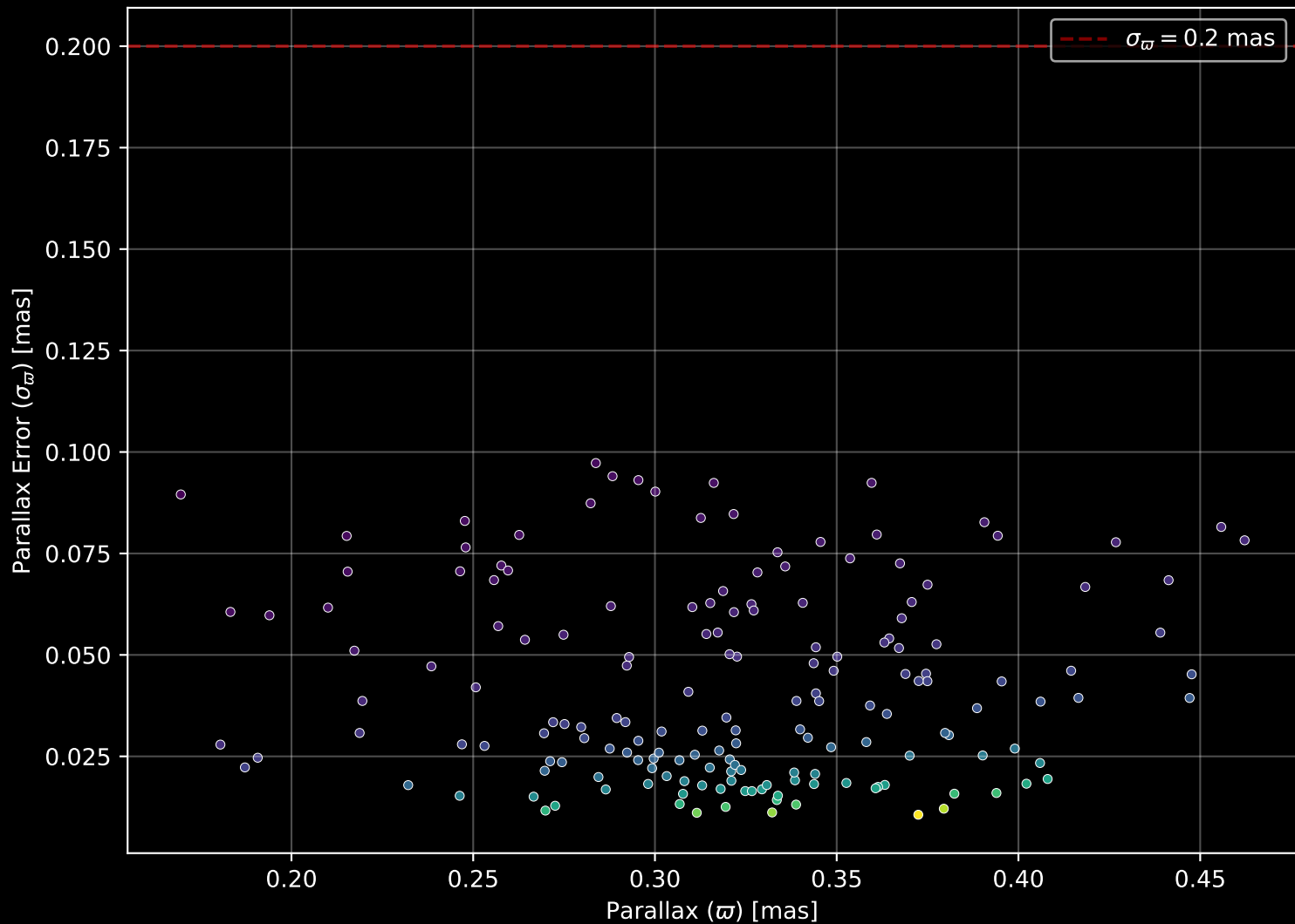
Gaia Cluster: [Gulliver_4] Parallax Quality (n= 171)
