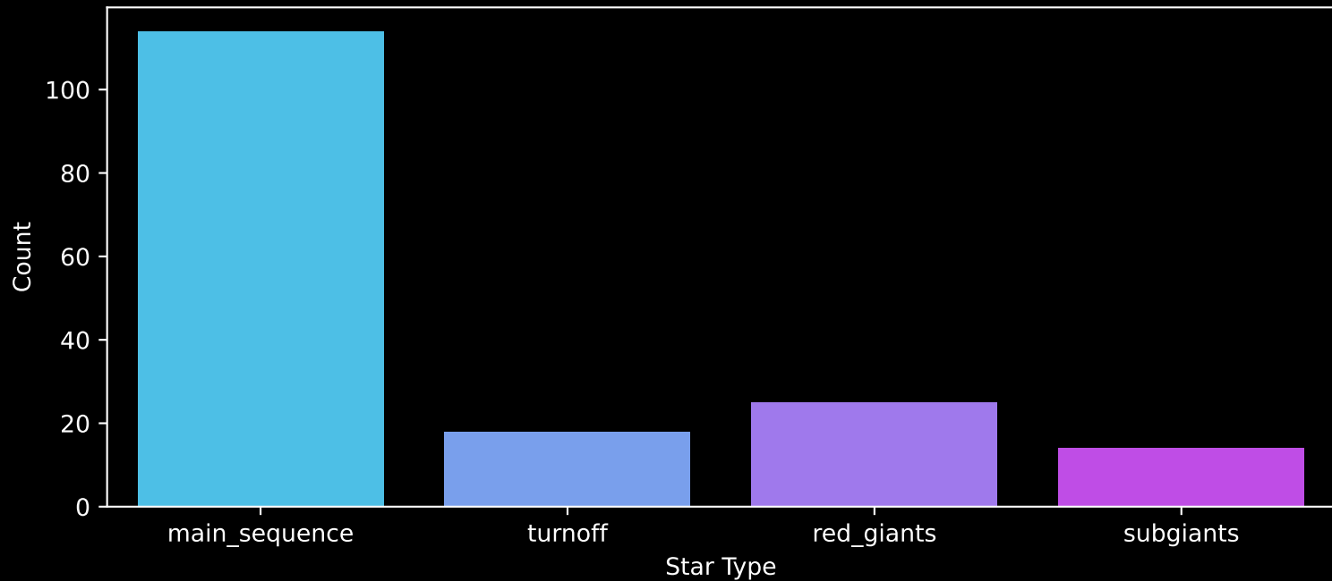
Gaia Cluster: [Gulliver_4] Count plot of Star Type
