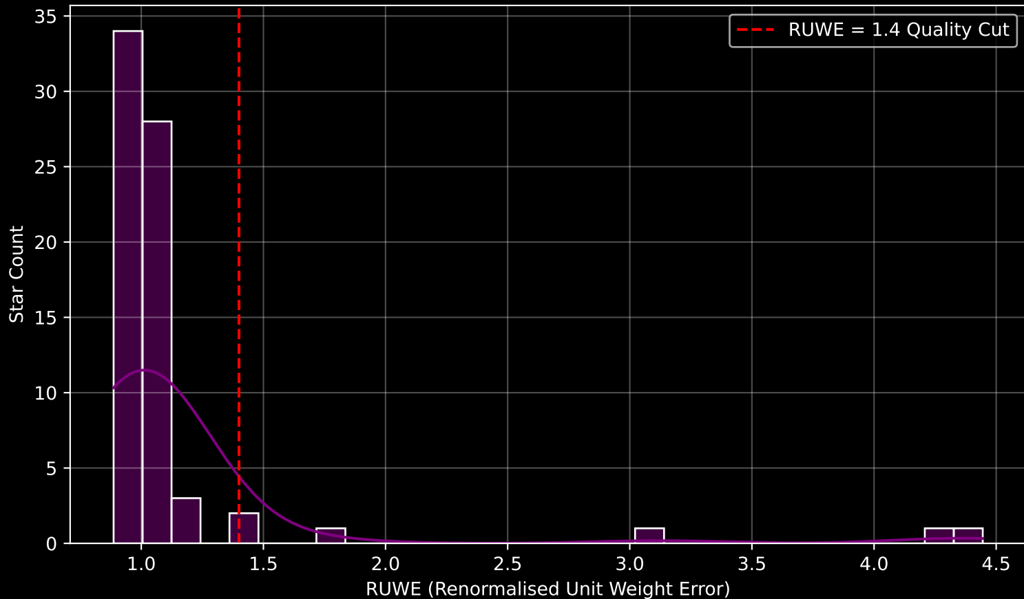
Gaia Cluster: [Gulliver_40] RUWE Distribution (n= 71)
