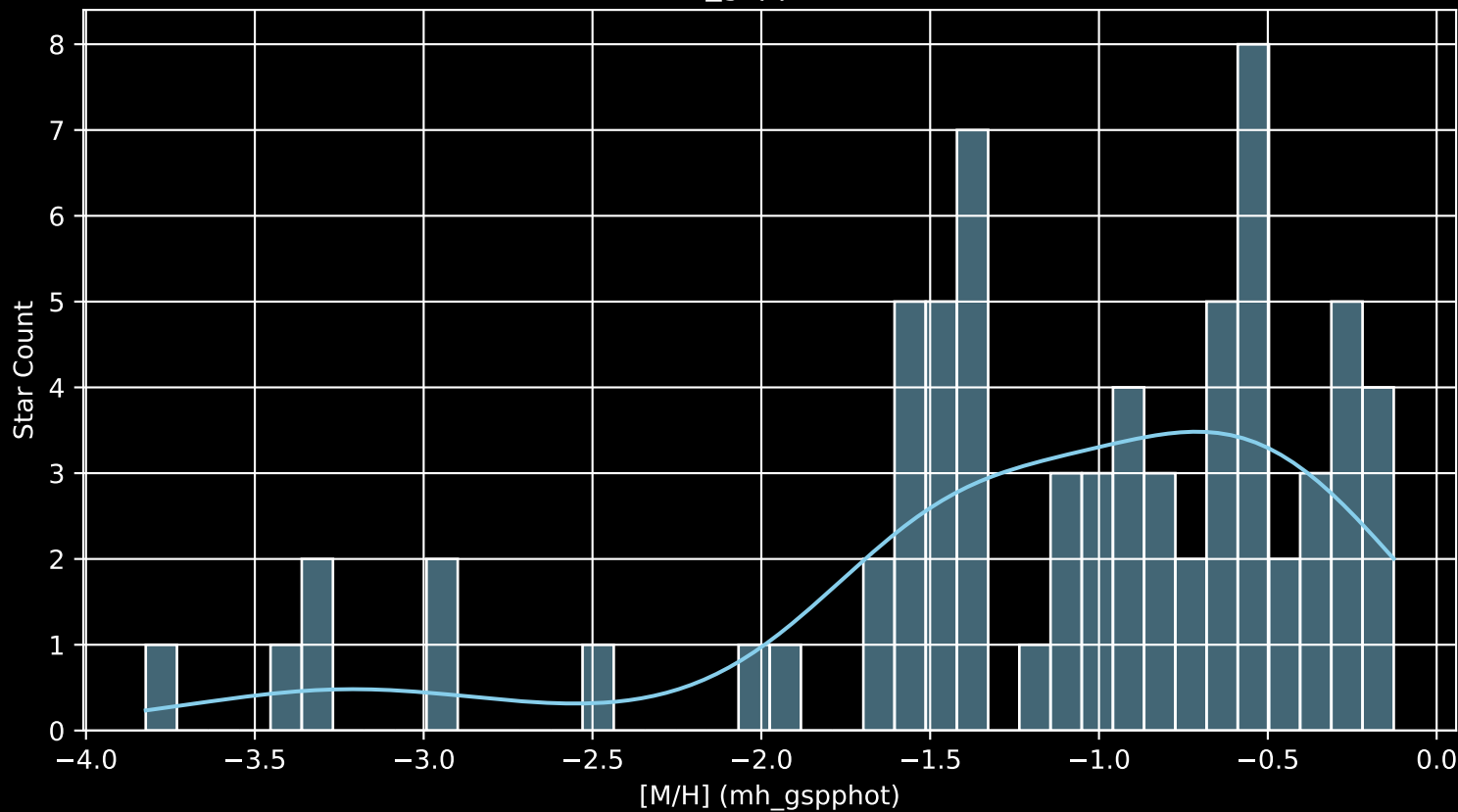
Gaia Cluster: [Gulliver_40 [M/H] (mh_gspphot) (n= 71)
