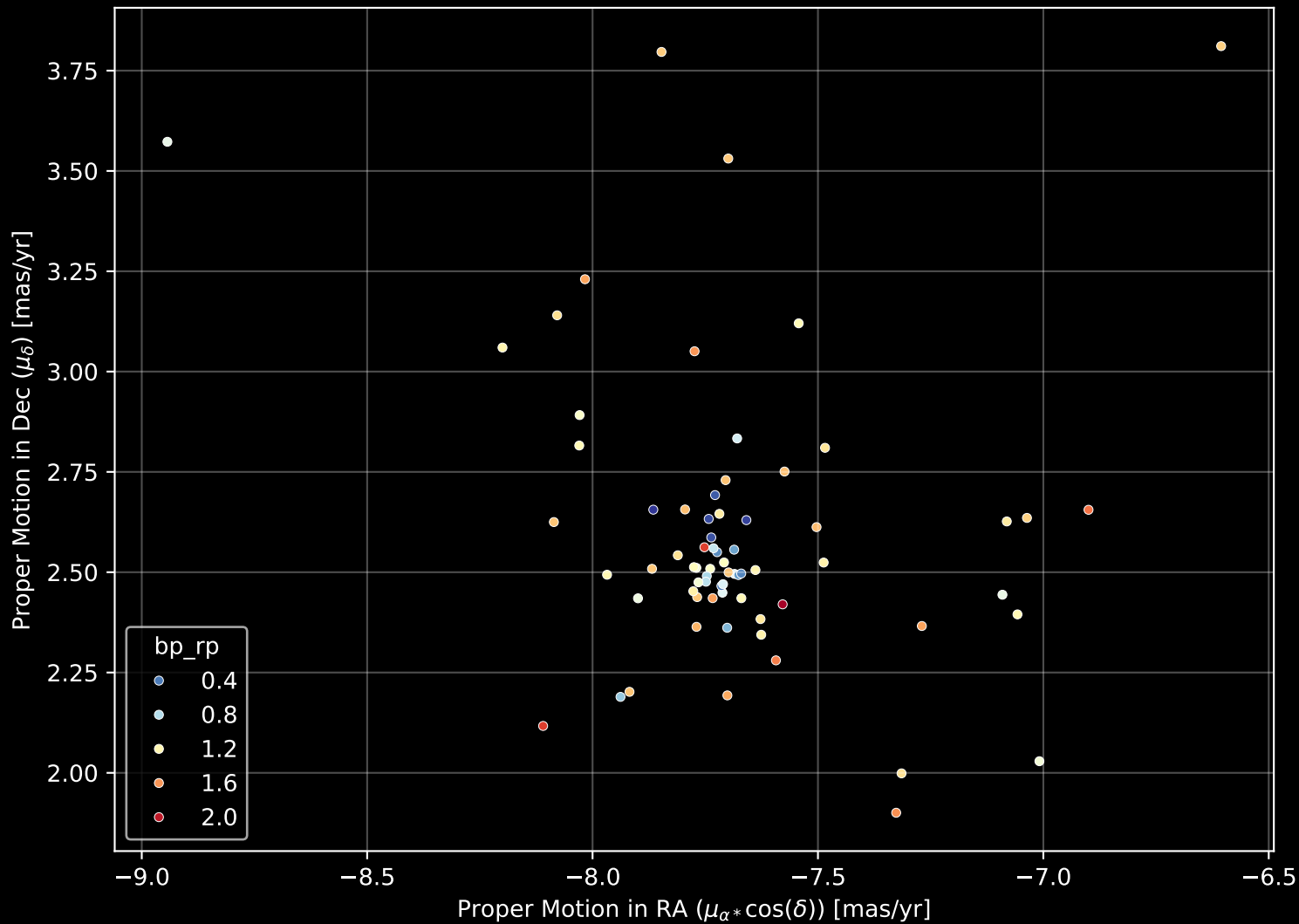
Gaia Cluster: [Gulliver_40] Proper Motion Diagram (n= 71)
