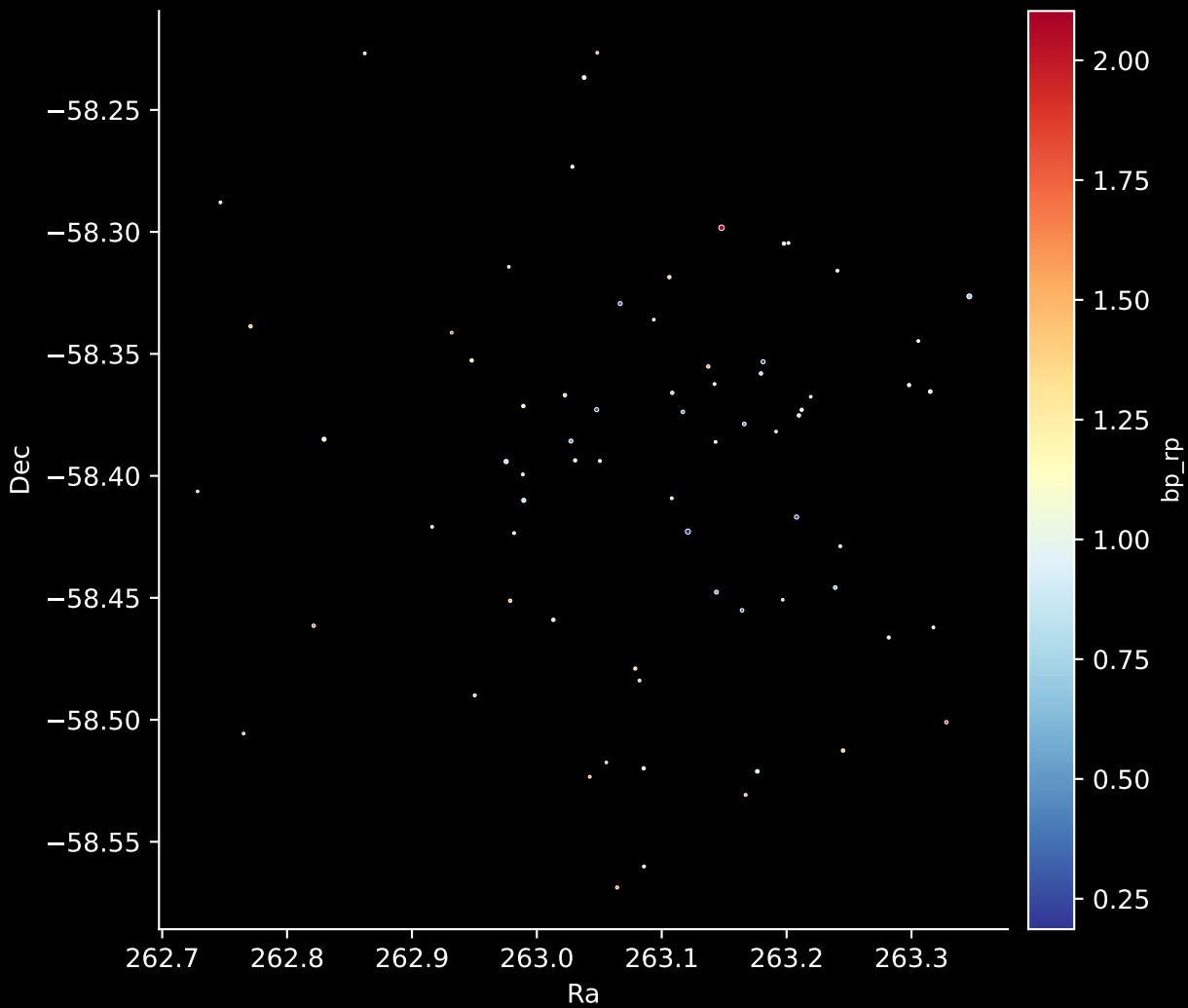
Gaia Cluster: [Gulliver_40] Stars: 71
