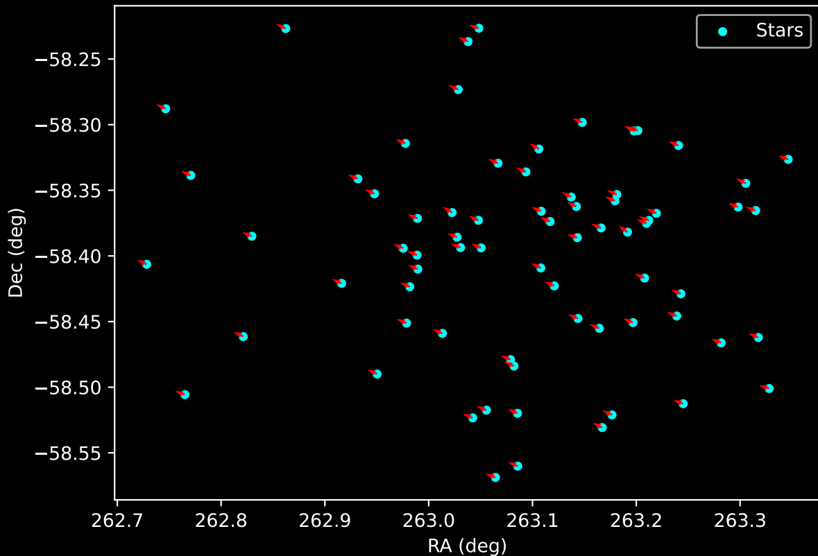
Gaia Cluster: [Gulliver_40] Proper Motion Vectors for Gaia Star Field (n= 71)
