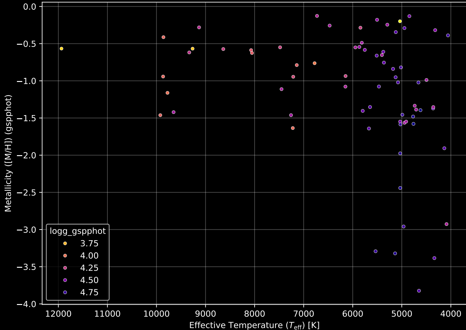
Gaia Cluster: [Gulliver_40] Stellar Population Parameters (n= 71)
