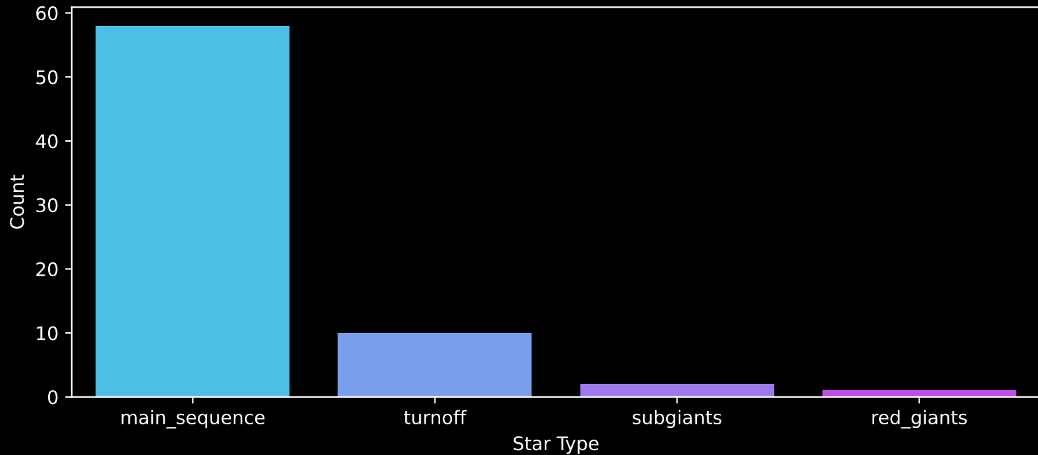
Gaia Cluster: [Gulliver_40] Count plot of Star Type
