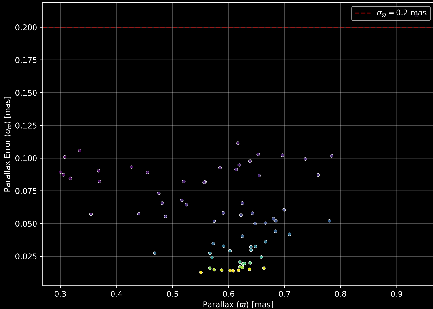
Gaia Cluster: [Gulliver_40] Parallax Quality (n= 71)
