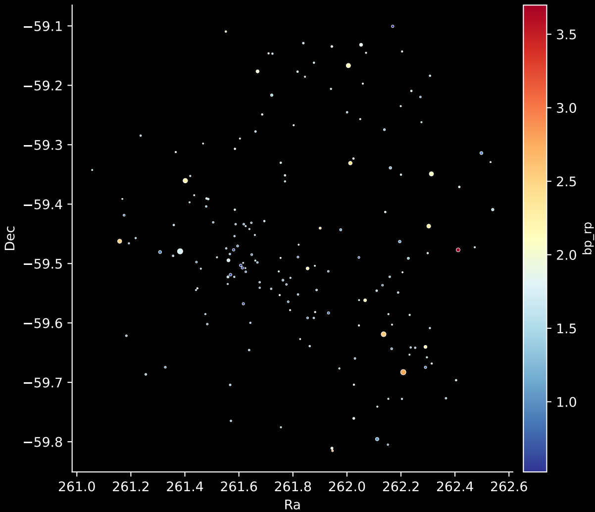
Gaia Cluster: [Gulliver_52] Stars: 174
