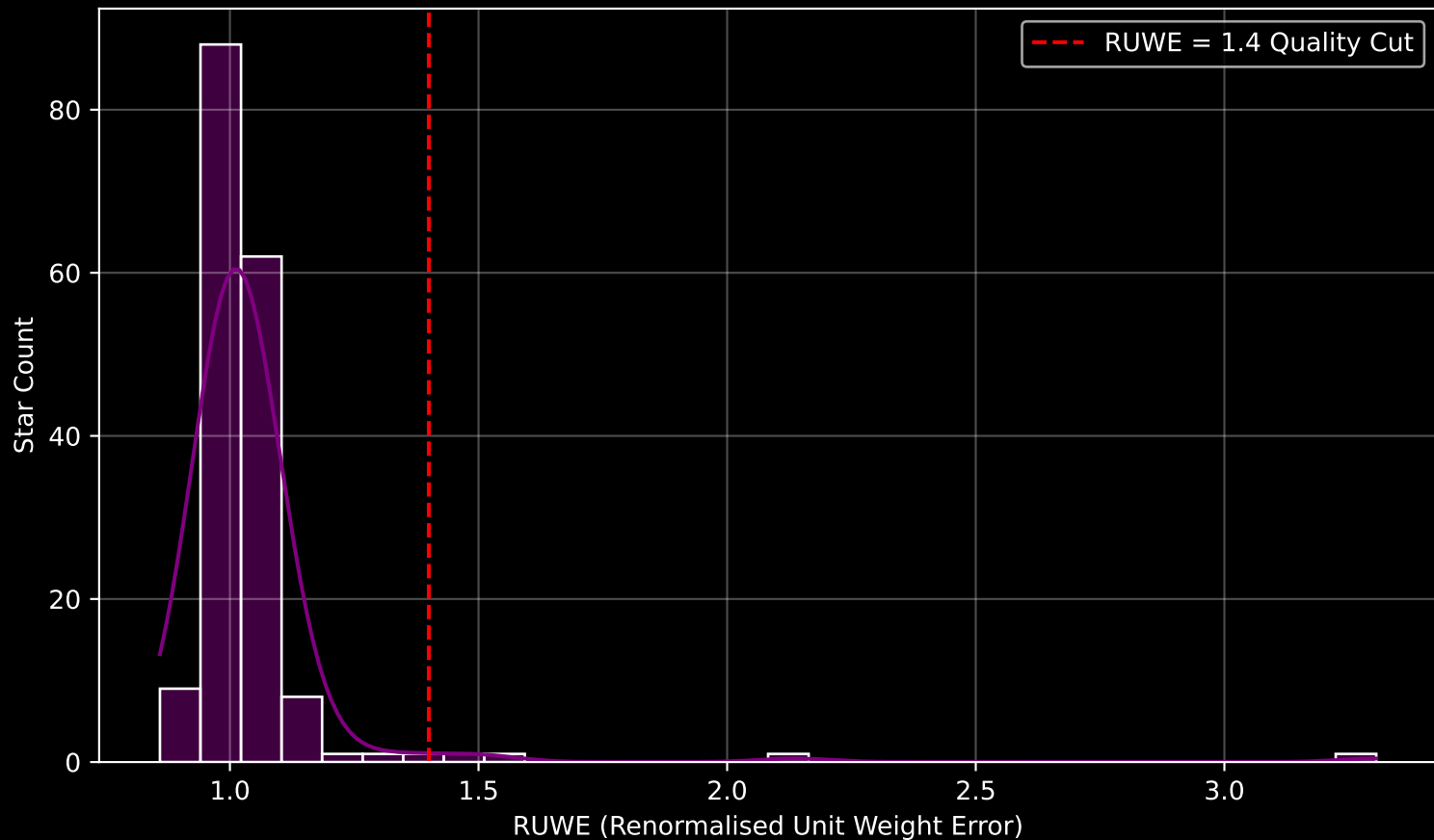
Gaia Cluster: [Gulliver_52] RUWE Distribution (n= 174)
