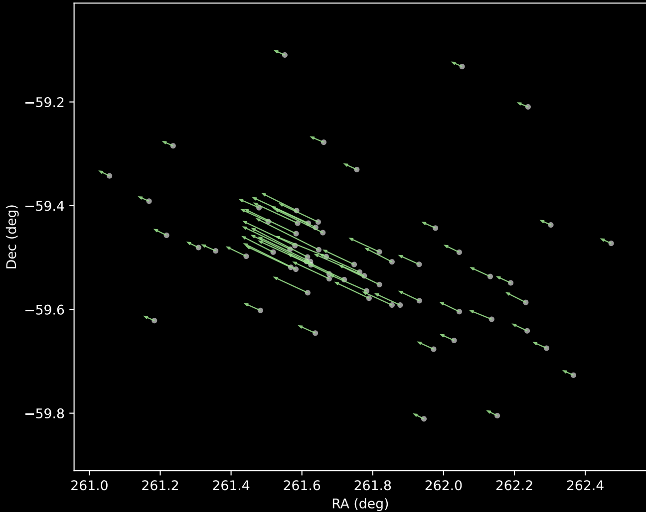
Gaia DR3 Cluster 5 Proper Motion Vectors (n=67)
