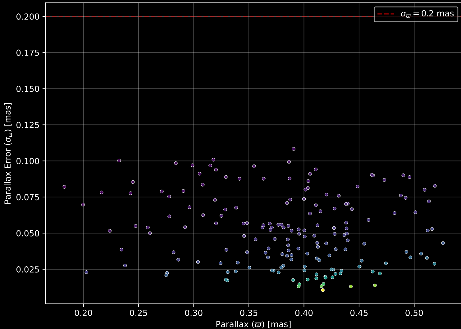
Gaia Cluster: [Gulliver_52] Parallax Quality (n= 174)
