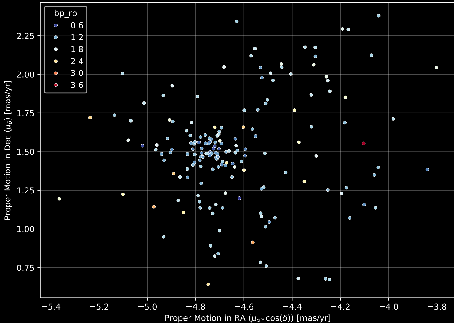
Gaia Cluster: [Gulliver_52] Proper Motion Diagram (n= 174)
