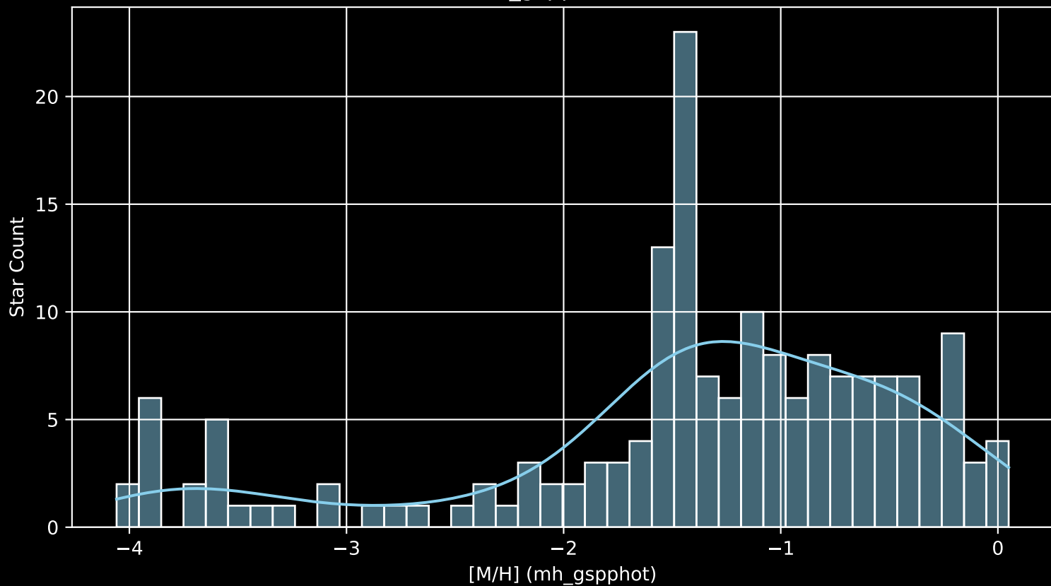
Gaia Cluster: [Gulliver_52 [M/H] (mh_gspphot) (n= 174)
