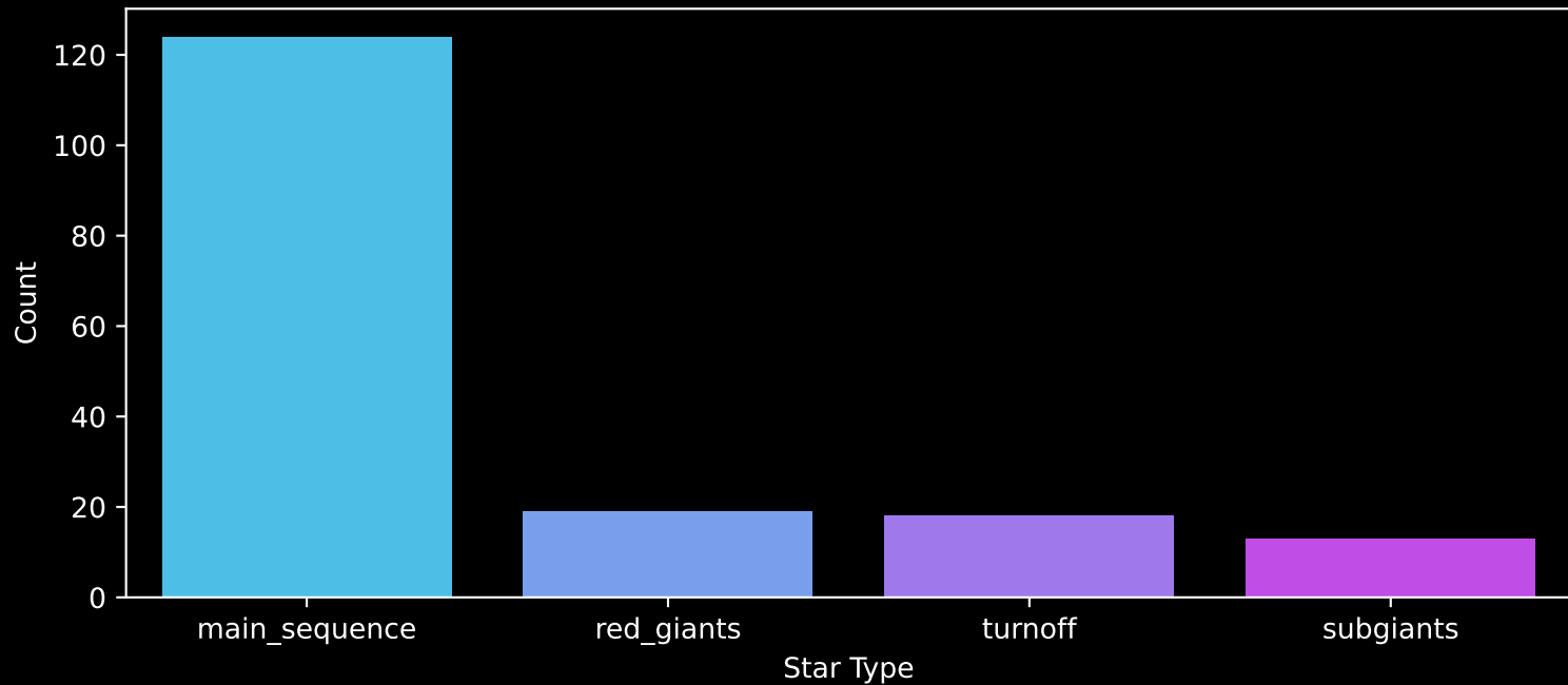
Gaia Cluster: [Gulliver_52] Count plot of Star Type
