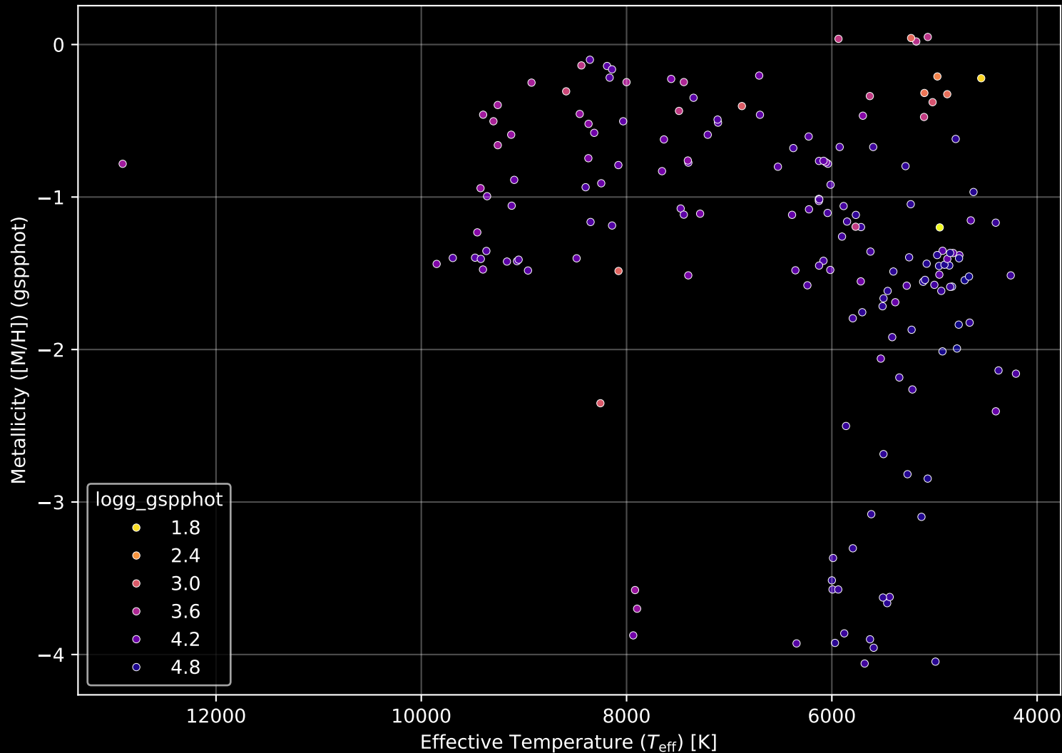
Gaia Cluster: [Gulliver_52] Stellar Population Parameters (n= 174)
